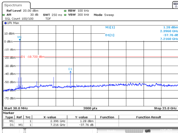
BLE_1M_Low_Channel
