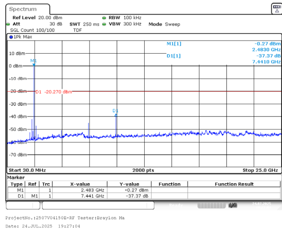
BLE_2M_High_Channel
