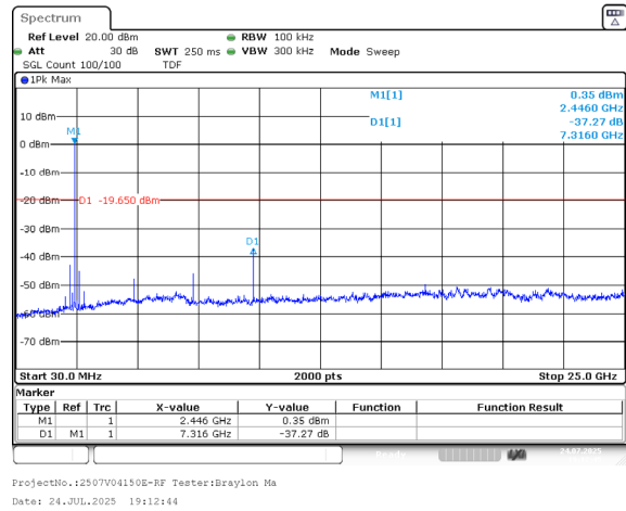
BLE_1M_Middle_Channel
