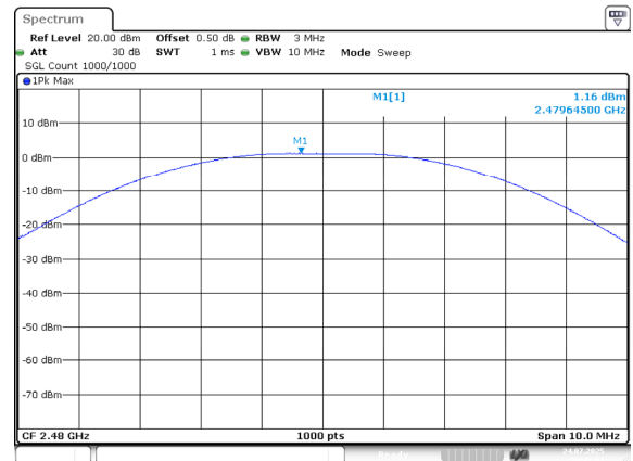
BLE_2M_High_Channel
