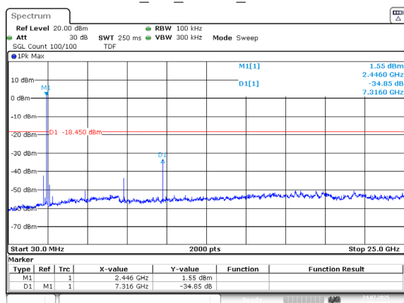
BLE_2M_Middle_Channel
