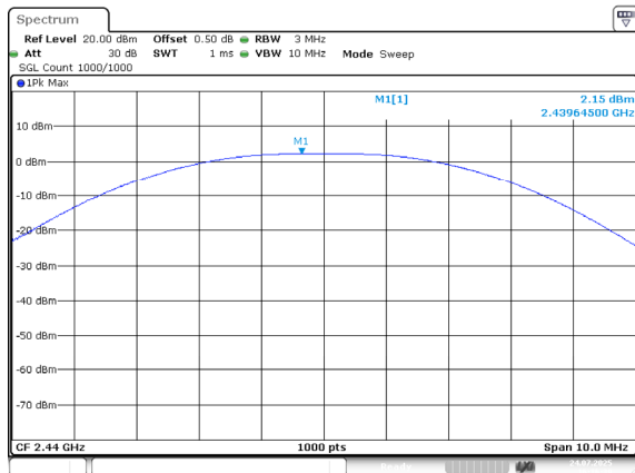
BLE_2M_Middle_Channel
