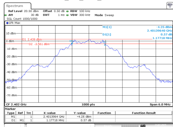
BLE_2M_Low_Channel
