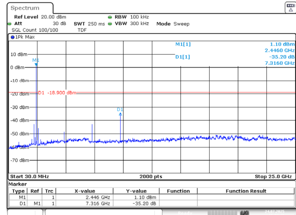
BLE_1M_Middle_Channel
