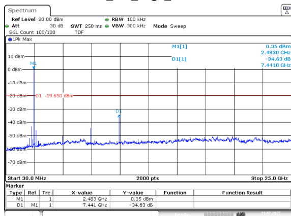
BLE_1M_High_Channel
