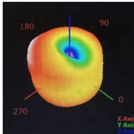
\phi=0^\circ , \theta=0^\circ , Frequency: 2480MHz, Gain; 0.89dBi
