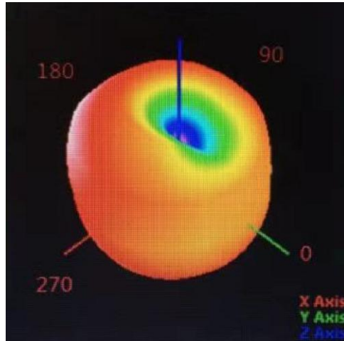
2441MHz \phi=0^\circ , \theta=0^\circ
