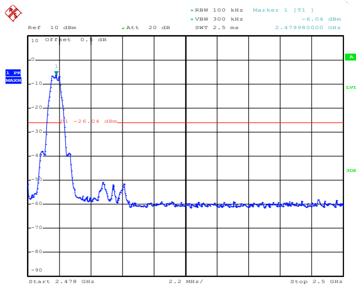
GFSK: Band Edge, Right Side
