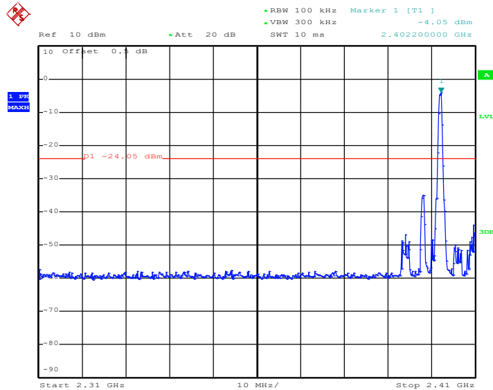
GFSK: Band Edge, Left Side
