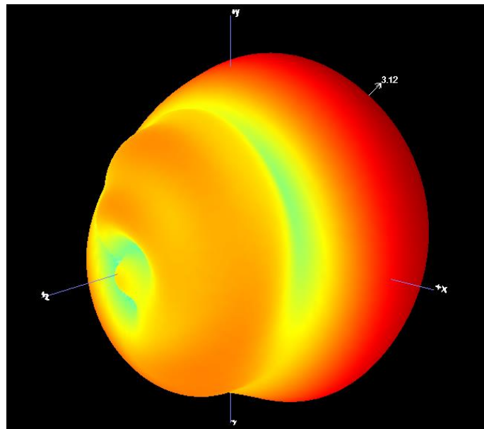
B1.2 3D Pattern for 2450MHz
