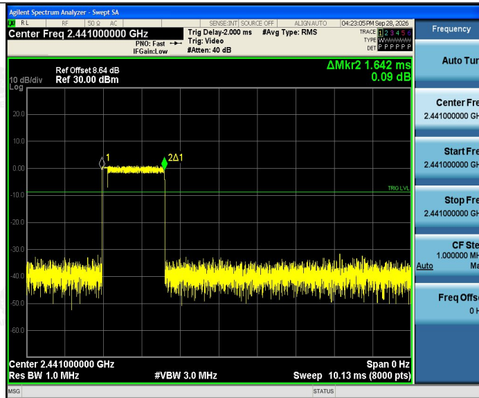
2DH3-Ant1-Hop-PASS
