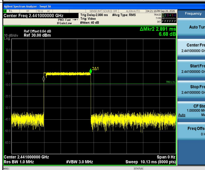
2DH5-Ant1-Hop-PASS
