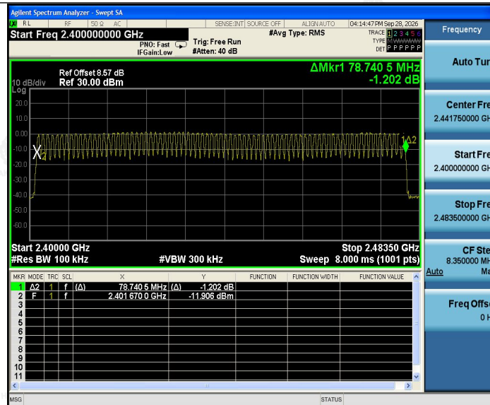
DH5-Ant1-Hop-PASS
