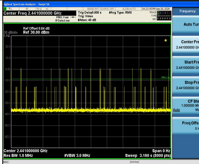
2DH3-Ant1-Hop-PASS
