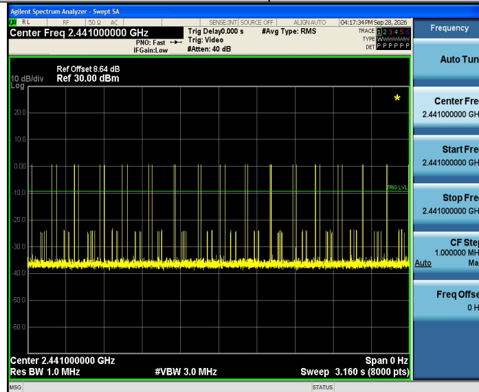
DH1-Ant1-Hop-PASS
