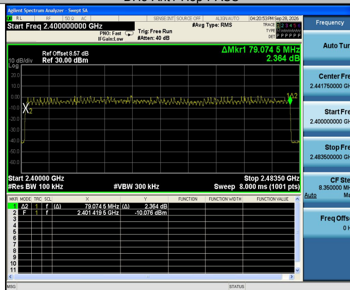
2DH5-Ant1-Hop-PASS
