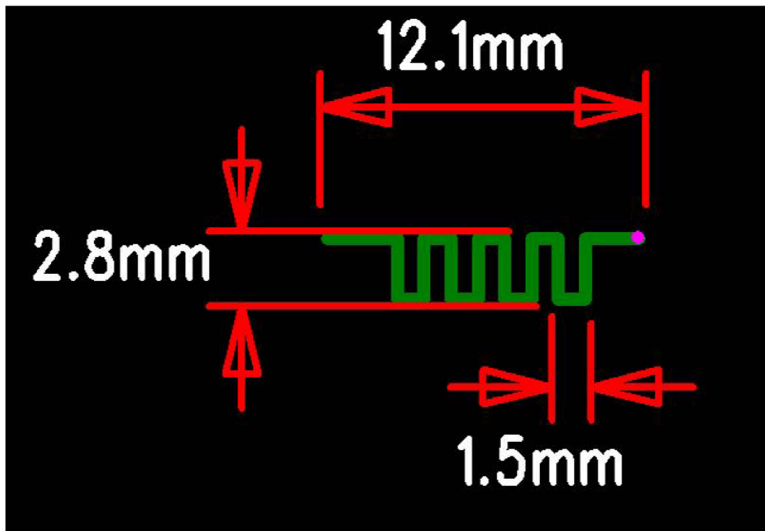
Picture of antenna and Antenna Dimensions
