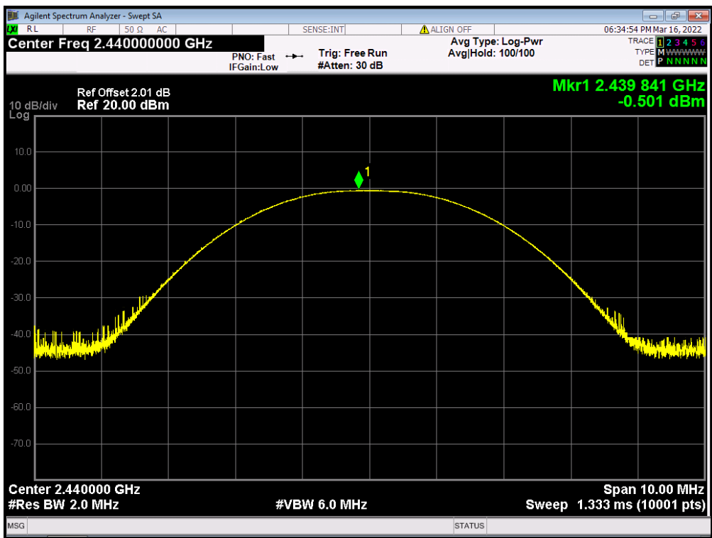
Channel 20:2.440GHz:
