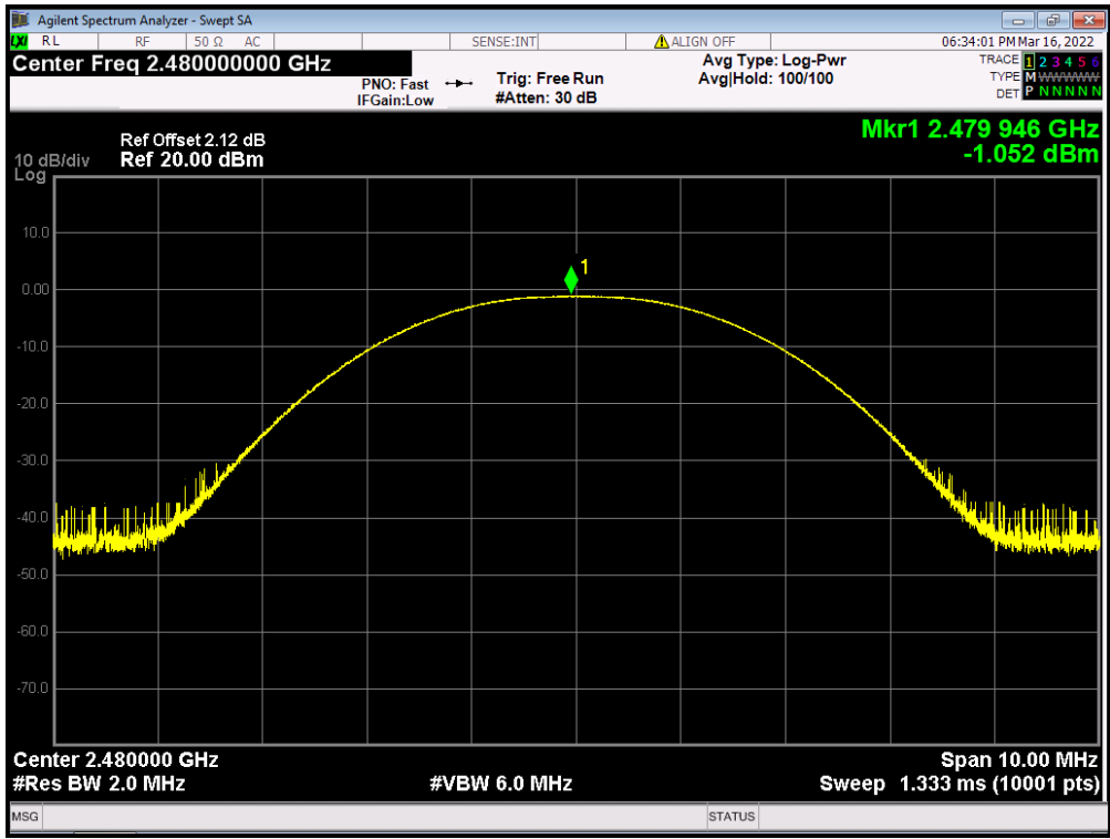
Channel 40:2.480GHz:
