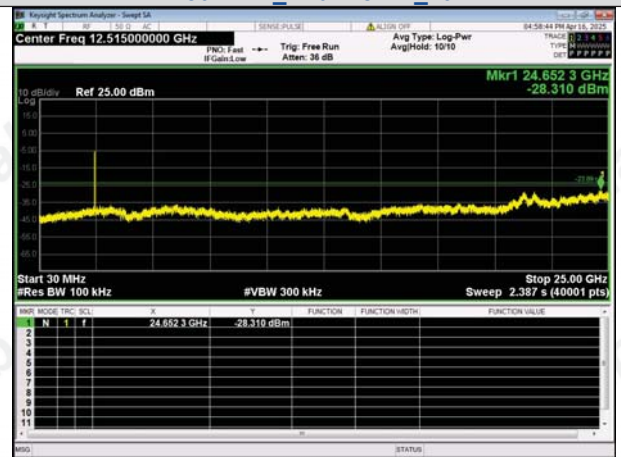
30.0 MHz - 25000.0 MHz IEEE 802.11n_Channel 11_20MHz
