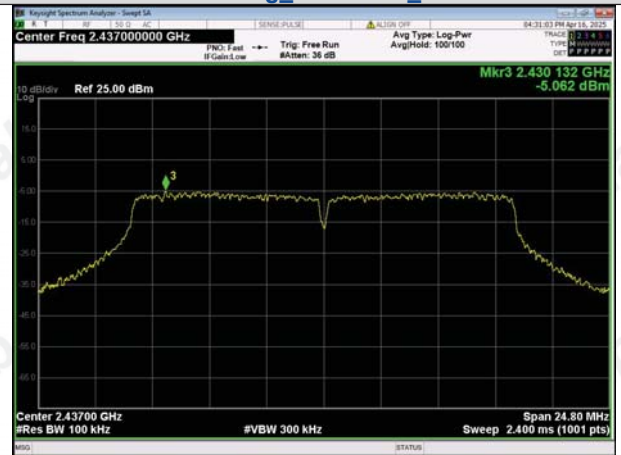
In-Band Reference Level IEEE 802.11g_Channel 6_20MHz
