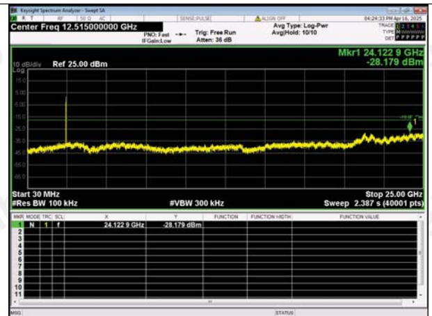
30.0 MHz - 25000.0 MHz IEEE 802.11b_Channel 11_20MHz
