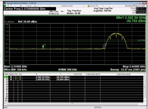
Out Of Band Emission IEEE 802.11b_Channel 1_20MHz
