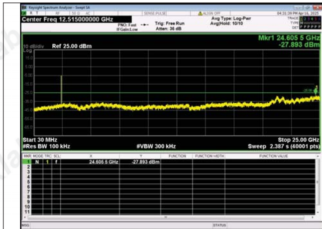
30.0 MHz - 25000.0 MHz IEEE 802.11g_Channel 6_20MHz
