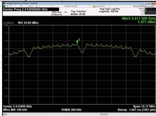
In-Band Reference Level IEEE 802.11b_Channel 1_20MHz
