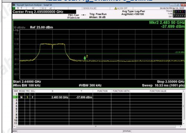
Out Of Band Emission IEEE 802.11g_Channel 11_20MHz
