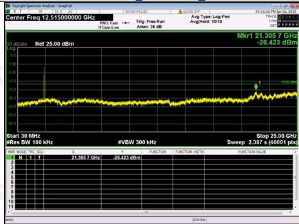
30.0 MHz - 25000.0 MHz IEEE 802.11b_Channel 1_20MHz
