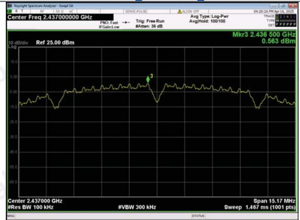
In-Band Reference Level IEEE 802.11b_Channel 6_20MHz
