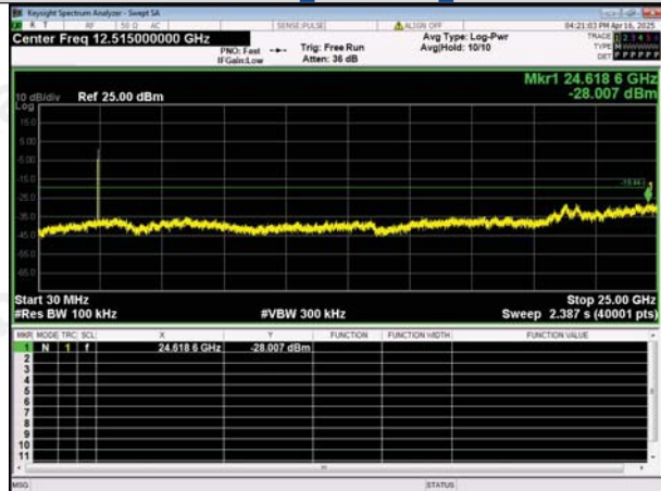
30.0 MHz - 25000.0 MHz IEEE 802.11b_Channel 6_20MHz
