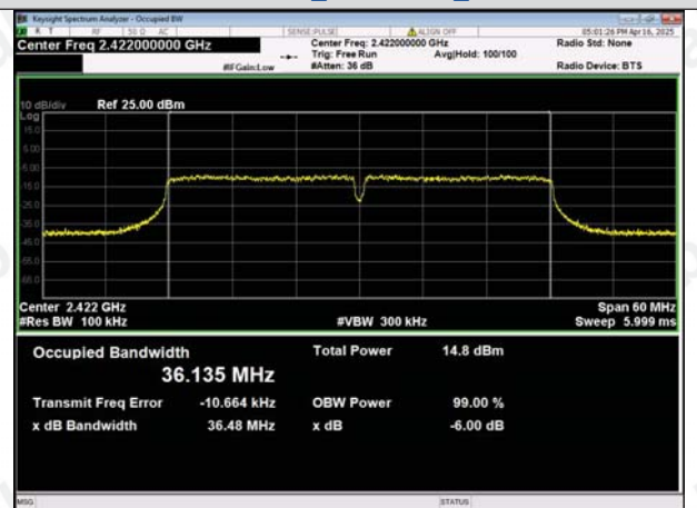
IEEE 802.11n_Channel 3_40MHz
