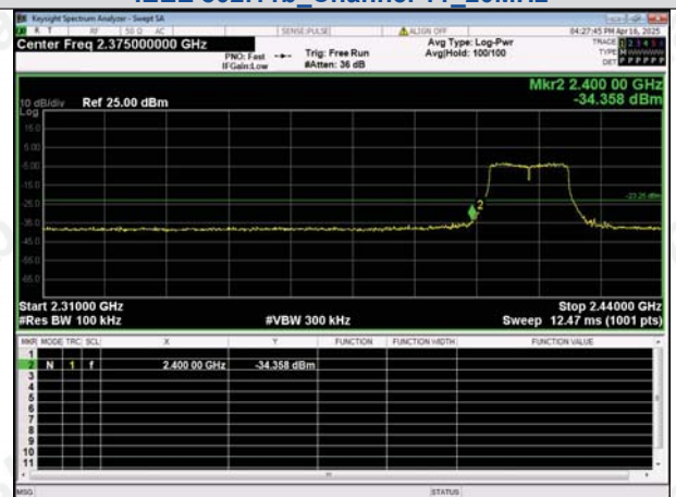
Out Of Band Emission IEEE 802.11g_Channel 1_20MHz
