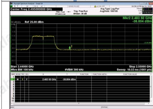
Out Of Band Emission IEEE 802.11n_Channel 11_20MHz
