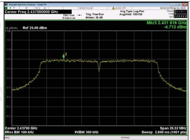
In-Band Reference Level IEEE 802.11n_Channel 6_20MHz
