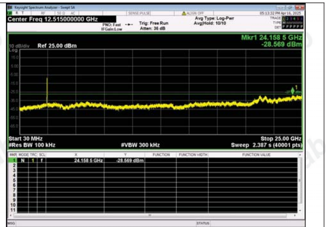
30.0 MHz - 25000.0 MHz IEEE 802.11n Channel 9 40MHz
