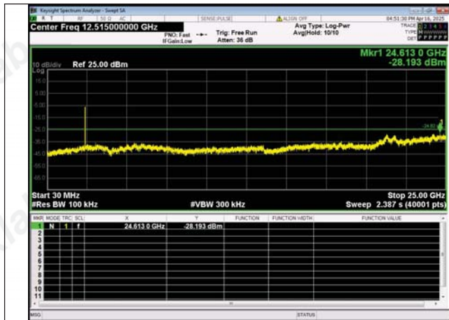
30.0 MHz - 25000.0 MHz IEEE 802.11n_Channel 1_20MHz
