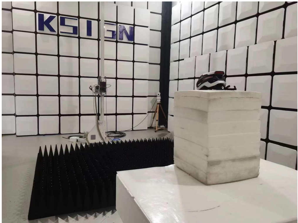
Emissions in frequency bands (above 1GHz)
