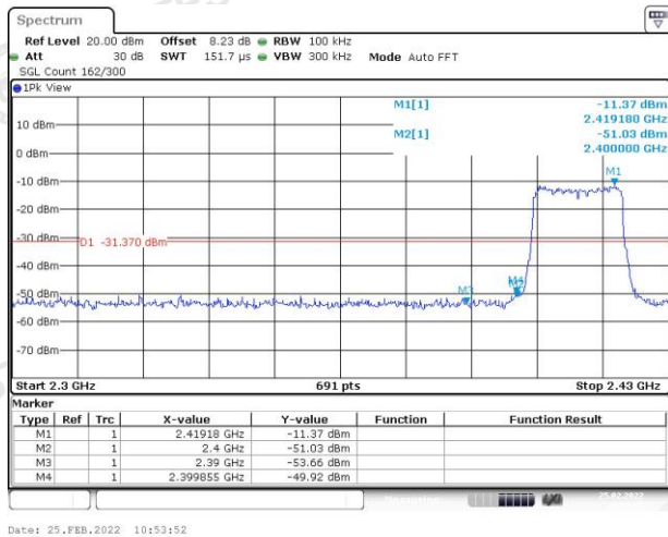
Left bandedge
