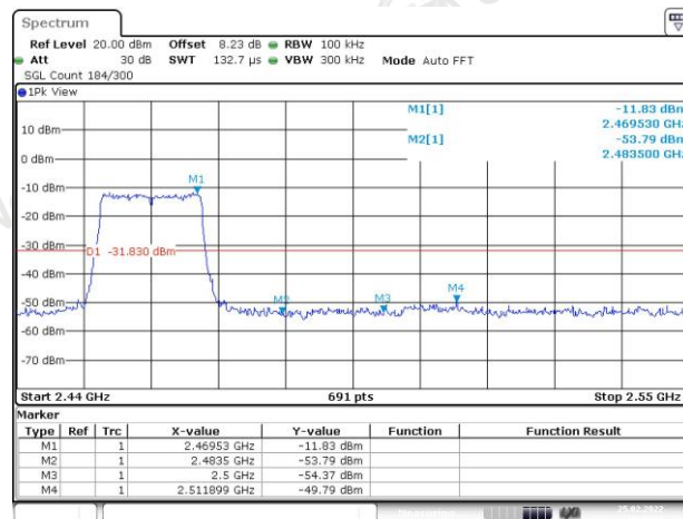
Right bandedge
