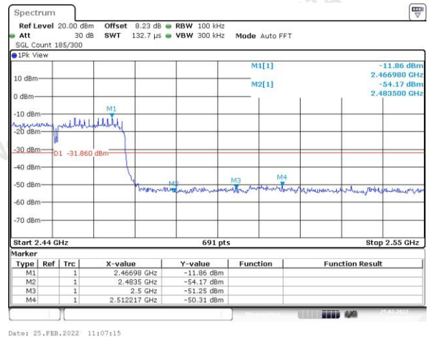
Right bandedge
