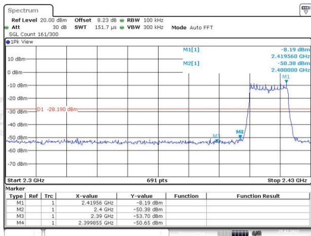
Left bandedge
