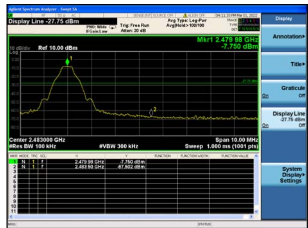
Right bandedge
