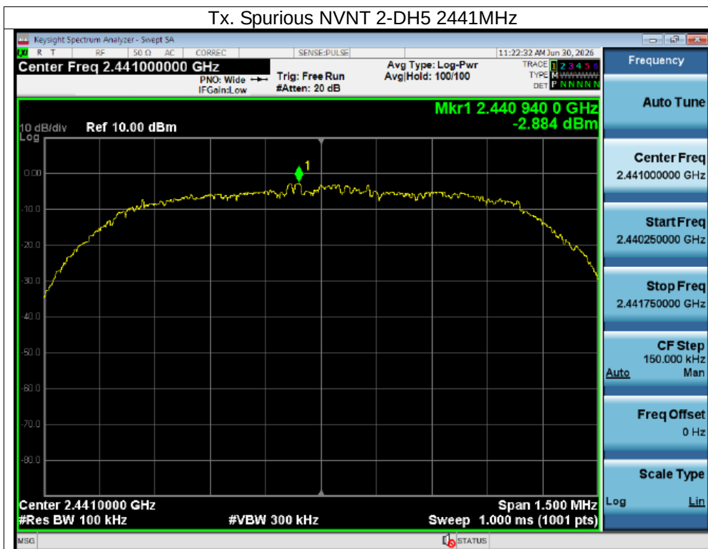
Tx. Spurious NVNT 2-DH5 2441MHz Emission
