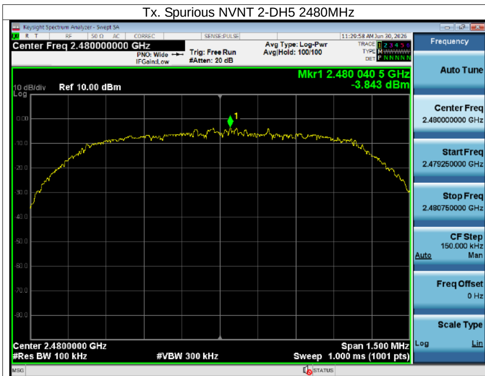
Tx. Spurious NVNT 2-DH5 2480MHz Emission
