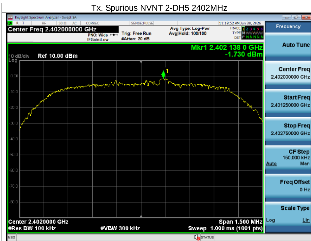
Tx. Spurious NVNT 2-DH5 2402MHz Emission
