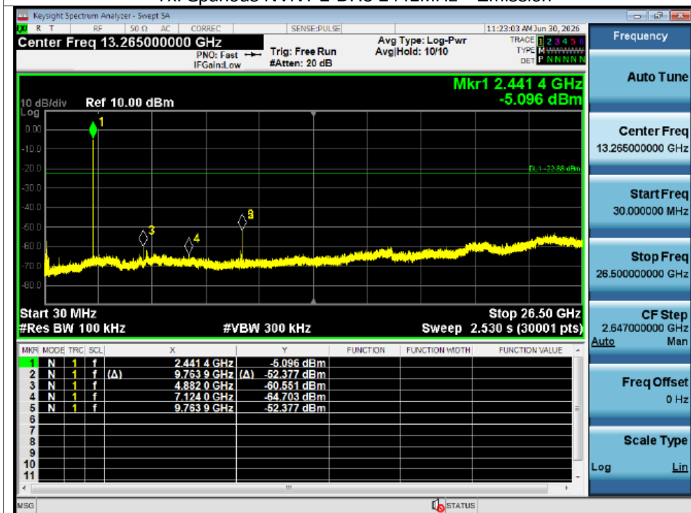
Tx. Spurious NVNT 2-DH5 2441MHz Emission
