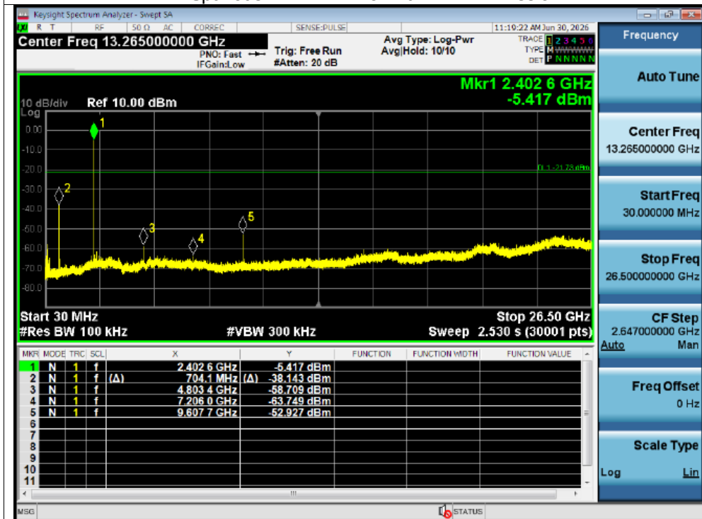
Tx. Spurious NVNT 2-DH5 2402MHz Emission
