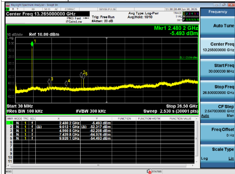
Tx. Spurious NVNT 2-DH5 2480MHz Emission
