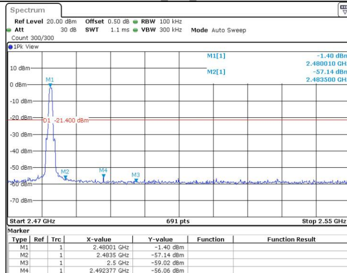
BLE_High_2480
