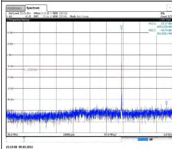
Band12-1.4MHz-16QAM-23017-1RB#0-Rang e1:30~1000MHz
