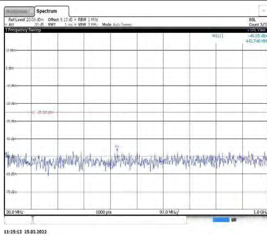
Band7-15MHz-QPSK-20825-1RB#0-Range1: 30~1000MHz
