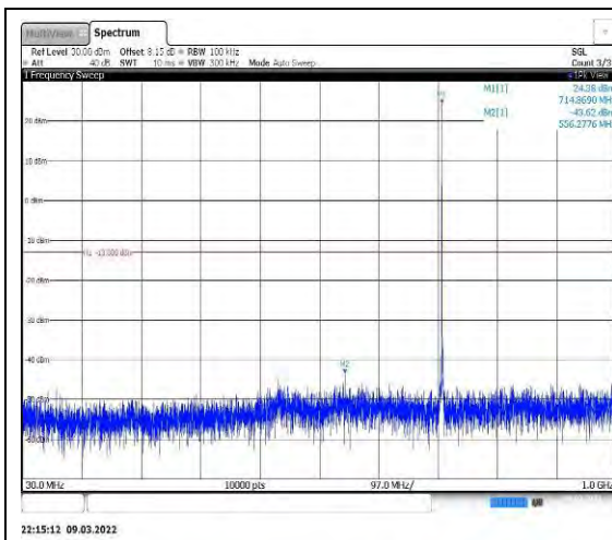
Band12-1.4MHz-QPSK-23173-1RB#0-Range 1:30~1000MHz
