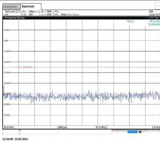
Band7-15MHz-QPSK-21100-1RB#0-Range1: 30~1000MHz
