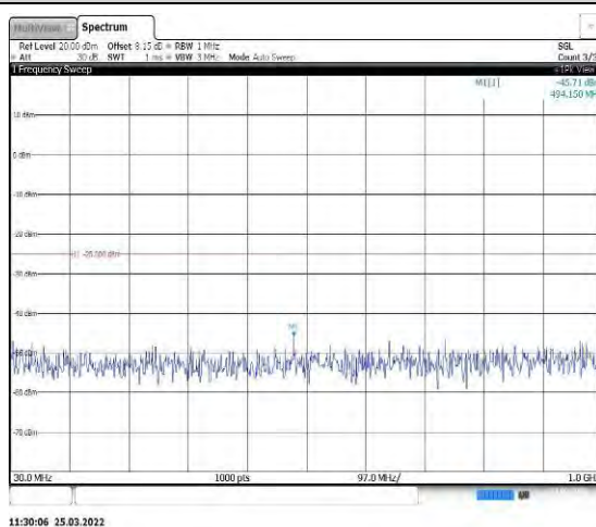
Band7-20MHz-QPSK-21350-1RB#0-Range1: 30~1000MHz
