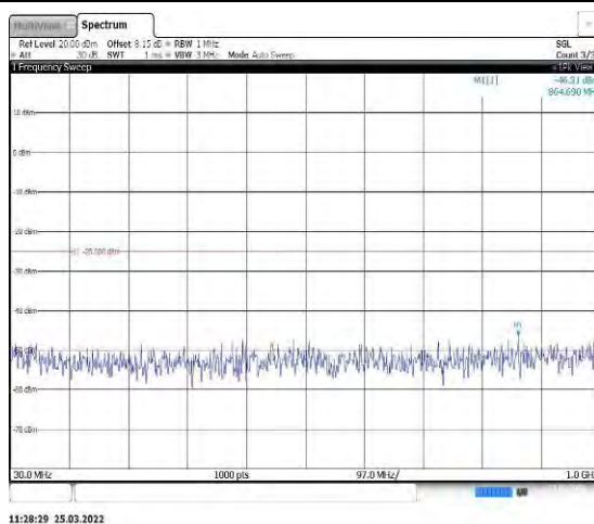
Band7-20MHz-QPSK-20850-1RB#0-Range1: 30~1000MHz
