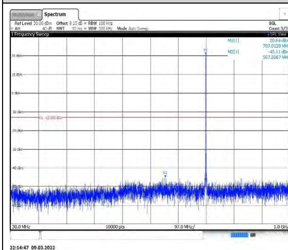
Band12-1.4MHz-16QAM-23095-1RB#0-Rang e1:30~1000MHz
