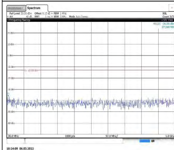
Band2-15MHz-16QAM-18900-1RB#0-Range 1:30~1000MHz
