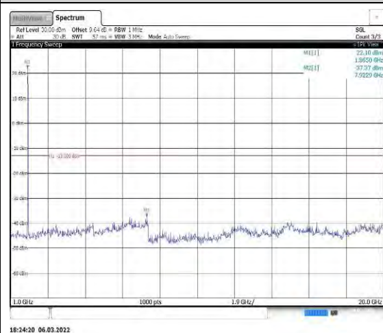
Band2-15MHz-16QAM-18900-1RB#0-Range 2:1000~20000MHz
