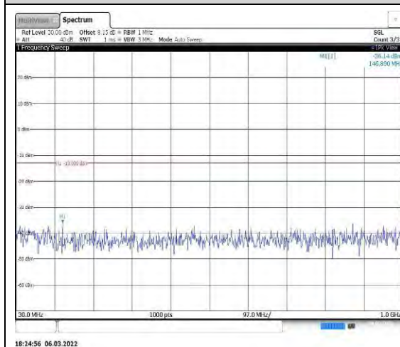
Band2-15MHz-16QAM-19125-1RB#0-Range 1:30~1000MHz
