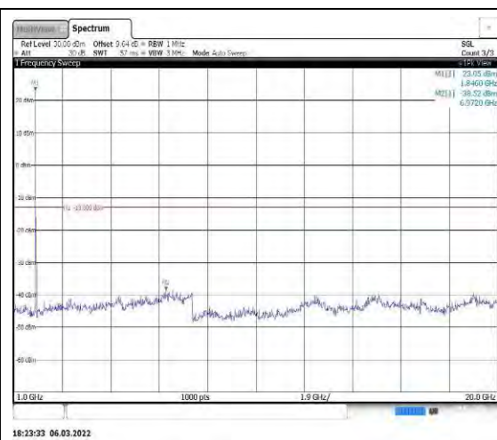
Band2-15MHz-16QAM-18675-1RB#0-Range 2:1000~20000MHz
