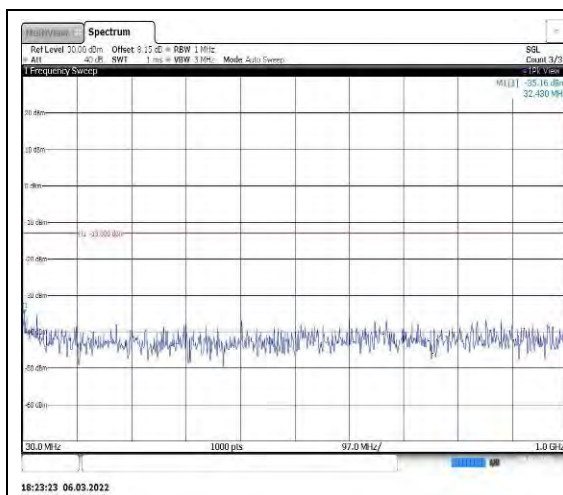
Band2-15MHz-16QAM-18675-1RB#0-Range 1:30~1000MHz
