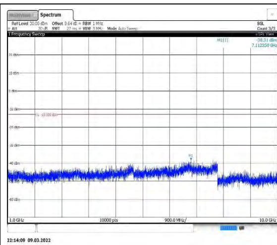
Band12-1.4MHz-16QAM-23017-1RB#0-Ran ge2:1000~10000MHz
