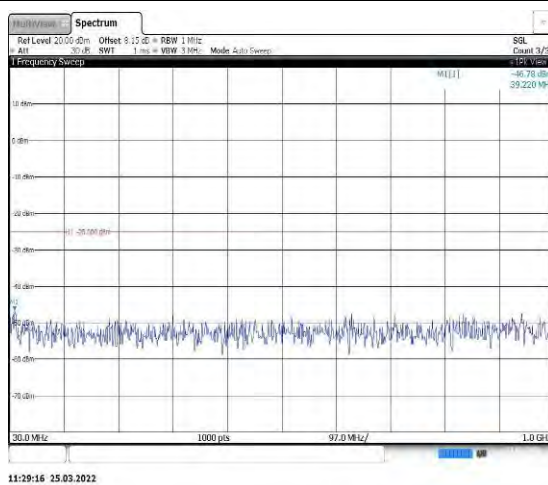
Band7-20MHz-QPSK-21100-1RB#0-Range1: 30~1000MHz
