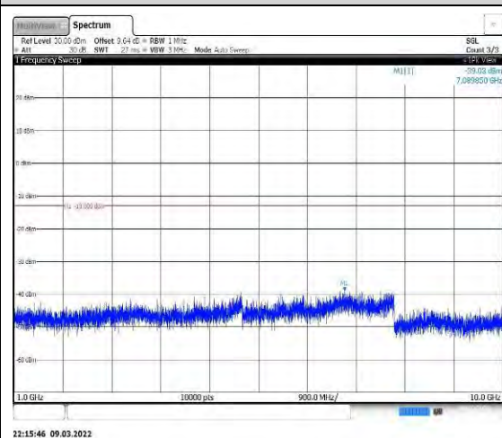
Band12-1.4MHz-16QAM-23173-1RB#0-Ran ge2:1000~10000MHz
