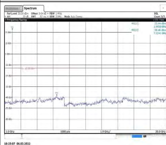
Band2-15MHz-16QAM-19125-1RB#0-Range 2:1000~20000MHz
