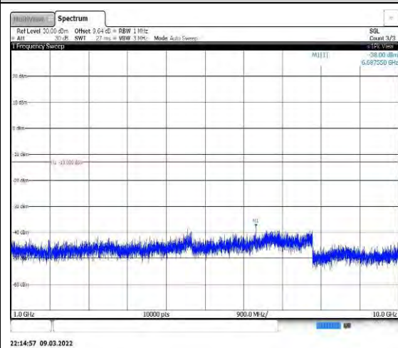
Band12-1.4MHz-16QAM-23095-1RB#0-Ran ge2:1000~10000MHz
