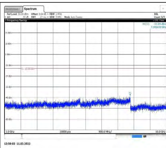
Band26-10MHz-QPSK-26740-1RB#0-Range 2:1000~10000MHz
