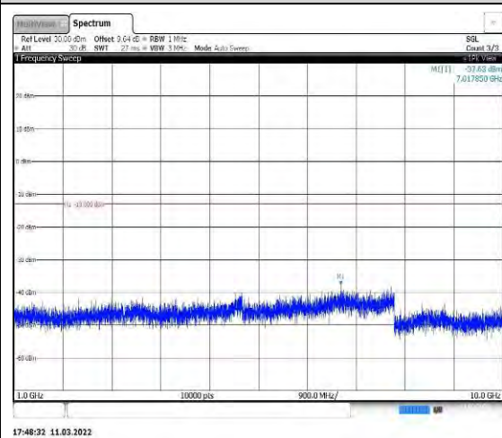
Band26-10MHz-QPSK-26840-1RB#0-Range 2:1000~10000MHz
