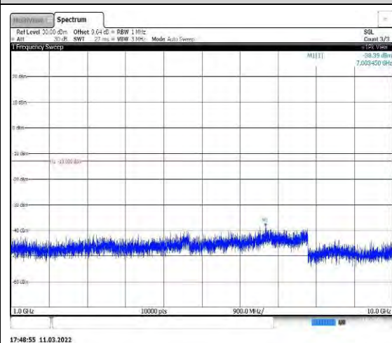
Band26-10MHz-16QAM-26840-1RB#0-Rang e2:1000~10000MHz
