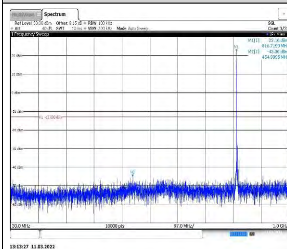
Band26-5MHz-QPSK-26740-1RB#0-Range1: 30~1000MHz
