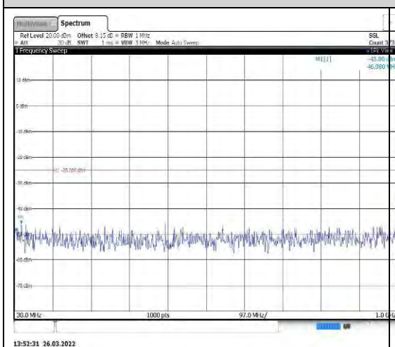
Band38-5MHz-QPSK-37775-1RB#0-Range 1:30~1000MHz
