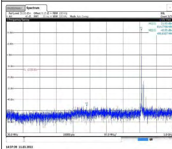
Band26-15MHz-16QAM-26765-1RB#0-Rang e1:30~1000MHz
