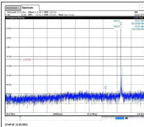
Band26-10MHz-QPSK-26915-1RB#0-Range 1:30~1000MHz
