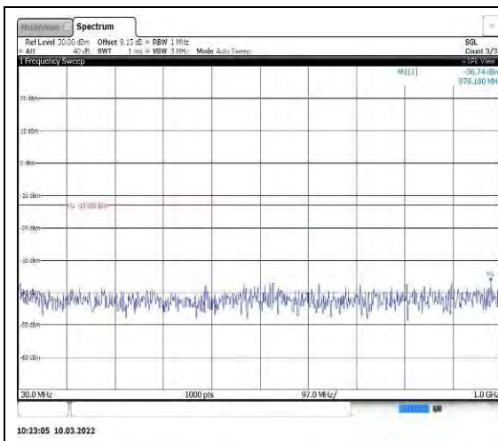
Band25-3MHz-16QAM-26675-1RB#0-Range 1:30~1000MHz
