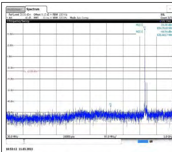
Band26-15MHz-QPSK-26965-1RB#0-Range 1:30~1000MHz
