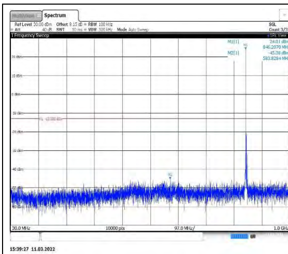
Band26-3MHz-16QAM-27025-1RB#0-Range 1:30~1000MHz
