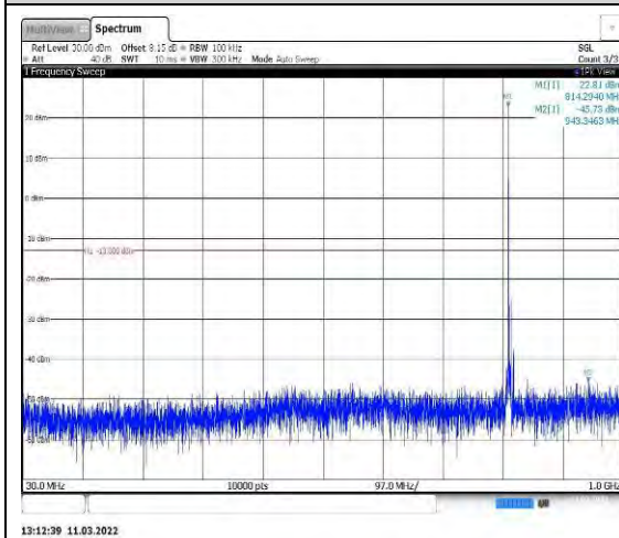
Band26-5MHz-QPSK-26715-1RB#0-Range1: 30~1000MHz
