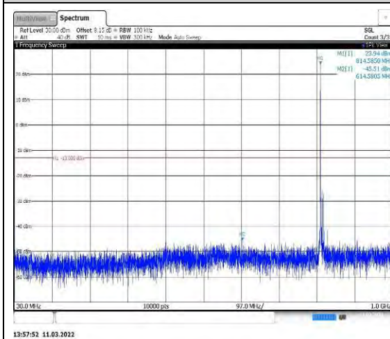
Band26-10MHz-QPSK-26740-1RB#0-Range 1:30~1000MHz
