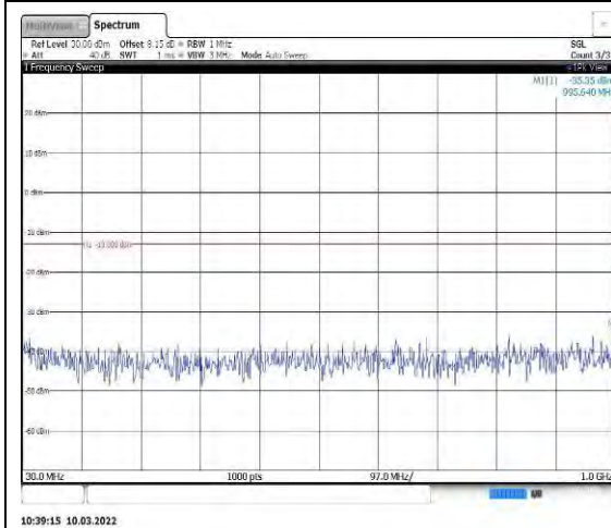
Band25-5MHz-QPSK-26065-1RB#0-Range1: 30~1000MHz
