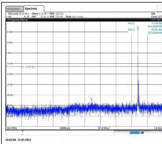
Band26-5MHz-16QAM-27015-1RB#0-Range 1:30~1000MHz
