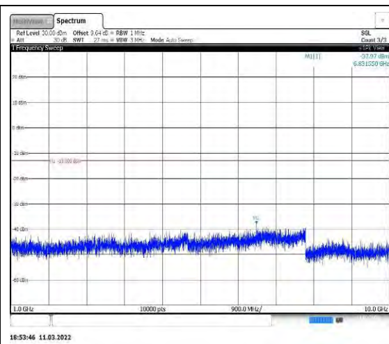
Band26-15MHz-16QAM-26965-1RB#0-Rang e2:1000~10000MHz
