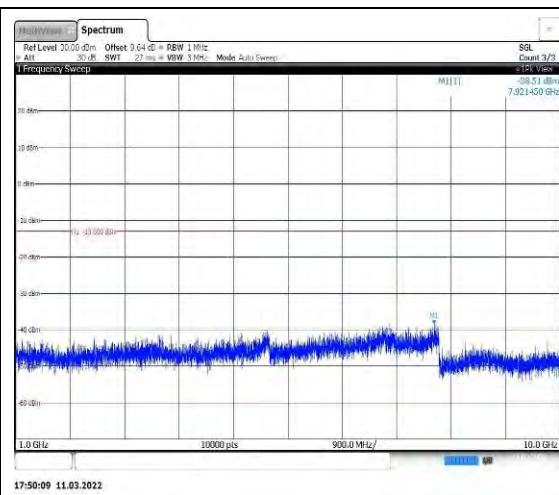
Band26-10MHz-QPSK-26990-1RB#0-Range 2:1000~10000MHz
