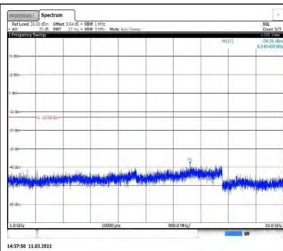
Band26-15MHz-16QAM-26765-1RB#0-Rang e2:1000~10000MHz
