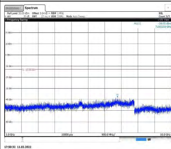
Band26-10MHz-16QAM-26990-1RB#0-Rang e2:1000~10000MHz
