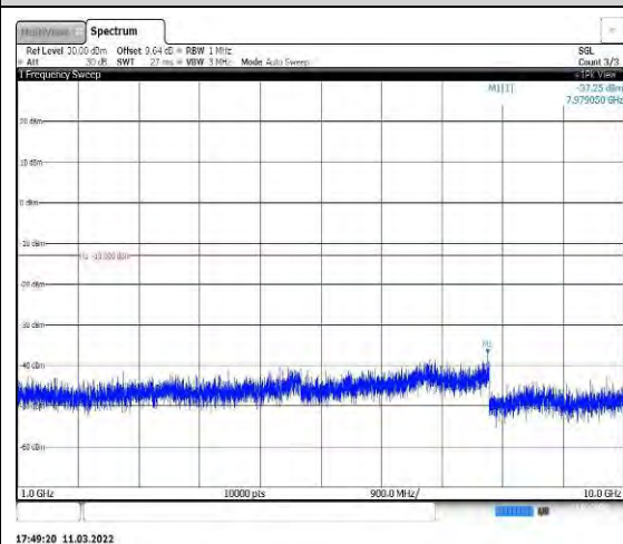
Band26-10MHz-QPSK-26915-1RB#0-Range 2:1000~10000MHz
