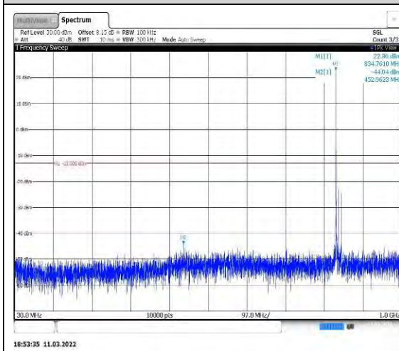
Band26-15MHz-16QAM-26965-1RB#0-Rang e1:30~1000MHz
