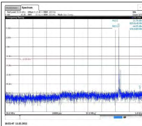
Band26-15MHz-16QAM-26915-1RB#0-Rang e1:30~1000MHz
