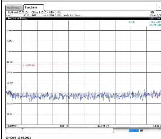
Band25-5MHz-QPSK-26365-1RB#0-Range1: 30~1000MHz
