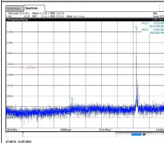
Band26-10MHz-QPSK-26840-1RB#0-Range 1:30~1000MHz
