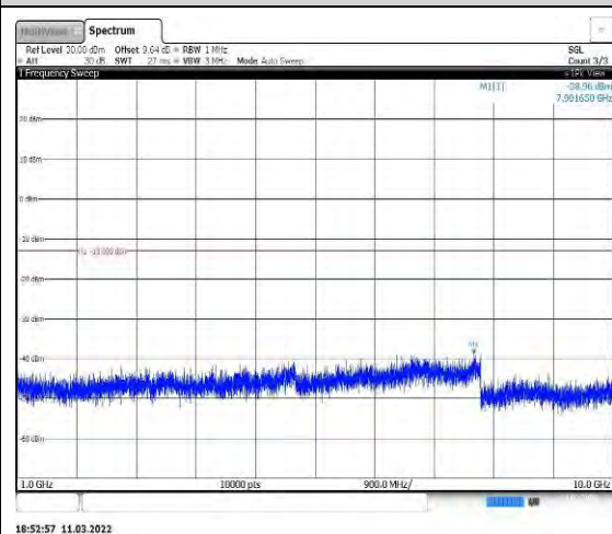
Band26-15MHz-16QAM-26915-1RB#0-Rang e2:1000~10000MHz
