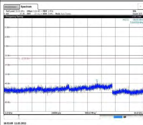
Band26-15MHz-16QAM-26865-1RB#0-Rang e2:1000~10000MHz
