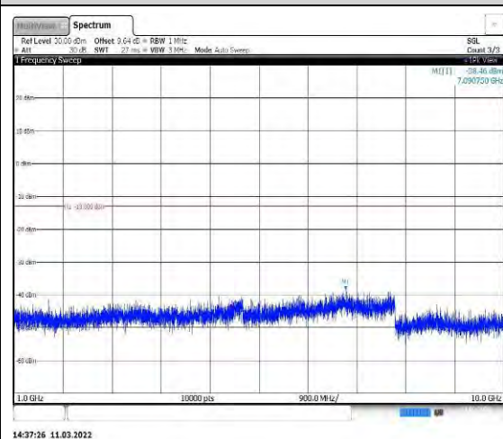
Band26-15MHz-QPSK-26765-1RB#0-Range 2:1000~10000MHz
