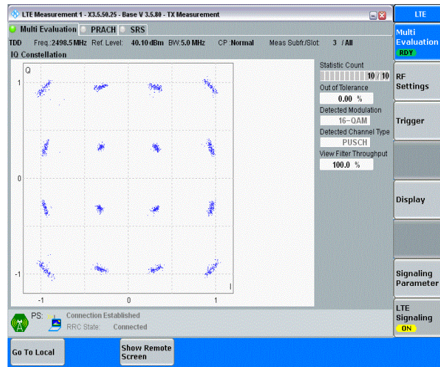
Band41-5MHz-16QAM-40065-25RB#0
