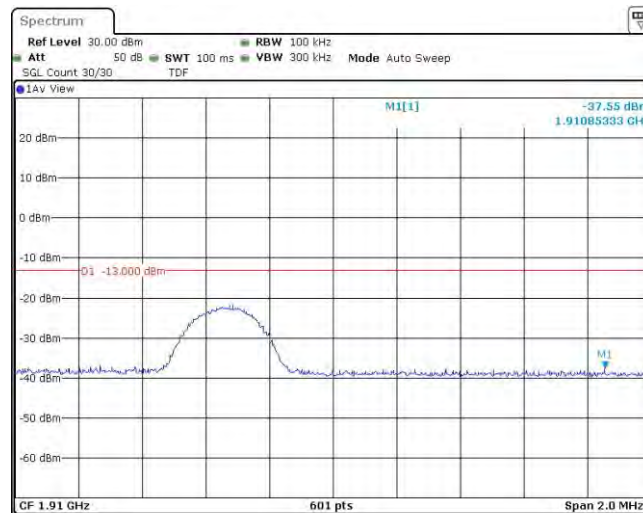
Band2-5MHz-16QAM-19175-1RB#24
