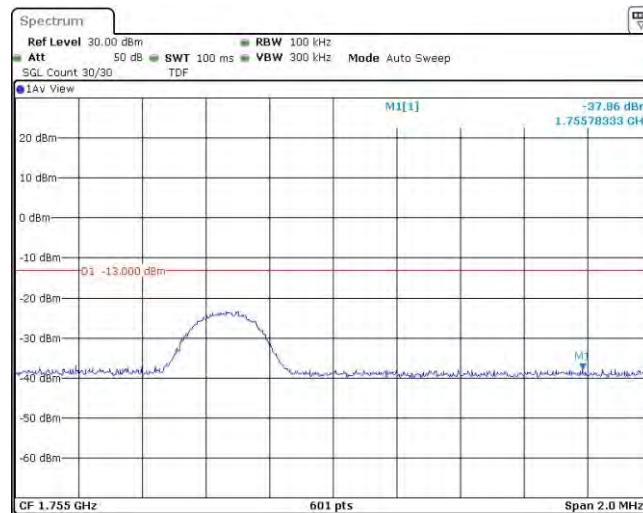
Band4-5MHz-16QAM-20375-1RB#24
