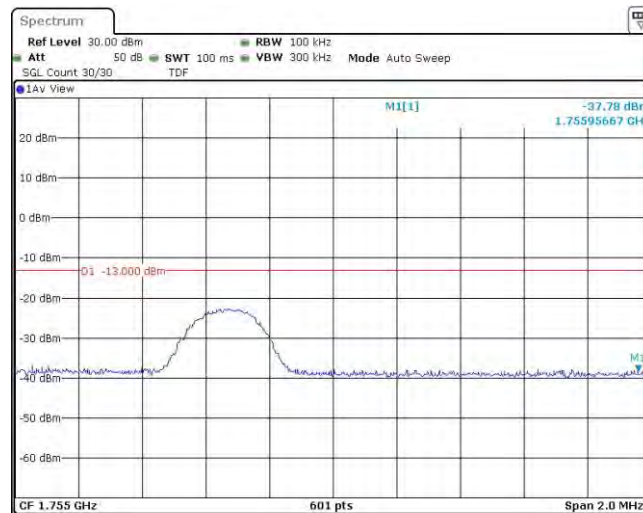
Band4-5MHz-QPSK-20375-1RB#24
