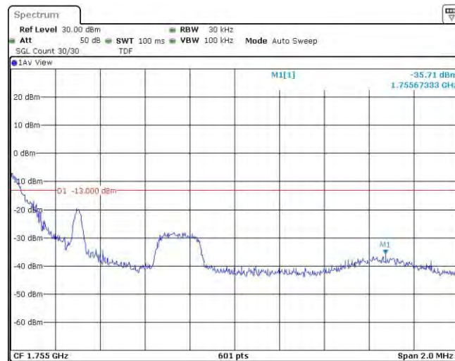
Band4-1.4MHz-16QAM-20393-1RB#5
