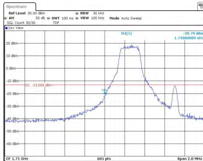
Band4-1.4MHz-16QAM-19957-1RB#5
