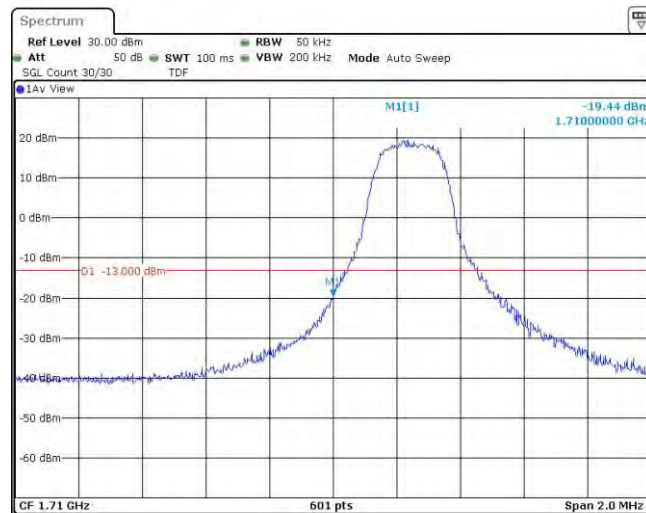
Band4-3MHz-16QAM-19965-1RB#14
