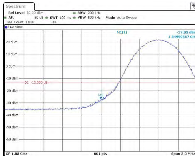
Band2-10MHz-16QAM-18650-1RB#49
