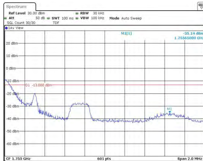
Band4-1.4MHz-QPSK-20393-1RB#5
