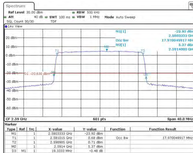
Band41-20MHz-16QAM-40620-100RB#0
