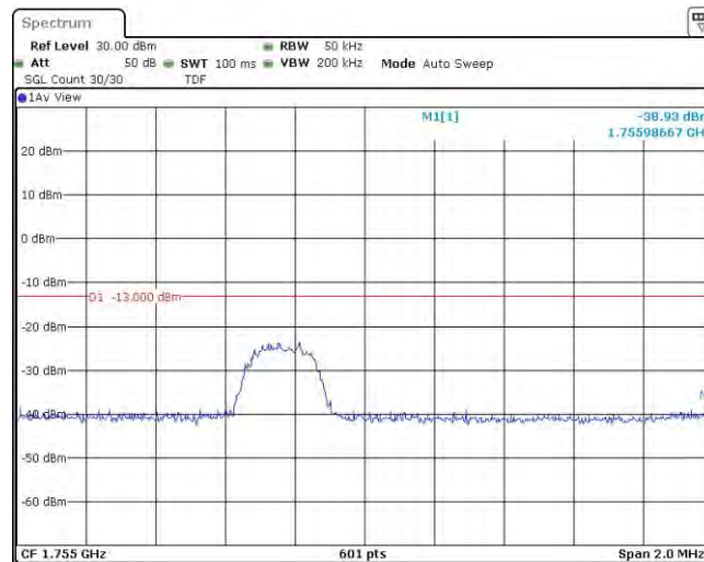
Band4-3MHz-16QAM-20385-1RB#14
