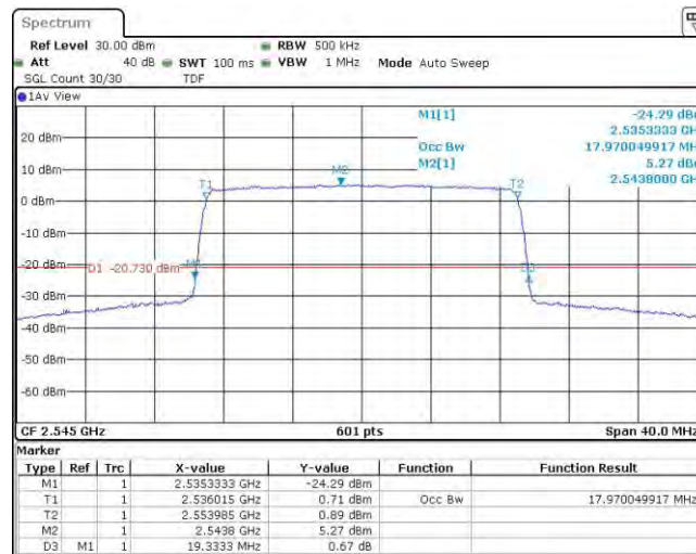
Band41-20MHz-16QAM-40340-100RB#0
