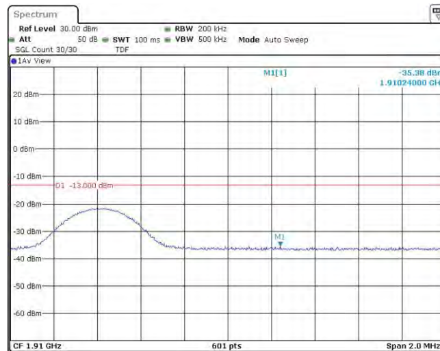
Band2-10MHz-QPSK-19150-1RB#49
