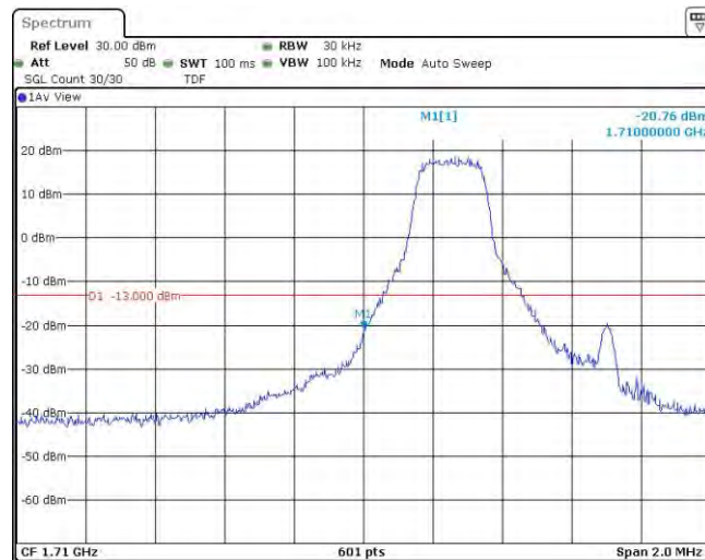
Band4-1.4MHz-QPSK-19957-1RB#5
