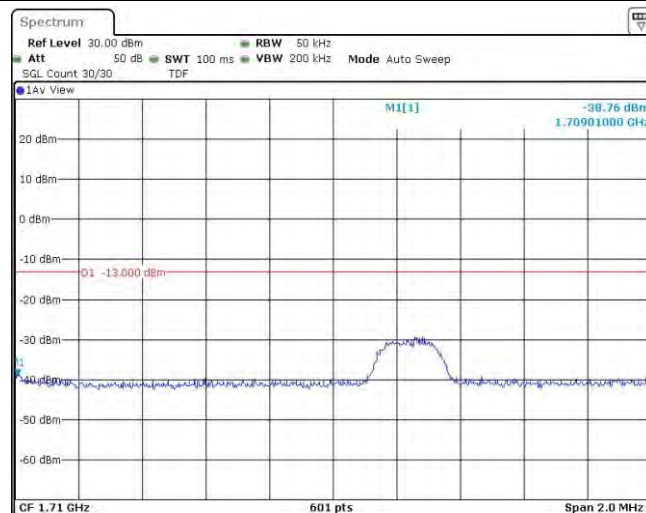
Band4-3MHz-16QAM-19965-15RB#0
