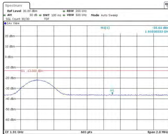
Band2-10MHz-16QAM-19150-1RB#49
