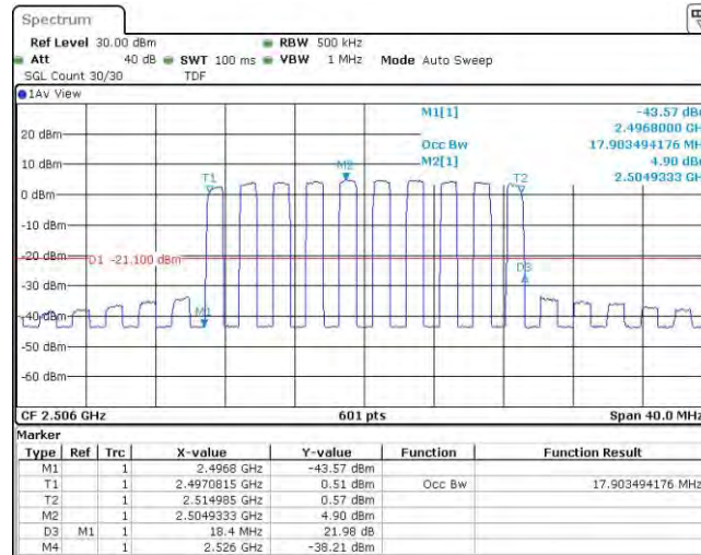
Band41-20MHz-16QAM-40140-100RB#0
