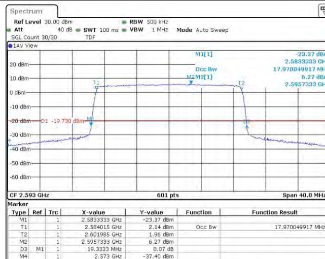
Band41-20MHz-QPSK-40620-100RB#0
