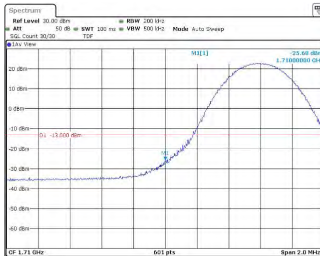
Band4-10MHz-QPSK-20000-1RB#49
