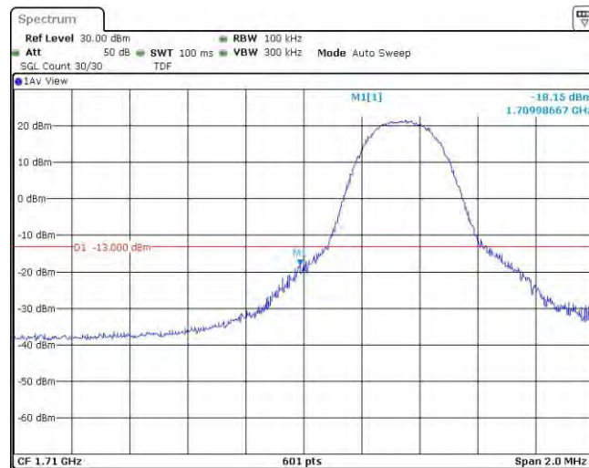
Band4-5MHz-QPSK-19975-1RB#24
