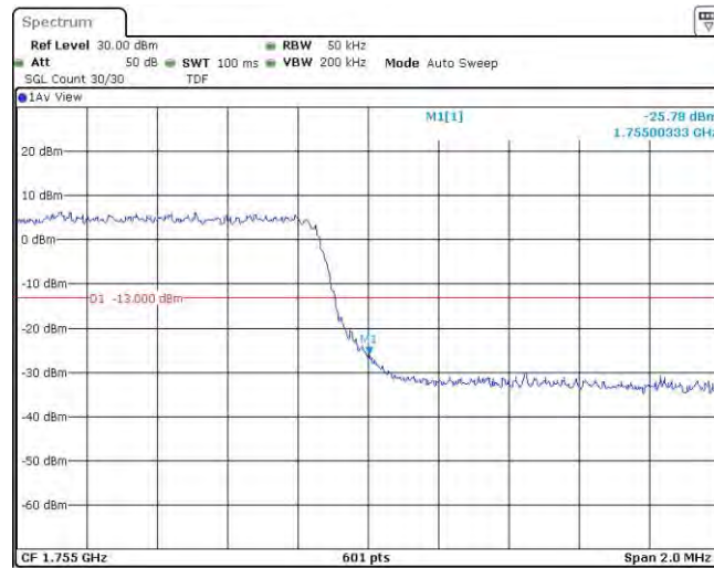
Band4-5MHz-QPSK-19975-1RB#0
