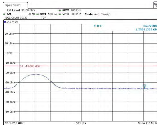
Band4-10MHz-QPSK-20350-1RB#49
