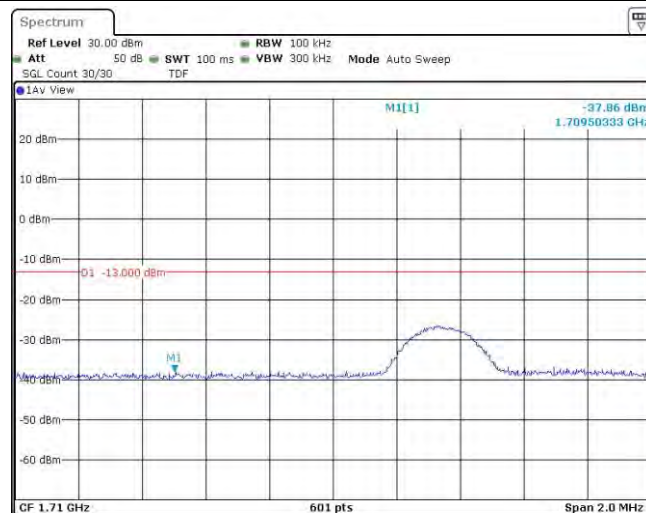
Band4-5MHz-QPSK-19975-25RB#0
