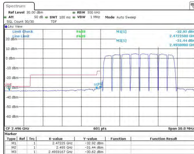
Band41-20MHz-16QAM-40140-1RB#0
