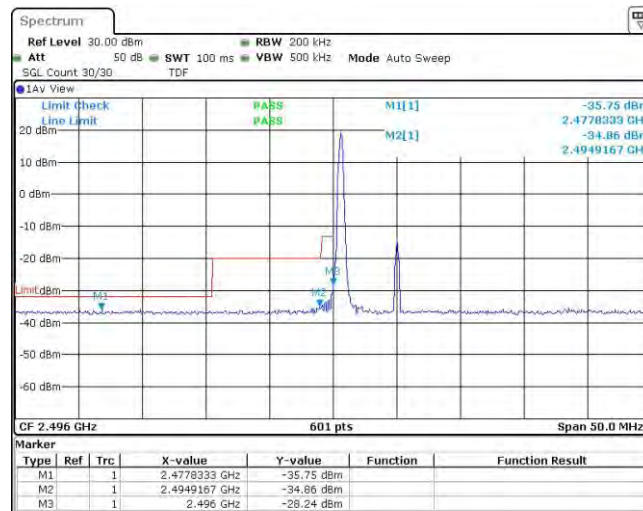
Band41-10MHz-16QAM-39700-1RB#49
