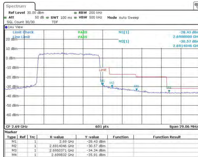
Band41-10MHz-16QAM-39700-1RB#0
