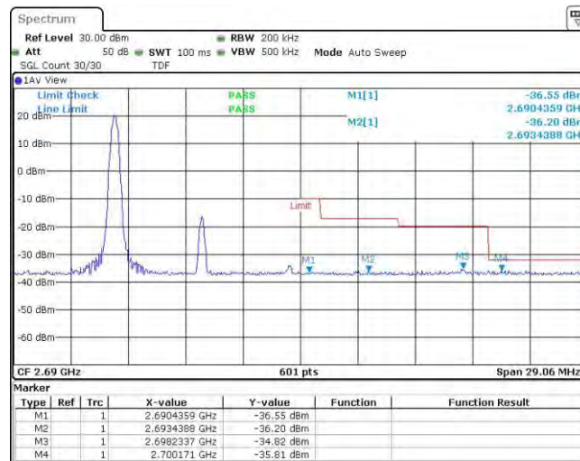
Band41-10MHz-16QAM-41540-1RB#49
