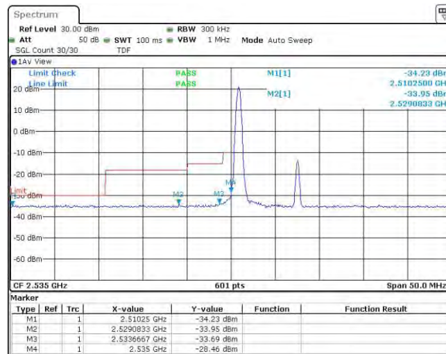
Band41-15MHz-QPSK-40115-1RB#74
