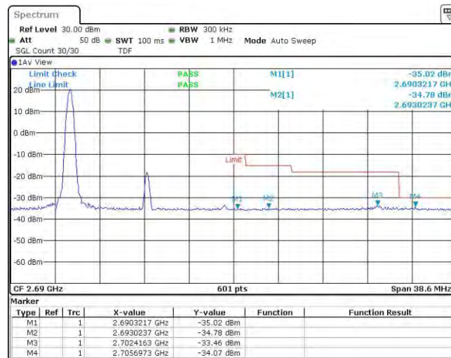
Band41-15MHz-16QAM-41515-1RB#74
