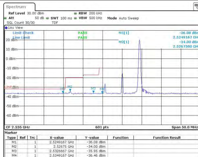
Band41-10MHz-16QAM-40090-50RB#0
