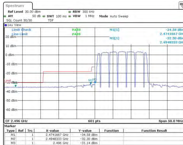
Band41-15MHz-16QAM-40115-1RB#0
