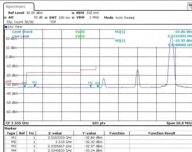
Band41-20MHz-16QAM-40140-100RB#0
