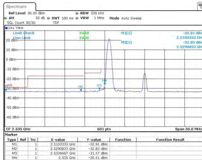
Band41-20MHz-16QAM-40140-1RB#99
