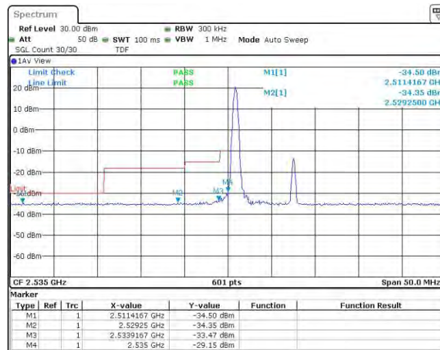
Band41-15MHz-16QAM-40115-1RB#74
