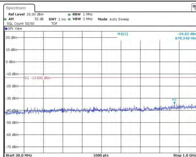
Band2-1.4MHz-QPSK-18607-1RB#0-Range1:30~1000MHz
