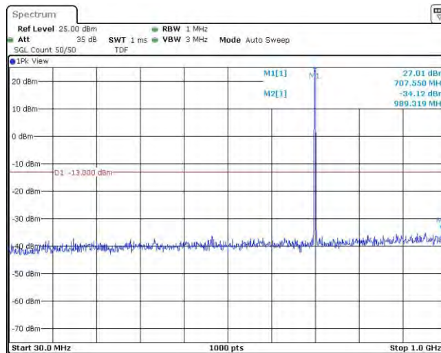
Band12-1.4MHz-QPSK-23095-1RB#0-Range2:1000~10000MHz
