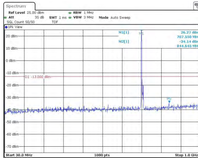
Band12-10MHz-QPSK-23130-1RB#0-Range2:1000~10000MHz
