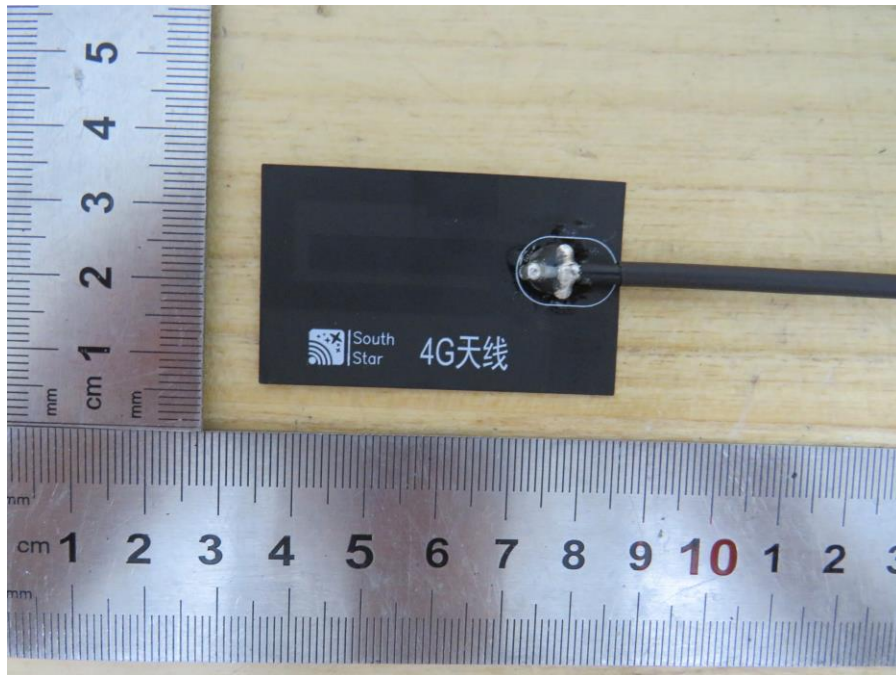
Detail View of Antenna(030383F4GA)
