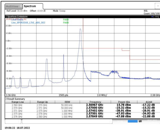
Band7-10MHz-QPSK-20800-1RB#0
