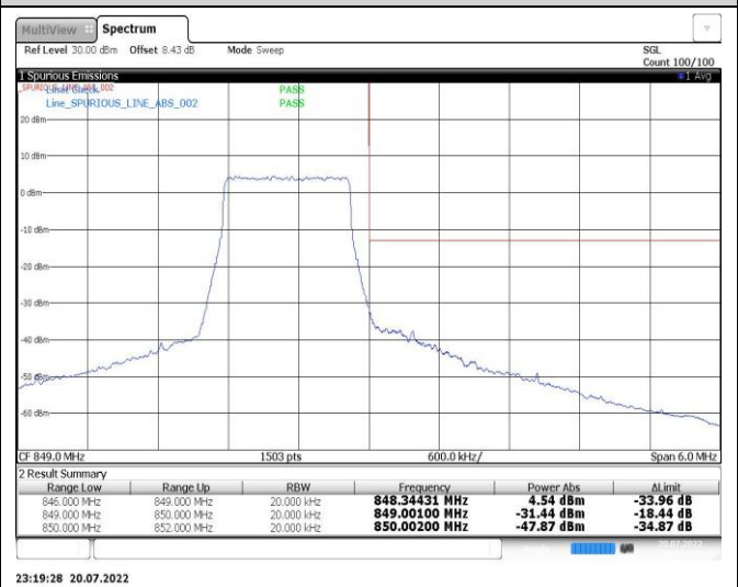
Band5-3MHz-QPSK-20415-15RB#0
