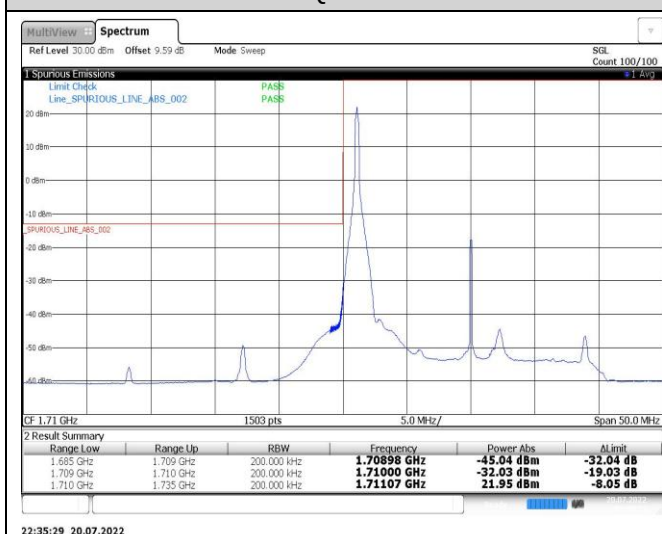
Band4-20MHz-16QAM-20050-1RB#0
