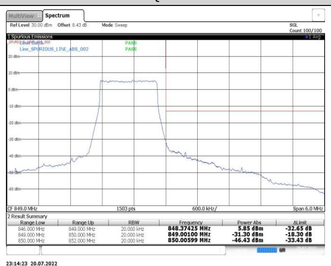
Band5-1.4MHz-16QAM-20407-6RB#0
