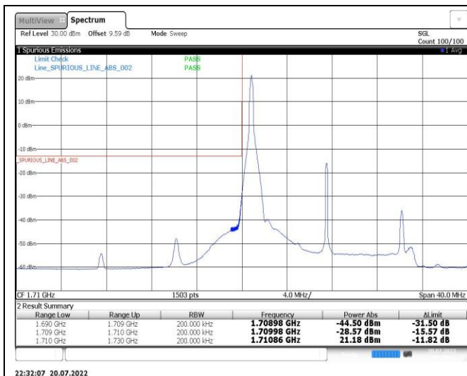
Band4-15MHz-16QAM-20325-1RB#74
