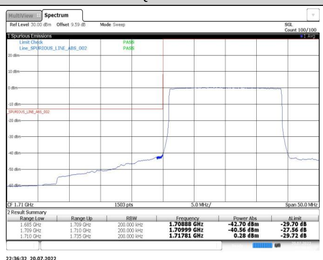
Band4-20MHz-16QAM-20050-100RB#0
