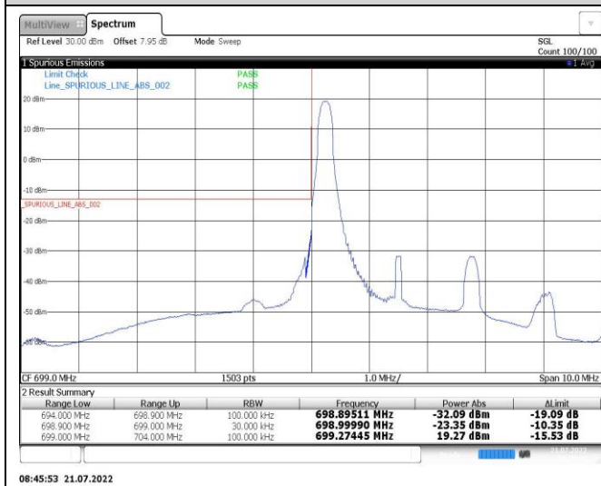
Band12-3MHz-16QAM-23165-1RB#14
