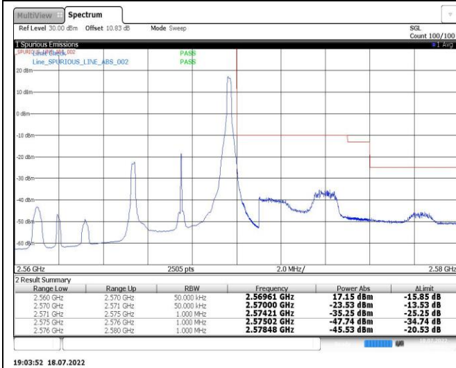
Band7-5MHz-16QAM-20775-1RB#0
