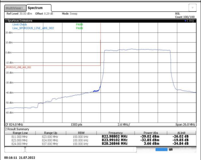
Band5-10MHz-16QAM-20450-50RB#0
