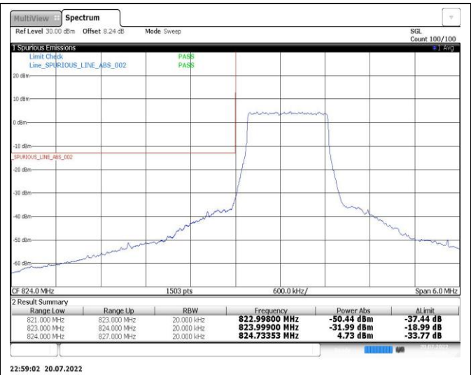
Band5-1.4MHz-16QAM-20643-6RB#0
