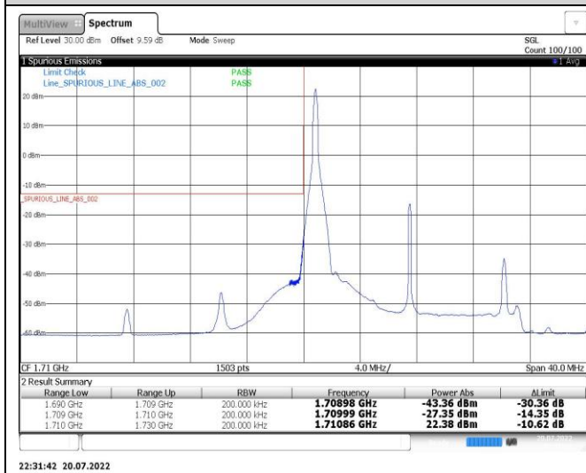
Band4-15MHz-QPSK-20325-1RB#74
