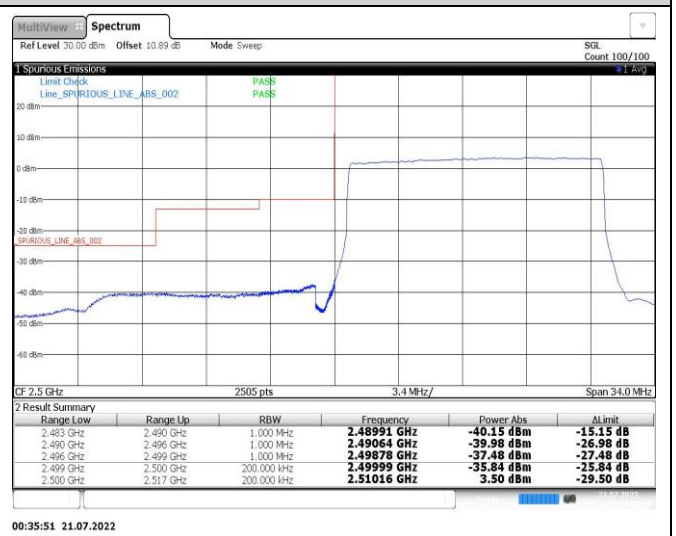
Band7-15MHz-QPSK-21375-75RB#0
