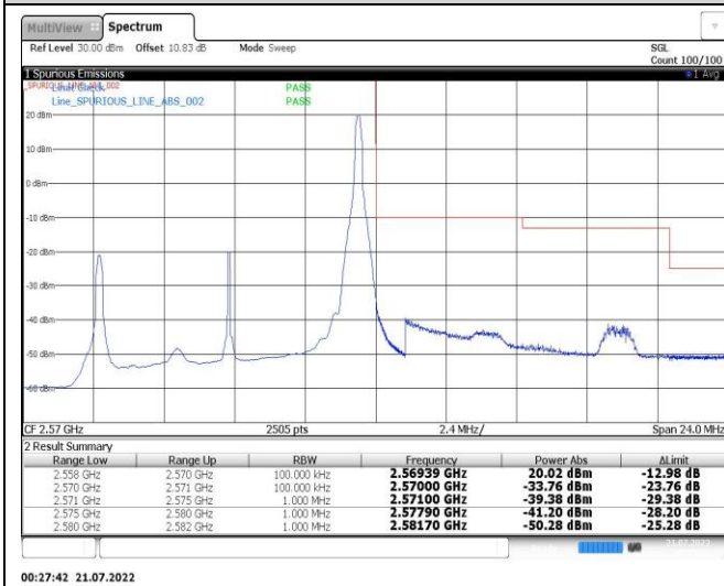
Band7-10MHz-16QAM-20800-1RB#0
