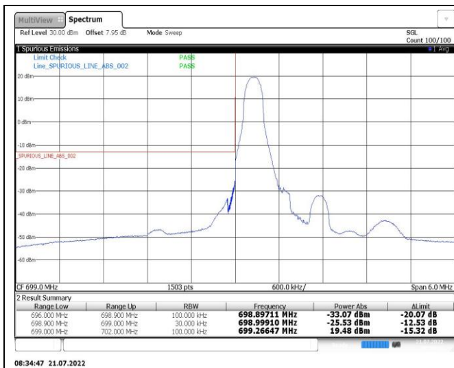
Band12-1.4MHz-16QAM-23173-1RB#5
