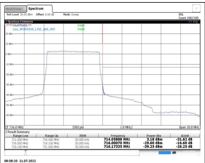
Band12-3MHz-16QAM-23025-15RB#0
