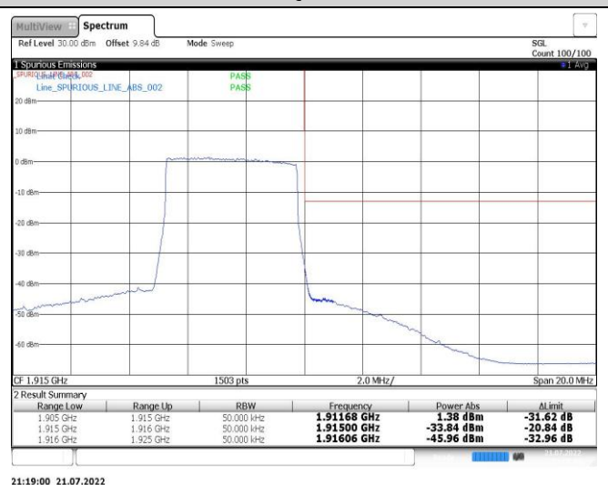
Band25-10MHz-QPSK-26090-50RB#0
