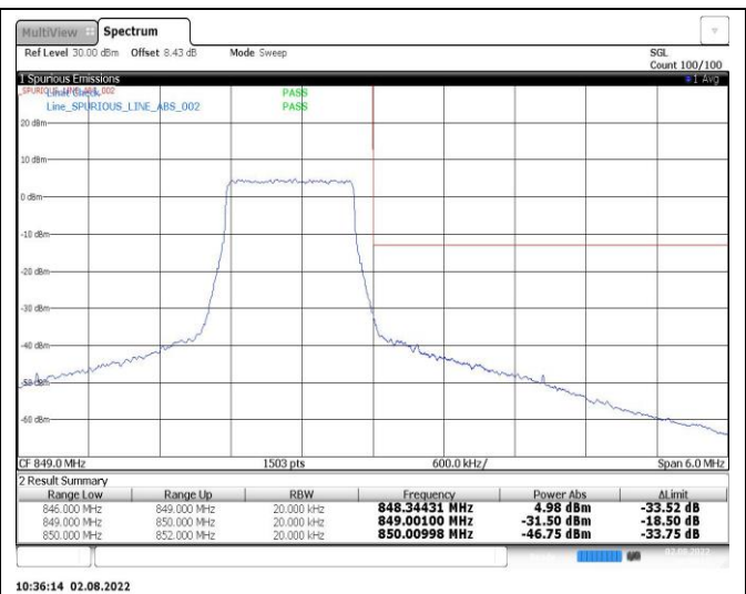
Band26-3MHz-QPSK-26705-15RB#0
