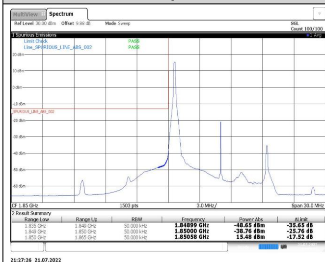
Band25-10MHz-16QAM-26640-1RB#49
