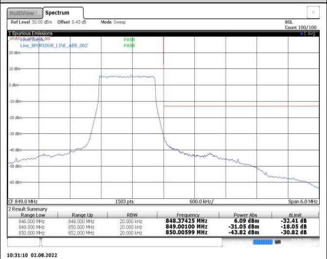
Band26-1.4MHz-16QAM-26697-6RB#0
