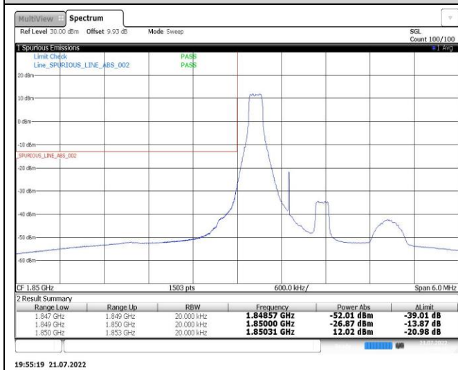
Band25-1.4MHz-16QAM-26683-1RB#5
