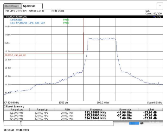
Band26-1.4MHz-QPSK-27033-6RB#0
