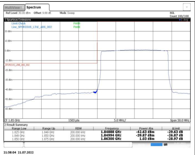
Band25-20MHz-16QAM-26590-100RB#0
