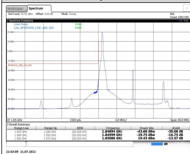
Band25-15MHz-16QAM-26615-1RB#74
