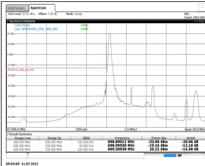
Band12-5MHz-16QAM-23035-1RB#0
