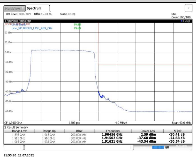
Band25-15MHz-16QAM-26115-75RB#0
