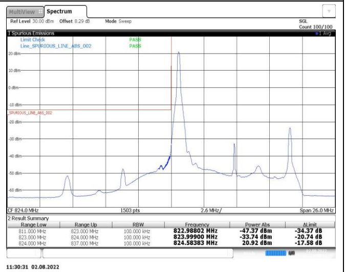
Band26-10MHz-16QAM-26740-1RB#0
