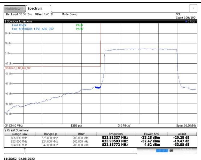
Band26-15MHz-16QAM-26865-75RB#0
