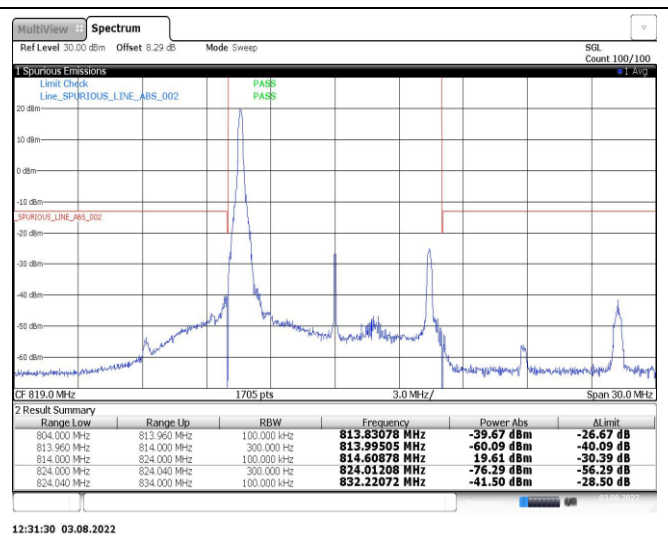
Band26-10MHz-16QAM-26740-50RB#0
