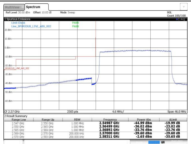
Band38-20MHz-16QAM-37850-100RB#0
