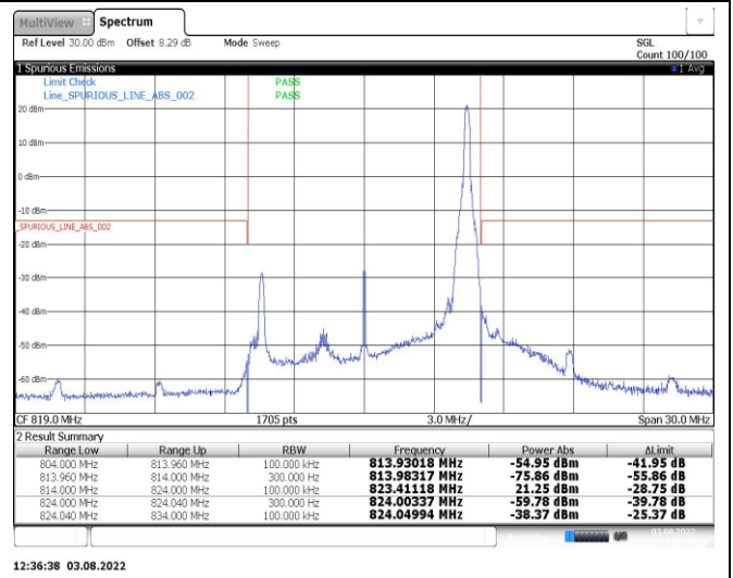
Band26-10MHz-QPSK-26840-1RB#0
