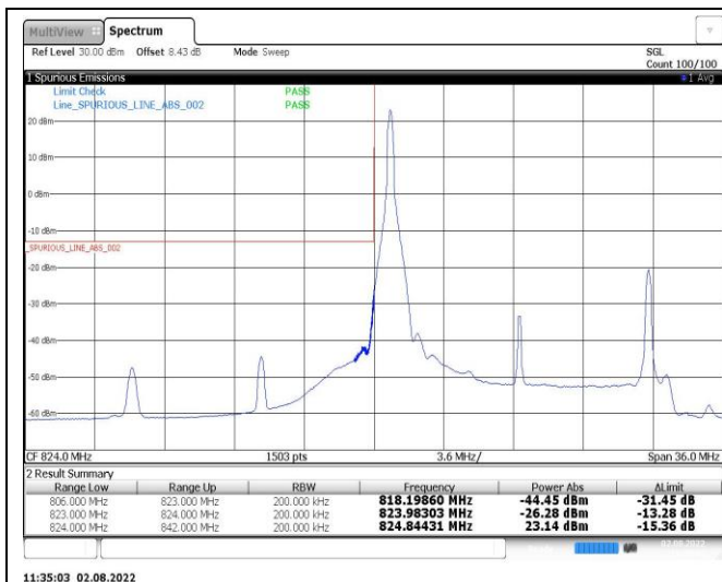
Band26-15MHz-16QAM-26865-1RB#0
