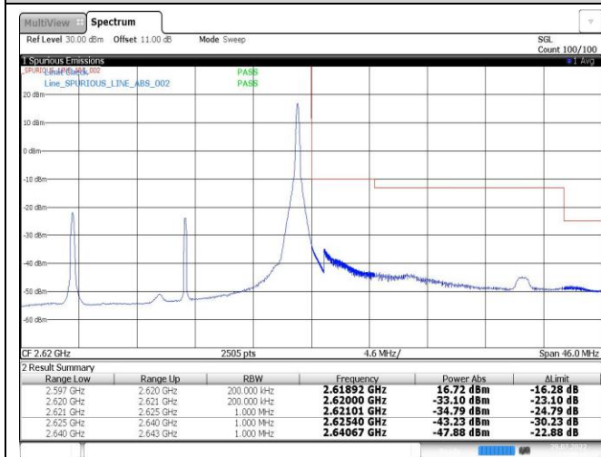
Band38-20MHz-16QAM-38150-1RB#99
