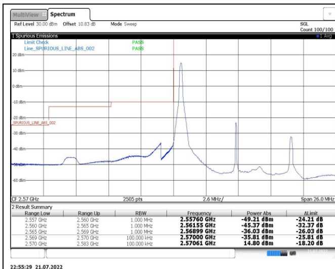
Band38-10MHz-QPSK-38200-1RB#49
