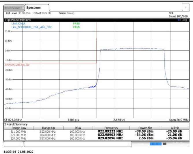
Band26-15MHz-QPSK-26865-75RB#0
