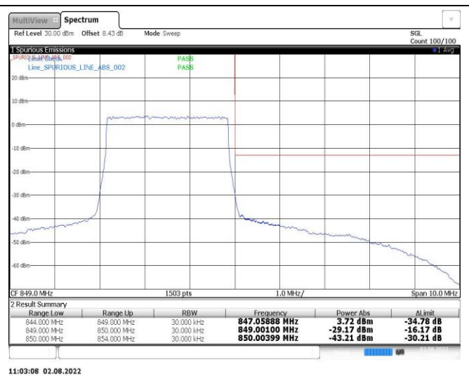
Band26-3MHz-16QAM-26705-15RB#0
