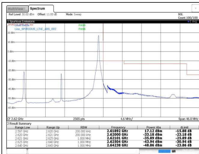
Band38-20MHz-16QAM-37850-1RB#0
