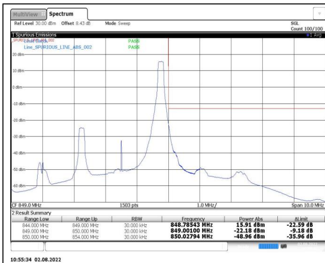
Band26-3MHz-16QAM-26705-1RB#0
