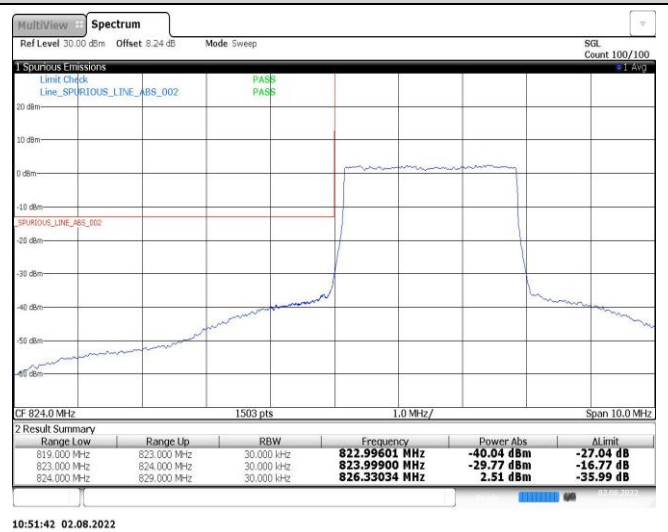
Band26-3MHz-16QAM-27025-15RB#0
