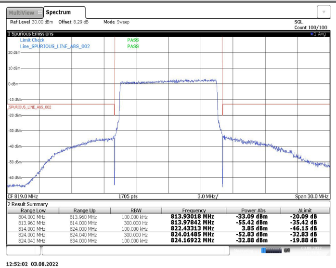
Band26-10MHz-16QAM-26840-50RB#0
