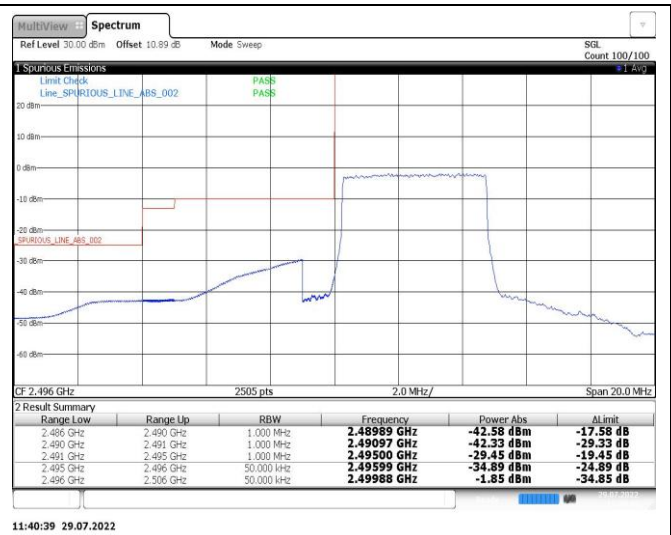
Band41-5MHz-QPSK-41565-25RB#0
