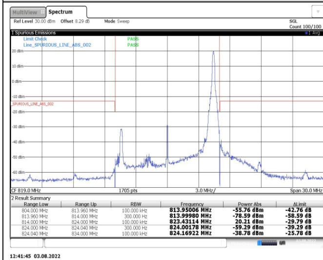
Band26-10MHz-16QAM-26840-1RB#0
