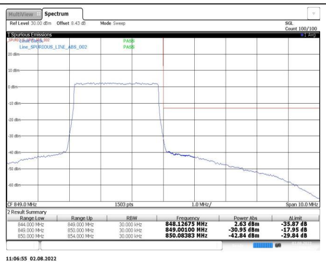
Band26-5MHz-QPSK-26715-25RB#0
