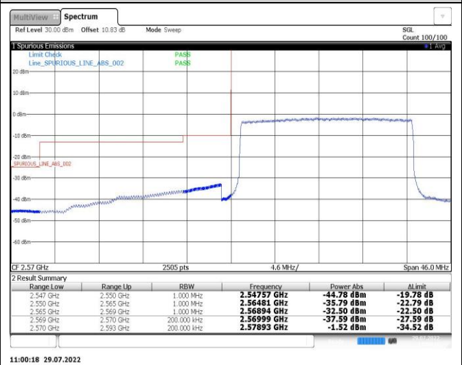
Band38-20MHz-QPSK-38150-100RB#0
