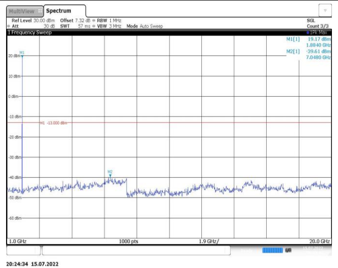
Band2-1.4MHz-16QAM-19193-1RB#0-Range2:1000~20000MHz
