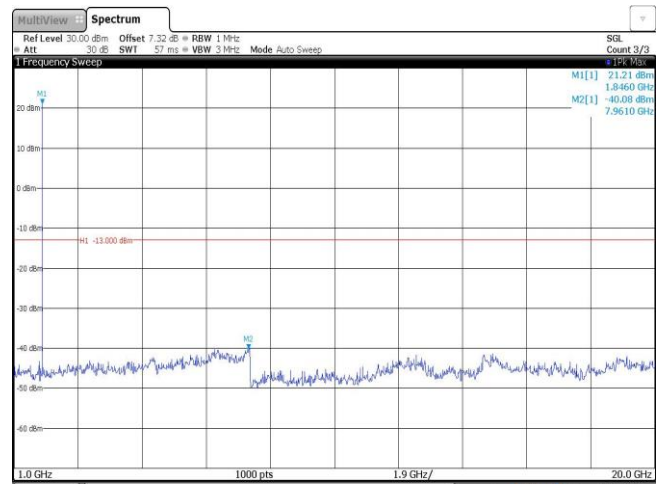
Band2-1.4MHz-QPSK-18607-1RB#0-Range2:1000~20000MHz
