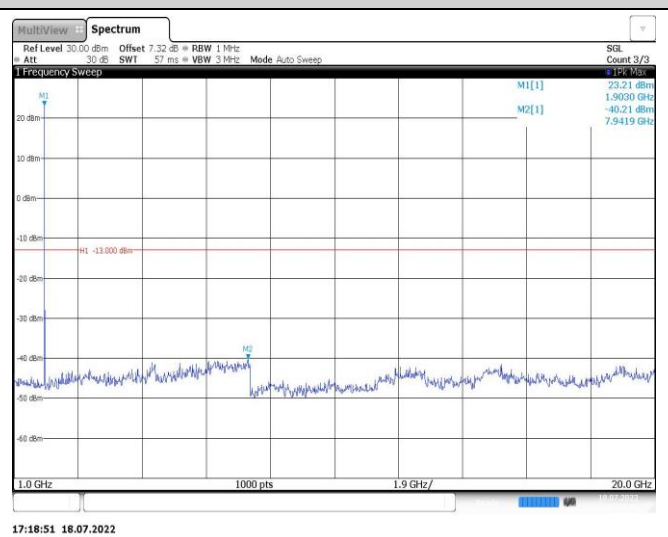
Band2-5MHz-16QAM-18625-1RB#0-Range2:1000~20000MHz
