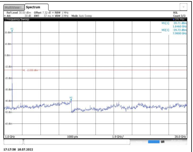
Band2-5MHz-16QAM-18900-1RB#0-Range2:1000~20000MHz
