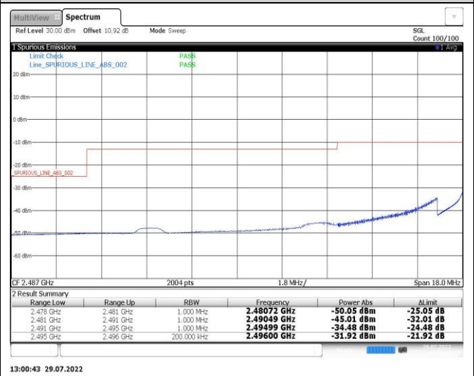
Band41-20MHz-QPSK-39750-100RB#0
