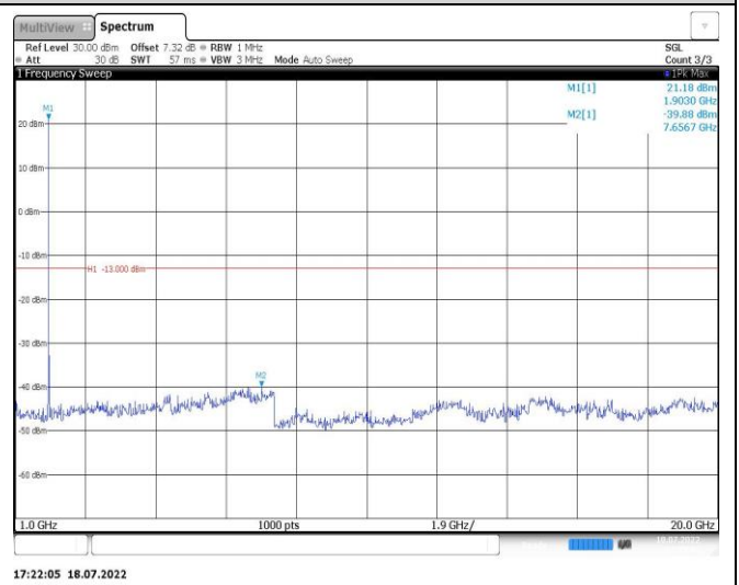
Band2-10MHz-16QAM-18650-1RB#0-Range2:1000~20000MHz
