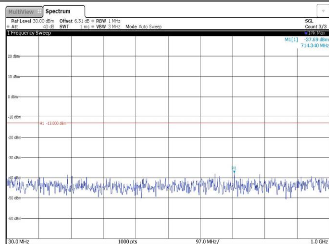
Band2-1.4MHz-QPSK-18900-1RB#0-Range1:30~1000MHz
