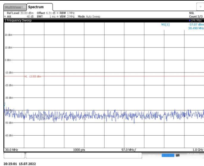
Band2-3MHz-QPSK-18615-1RB#0-Range1:30~1000MHz
