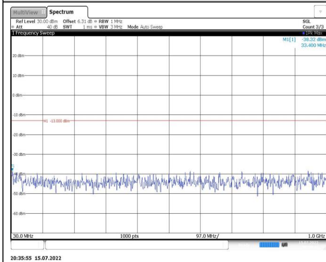
Band2-3MHz-QPSK-19185-1RB#0-Range1:30~1000MHz
