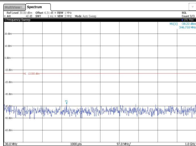
Band2-1.4MHz-QPSK-19193-1RB#0-Range1:30~1000MHz
