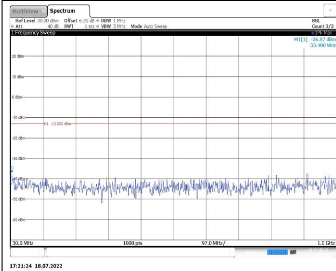
Band2-10MHz-QPSK-19150-1RB#0-Range1:30~1000MHz
