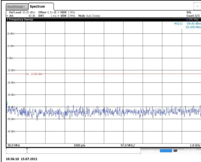
Band2-3MHz-16QAM-19185-1RB#0-Range1:30~1000MHz
