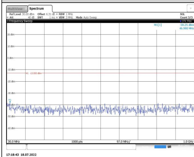
Band2-5MHz-16QAM-18625-1RB#0-Range1:30~1000MHz
