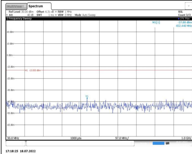
Band2-5MHz-16QAM-19175-1RB#0-Range1:30~1000MHz
