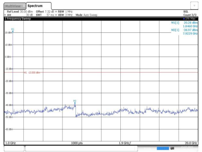
Band2-1.4MHz-16QAM-18607-1RB#0-Range2:1000~20000MHz
