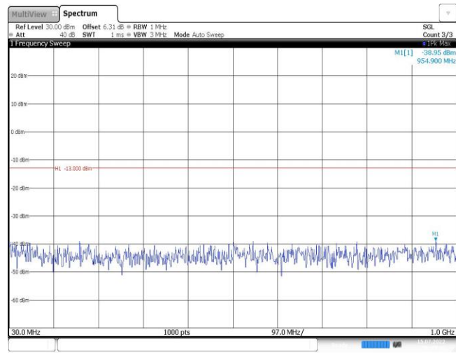
Band2-1.4MHz-16QAM-18607-1RB#0-Range1:30~1000MHz
