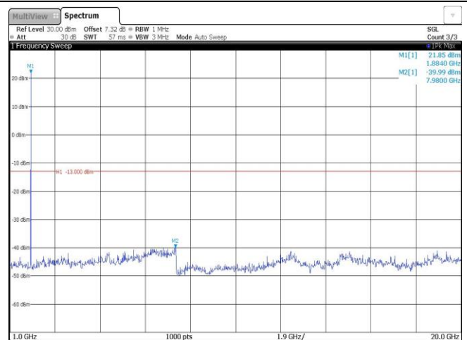
Band2-1.4MHz-QPSK-18900-1RB#0-Range2:1000~20000MHz
