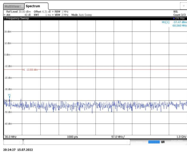
Band2-1.4MHz-16QAM-19193-1RB#0-Range1:30~1000MHz
