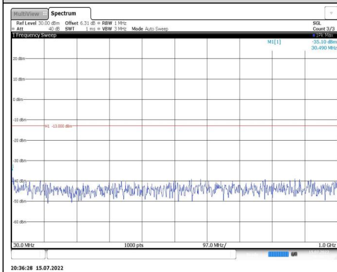
Band2-3MHz-16QAM-18615-1RB#0-Range1:30~1000MHz
