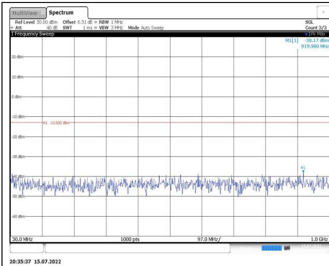
Band2-3MHz-16QAM-18900-1RB#0-Range1:30~1000MHz
