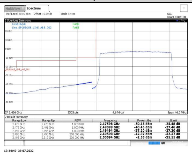
Band41-20MHz-16QAM-41490-100RB#0
