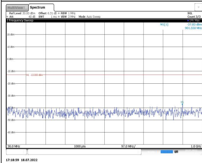
Band2-10MHz-QPSK-18650-1RB#0-Range1:30~1000MHz
