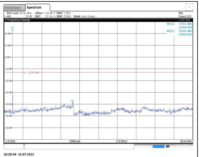
Band2-3MHz-16QAM-18900-1RB#0-Range2:1000~20000MHz
