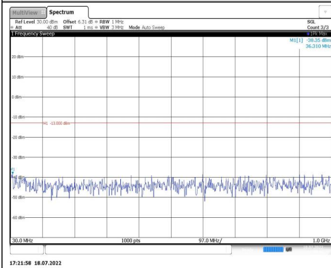
Band2-10MHz-16QAM-18650-1RB#0-Range1:30~1000MHz
