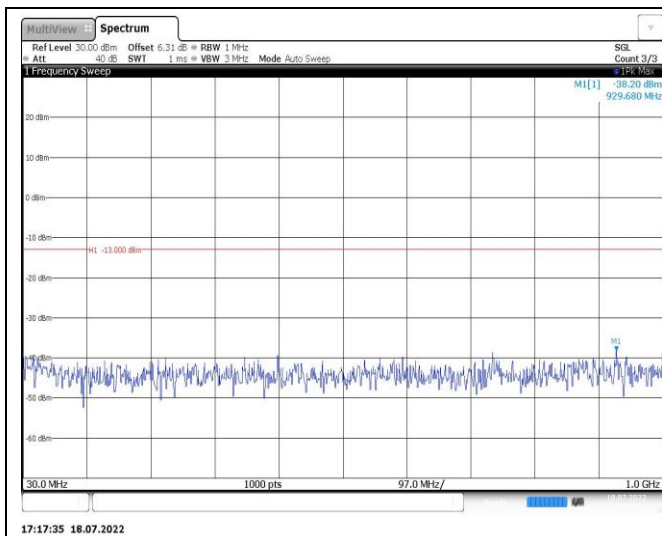
Band2-5MHz-QPSK-18900-1RB#0-Range1:30~1000MHz
