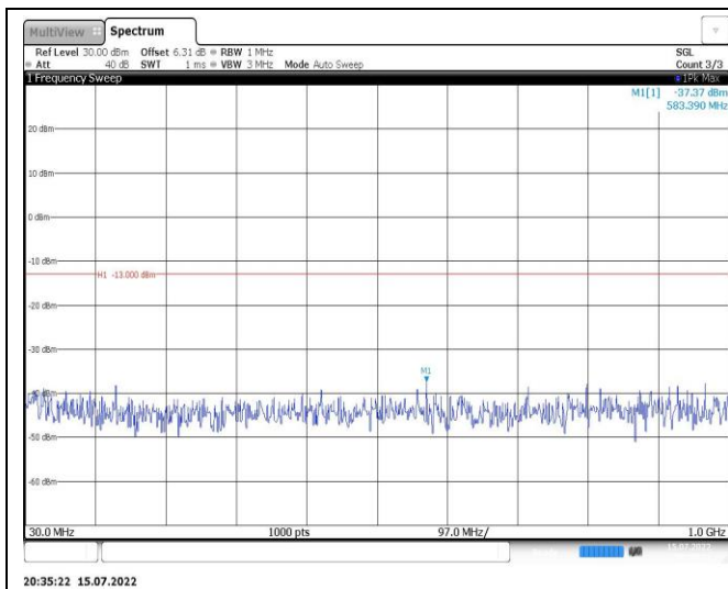
Band2-3MHz-QPSK-18900-1RB#0-Range1:30~1000MHz
