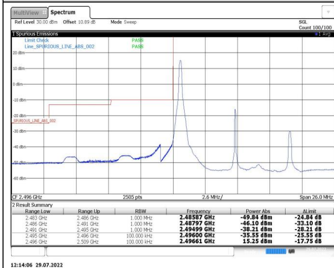
Band41-10MHz-QPSK-41540-1RB#49
