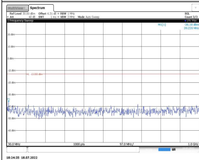
Band4-5MHz-QPSK-19975-1RB#0-Range1:30~1000MHz
