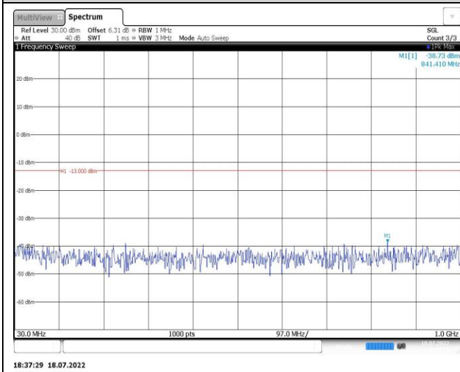
Band5-1.4MHz-QPSK-20407-1RB#0-Range1:30~1000MHz
