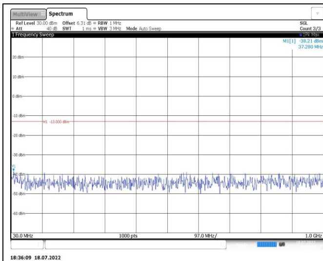
Band4-20MHz-QPSK-20175-1RB#0-Range1:30~1000MHz
