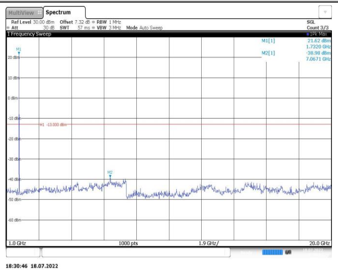
Band4-10MHz-16QAM-20350-1RB#0-Range2:1000~20000MHz
