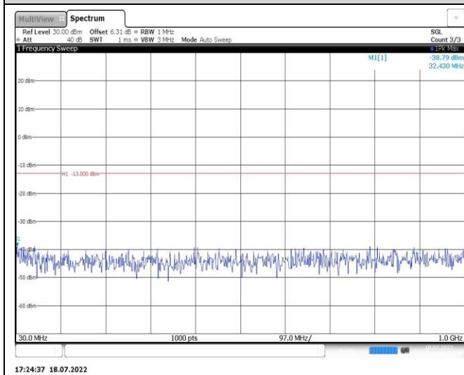
Band2-15MHz-QPSK-19125-1RB#0-Range1:30~1000MHz
