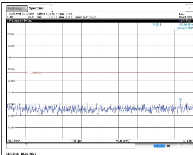
Band4-15MHz-16QAM-20175-1RB#0-Range1:30~1000MHz
