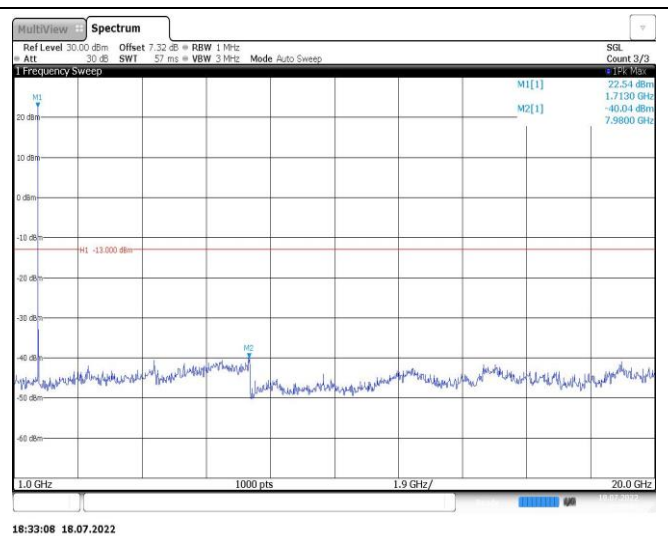
Band4-15MHz-QPSK-20175-1RB#0-Range2:1000~20000MHz
