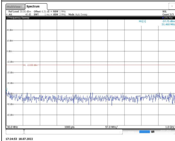
Band2-15MHz-16QAM-19125-1RB#0-Range1:30~1000MHz
