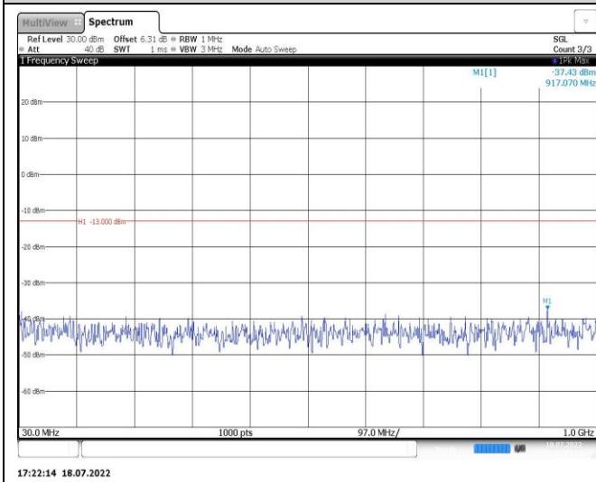
Band2-15MHz-QPSK-18675-1RB#0-Range1:30~1000MHz
