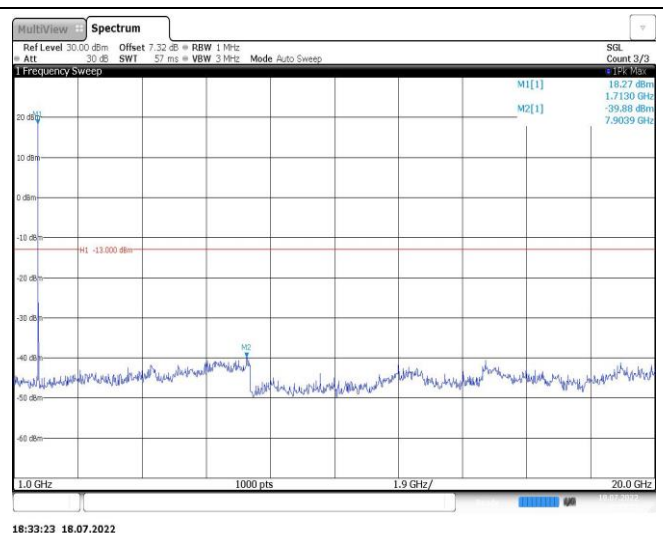
Band4-15MHz-16QAM-20175-1RB#0-Range2:1000~20000MHz
