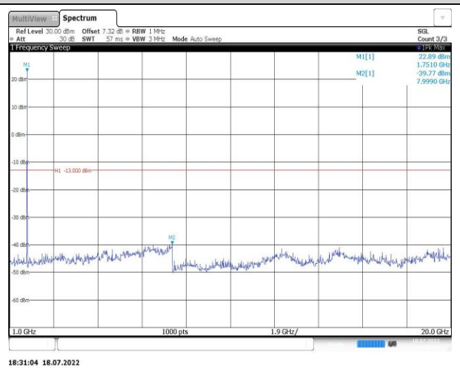
Band4-10MHz-16QAM-20000-1RB#0-Range2:1000~20000MHz
