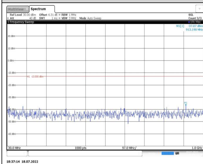
Band4-20MHz-16QAM-20050-1RB#0-Range1:30~1000MHz
