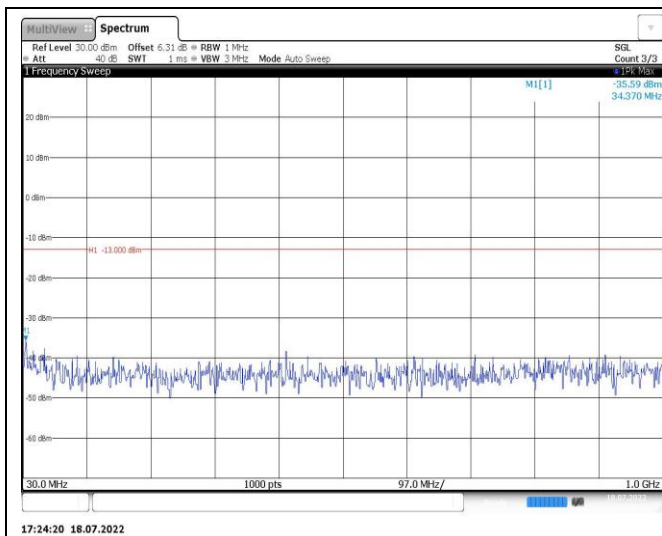
Band2-15MHz-16QAM-18900-1RB#0-Range1:30~1000MHz
