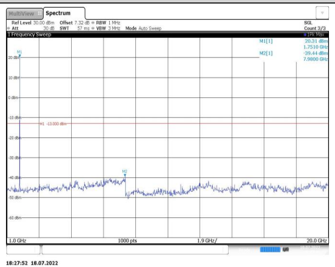
Band4-5MHz-16QAM-19975-1RB#0-Range2:1000~20000MHz
