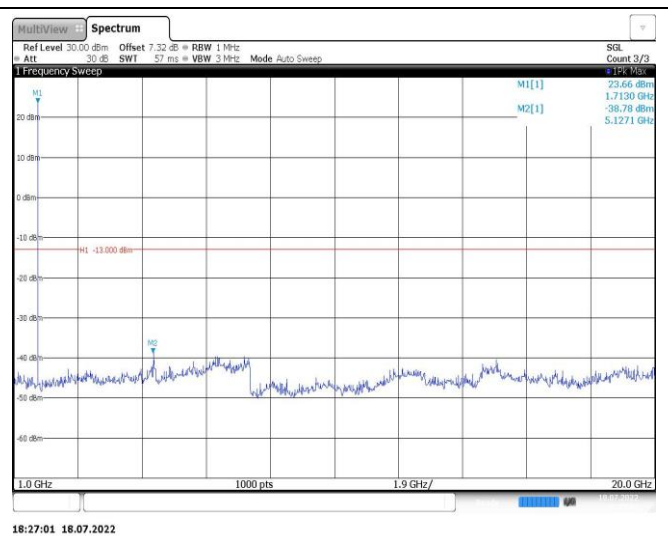
Band4-5MHz-16QAM-20175-1RB#0-Range2:1000~20000MHz
