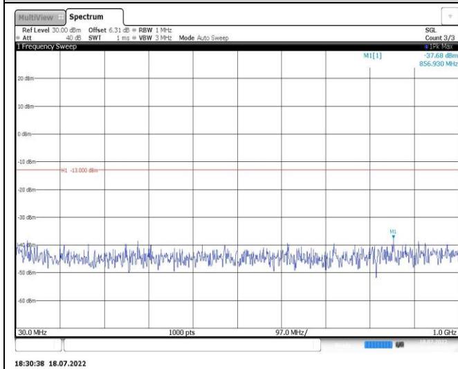
Band4-10MHz-16QAM-20350-1RB#0-Range1:30~1000MHz
