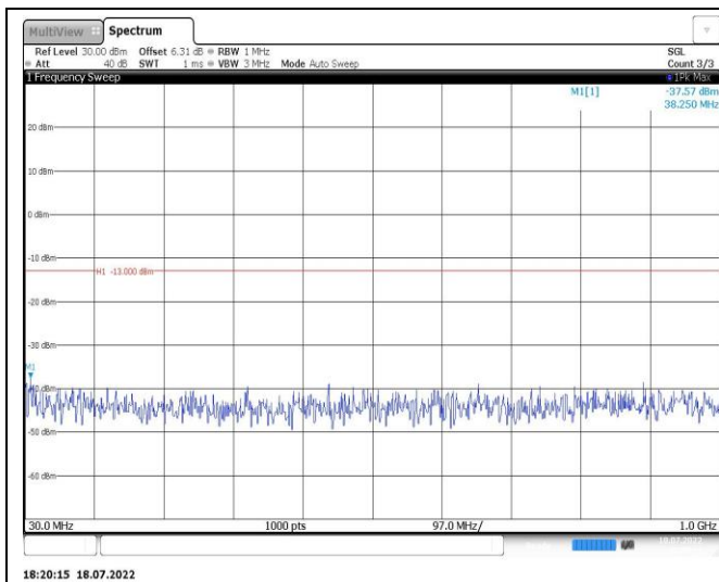
Band4-1.4MHz-16QAM-20175-1RB#0-Range1:30~1000MHz
