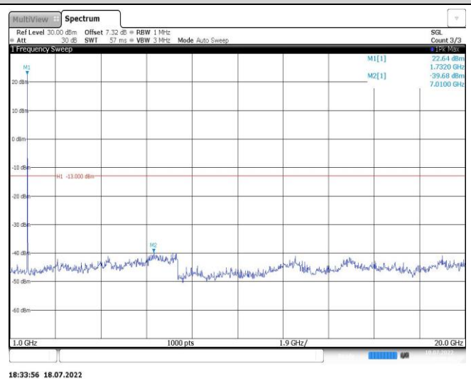
Band4-15MHz-16QAM-20325-1RB#0-Range2:1000~20000MHz
