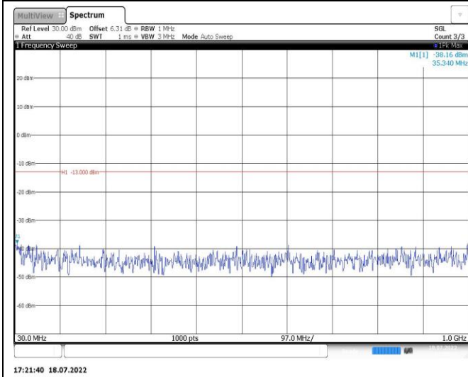
Band2-10MHz-16QAM-19150-1RB#0-Range1:30~1000MHz
