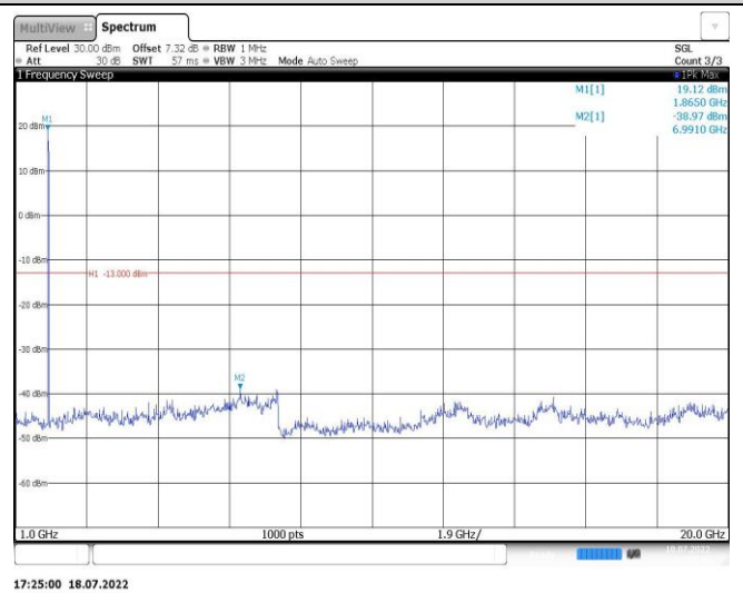
Band2-15MHz-16QAM-19125-1RB#0-Range2:1000~20000MHz
