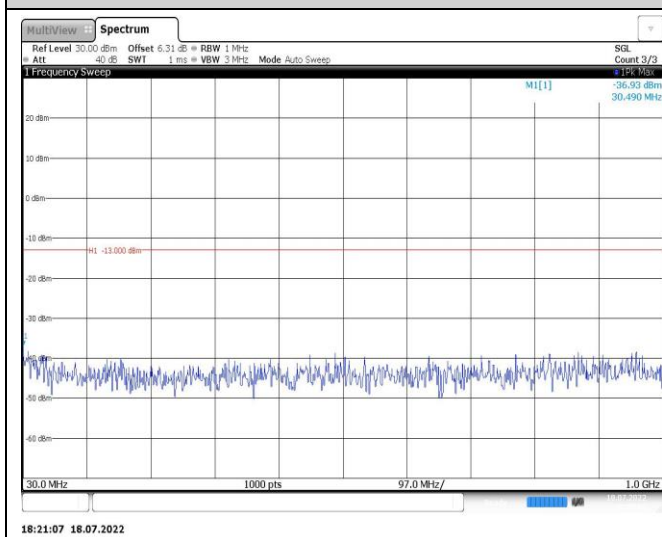
Band4-1.4MHz-16QAM-19957-1RB#0-Range1:30~1000MHz
