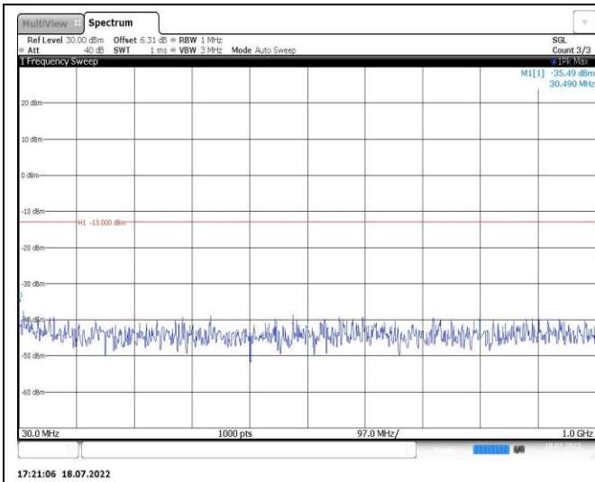
Band2-10MHz-16QAM-18900-1RB#0-Range1:30~1000MHz
