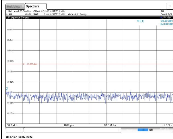
Band4-5MHz-16QAM-20375-1RB#0-Range1:30~1000MHz
