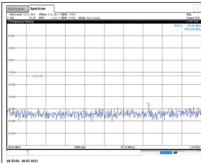
Band4-15MHz-QPSK-20175-1RB#0-Range1:30~1000MHz
