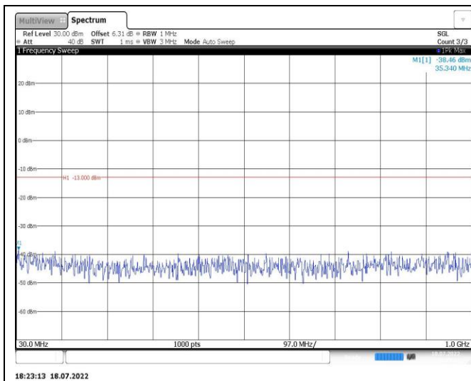
Band4-3MHz-QPSK-20175-1RB#0-Range1:30~1000MHz
