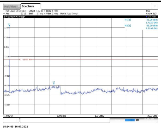
Band4-3MHz-16QAM-20385-1RB#0-Range2:1000~20000MHz
