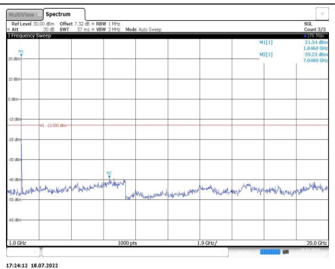
Band2-15MHz-QPSK-18900-1RB#0-Range2:1000~20000MHz
