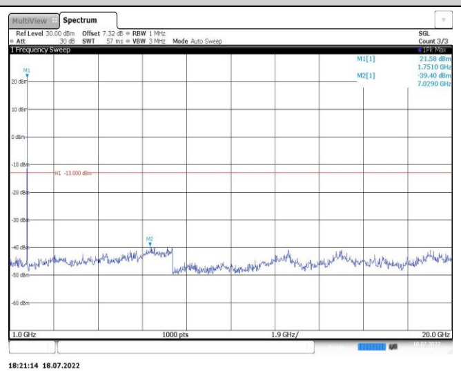
Band4-1.4MHz-16QAM-19957-1RB#0-Range2:1000~20000MHz
