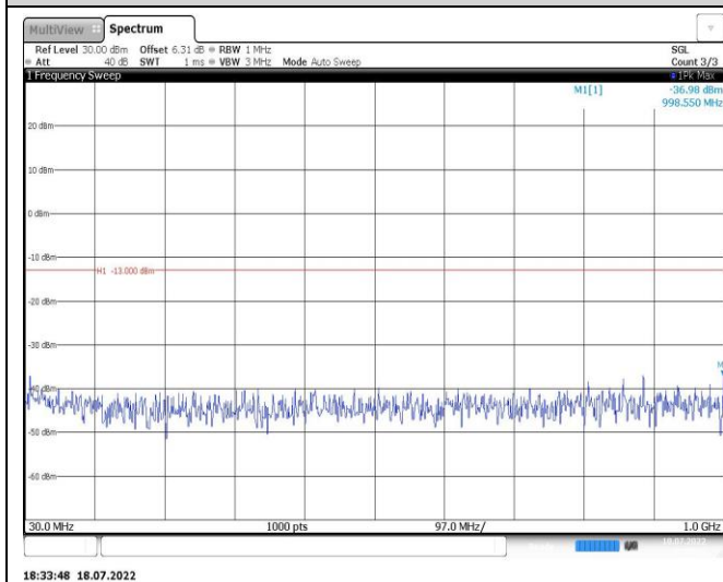
Band4-15MHz-16QAM-20325-1RB#0-Range1:30~1000MHz
