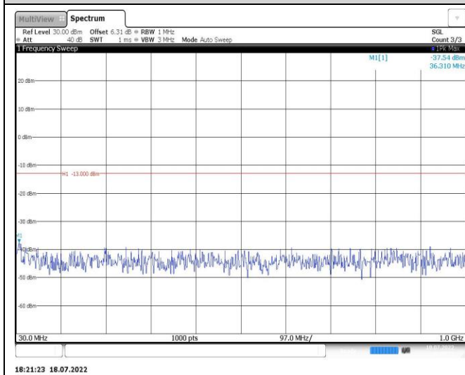
Band4-3MHz-QPSK-19965-1RB#0-Range1:30~1000MHz
