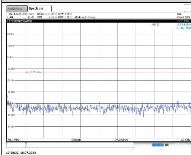
Band2-20MHz-16QAM-18700-1RB#0-Range1:30~1000MHz
