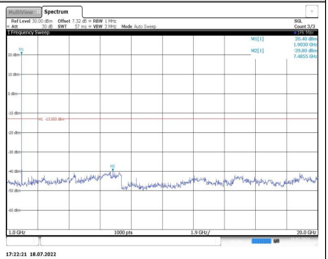
Band2-15MHz-QPSK-18675-1RB#0-Range2:1000~20000MHz
