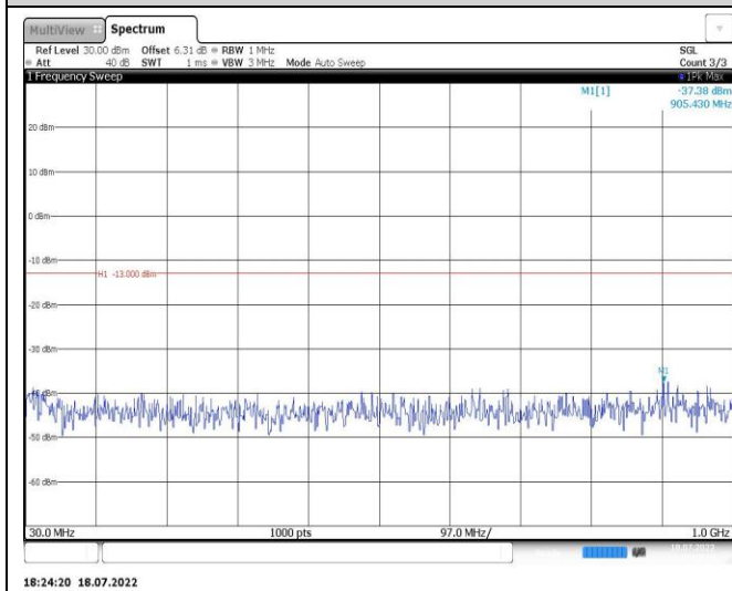
Band4-3MHz-16QAM-19965-1RB#0-Range1:30~1000MHz
