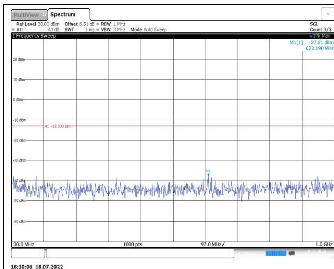
Band4-10MHz-16QAM-20175-1RB#0-Range1:30~1000MHz
