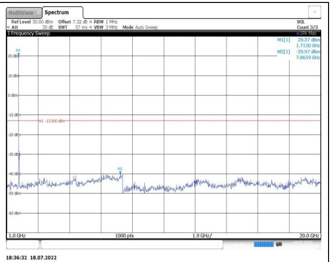
Band4-20MHz-16QAM-20175-1RB#0-Range2:1000~20000MHz
