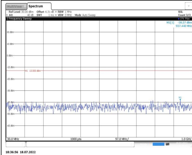
Band4-20MHz-16QAM-20300-1RB#0-Range1:30~1000MHz
