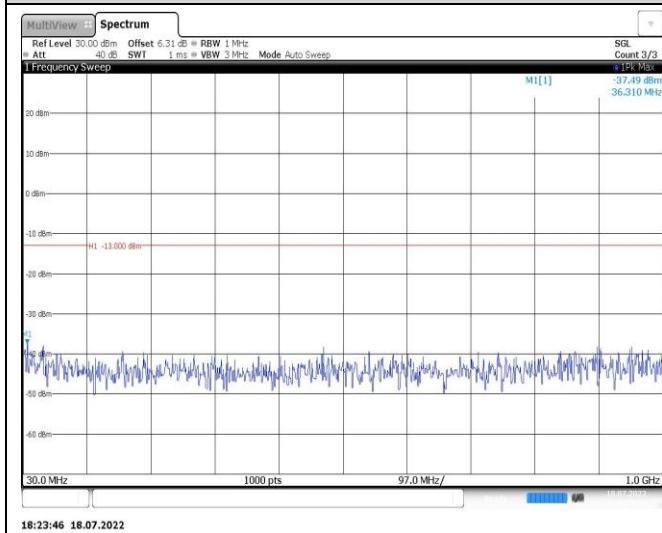
Band4-3MHz-QPSK-20385-1RB#0-Range1:30~1000MHz
