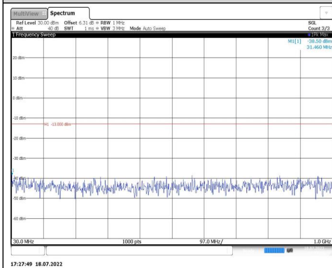
Band2-20MHz-QPSK-19100-1RB#0-Range1:30~1000MHz
