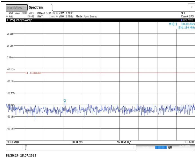
Band4-20MHz-16QAM-20175-1RB#0-Range1:30~1000MHz
