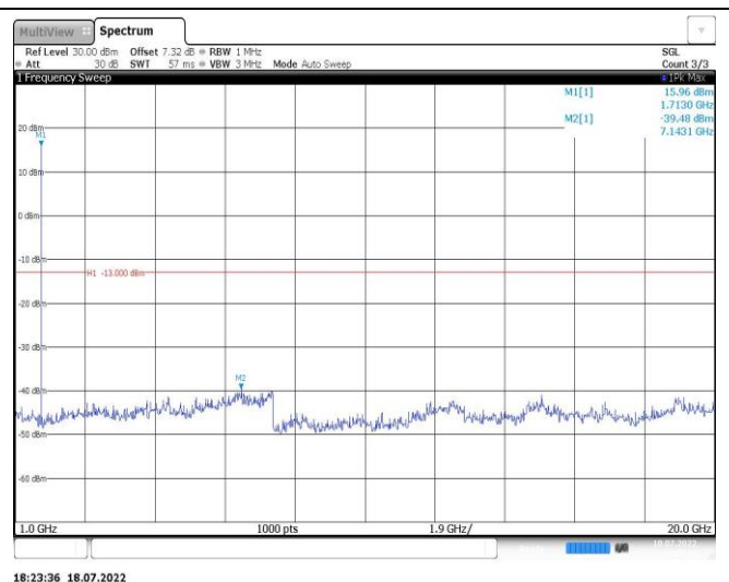
Band4-3MHz-16QAM-20175-1RB#0-Range2:1000~20000MHz
