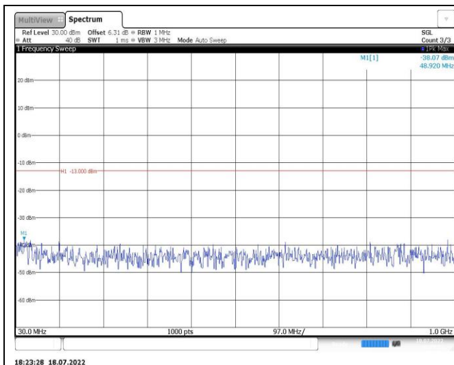
Band4-3MHz-16QAM-20175-1RB#0-Range1:30~1000MHz
