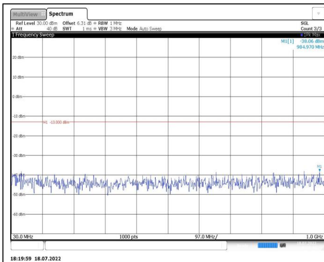
Band4-1.4MHz-QPSK-20175-1RB#0-Range1:30~1000MHz
