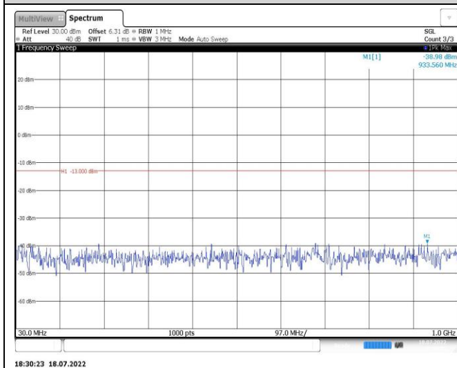
Band4-10MHz-QPSK-20350-1RB#0-Range1:30~1000MHz
