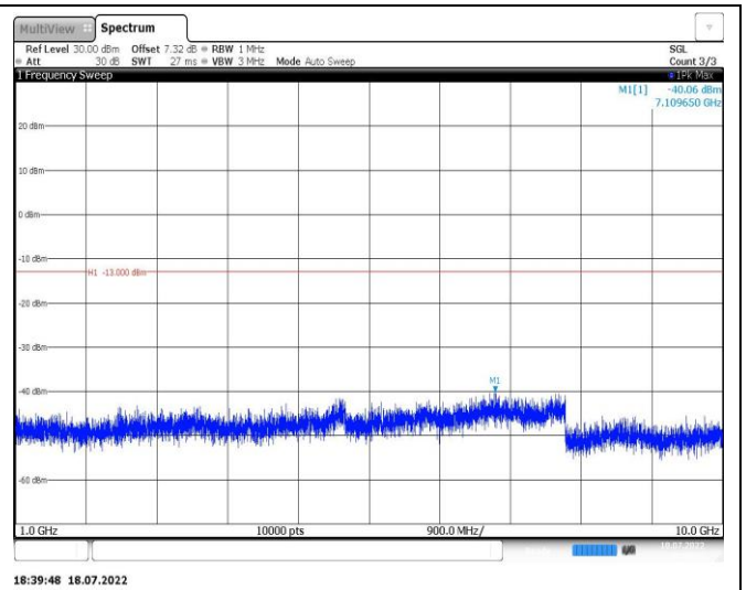
Band5-1.4MHz-QPSK-20525-1RB#0-Range2:1000~10000MHz
