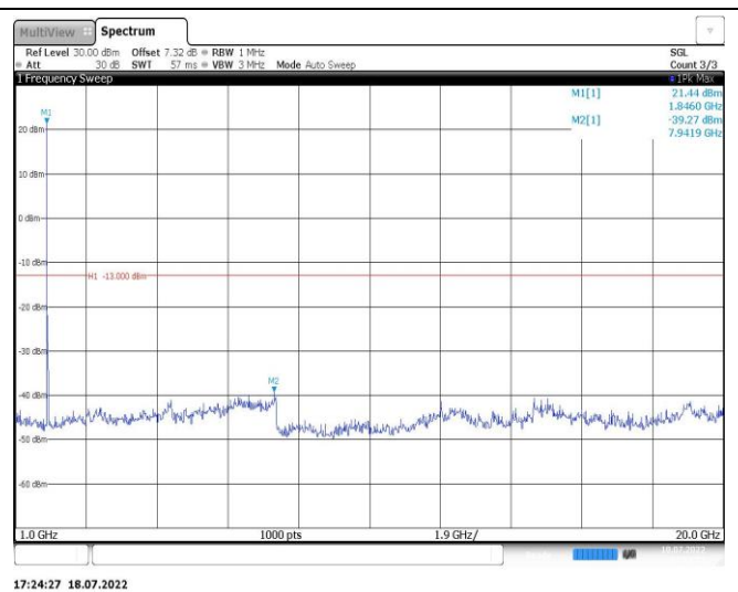
Band2-15MHz-16QAM-18900-1RB#0-Range2:1000~20000MHz
