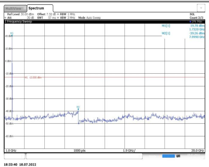
Band4-15MHz-QPSK-20325-1RB#0-Range2:1000~20000MHz
