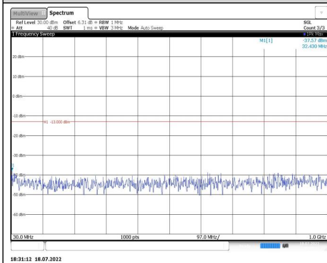
Band4-15MHz-QPSK-20025-1RB#0-Range1:30~1000MHz
