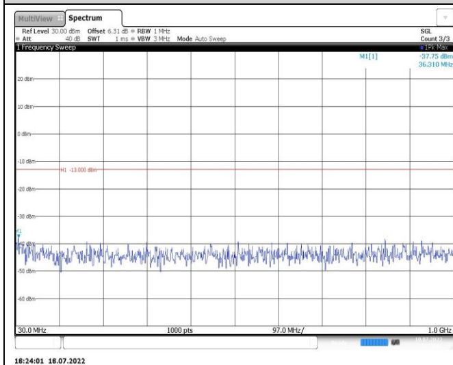
Band4-3MHz-16QAM-20385-1RB#0-Range1:30~1000MHz
