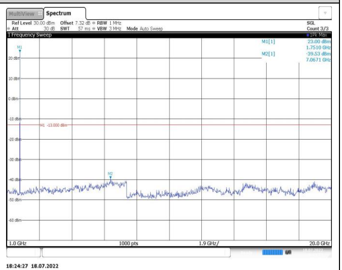
Band4-3MHz-16QAM-19965-1RB#0-Range2:1000~20000MHz
