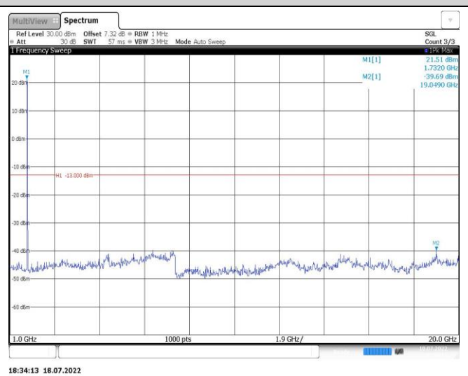
Band4-15MHz-16QAM-20025-1RB#0-Range2:1000~20000MHz
