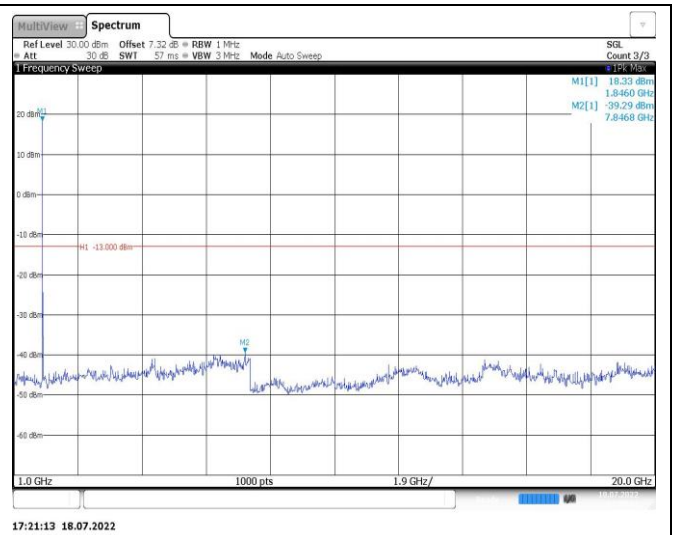
Band2-10MHz-16QAM-18900-1RB#0-Range2:1000~20000MHz
