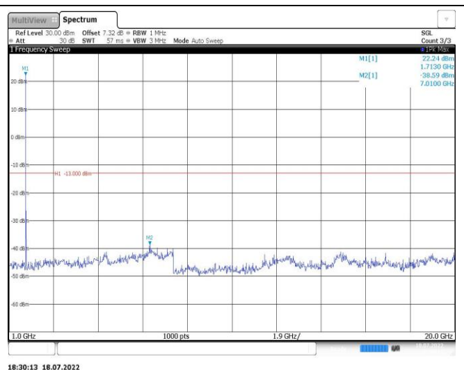
Band4-10MHz-16QAM-20175-1RB#0-Range2:1000~20000MHz
