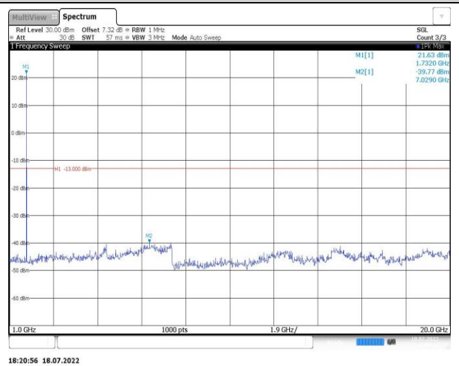
Band4-1.4MHz-16QAM-20393-1RB#0-Range2:1000~20000MHz
