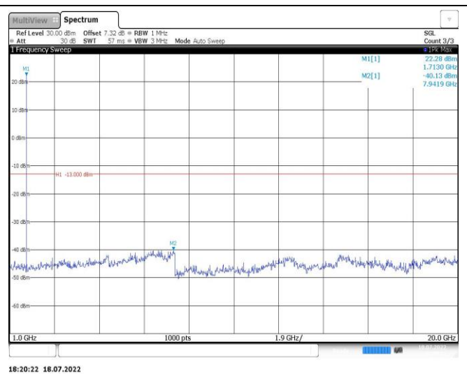
Band4-1.4MHz-16QAM-20175-1RB#0-Range2:1000~20000MHz
