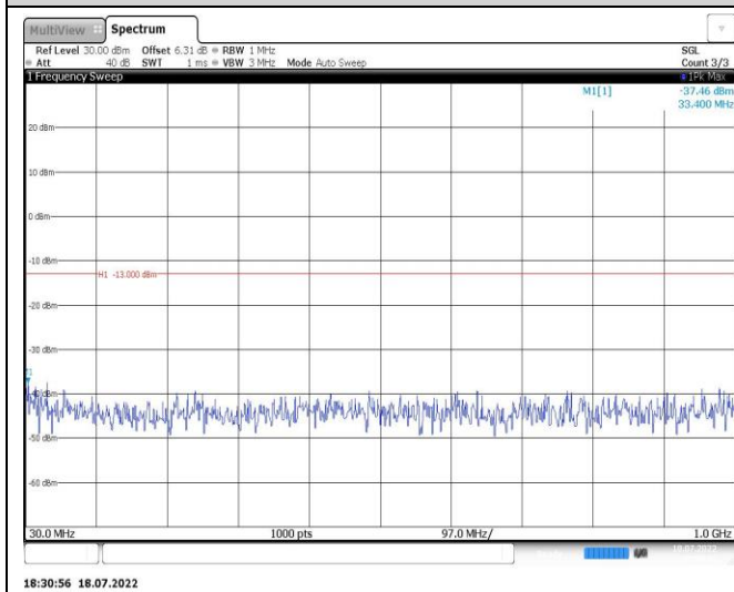
Band4-10MHz-16QAM-20000-1RB#0-Range1:30~1000MHz
