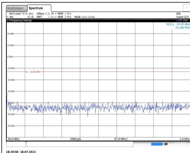
Band4-10MHz-QPSK-20175-1RB#0-Range1:30~1000MHz
