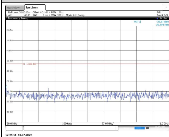
Band2-15MHz-16QAM-18675-1RB#0-Range1:30~1000MHz
