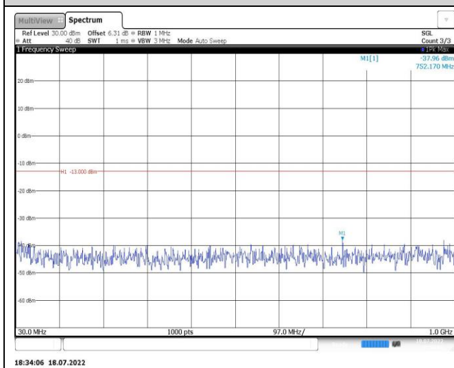
Band4-15MHz-16QAM-20025-1RB#0-Range1:30~1000MHz
