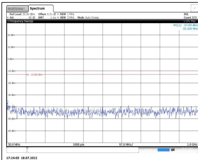
Band2-15MHz-QPSK-18900-1RB#0-Range1:30~1000MHz
