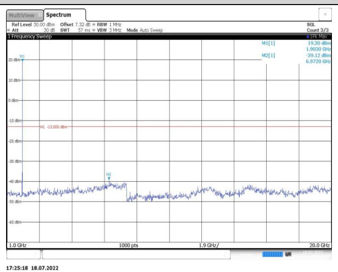
Band2-15MHz-16QAM-18675-1RB#0-Range2:1000~20000MHz
