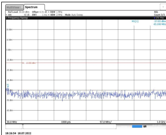
Band4-5MHz-16QAM-20175-1RB#0-Range1:30~1000MHz
