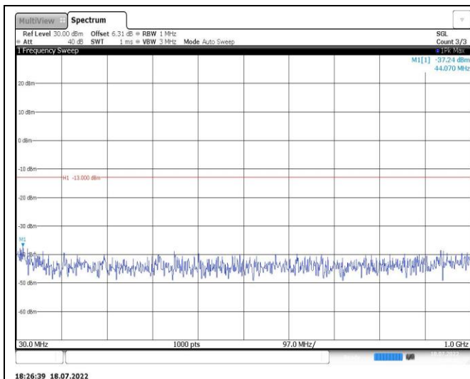
Band4-5MHz-QPSK-20175-1RB#0-Range1:30~1000MHz
