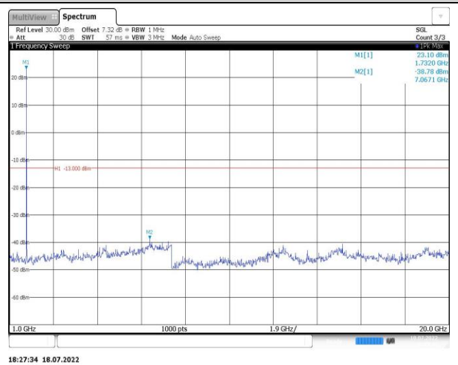
Band4-5MHz-16QAM-20375-1RB#0-Range2:1000~20000MHz
