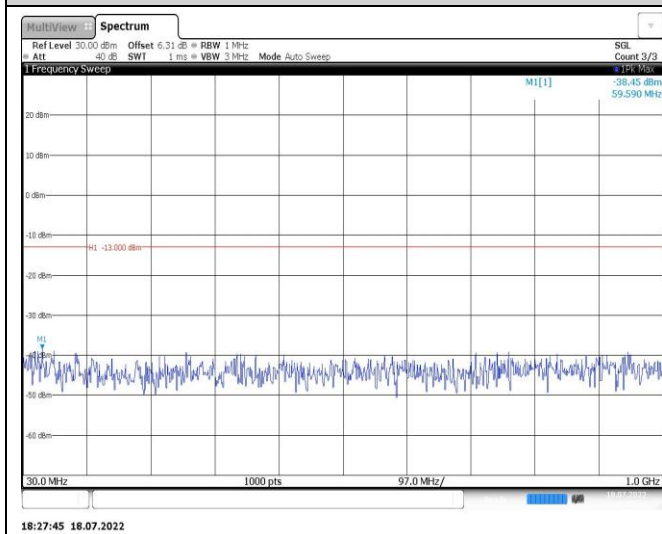
Band4-5MHz-16QAM-19975-1RB#0-Range1:30~1000MHz
