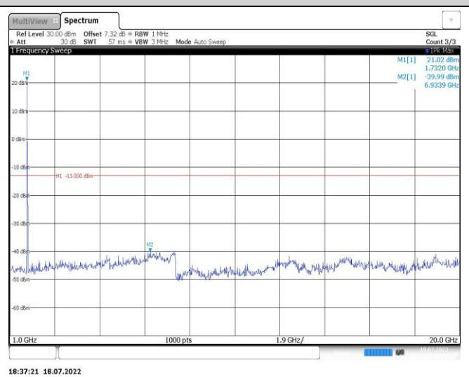
Band4-20MHz-16QAM-20050-1RB#0-Range2:1000~20000MHz
