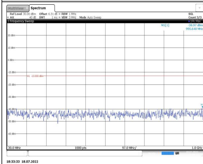
Band4-15MHz-QPSK-20325-1RB#0-Range1:30~1000MHz
