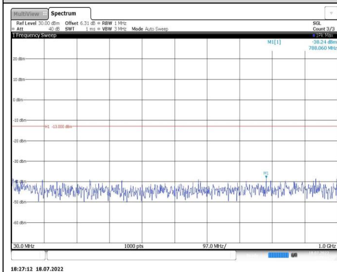
Band4-5MHz-QPSK-20375-1RB#0-Range1:30~1000MHz
