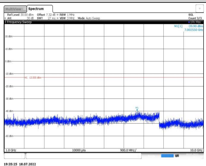
Band12-1.4MHz-QPSK-23173-1RB#0-Range2:1000~10000MHz
