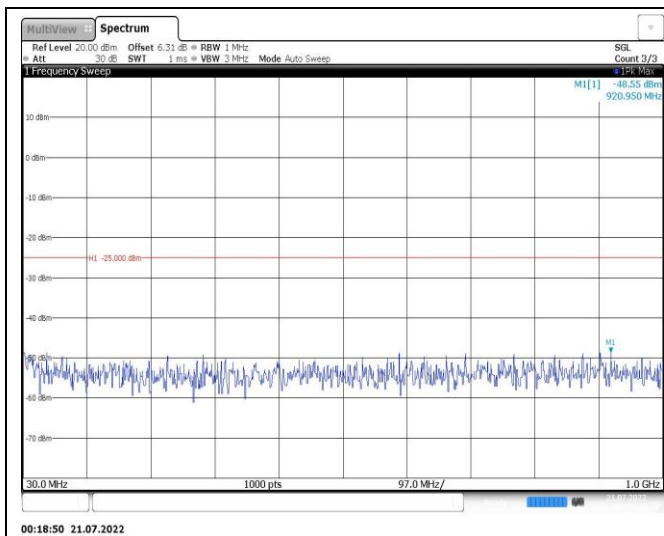
Band7-5MHz-16QAM-21100-1RB#0-Range1:30~1000MHz
