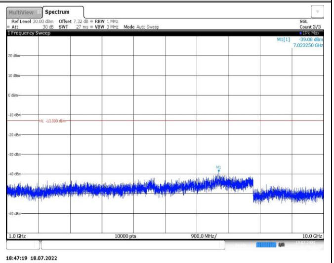
Band5-10MHz-QPSK-20450-1RB#0-Range2:1000~10000MHz
