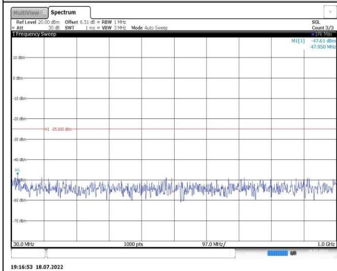
Band7-15MHz-16QAM-21375-1RB#0-Range1:30~1000MHz
