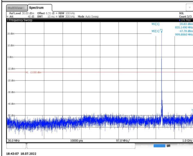
Band5-3MHz-16QAM-20635-1RB#0-Range1:30~1000MHz
