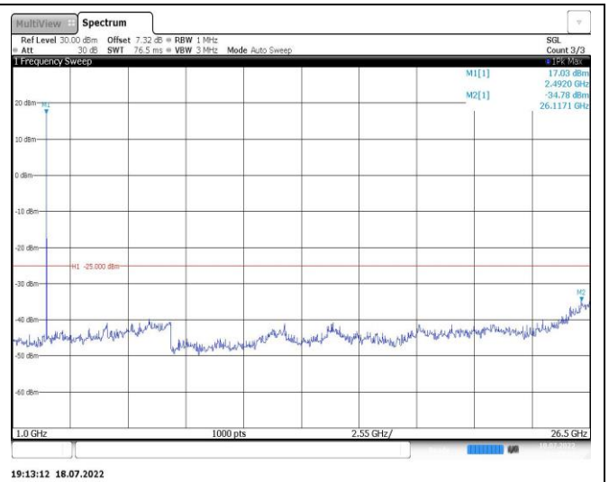
Band7-10MHz-16QAM-21100-1RB#0-Range2:1000~26500MHz
