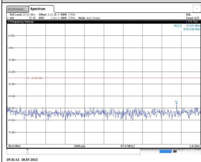
Band7-20MHz-16QAM-20850-1RB#0-Range1:30~1000MHz
