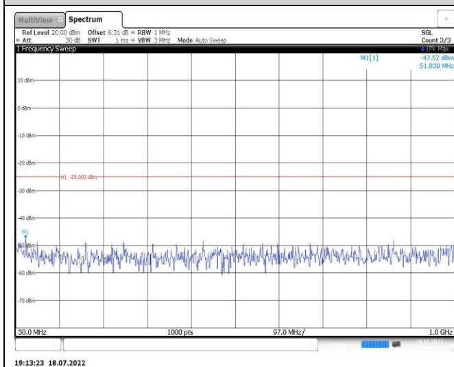
Band7-10MHz-QPSK-21400-1RB#0-Range1:30~1000MHz
