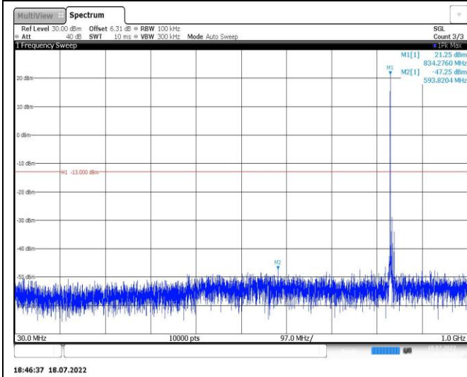
Band5-5MHz-16QAM-20625-1RB#0-Range1:30~1000MHz
