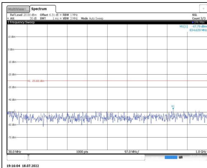
Band7-15MHz-QPSK-21100-1RB#0-Range1:30~1000MHz
