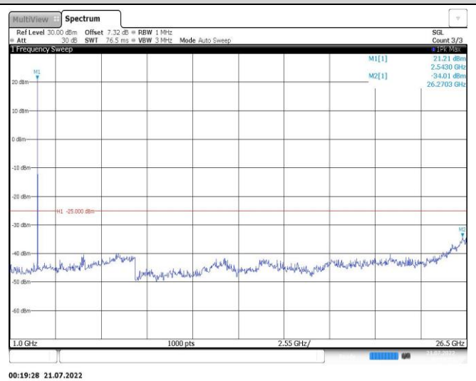
Band7-5MHz-16QAM-21425-1RB#0-Range2:1000~26500MHz
