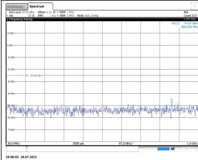
Band7-20MHz-16QAM-21350-1RB#0-Range1:30~1000MHz
