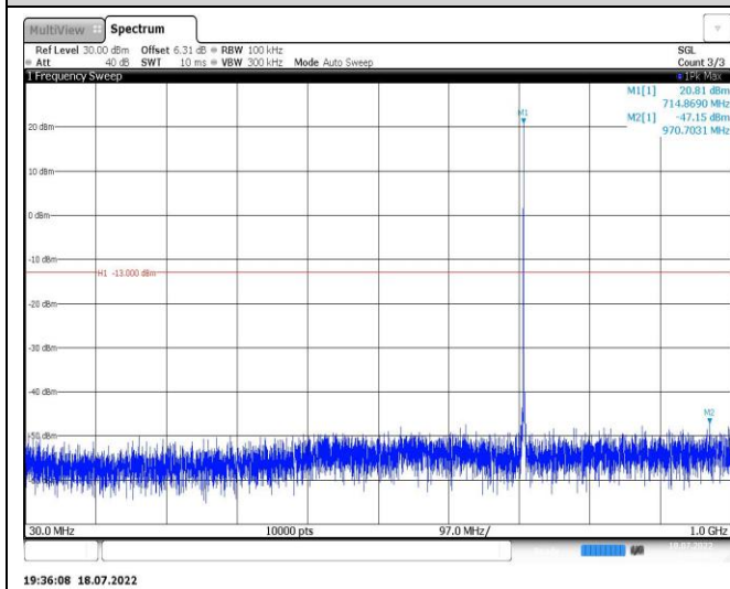
Band12-3MHz-QPSK-23025-1RB#0-Range1:30~1000MHz
