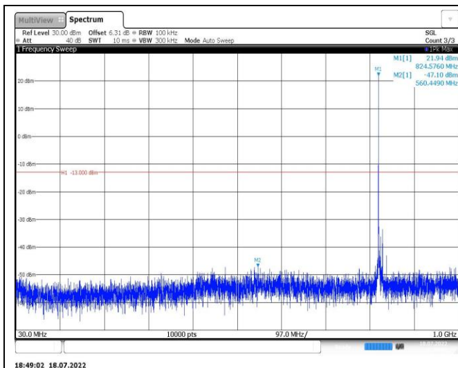
Band5-10MHz-QPSK-20525-1RB#0-Range1:30~1000MHz
