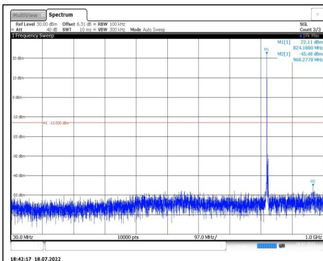
Band5-3MHz-QPSK-20525-1RB#0-Range1:30~1000MHz
