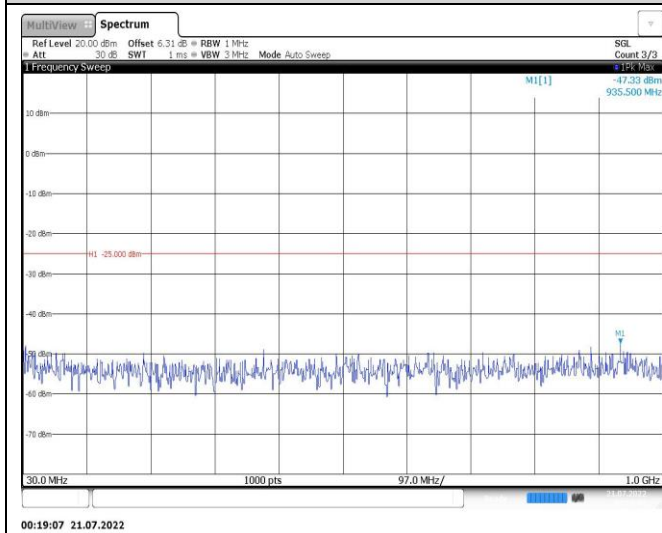
Band7-5MHz-QPSK-21425-1RB#0-Range1:30~1000MHz
