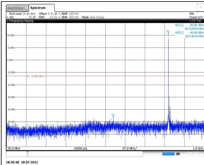
Band5-5MHz-QPSK-20525-1RB#0-Range1:30~1000MHz
