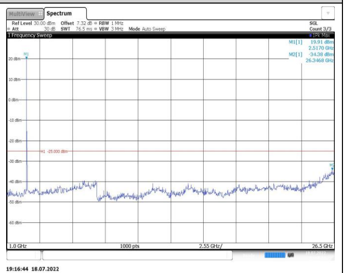
Band7-15MHz-QPSK-21375-1RB#0-Range2:1000~26500MHz
