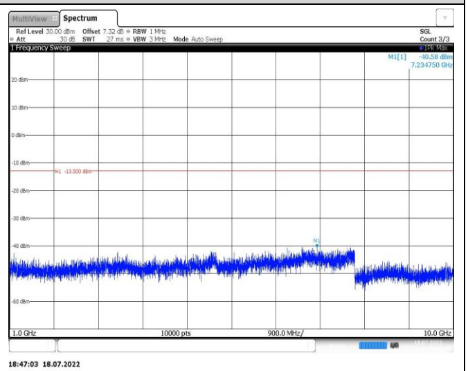
Band5-5MHz-16QAM-20425-1RB#0-Range2:1000~10000MHz
