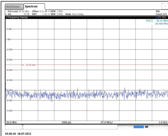
Band7-20MHz-16QAM-21100-1RB#0-Range1:30~1000MHz
