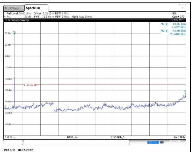
Band7-15MHz-QPSK-21100-1RB#0-Range2:1000~26500MHz
