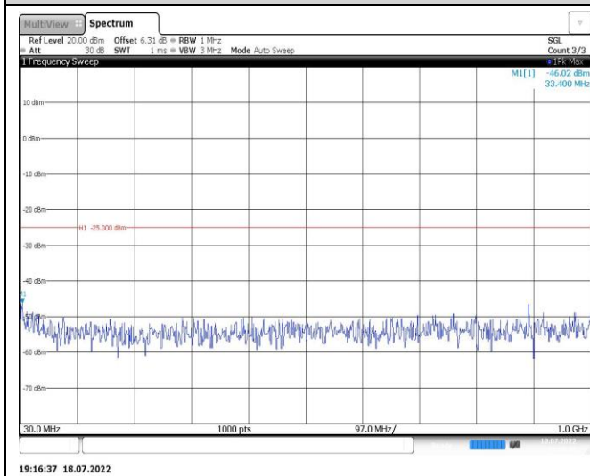
Band7-15MHz-QPSK-21375-1RB#0-Range1:30~1000MHz
