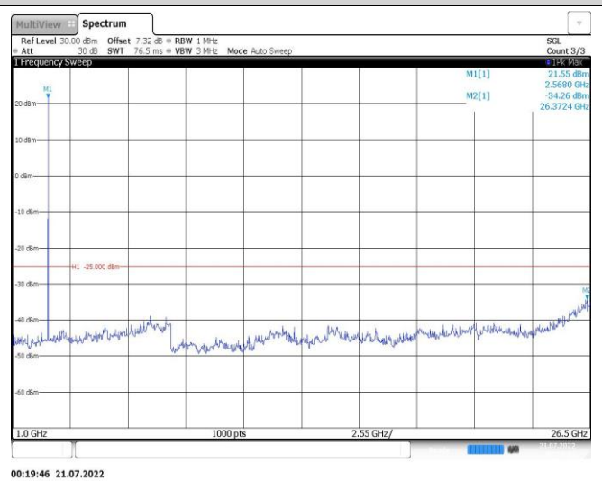
Band7-5MHz-16QAM-20775-1RB#0-Range2:1000~26500MHz
