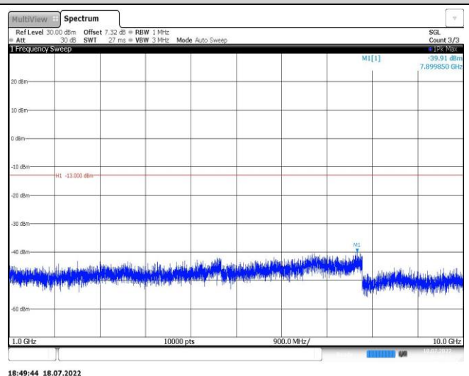
Band5-10MHz-QPSK-20600-1RB#0-Range2:1000~10000MHz
