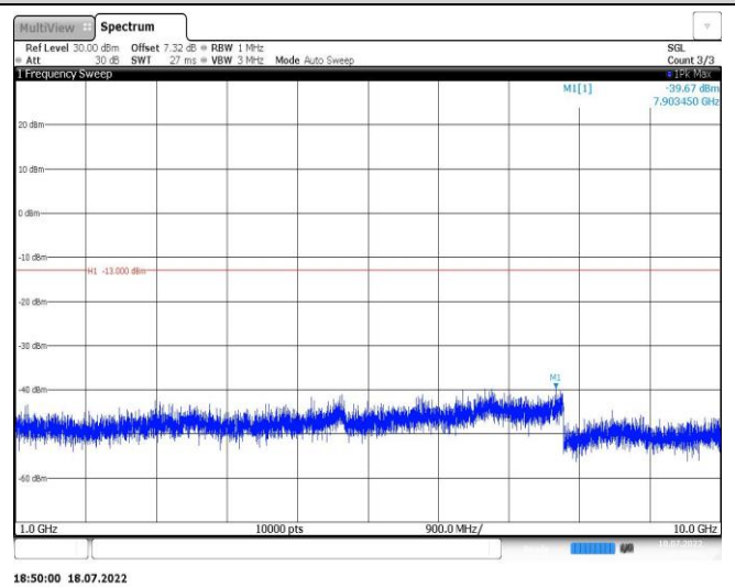
Band5-10MHz-16QAM-20600-1RB#0-Range2:1000~10000MHz
