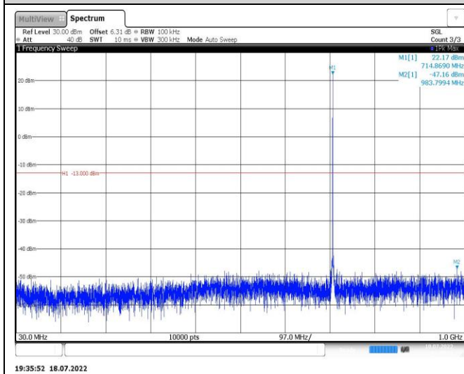
Band12-1.4MHz-16QAM-23017-1RB#0-Range1:30~1000MHz
