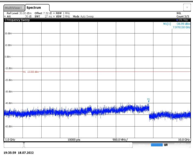
Band12-1.4MHz-16QAM-23017-1RB#0-Range2:1000~10000MHz
