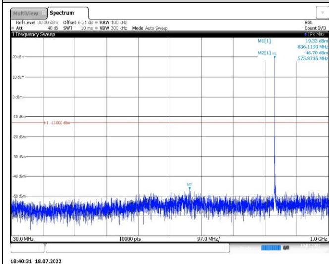
Band5-1.4MHz-16QAM-20643-1RB#0-Range1:30~1000MHz
