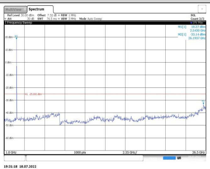
Band7-20MHz-16QAM-20850-1RB#0-Range2:1000~26500MHz
