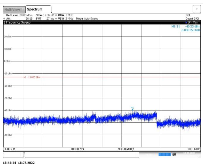
Band5-3MHz-QPSK-20525-1RB#0-Range2:1000~10000MHz
