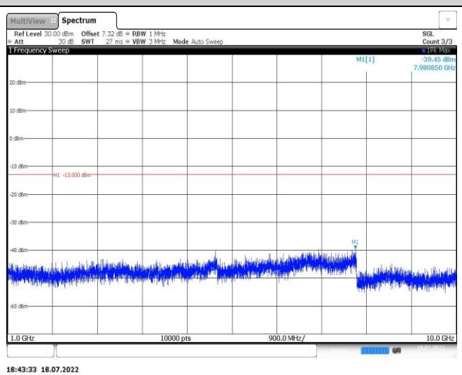
Band5-3MHz-16QAM-20415-1RB#0-Range2:1000~10000MHz
