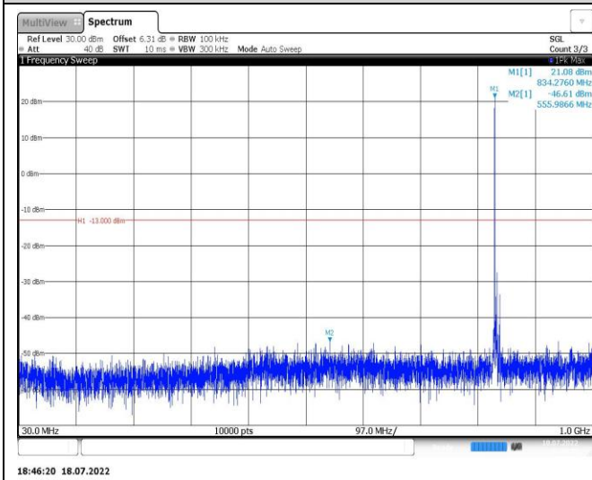
Band5-5MHz-QPSK-20625-1RB#0-Range1:30~1000MHz
