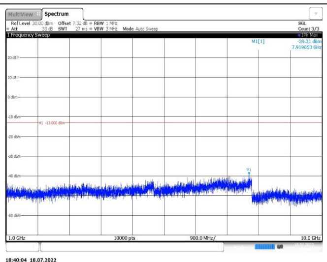
Band5-1.4MHz-16QAM-20525-1RB#0-Range2:1000~10000MHz
