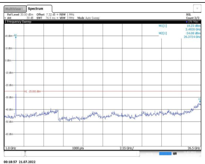
Band7-5MHz-16QAM-21100-1RB#0-Range2:1000~26500MHz
