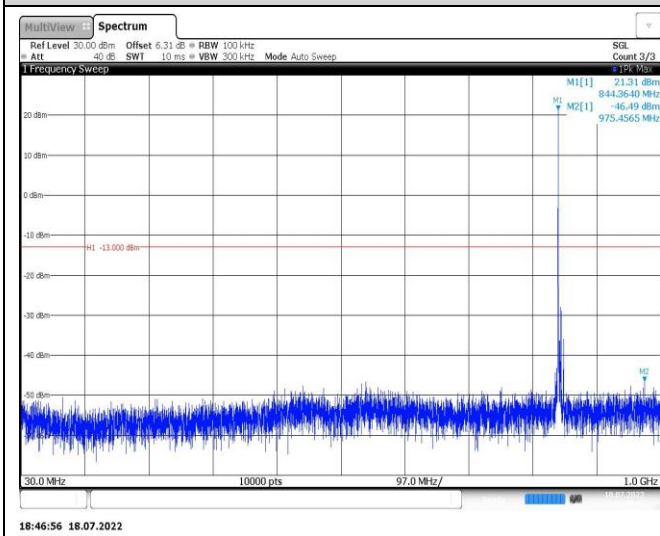
Band5-5MHz-16QAM-20425-1RB#0-Range1:30~1000MHz
