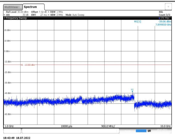
Band5-5MHz-QPSK-20425-1RB#0-Range2:1000~10000MHz
