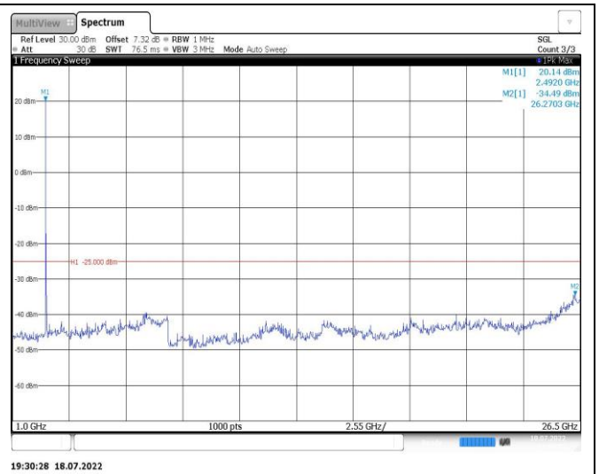
Band7-20MHz-16QAM-21100-1RB#0-Range2:1000~26500MHz
