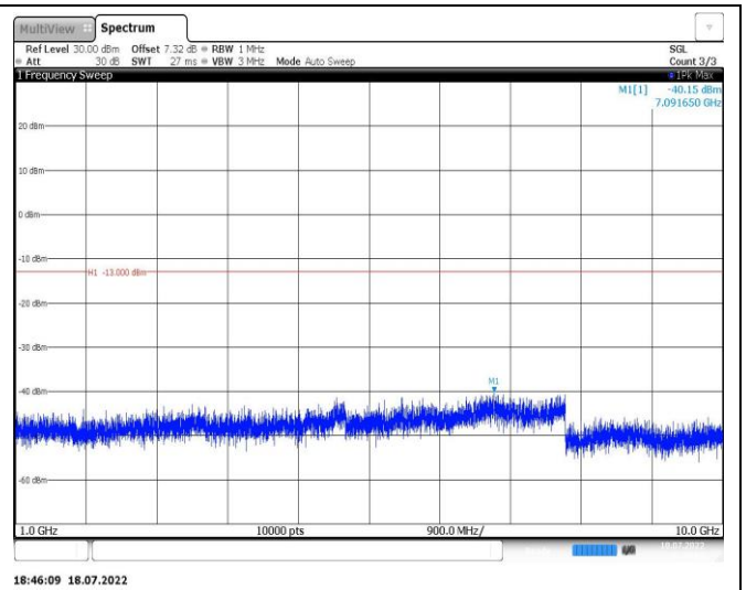
Band5-5MHz-16QAM-20525-1RB#0-Range2:1000~10000MHz
