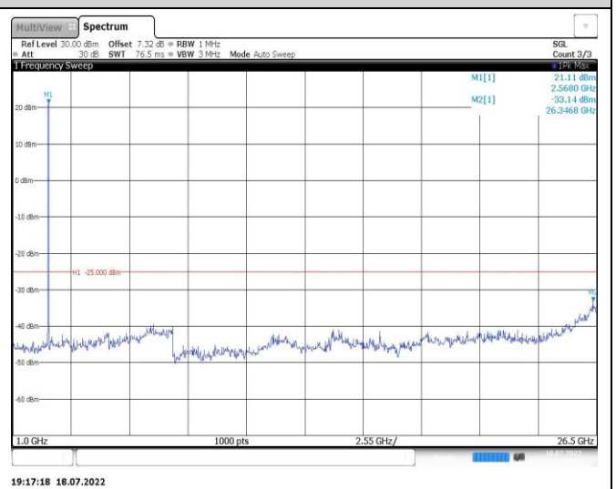
Band7-15MHz-16QAM-20825-1RB#0-Range2:1000~26500MHz
