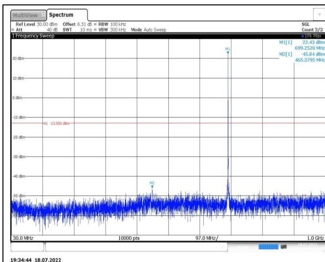
Band12-1.4MHz-QPSK-23095-1RB#0-Range1:30~1000MHz
