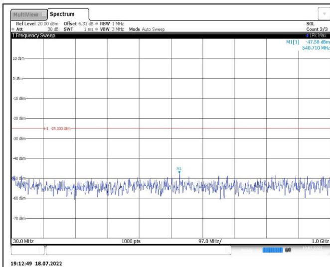
Band7-10MHz-QPSK-21100-1RB#0-Range1:30~1000MHz
