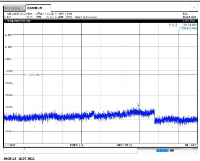
Band12-3MHz-QPSK-23025-1RB#0-Range2:1000~10000MHz
