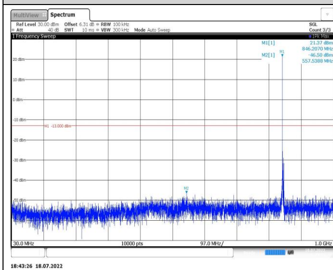
Band5-3MHz-16QAM-20415-1RB#0-Range1:30~1000MHz
