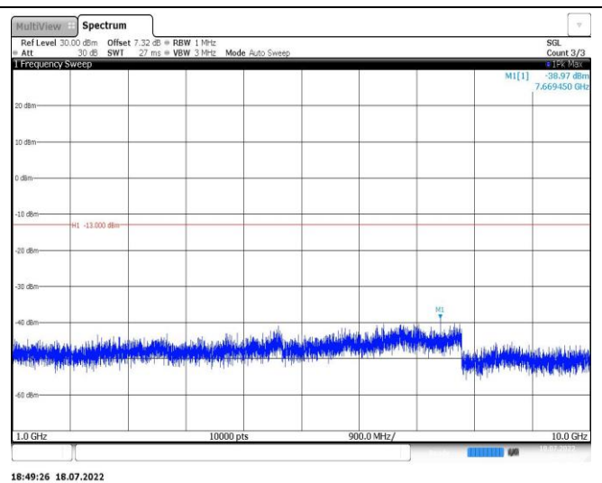
Band5-10MHz-16QAM-20525-1RB#0-Range2:1000~10000MHz
