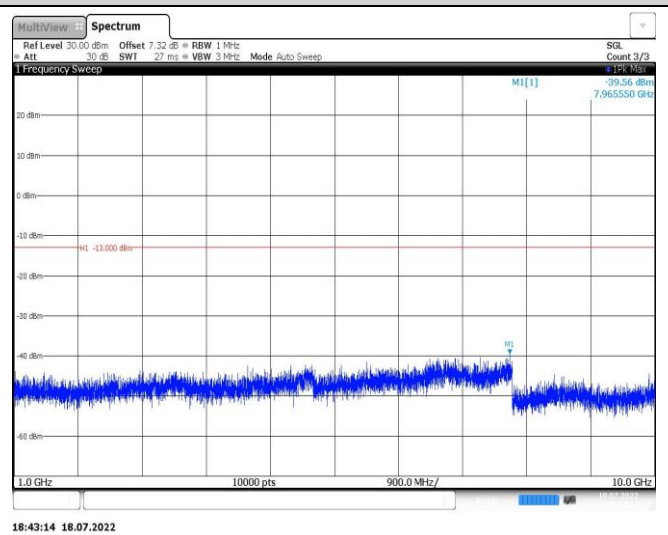
Band5-3MHz-16QAM-20635-1RB#0-Range2:1000~10000MHz
