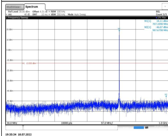
Band12-1.4MHz-16QAM-23173-1RB#0-Range1:30~1000MHz
