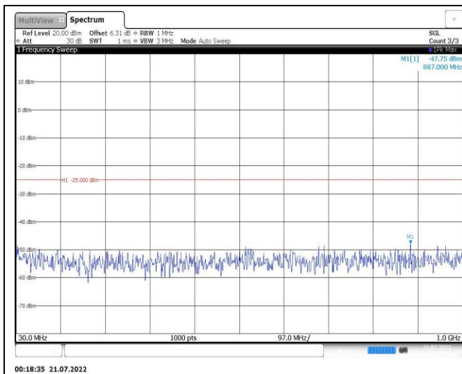
Band7-5MHz-QPSK-21100-1RB#0-Range1:30~1000MHz
