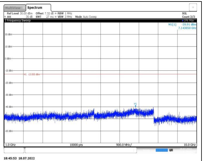
Band5-5MHz-QPSK-20525-1RB#0-Range2:1000~10000MHz
