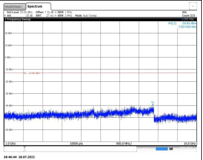
Band5-5MHz-16QAM-20625-1RB#0-Range2:1000~10000MHz
