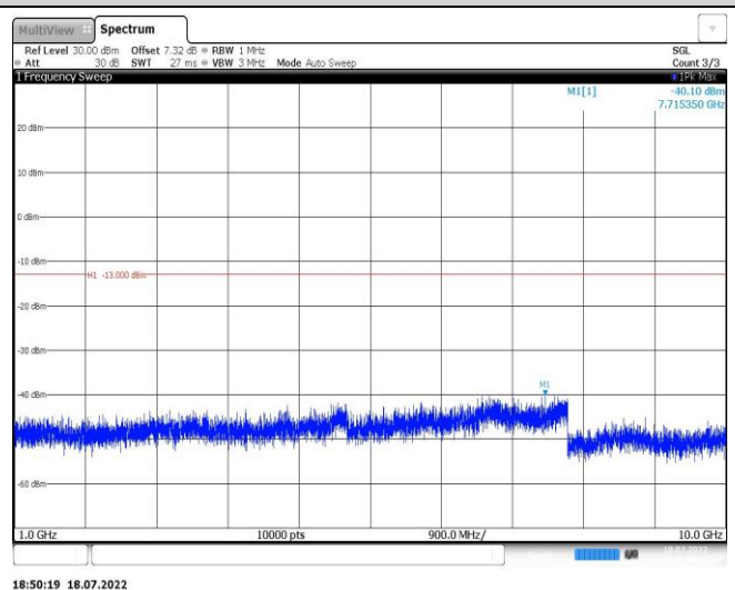
Band5-10MHz-16QAM-20450-1RB#0-Range2:1000~10000MHz
