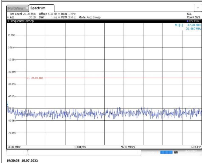
Band7-20MHz-QPSK-21350-1RB#0-Range1:30~1000MHz
