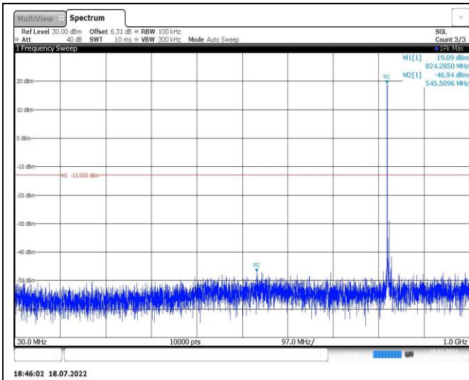
Band5-5MHz-16QAM-20525-1RB#0-Range1:30~1000MHz
