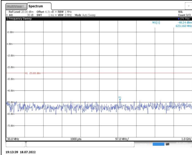
Band7-10MHz-16QAM-21400-1RB#0-Range1:30~1000MHz
