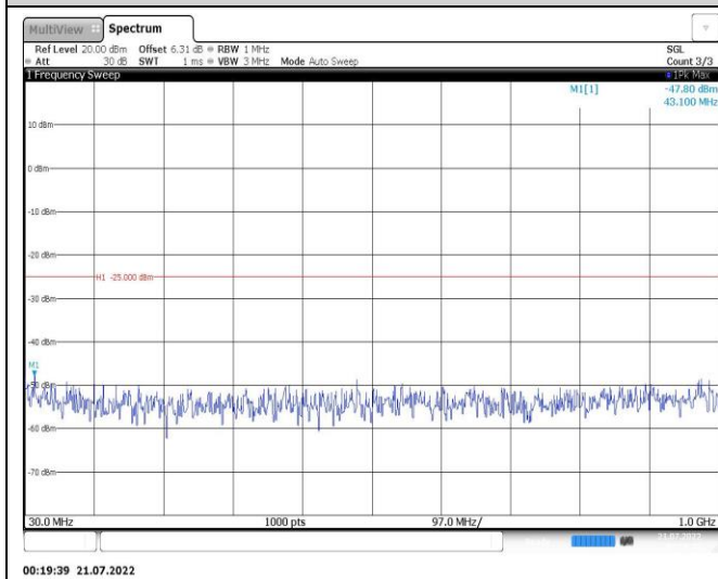
Band7-5MHz-16QAM-20775-1RB#0-Range1:30~1000MHz
