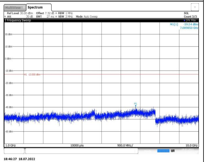
Band5-5MHz-QPSK-20625-1RB#0-Range2:1000~10000MHz
