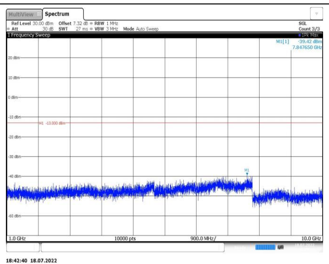
Band5-3MHz-16QAM-20525-1RB#0-Range2:1000~10000MHz
