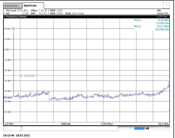
Band7-10MHz-16QAM-21400-1RB#0-Range2:1000~26500MHz
