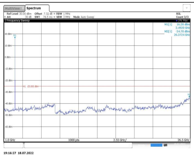
Band7-15MHz-16QAM-21100-1RB#0-Range2:1000~26500MHz
