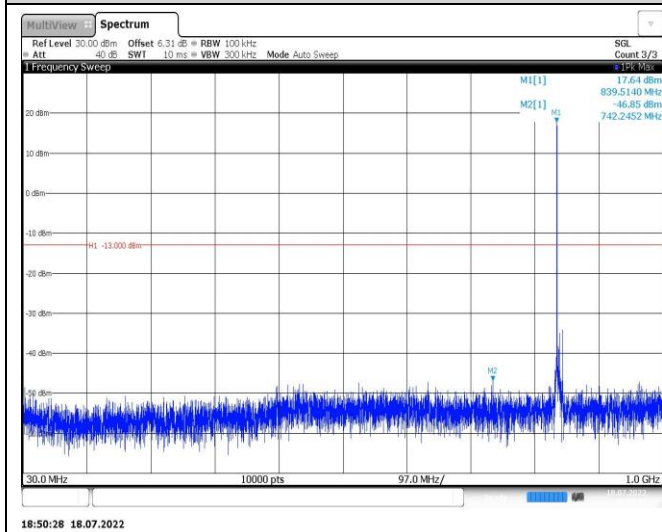
Band7-5MHz-QPSK-20775-1RB#0-Range1:30~1000MHz
