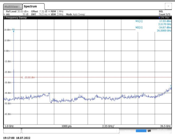
Band7-15MHz-16QAM-21375-1RB#0-Range2:1000~26500MHz
