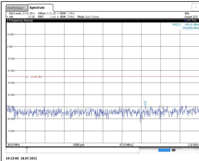
Band7-10MHz-16QAM-21100-1RB#0-Range1:30~1000MHz
