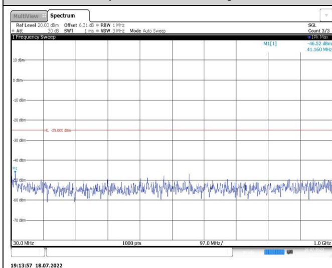
Band7-10MHz-16QAM-20800-1RB#0-Range1:30~1000MHz
