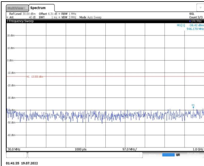
Band25-1.4MHz-16QAM-26365-1RB#0-Range1:30~1000MHz
