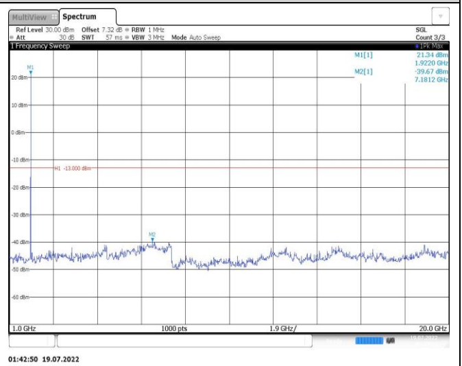
Band25-3MHz-QPSK-26055-1RB#0-Range2:1000~20000MHz
