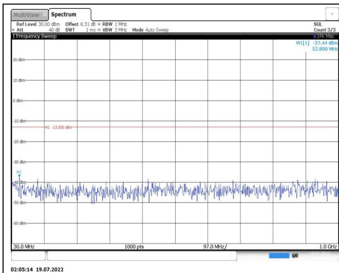
Band25-5MHz-16QAM-26365-1RB#0-Range1:30~1000MHz
