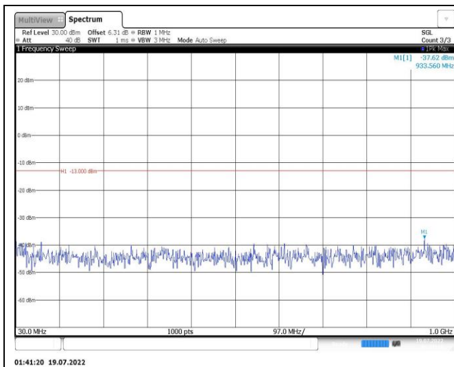
Band25-1.4MHz-QPSK-26365-1RB#0-Range1:30~1000MHz
