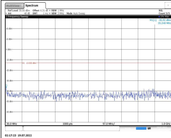
Band25-10MHz-QPSK-26640-1RB#0-Range1:30~1000MHz
