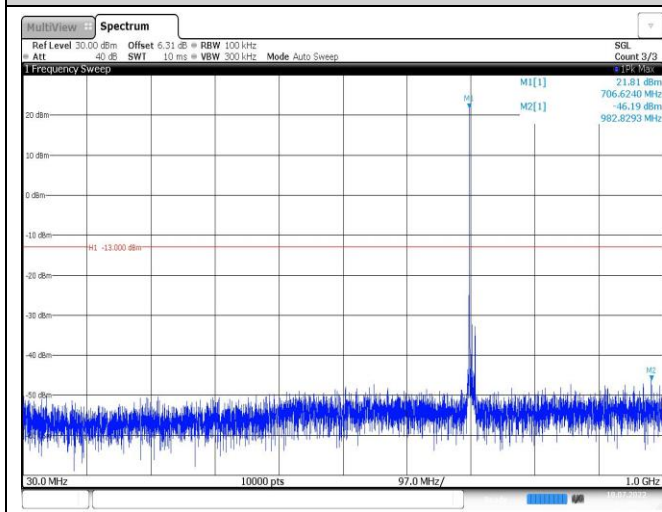
Band12-10MHz-QPSK-23130-1RB#0-Range1:30~1000MHz
