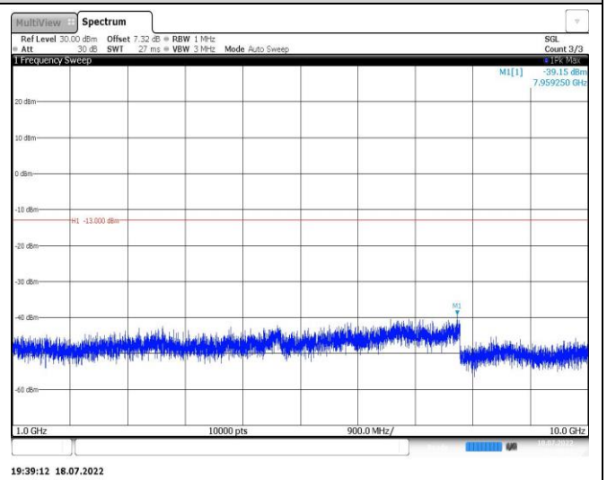
Band12-3MHz-16QAM-23025-1RB#0-Range2:1000~10000MHz
