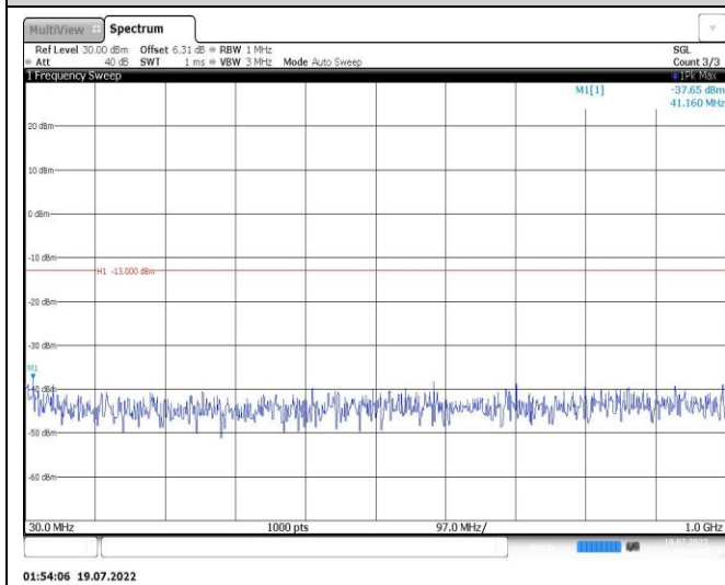
Band25-3MHz-16QAM-26055-1RB#0-Range1:30~1000MHz
