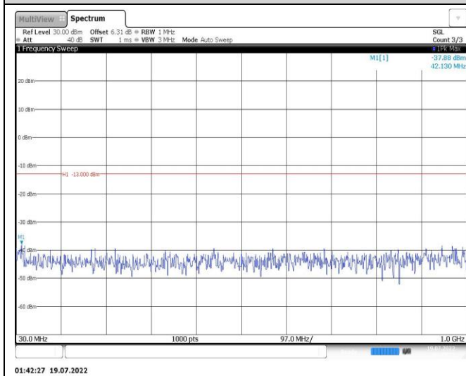
Band25-1.4MHz-16QAM-26047-1RB#0-Range1:30~1000MHz
