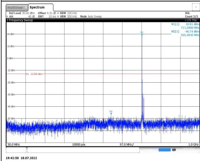
Band12-10MHz-QPSK-23060-1RB#0-Range1:30~1000MHz
