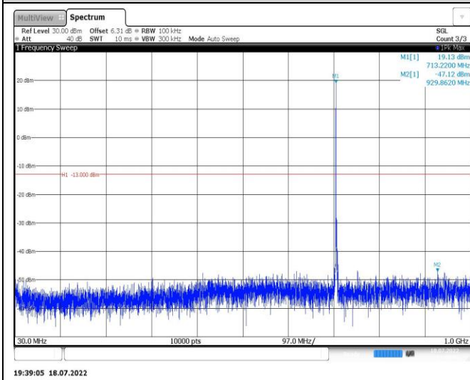
Band12-3MHz-16QAM-23025-1RB#0-Range1:30~1000MHz
