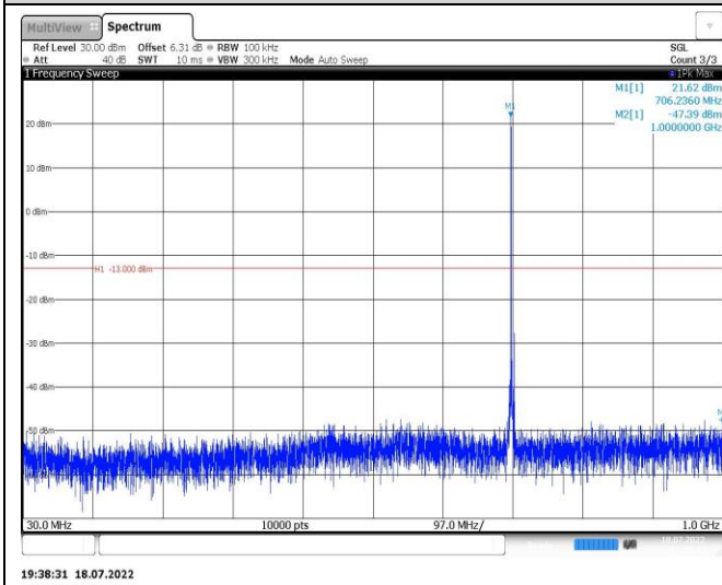
Band12-3MHz-QPSK-23165-1RB#0-Range1:30~1000MHz
