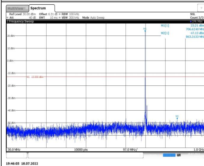
Band13-5MHz-QPSK-23205-1RB#0-Range1:30~1000MHz
