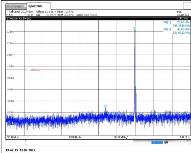
Band12-5MHz-16QAM-23155-1RB#0-Range1:30~1000MHz
