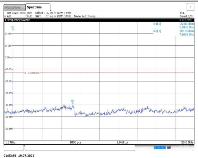
Band25-3MHz-16QAM-26675-1RB#0-Range2:1000~20000MHz
