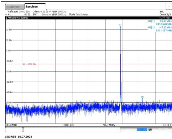
Band12-3MHz-QPSK-23095-1RB#0-Range1:30~1000MHz
