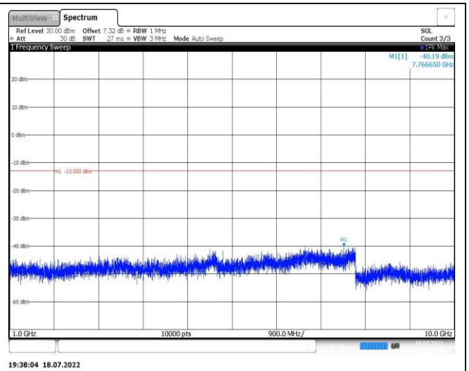
Band12-3MHz-QPSK-23095-1RB#0-Range2:1000~10000MHz
