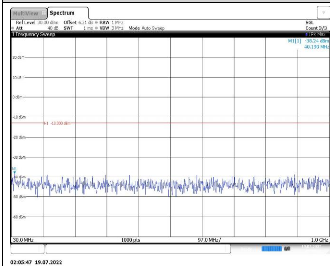
Band25-5MHz-16QAM-26665-1RB#0-Range1:30~1000MHz
