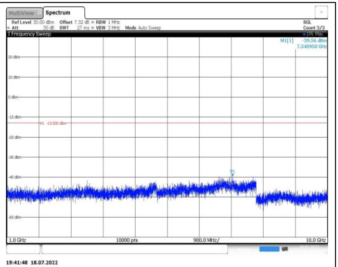
Band12-5MHz-16QAM-23095-1RB#0-Range2:1000~10000MHz
