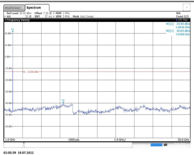
Band25-5MHz-QPSK-26665-1RB#0-Range2:1000~20000MHz
