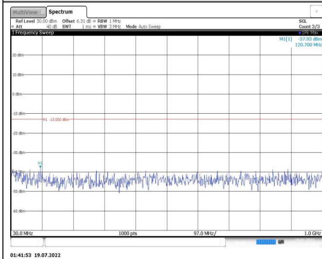
Band25-1.4MHz-QPSK-26683-1RB#0-Range1:30~1000MHz
