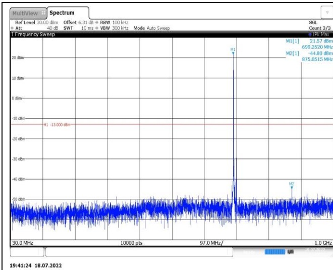
Band12-5MHz-QPSK-23095-1RB#0-Range1:30~1000MHz
