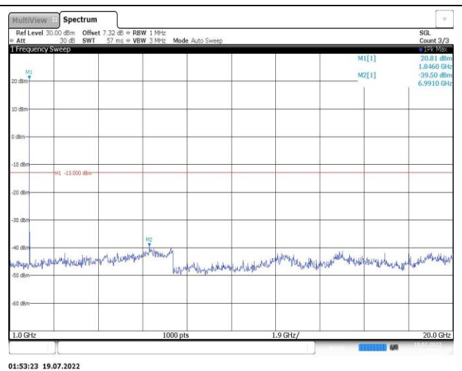
Band25-3MHz-16QAM-26365-1RB#0-Range2:1000~20000MHz
