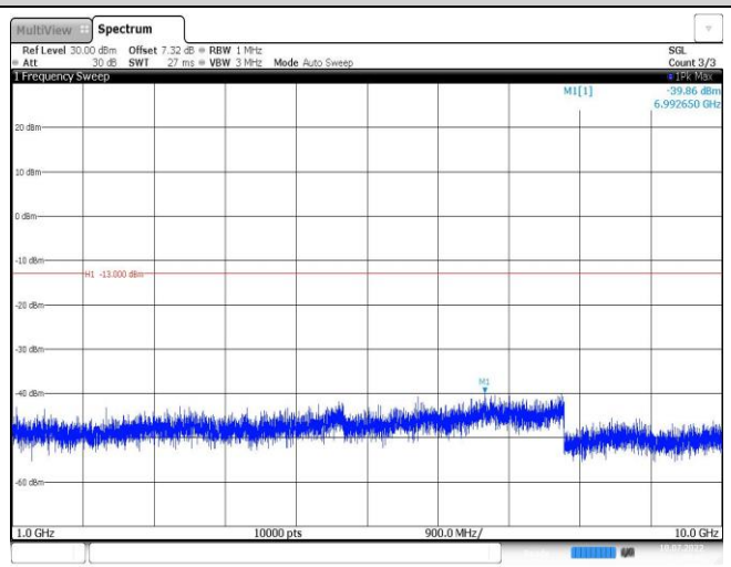
Band12-10MHz-QPSK-23130-1RB#0-Range2:1000~10000MHz
