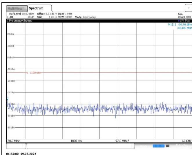
Band25-3MHz-QPSK-26365-1RB#0-Range1:30~1000MHz
