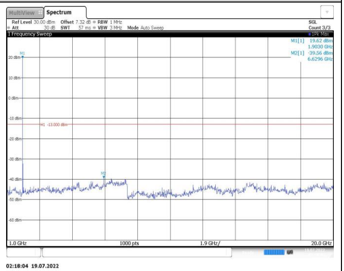
Band25-10MHz-16QAM-26090-1RB#0-Range2:1000~20000MHz
