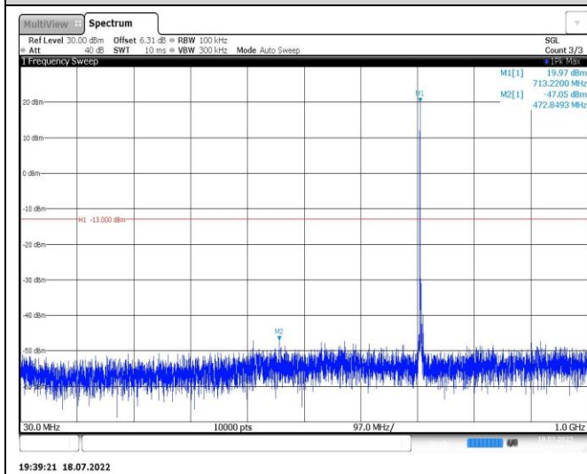
Band12-5MHz-QPSK-23035-1RB#0-Range1:30~1000MHz
