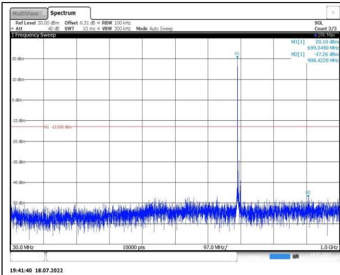
Band12-5MHz-16QAM-23095-1RB#0-Range1:30~1000MHz
