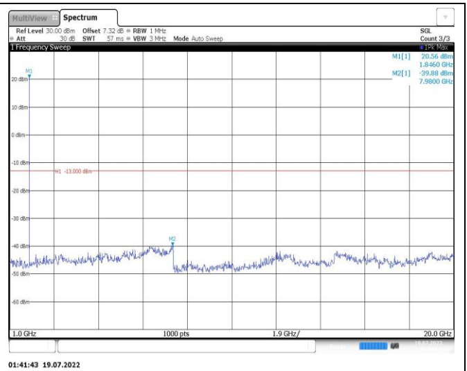
Band25-1.4MHz-16QAM-26365-1RB#0-Range2:1000~20000MHz
