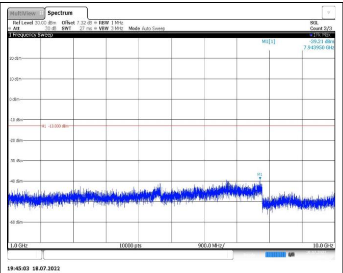
Band12-10MHz-16QAM-23095-1RB#0-Range2:1000~10000MHz
