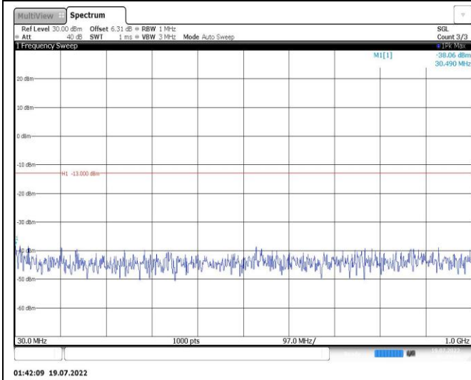
Band25-1.4MHz-16QAM-26683-1RB#0-Range1:30~1000MHz
