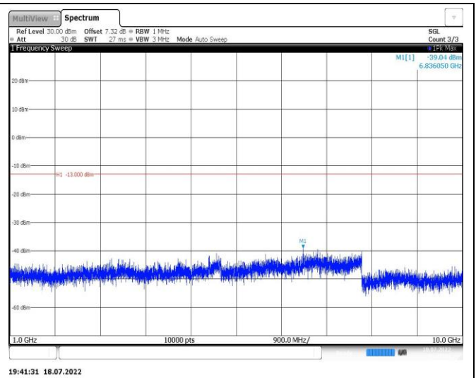
Band12-5MHz-QPSK-23095-1RB#0-Range2:1000~10000MHz
