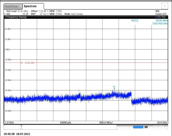
Band12-10MHz-16QAM-23130-1RB#0-Range2:1000~10000MHz
