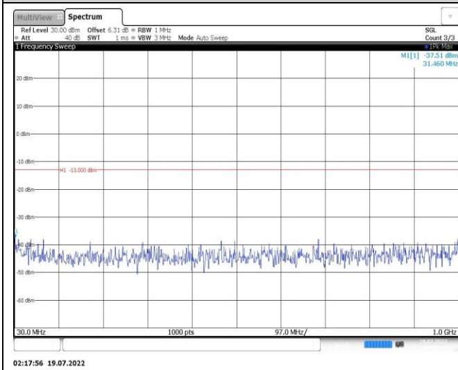
Band25-10MHz-16QAM-26090-1RB#0-Range1:30~1000MHz
