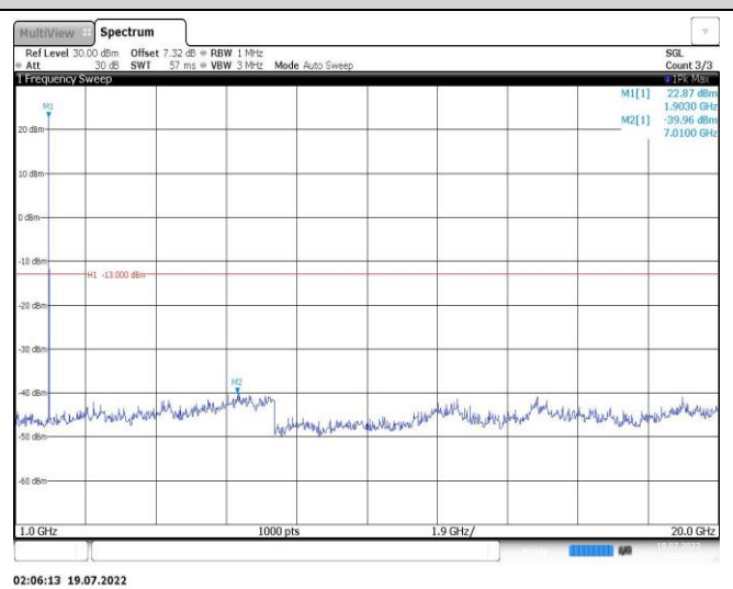
Band25-5MHz-16QAM-26065-1RB#0-Range2:1000~20000MHz
