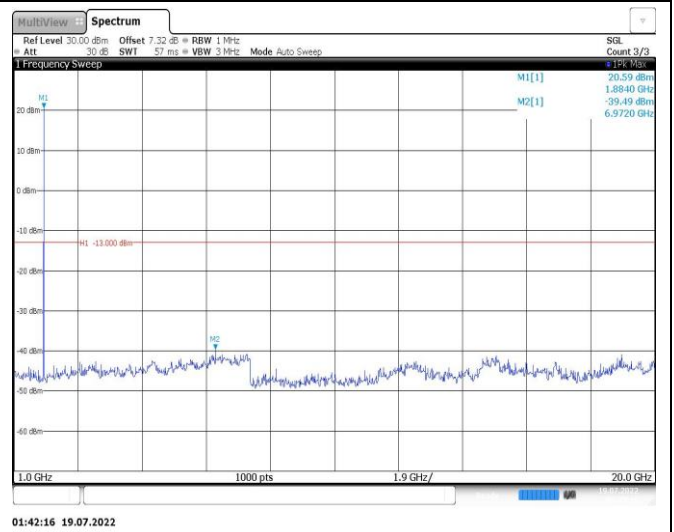
Band25-1.4MHz-16QAM-26683-1RB#0-Range2:1000~20000MHz
