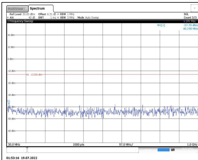
Band25-3MHz-16QAM-26365-1RB#0-Range1:30~1000MHz
