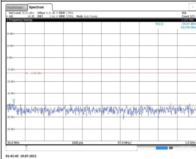
Band25-3MHz-QPSK-26055-1RB#0-Range1:30~1000MHz
