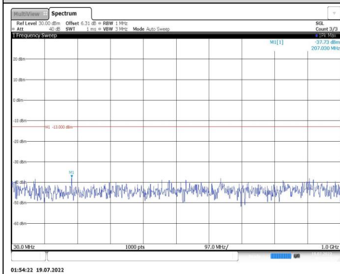
Band25-5MHz-QPSK-26065-1RB#0-Range1:30~1000MHz
