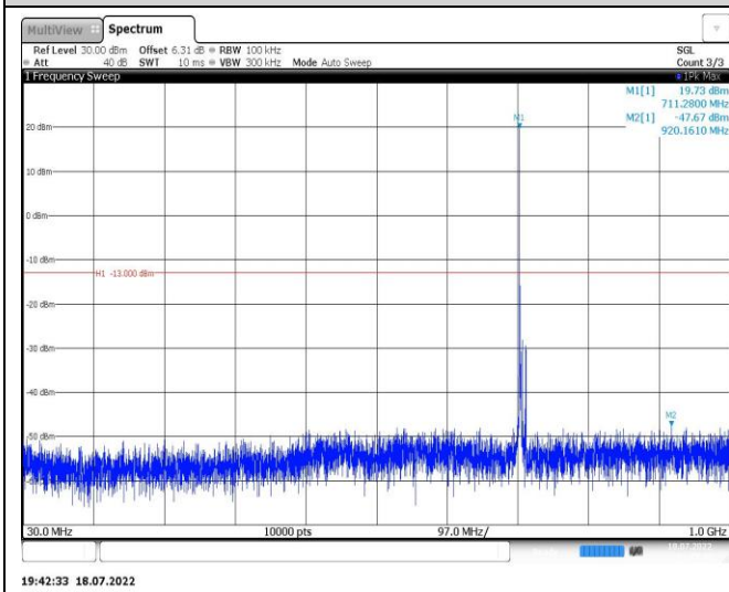
Band12-5MHz-16QAM-23035-1RB#0-Range1:30~1000MHz
