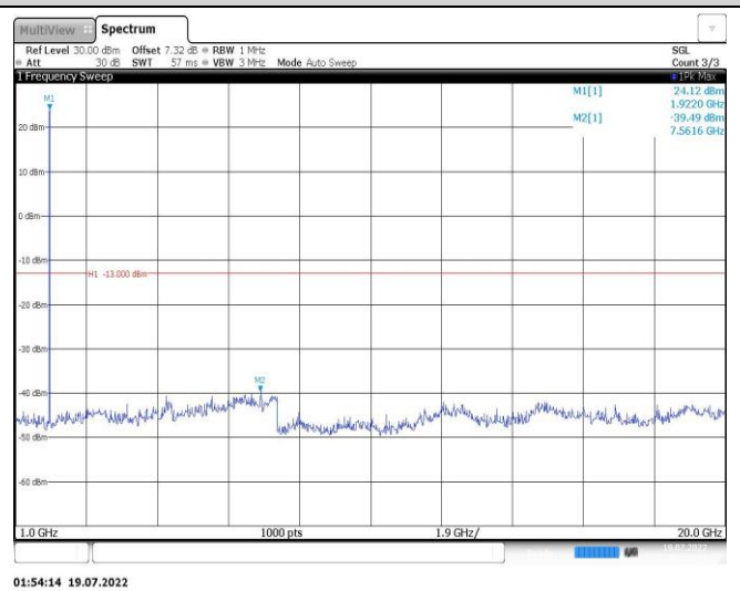
Band25-3MHz-16QAM-26055-1RB#0-Range2:1000~20000MHz
