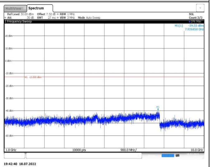
Band12-5MHz-16QAM-23035-1RB#0-Range2:1000~10000MHz
