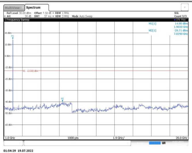
Band25-5MHz-QPSK-26065-1RB#0-Range2:1000~20000MHz
