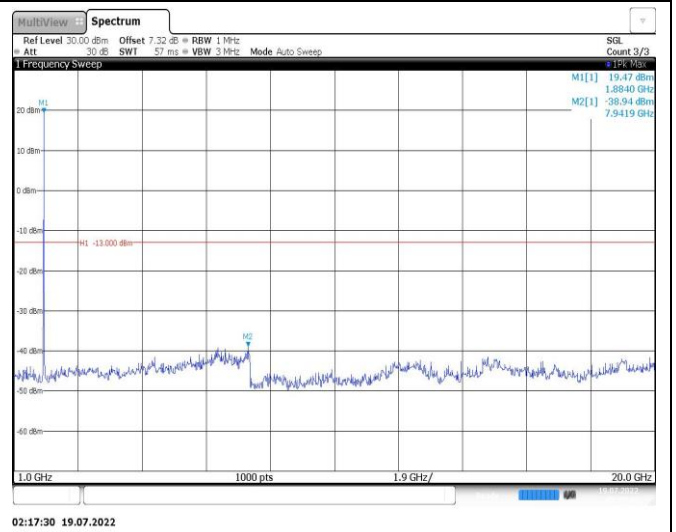
Band25-10MHz-QPSK-26640-1RB#0-Range2:1000~20000MHz
