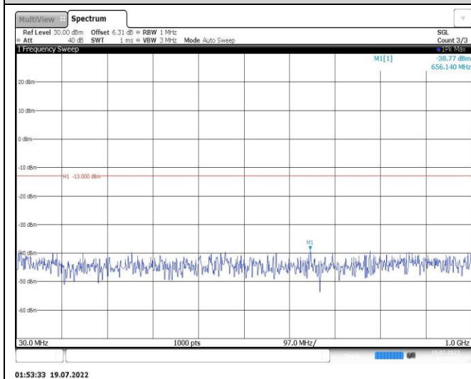
Band25-3MHz-QPSK-26675-1RB#0-Range1:30~1000MHz
