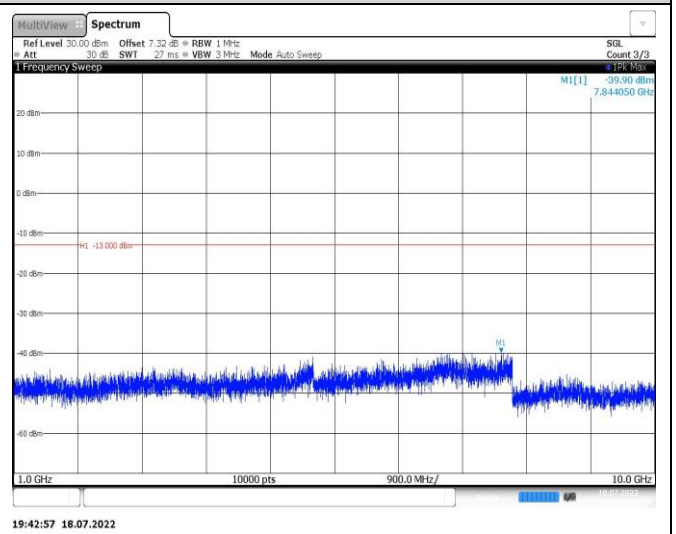
Band12-10MHz-QPSK-23060-1RB#0-Range2:1000~10000MHz
