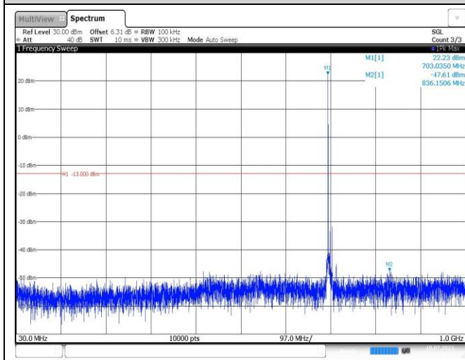
Band12-10MHz-QPSK-23095-1RB#0-Range1:30~1000MHz
