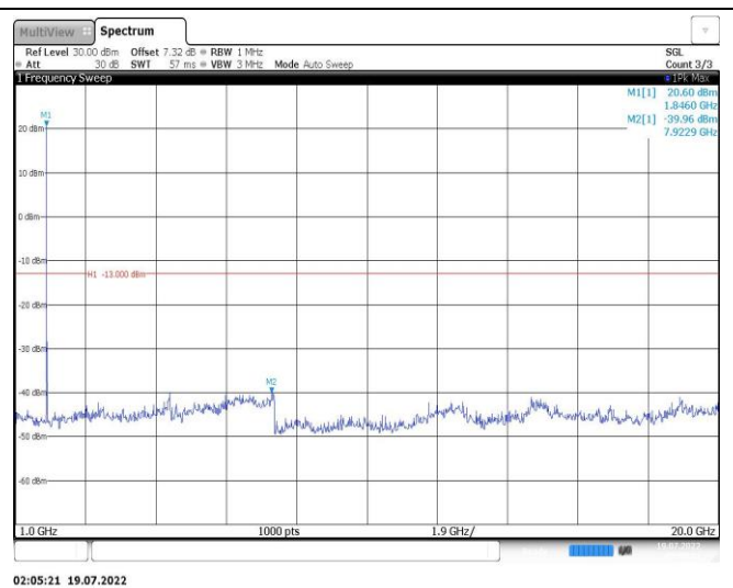
Band25-5MHz-16QAM-26365-1RB#0-Range2:1000~20000MHz
