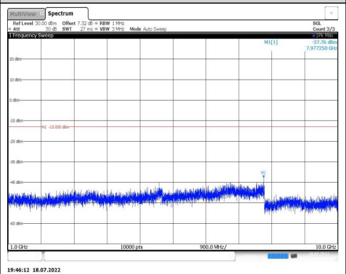
Band13-5MHz-QPSK-23205-1RB#0-Range2:1000~10000MHz
