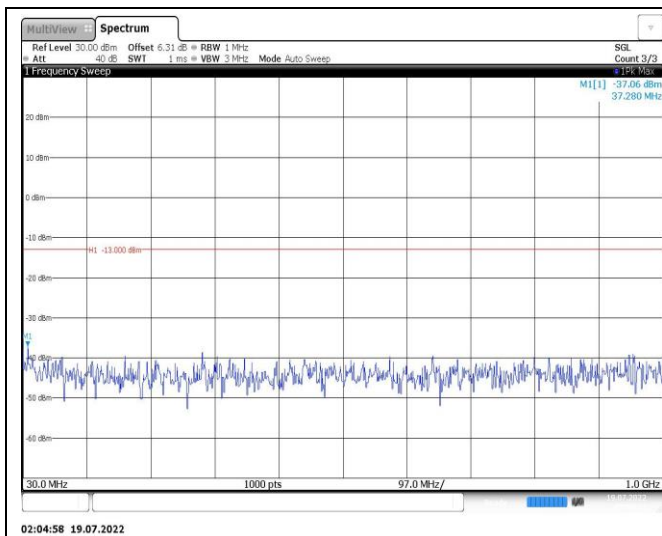
Band25-5MHz-QPSK-26365-1RB#0-Range1:30~1000MHz
