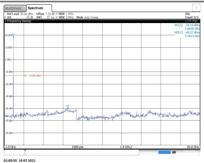
Band25-5MHz-16QAM-26665-1RB#0-Range2:1000~20000MHz
