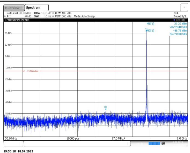
Band13-5MHz-16QAM-23255-1RB#0-Range3:1559~1610MHz
