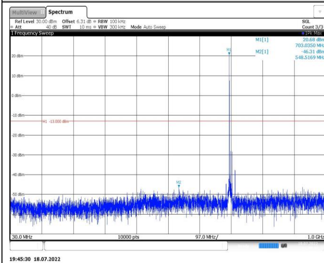
Band12-10MHz-16QAM-23130-1RB#0-Range1:30~1000MHz
