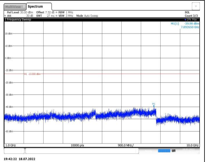
Band12-5MHz-16QAM-23155-1RB#0-Range2:1000~10000MHz
