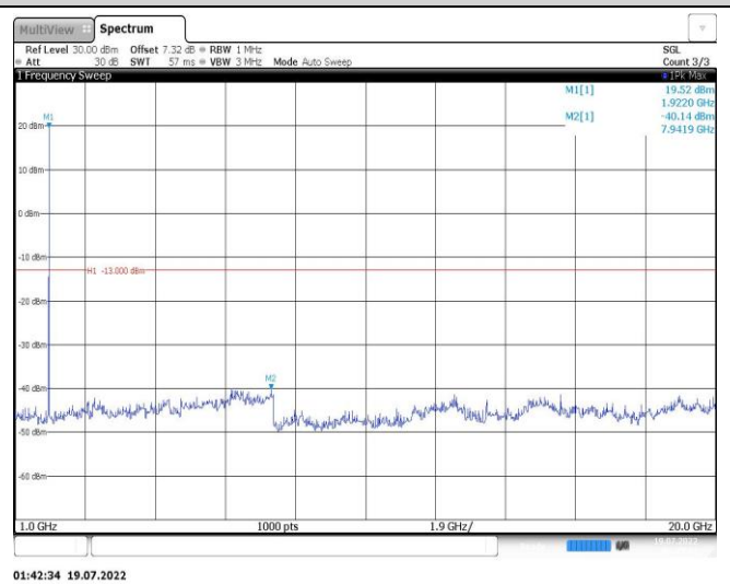
Band25-1.4MHz-16QAM-26047-1RB#0-Range2:1000~20000MHz
