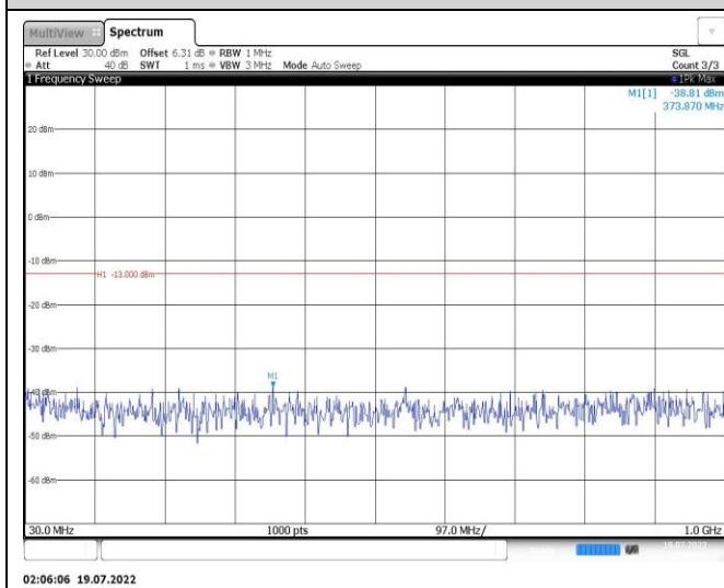
Band25-5MHz-16QAM-26065-1RB#0-Range1:30~1000MHz
