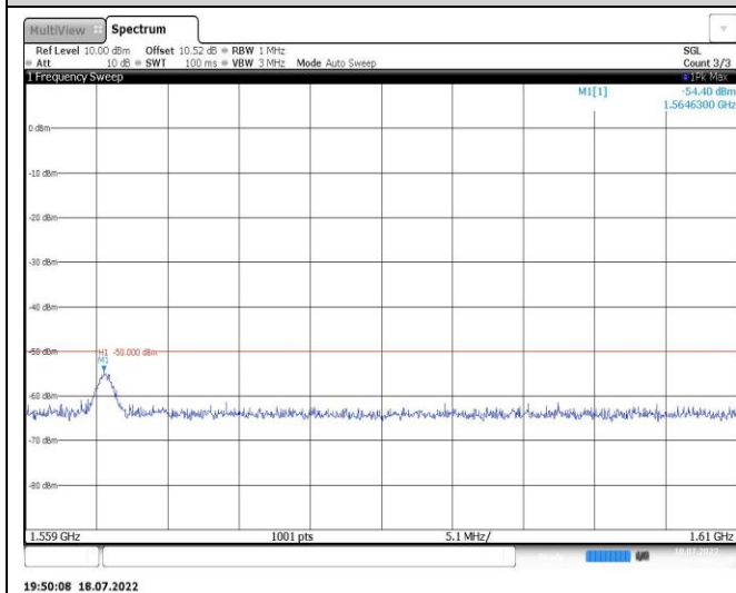
Band13-5MHz-16QAM-23205-1RB#0-Range2:1000~10000MHz
