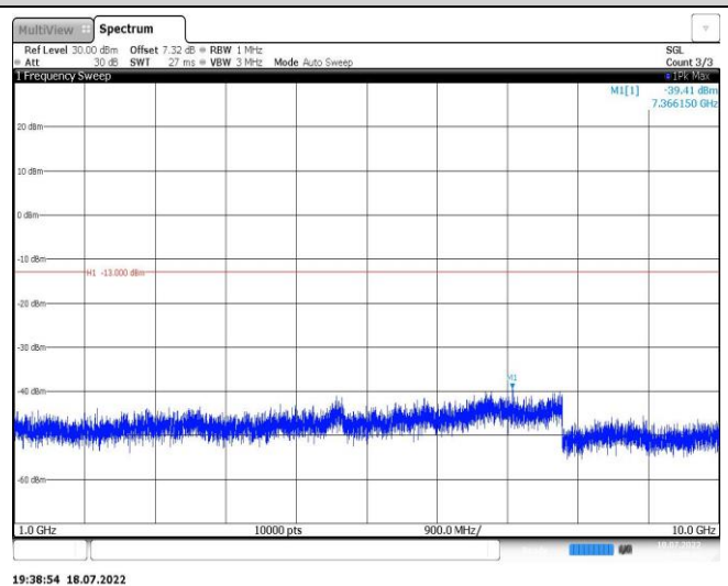
Band12-3MHz-16QAM-23165-1RB#0-Range2:1000~10000MHz
