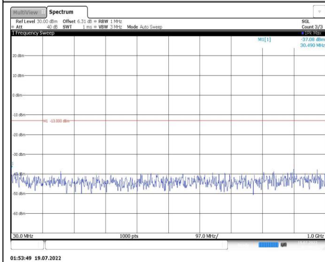
Band25-3MHz-16QAM-26675-1RB#0-Range1:30~1000MHz
