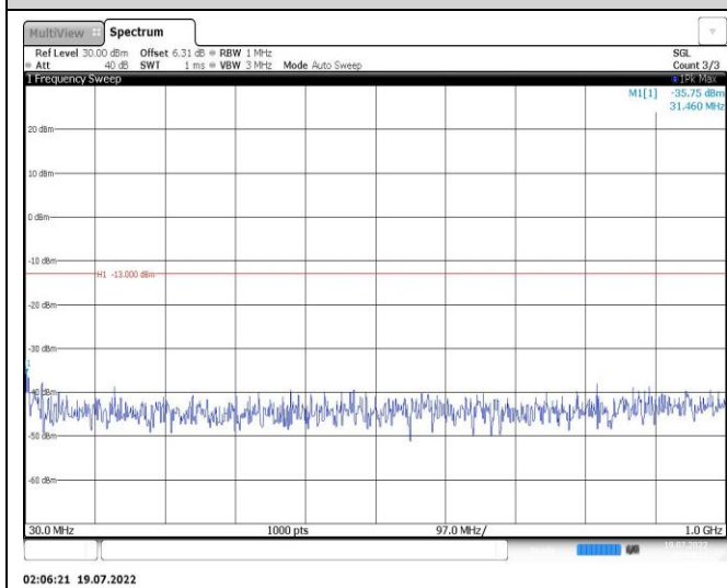
Band25-10MHz-QPSK-26090-1RB#0-Range1:30~1000MHz
