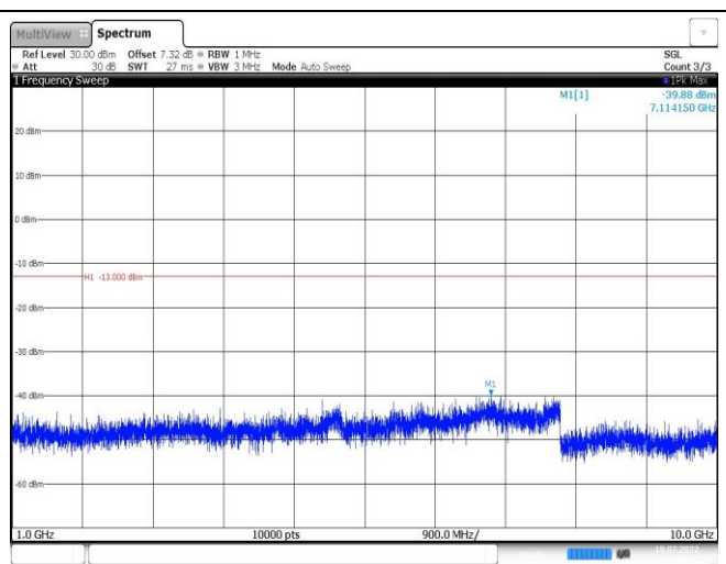
Band12-10MHz-QPSK-23095-1RB#0-Range2:1000~10000MHz
