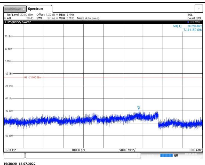
Band12-3MHz-16QAM-23095-1RB#0-Range2:1000~10000MHz
