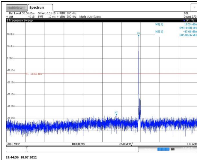
Band12-10MHz-16QAM-23095-1RB#0-Range1:30~1000MHz
