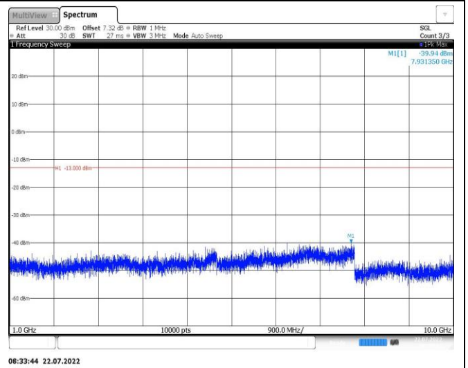
Band26-3MHz-16QAM-27025-1RB#0-Range2:1000~10000MHz
