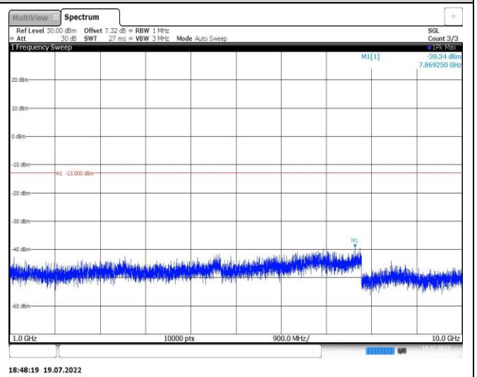
Band26-1.4MHz-16QAM-26797-1RB#0-Range2:1000~10000MHz
