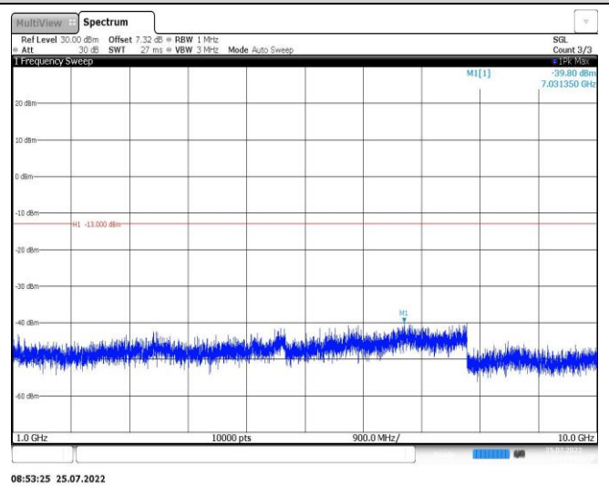
Band26-5MHz-16QAM-27015-1RB#0-Range2:1000~10000MHz
