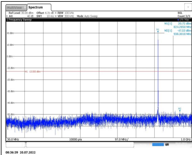
Band26-1.4MHz-16QAM-26915-1RB#0-Range1:30~1000MHz
