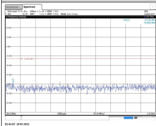
Band26-1.4MHz-QPSK-26697-1RB#0-Range1:30~1000MHz
