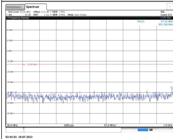
Band25-20MHz-16QAM-26140-1RB#0-Range1:30~1000MHz
