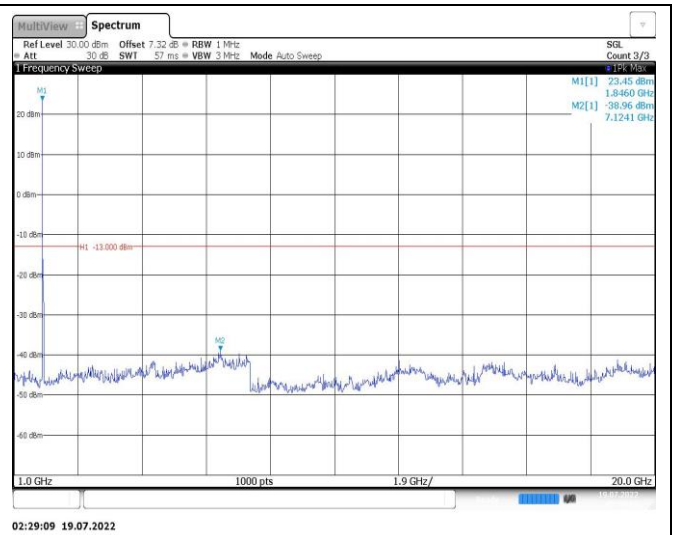
Band25-15MHz-16QAM-26365-1RB#0-Range2:1000~20000MHz
