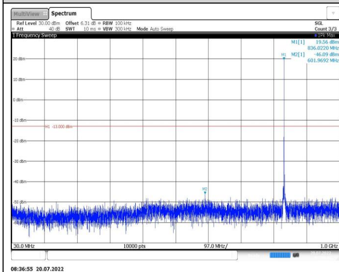
Band26-1.4MHz-QPSK-27033-1RB#0-Range1:30~1000MHz
