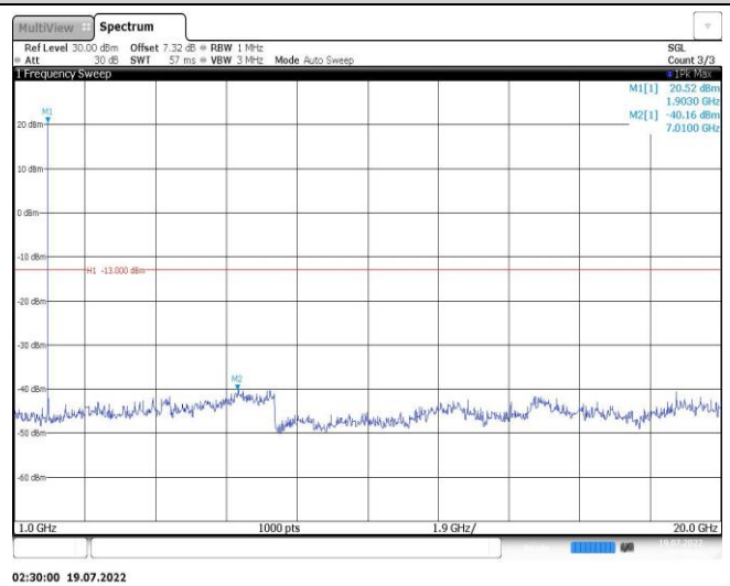
Band25-15MHz-16QAM-26115-1RB#0-Range2:1000~20000MHz
