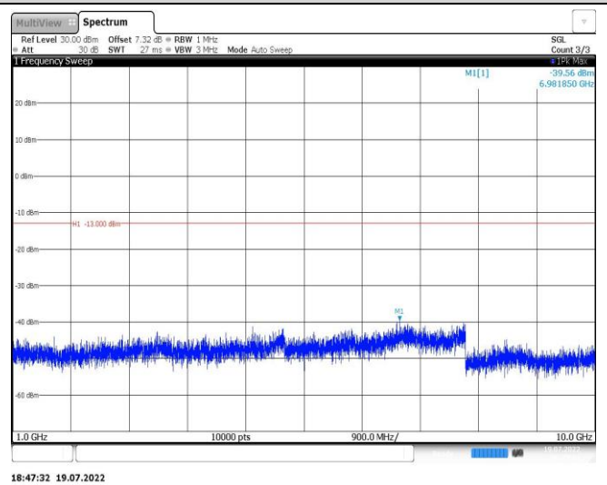
Band26-1.4MHz-QPSK-26783-1RB#0-Range2:1000~10000MHz
