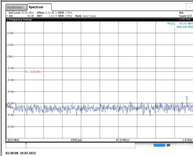
Band25-20MHz-QPSK-26140-1RB#0-Range1:30~1000MHz
