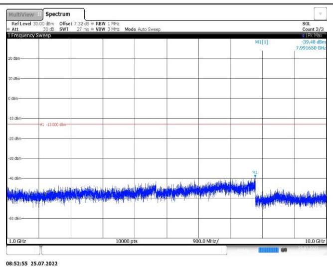
Band26-5MHz-16QAM-26915-1RB#0-Range2:1000~10000MHz
