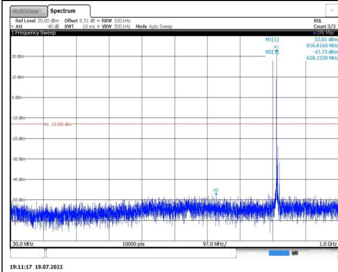
Band26-5MHz-16QAM-26765-1RB#0-Range1:30~1000MHz
