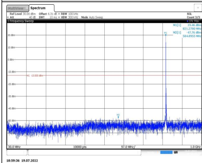
Band26-3MHz-QPSK-26805-1RB#0-Range1:30~1000MHz
