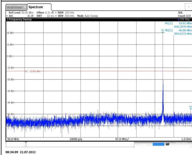
Band26-5MHz-QPSK-26715-1RB#0-Range1:30~1000MHz
