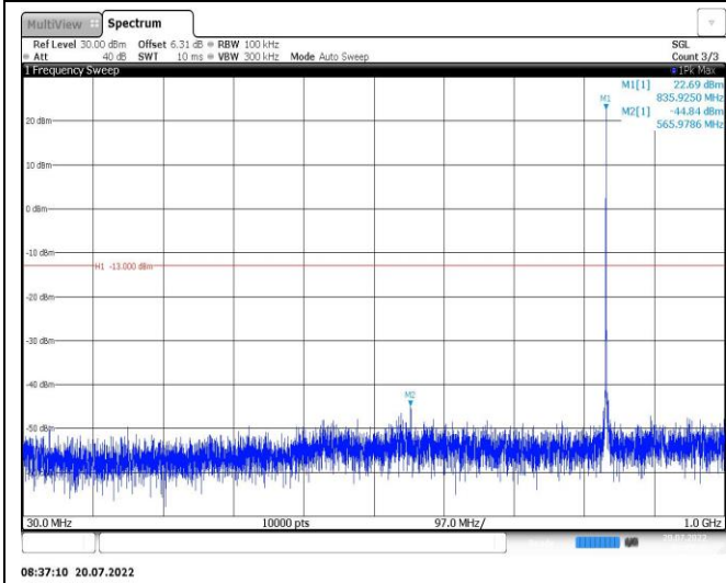
Band26-1.4MHz-16QAM-27033-1RB#0-Range1:30~1000MHz
