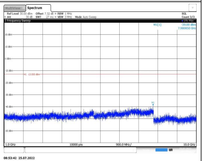
Band26-5MHz-16QAM-26715-1RB#0-Range2:1000~10000MHz
