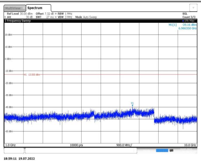
Band26-3MHz-QPSK-26775-1RB#0-Range2:1000~10000MHz
