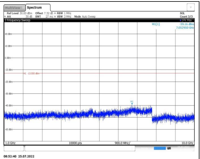
Band26-5MHz-QPSK-26915-1RB#0-Range2:1000~10000MHz
