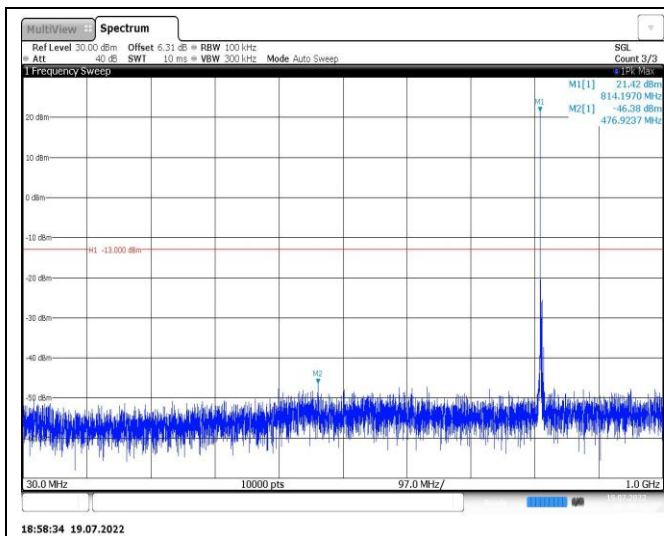
Band26-3MHz-QPSK-26740-1RB#0-Range1:30~1000MHz
