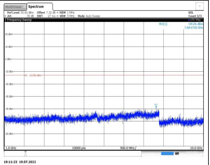
Band26-5MHz-16QAM-26765-1RB#0-Range2:1000~10000MHz
