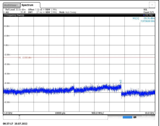
Band26-1.4MHz-16QAM-27033-1RB#0-Range2:1000~10000MHz
