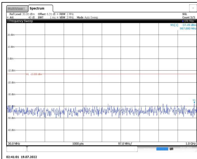
Band25-20MHz-16QAM-26365-1RB#0-Range1:30~1000MHz
