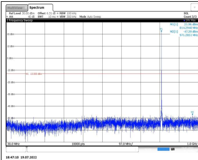
Band26-1.4MHz-16QAM-26740-1RB#0-Range1:30~1000MHz
