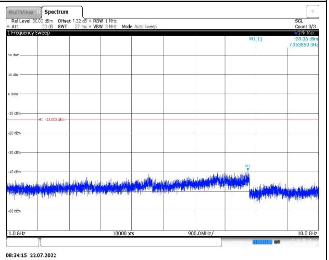
Band26-5MHz-QPSK-26715-1RB#0-Range2:1000~10000MHz
