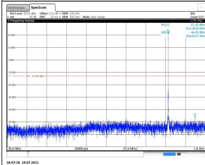
Band26-1.4MHz-QPSK-26783-1RB#0-Range1:30~1000MHz
