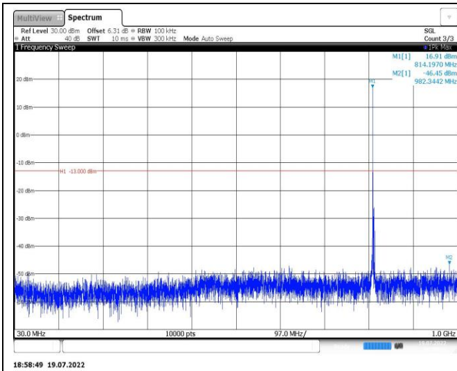
Band26-3MHz-16QAM-26740-1RB#0-Range1:30~1000MHz
