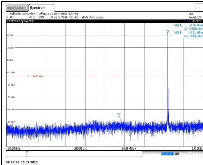
Band26-3MHz-QPSK-26915-1RB#0-Range1:30~1000MHz
