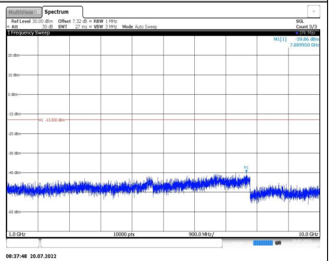
Band26-3MHz-QPSK-26705-1RB#0-Range2:1000~10000MHz
