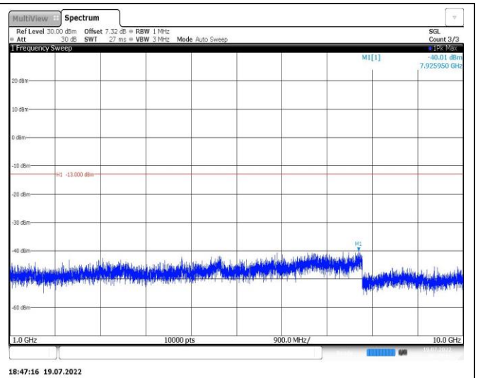
Band26-1.4MHz-16QAM-26740-1RB#0-Range2:1000~10000MHz
