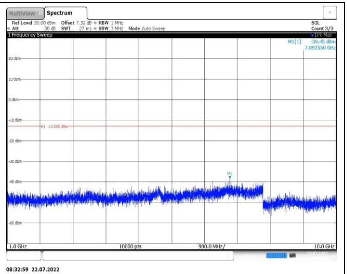
Band26-3MHz-QPSK-26915-1RB#0-Range2:1000~10000MHz
