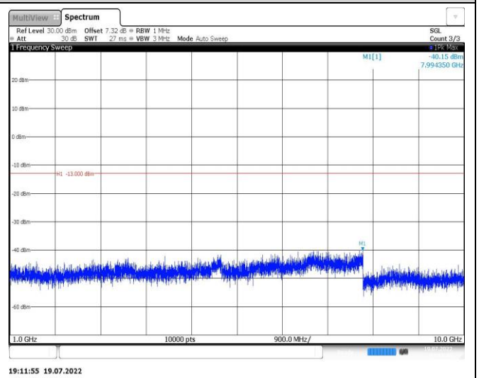
Band26-5MHz-16QAM-26815-1RB#0-Range2:1000~10000MHz
