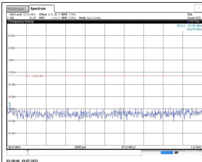
Band25-15MHz-QPSK-26365-1RB#0-Range1:30~1000MHz
