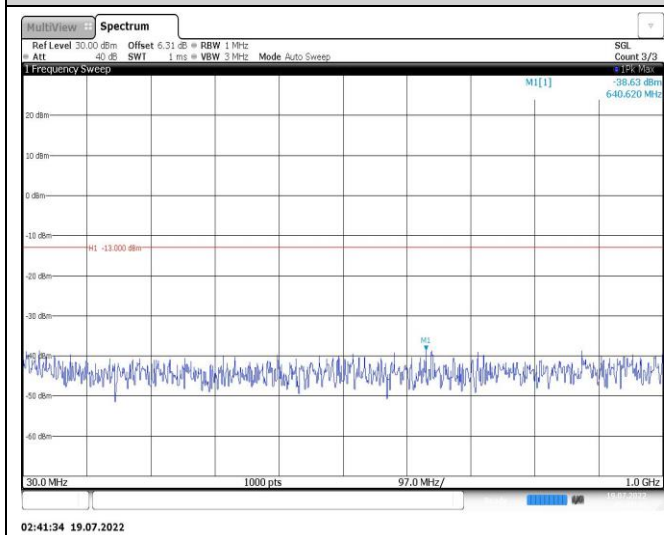
Band25-20MHz-16QAM-26590-1RB#0-Range1:30~1000MHz
