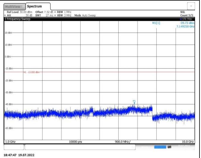
Band26-1.4MHz-16QAM-26783-1RB#0-Range2:1000~10000MHz
