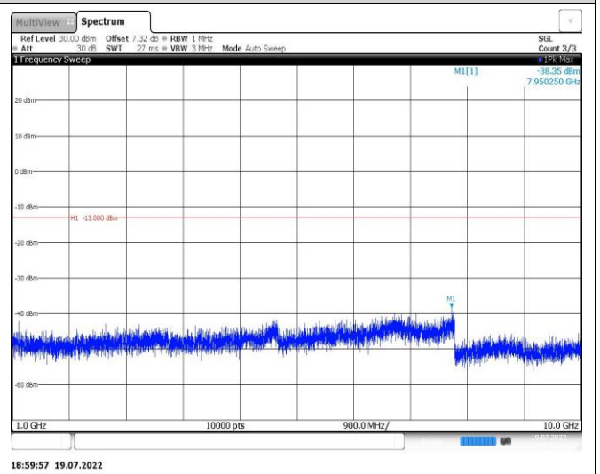
Band26-3MHz-16QAM-26805-1RB#0-Range2:1000~10000MHz
