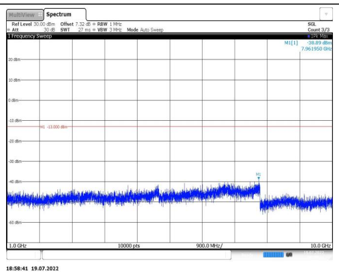
Band26-3MHz-QPSK-26740-1RB#0-Range2:1000~10000MHz
