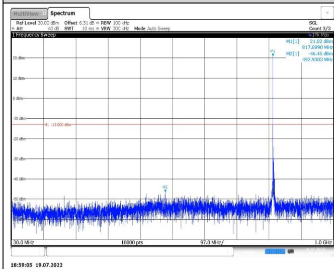
Band26-3MHz-QPSK-26775-1RB#0-Range1:30~1000MHz
