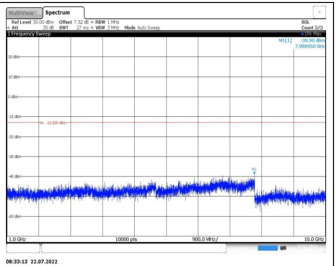
Band26-3MHz-16QAM-26915-1RB#0-Range2:1000~10000MHz
