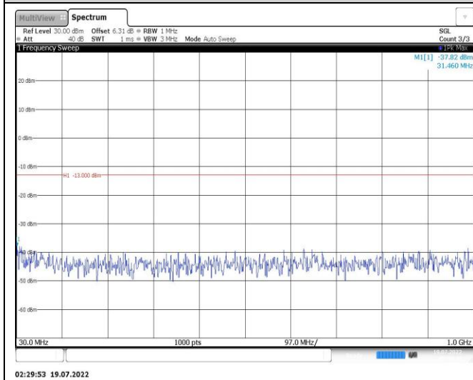
Band25-15MHz-16QAM-26115-1RB#0-Range1:30~1000MHz
