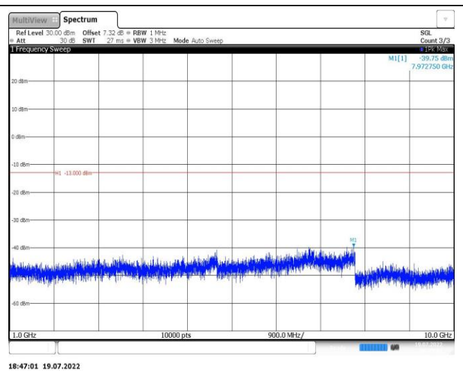
Band26-1.4MHz-QPSK-26740-1RB#0-Range2:1000~10000MHz
