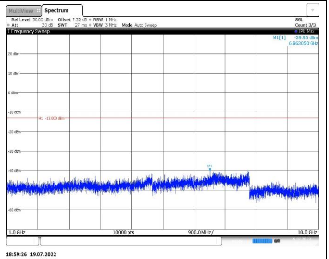
Band26-3MHz-16QAM-26775-1RB#0-Range2:1000~10000MHz
