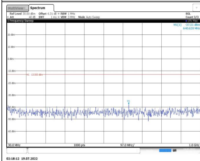
Band25-15MHz-QPSK-26115-1RB#0-Range1:30~1000MHz
