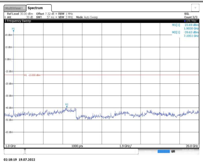
Band25-15MHz-QPSK-26115-1RB#0-Range2:1000~20000MHz
