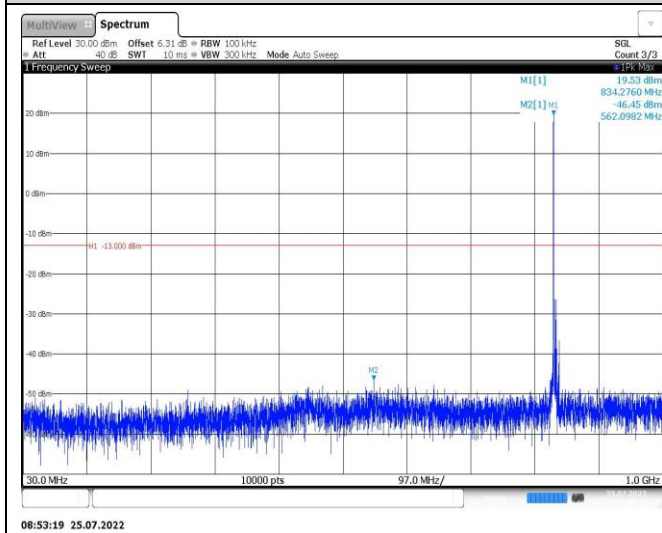
Band26-5MHz-16QAM-27015-1RB#0-Range1:30~1000MHz
