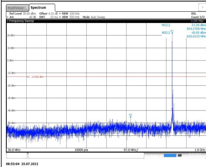
Band26-5MHz-QPSK-27015-1RB#0-Range1:30~1000MHz
