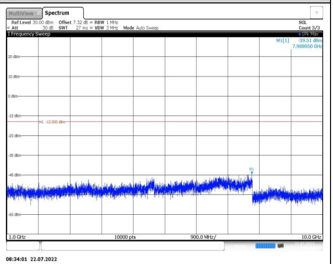
Band26-3MHz-16QAM-26705-1RB#0-Range2:1000~10000MHz
