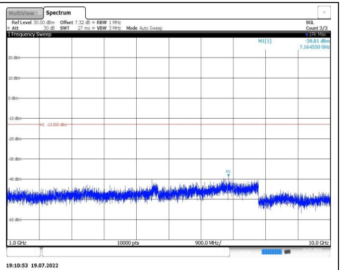
Band26-5MHz-16QAM-26740-1RB#0-Range2:1000~10000MHz
