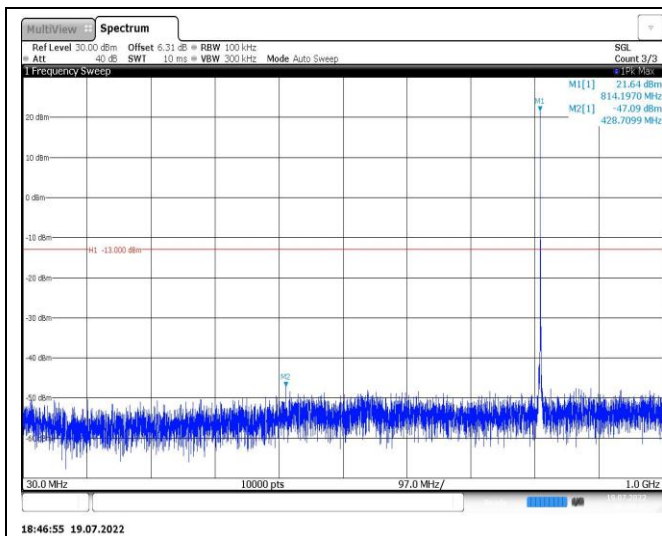
Band26-1.4MHz-QPSK-26740-1RB#0-Range1:30~1000MHz
