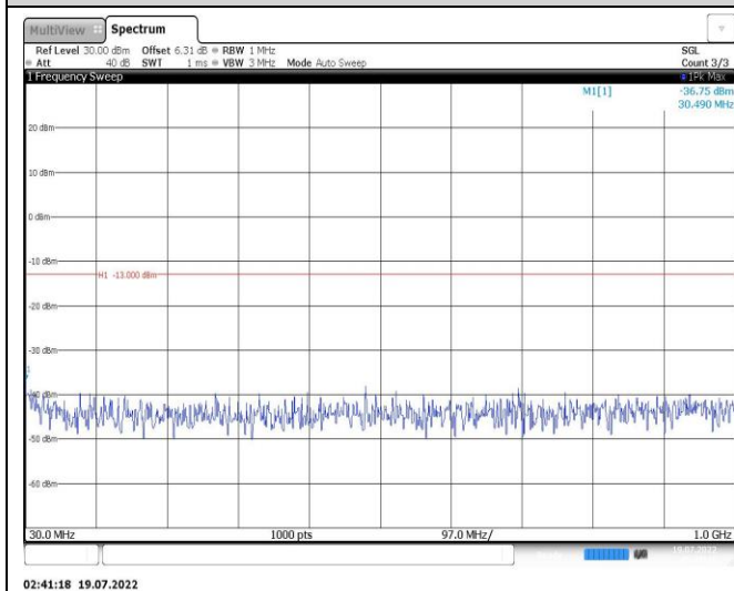
Band25-20MHz-QPSK-26590-1RB#0-Range1:30~1000MHz
