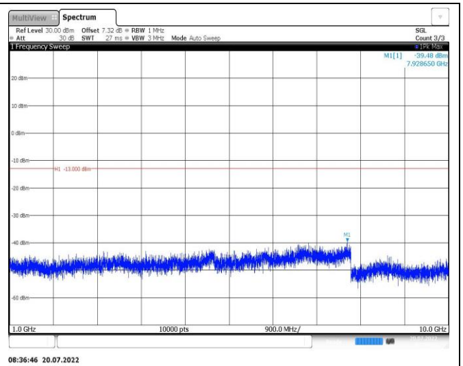
Band26-1.4MHz-16QAM-26915-1RB#0-Range2:1000~10000MHz
