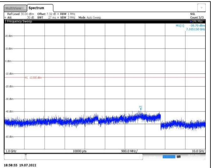
Band26-3MHz-16QAM-26740-1RB#0-Range2:1000~10000MHz
