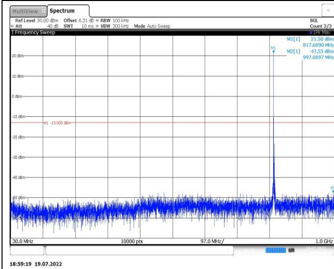
Band26-3MHz-16QAM-26775-1RB#0-Range1:30~1000MHz
