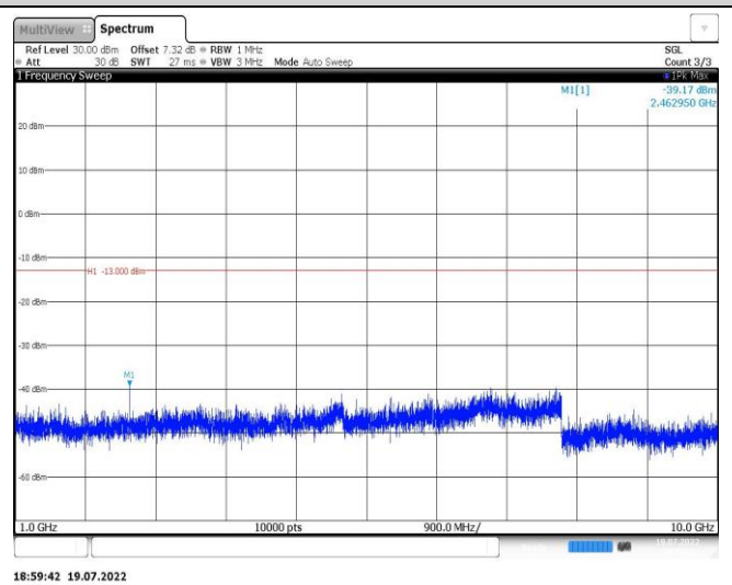
Band26-3MHz-QPSK-26805-1RB#0-Range2:1000~10000MHz
