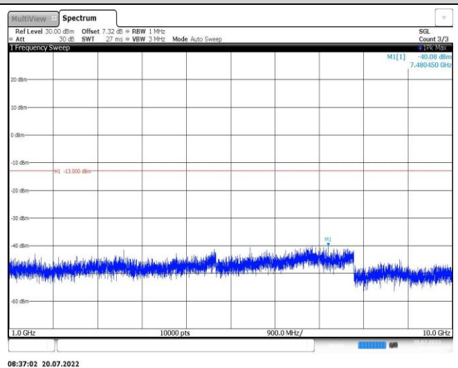
Band26-1.4MHz-QPSK-27033-1RB#0-Range2:1000~10000MHz
