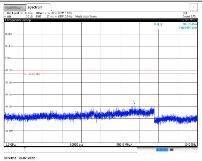
Band26-5MHz-QPSK-27015-1RB#0-Range2:1000~10000MHz
