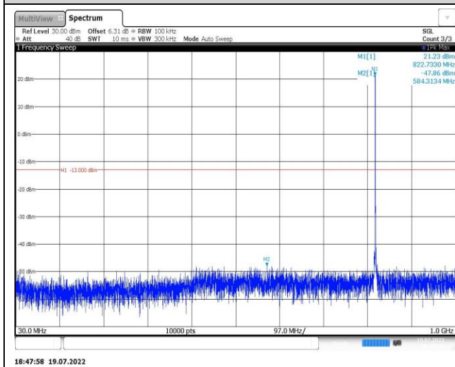
Band26-1.4MHz-QPSK-26797-1RB#0-Range1:30~1000MHz
