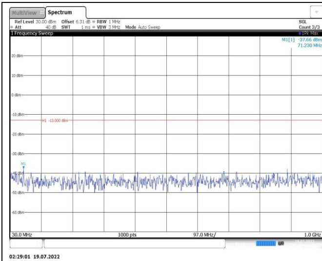
Band25-15MHz-16QAM-26365-1RB#0-Range1:30~1000MHz
