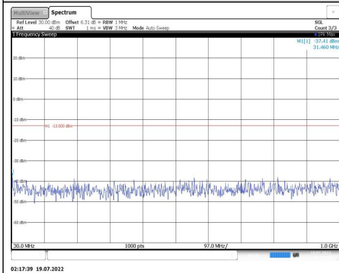
Band25-10MHz-16QAM-26640-1RB#0-Range1:30~1000MHz
