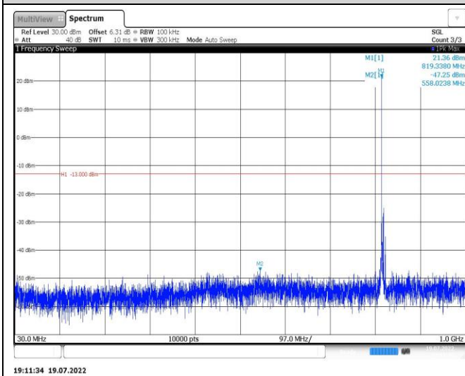
Band26-5MHz-QPSK-26815-1RB#0-Range1:30~1000MHz
