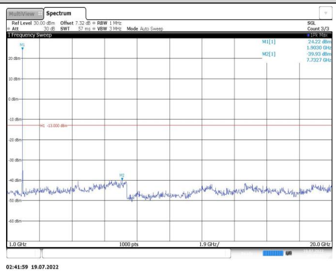
Band25-20MHz-16QAM-26140-1RB#0-Range2:1000~20000MHz
