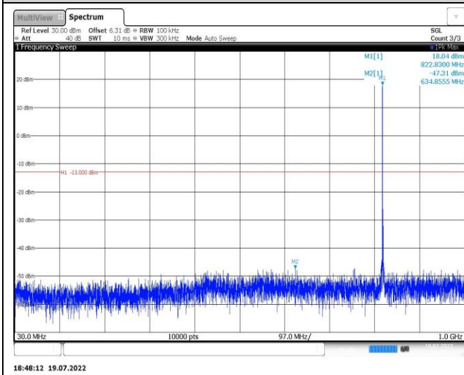
Band26-1.4MHz-16QAM-26797-1RB#0-Range1:30~1000MHz
