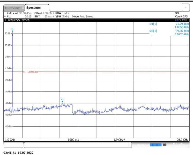
Band25-20MHz-16QAM-26590-1RB#0-Range2:1000~20000MHz
