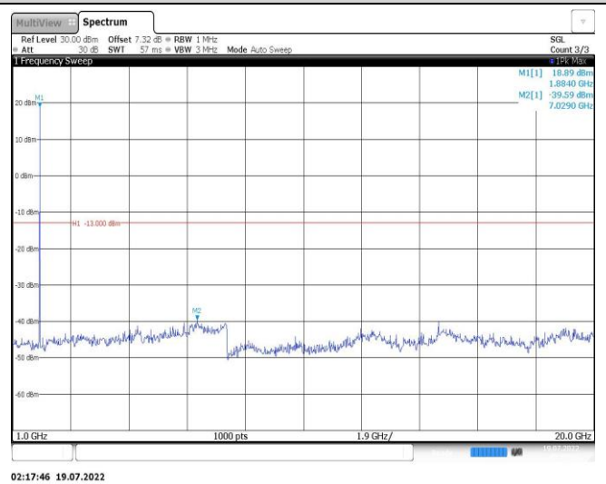
Band25-10MHz-16QAM-26640-1RB#0-Range2:1000~20000MHz
