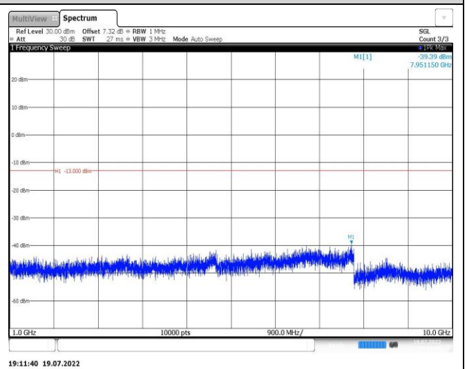
Band26-5MHz-QPSK-26815-1RB#0-Range2:1000~10000MHz
