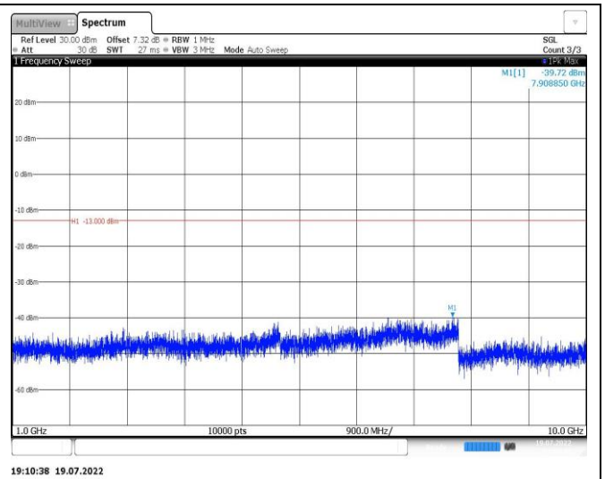
Band26-5MHz-QPSK-26740-1RB#0-Range2:1000~10000MHz
