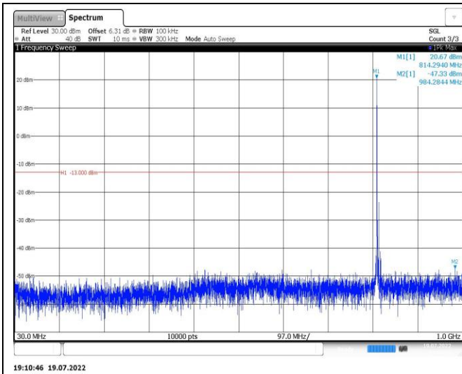
Band26-5MHz-16QAM-26740-1RB#0-Range1:30~1000MHz
