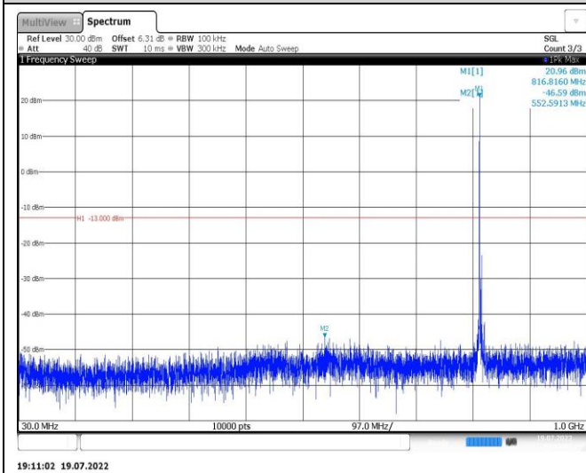
Band26-5MHz-QPSK-26765-1RB#0-Range1:30~1000MHz
