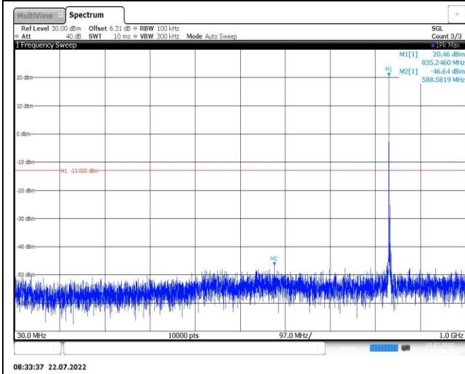
Band26-3MHz-16QAM-27025-1RB#0-Range1:30~1000MHz
