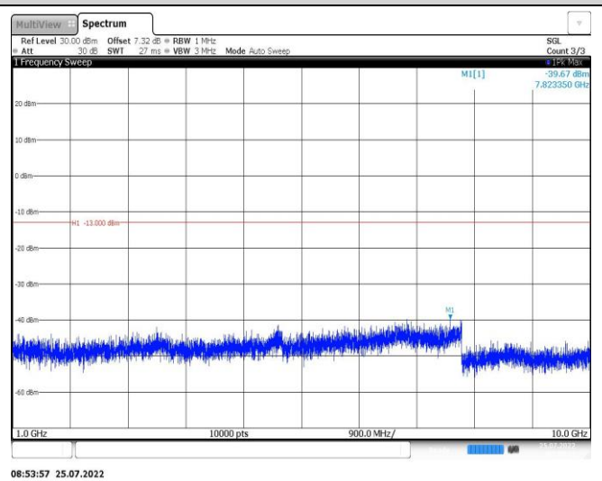
Band26-10MHz-QPSK-26740-1RB#0-Range2:1000~10000MHz
