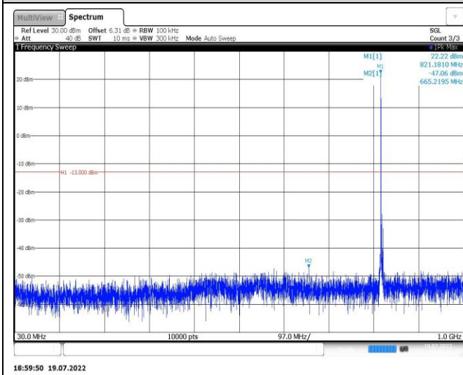
Band26-3MHz-16QAM-26805-1RB#0-Range1:30~1000MHz
