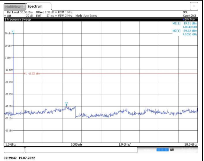
Band25-15MHz-16QAM-26615-1RB#0-Range2:1000~20000MHz
