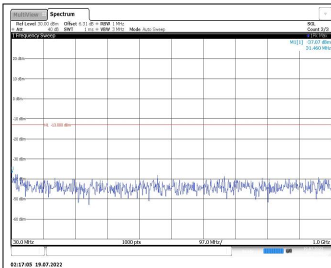
Band25-10MHz-16QAM-26365-1RB#0-Range1:30~1000MHz
