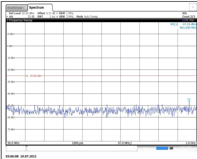
Band38-10MHz-16QAM-38200-1RB#0-Range1:30~1000MHz
