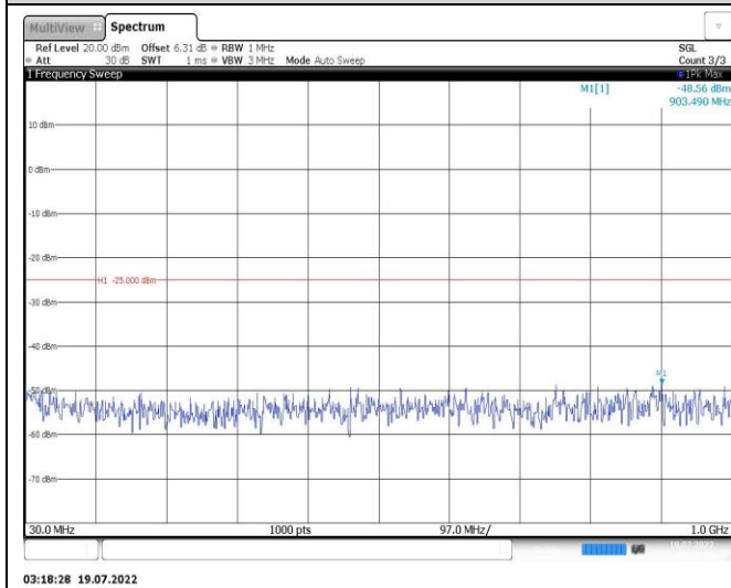
Band38-15MHz-16QAM-37825-1RB#0-Range1:30~1000MHz
