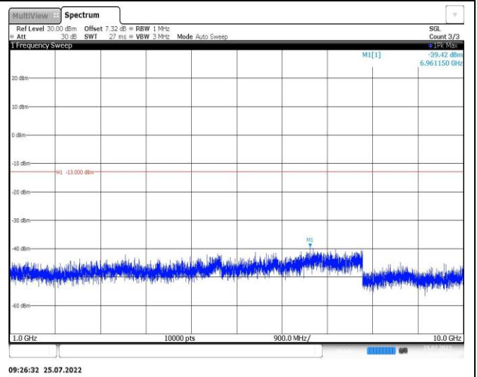
Band26-15MHz-16QAM-26865-1RB#0-Range2:1000~10000MHz
