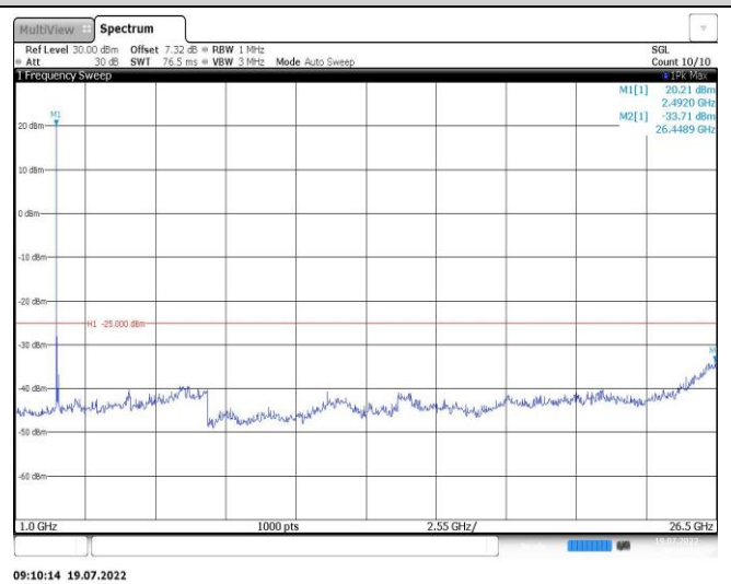
Band41-15MHz-QPSK-40620-1RB#0-Range2:1000~26500MHz
