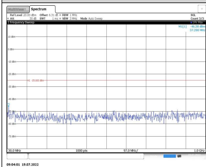
Band41-5MHz-16QAM-40620-1RB#0-Range1:30~1000MHz
