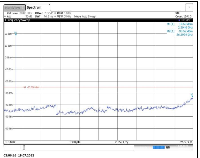
Band38-10MHz-16QAM-38200-1RB#0-Range2:1000~26500MHz
