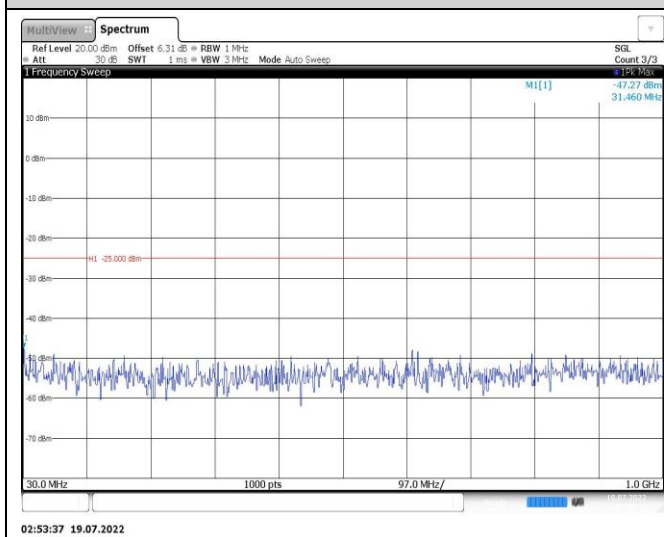
Band38-5MHz-16QAM-38000-1RB#0-Range1:30~1000MHz
