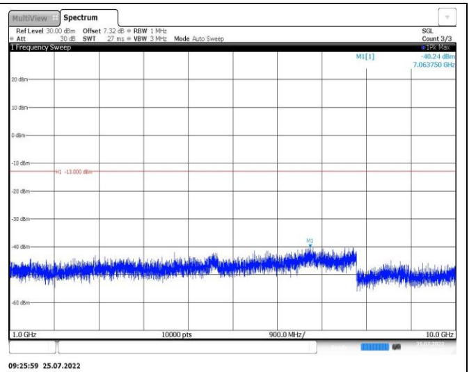
Band26-15MHz-QPSK-26965-1RB#0-Range2:1000~10000MHz
