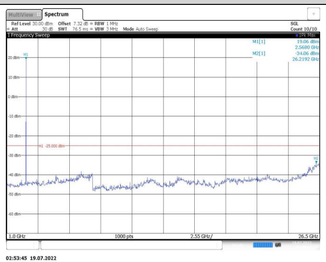
Band38-5MHz-16QAM-38000-1RB#0-Range2:1000~26500MHz
