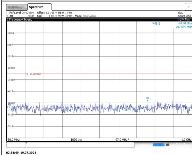
Band38-10MHz-QPSK-37800-1RB#0-Range1:30~1000MHz
