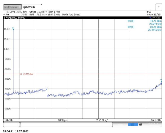
Band41-5MHz-16QAM-41565-1RB#0-Range2:1000~26500MHz
