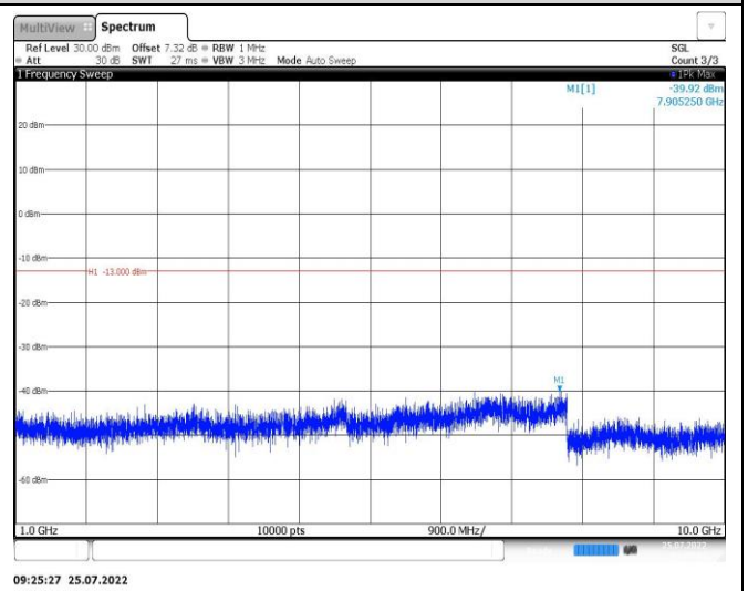
Band26-15MHz-QPSK-26915-1RB#0-Range2:1000~10000MHz
