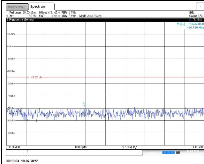
Band41-10MHz-16QAM-39700-1RB#0-Range1:30~1000MHz
