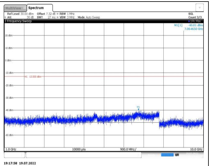
Band26-10MHz-QPSK-26840-1RB#0-Range2:1000~10000MHz
