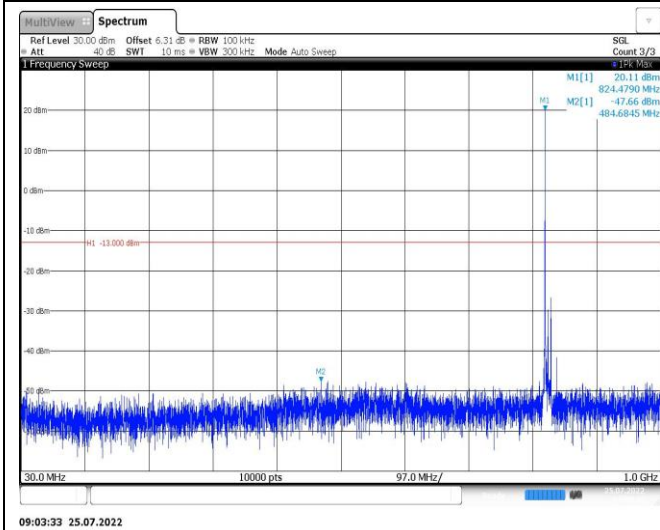
Band26-10MHz-QPSK-26915-1RB#0-Range1:30~1000MHz
