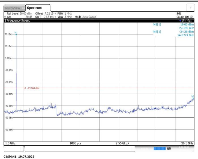
Band38-5MHz-16QAM-37775-1RB#0-Range2:1000~26500MHz
