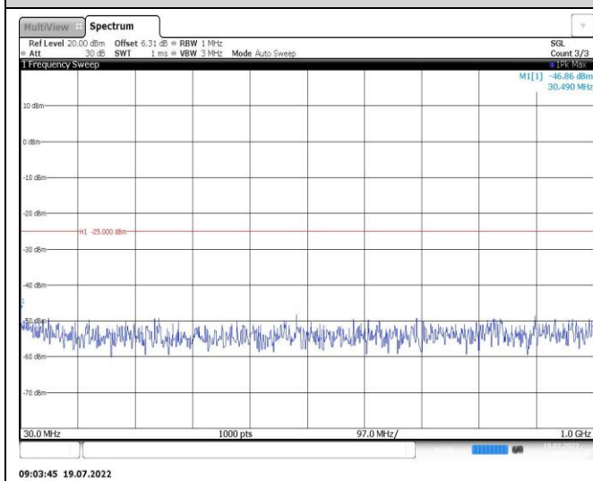
Band41-5MHz-QPSK-40620-1RB#0-Range1:30~1000MHz
