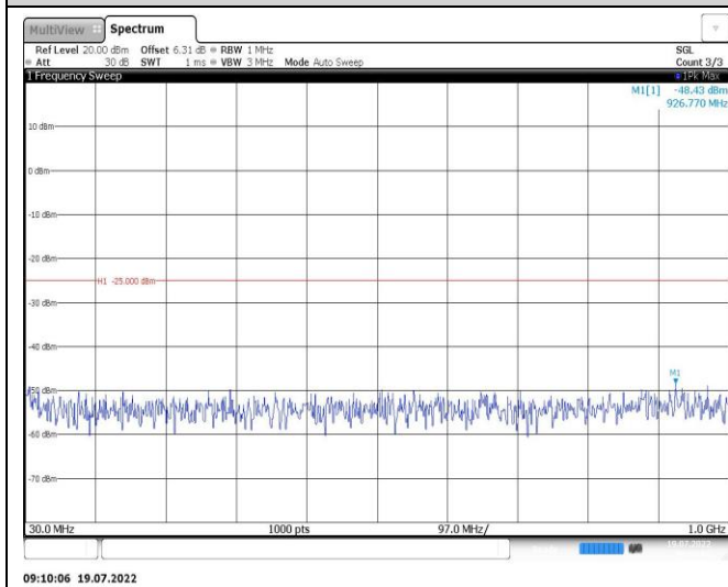
Band41-15MHz-QPSK-40620-1RB#0-Range1:30~1000MHz
