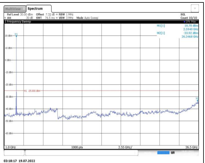
Band38-15MHz-16QAM-38175-1RB#0-Range2:1000~26500MHz
