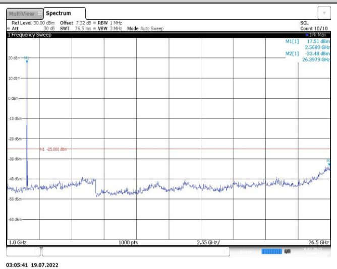
Band38-10MHz-16QAM-38000-1RB#0-Range2:1000~26500MHz
