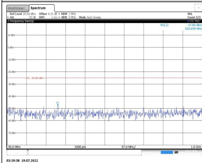
Band38-20MHz-16QAM-38000-1RB#0-Range1:30~1000MHz
