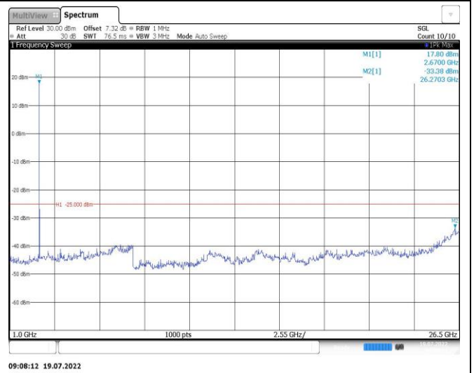
Band41-10MHz-16QAM-39700-1RB#0-Range2:1000~26500MHz
