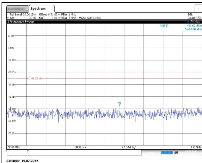
Band38-15MHz-16QAM-38175-1RB#0-Range1:30~1000MHz
