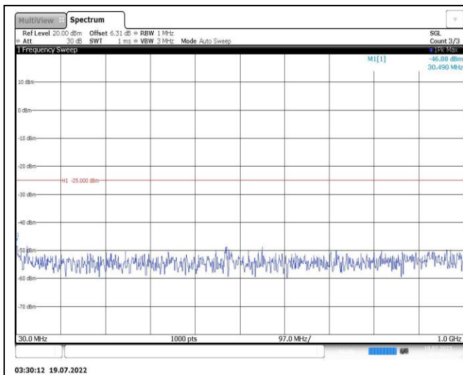
Band38-20MHz-16QAM-38150-1RB#0-Range1:30~1000MHz
