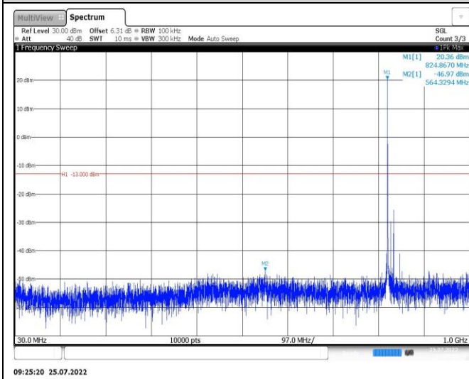
Band26-15MHz-QPSK-26915-1RB#0-Range1:30~1000MHz
