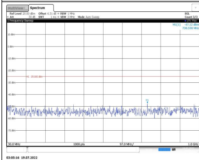
Band38-10MHz-QPSK-38000-1RB#0-Range1:30~1000MHz
