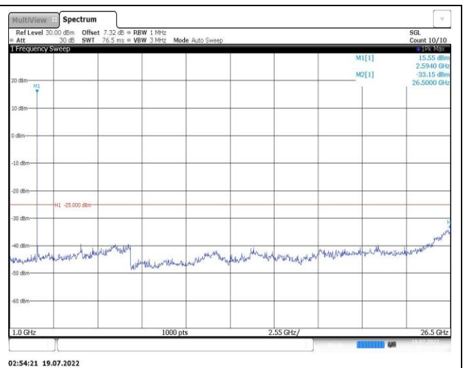
Band38-5MHz-16QAM-38225-1RB#0-Range2:1000~26500MHz
