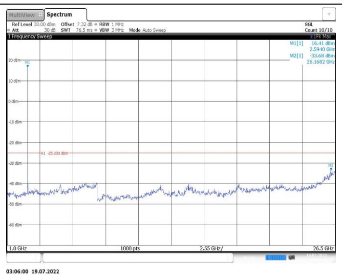
Band38-10MHz-QPSK-38200-1RB#0-Range2:1000~26500MHz
