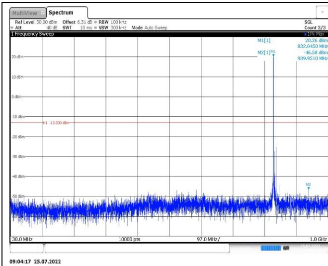
Band26-10MHz-16QAM-26990-1RB#0-Range1:30~1000MHz
