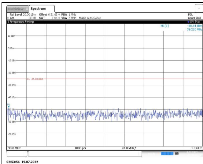
Band38-5MHz-QPSK-38225-1RB#0-Range1:30~1000MHz
