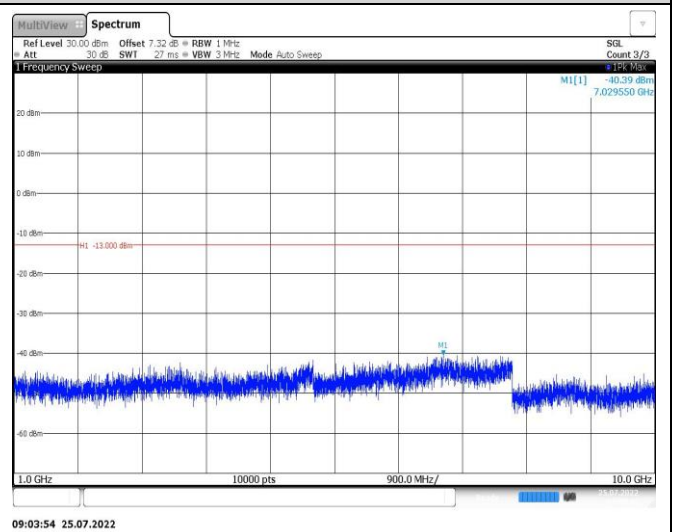
Band26-10MHz-16QAM-26915-1RB#0-Range2:1000~10000MHz
