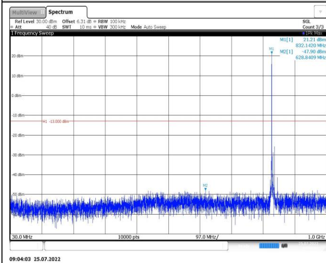
Band26-10MHz-QPSK-26990-1RB#0-Range1:30~1000MHz
