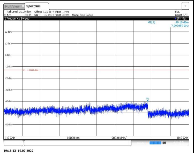
Band26-10MHz-16QAM-26840-1RB#0-Range2:1000~10000MHz
