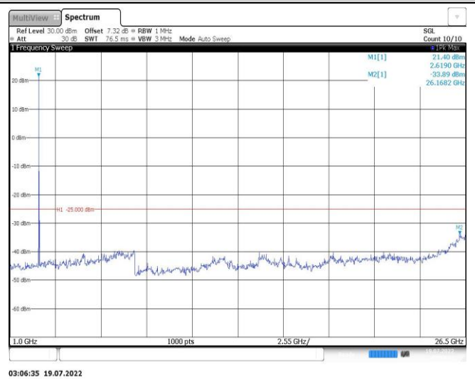
Band38-10MHz-16QAM-37800-1RB#0-Range2:1000~26500MHz
