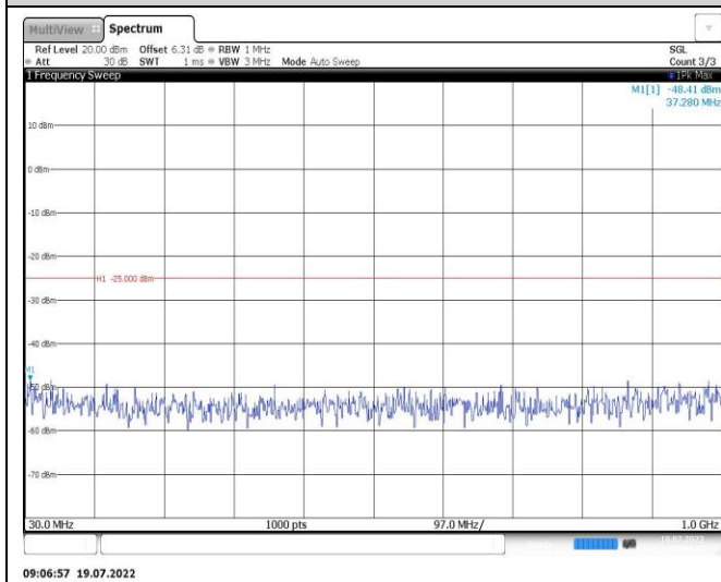
Band41-10MHz-QPSK-40620-1RB#0-Range1:30~1000MHz
