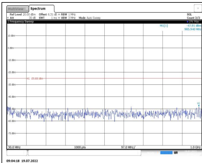
Band41-5MHz-QPSK-41565-1RB#0-Range1:30~1000MHz
