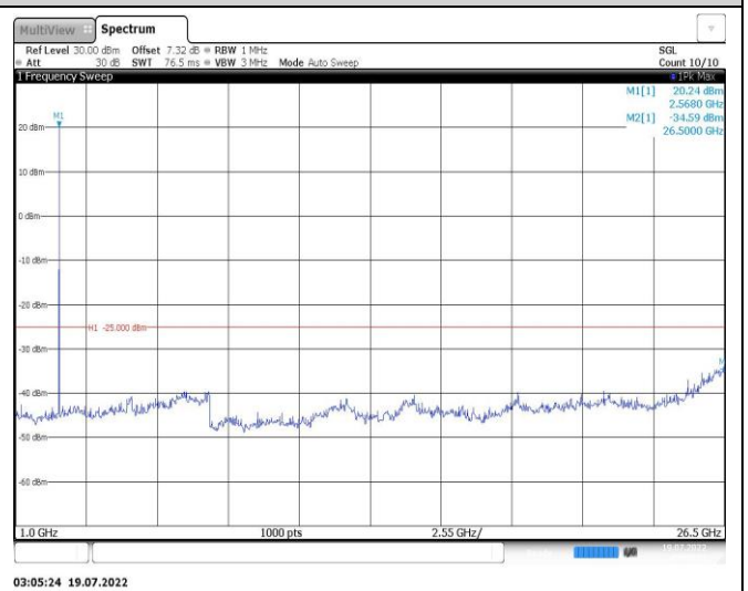
Band38-10MHz-QPSK-38000-1RB#0-Range2:1000~26500MHz
