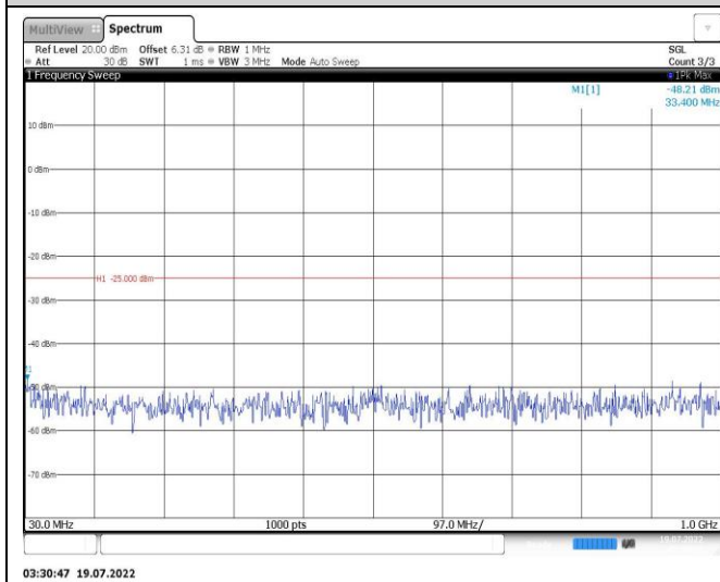
Band41-5MHz-QPSK-39675-1RB#0-Range1:30~1000MHz
