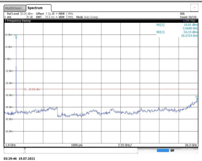
Band38-20MHz-16QAM-38000-1RB#0-Range2:1000~26500MHz
