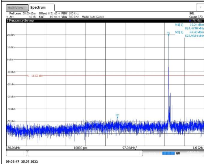
Band26-10MHz-16QAM-26915-1RB#0-Range1:30~1000MHz
