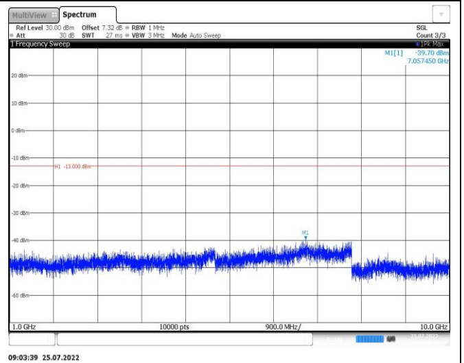
Band26-10MHz-QPSK-26915-1RB#0-Range2:1000~10000MHz
