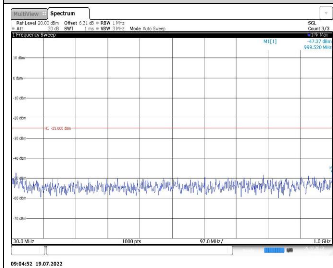
Band41-5MHz-16QAM-39675-1RB#0-Range1:30~1000MHz
