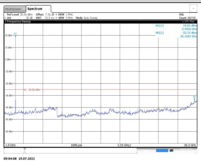
Band41-5MHz-16QAM-40620-1RB#0-Range2:1000~26500MHz
