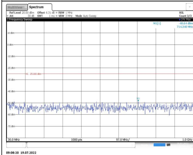
Band41-15MHz-QPSK-39725-1RB#0-Range1:30~1000MHz
