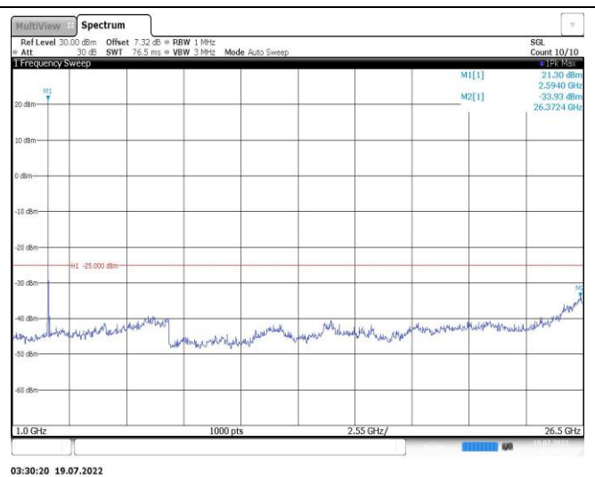
Band38-20MHz-16QAM-38150-1RB#0-Range2:1000~26500MHz
