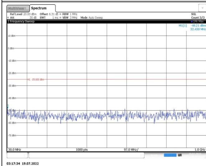
Band38-15MHz-16QAM-38000-1RB#0-Range1:30~1000MHz
