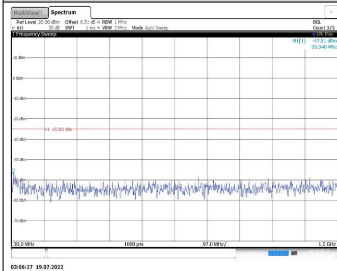
Band38-10MHz-16QAM-37800-1RB#0-Range1:30~1000MHz
