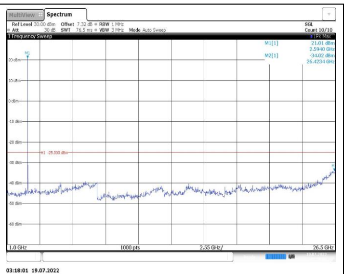
Band38-15MHz-QPSK-38175-1RB#0-Range2:1000~26500MHz
