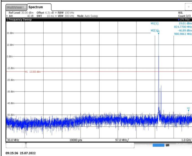
Band26-15MHz-16QAM-26915-1RB#0-Range1:30~1000MHz
