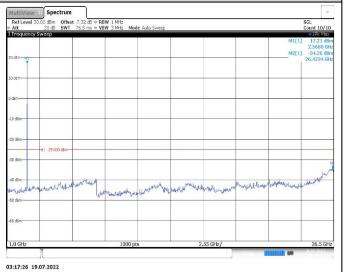
Band38-15MHz-QPSK-38000-1RB#0-Range2:1000~26500MHz
