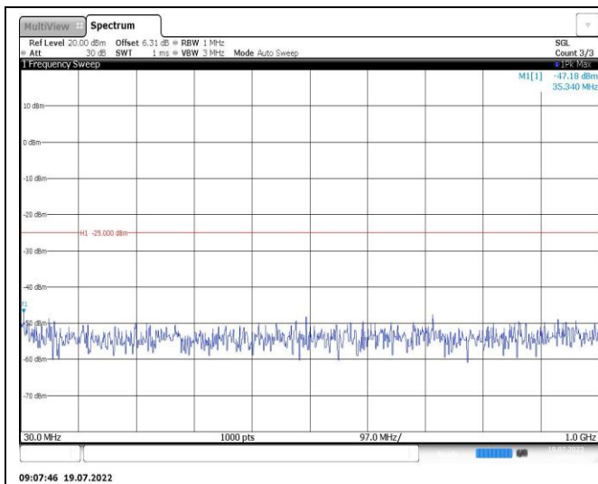
Band41-10MHz-16QAM-41540-1RB#0-Range1:30~1000MHz
