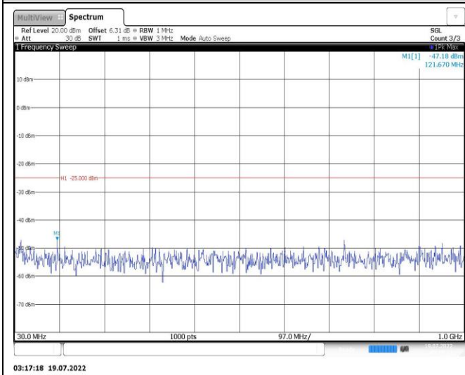
Band38-15MHz-QPSK-38000-1RB#0-Range1:30~1000MHz
