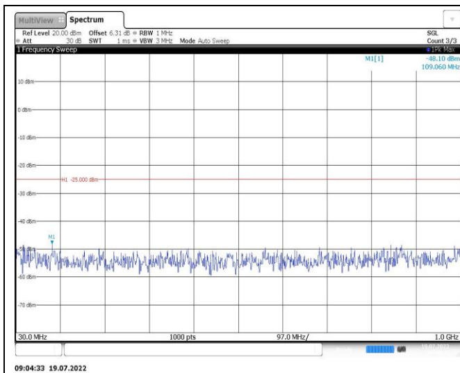
Band41-5MHz-16QAM-41565-1RB#0-Range1:30~1000MHz
