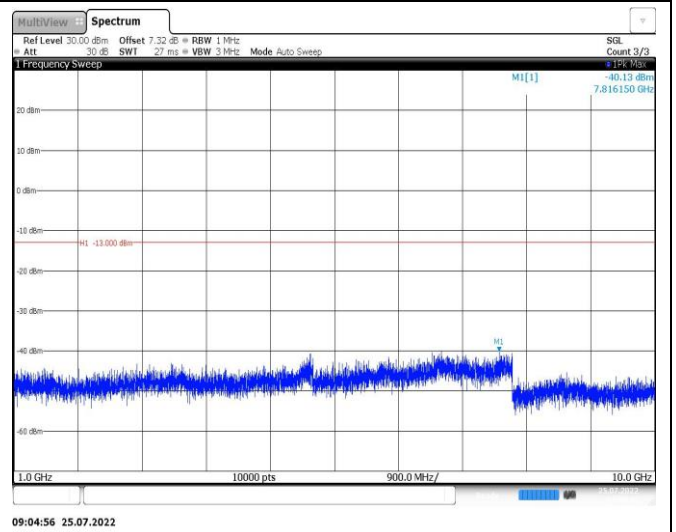
Band26-15MHz-QPSK-26865-1RB#0-Range2:1000~10000MHz
