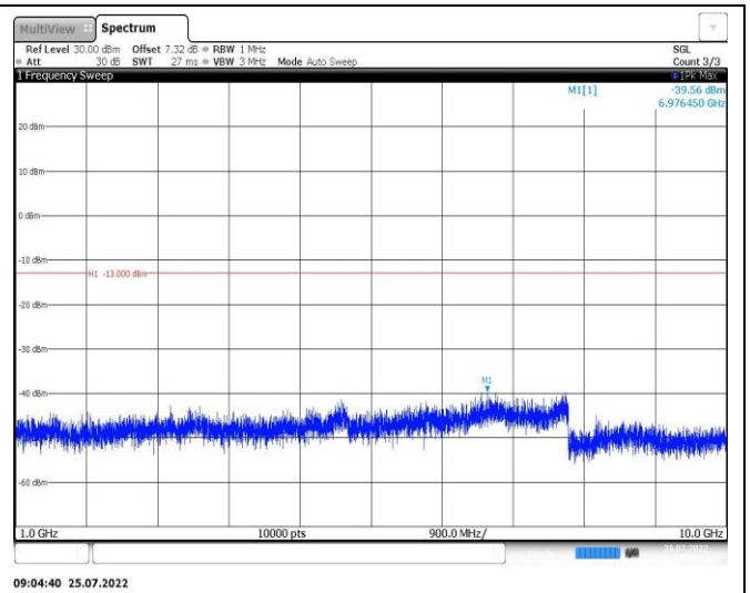
Band26-10MHz-16QAM-26740-1RB#0-Range2:1000~10000MHz
