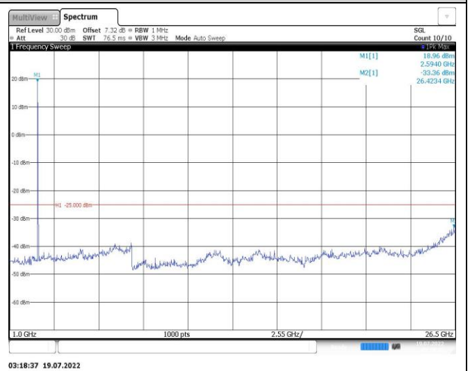
Band38-15MHz-16QAM-37825-1RB#0-Range2:1000~26500MHz
