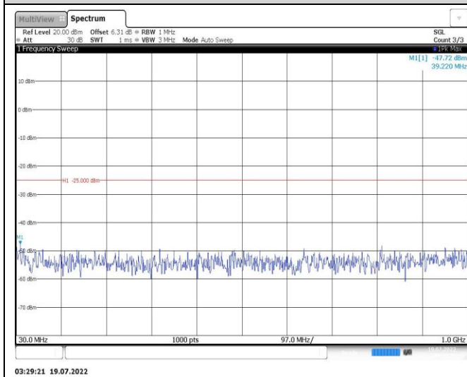
Band38-20MHz-QPSK-38000-1RB#0-Range1:30~1000MHz
