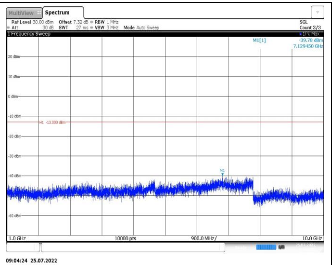
Band26-10MHz-16QAM-26990-1RB#0-Range2:1000~10000MHz
