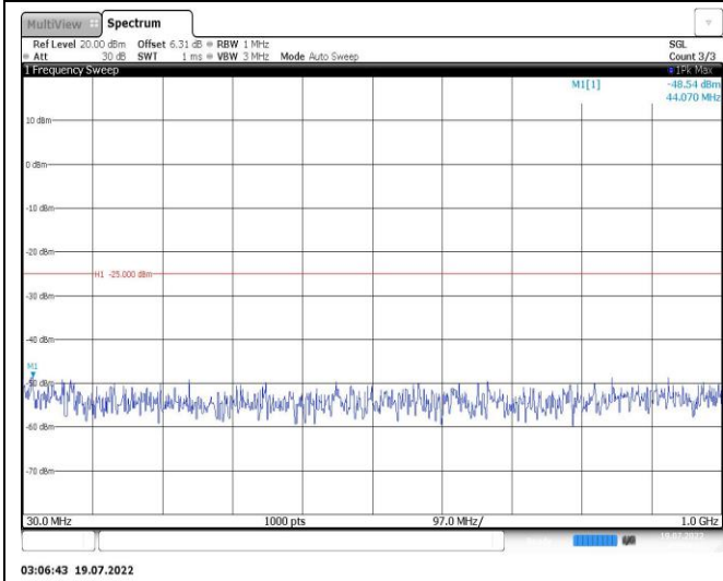
Band38-15MHz-QPSK-37825-1RB#0-Range1:30~1000MHz
