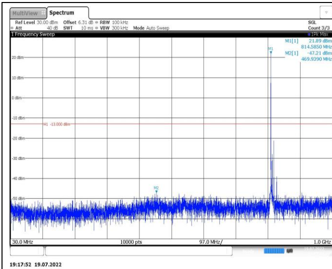
Band26-10MHz-QPSK-26840-1RB#0-Range1:30~1000MHz
