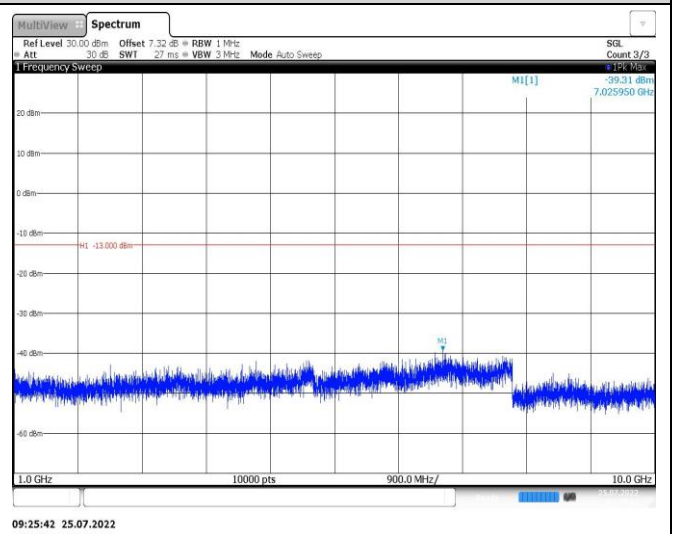
Band26-15MHz-16QAM-26915-1RB#0-Range2:1000~10000MHz
