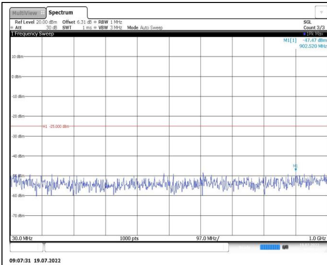
Band41-10MHz-QPSK-41540-1RB#0-Range1:30~1000MHz
