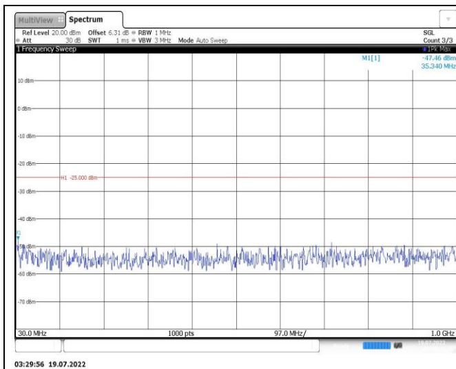
Band38-20MHz-QPSK-38150-1RB#0-Range1:30~1000MHz
