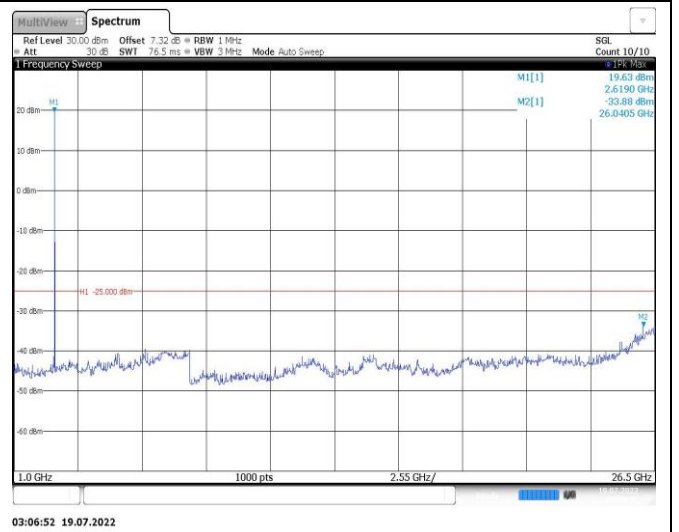
Band38-15MHz-QPSK-37825-1RB#0-Range2:1000~26500MHz
