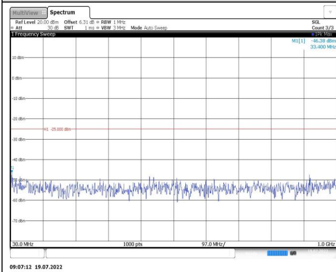
Band41-10MHz-16QAM-40620-1RB#0-Range1:30~1000MHz
