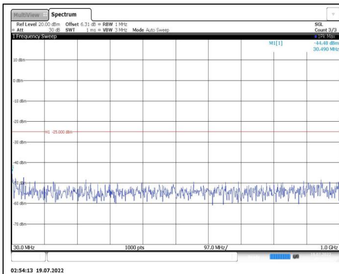
Band38-5MHz-16QAM-38225-1RB#0-Range1:30~1000MHz
