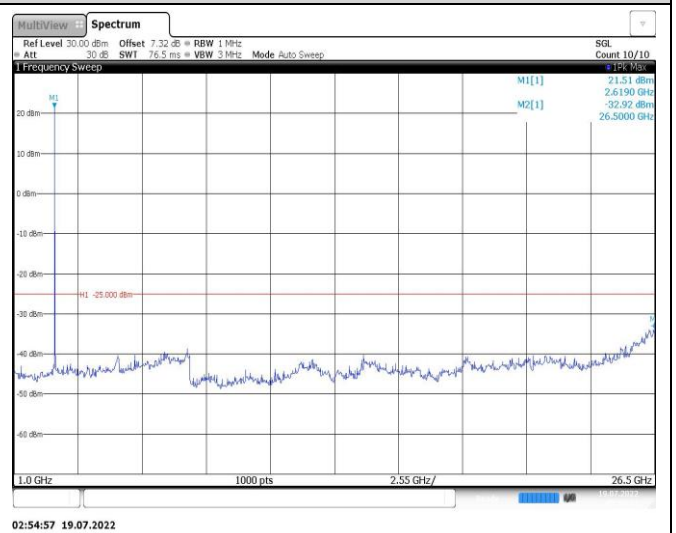
Band38-10MHz-QPSK-37800-1RB#0-Range2:1000~26500MHz
