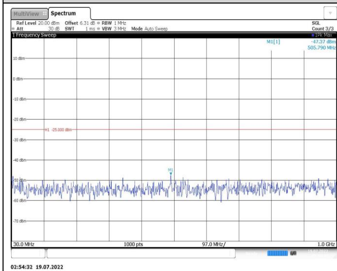
Band38-5MHz-16QAM-37775-1RB#0-Range1:30~1000MHz
