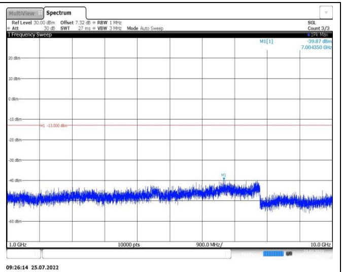
Band26-15MHz-16QAM-26965-1RB#0-Range2:1000~10000MHz
