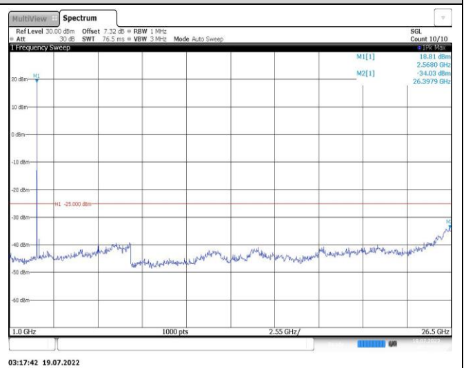
Band38-15MHz-16QAM-38000-1RB#0-Range2:1000~26500MHz
