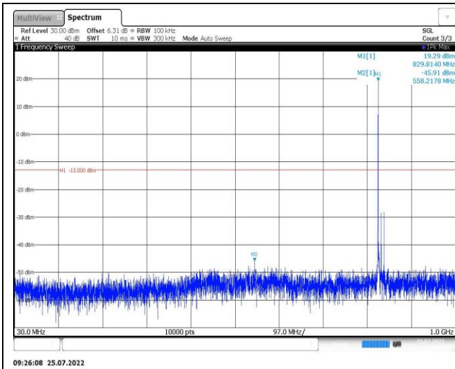
Band26-15MHz-16QAM-26965-1RB#0-Range1:30~1000MHz
