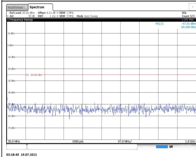
Band38-20MHz-QPSK-37850-1RB#0-Range1:30~1000MHz
