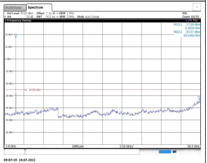
Band41-10MHz-16QAM-40620-1RB#0-Range2:1000~26500MHz
