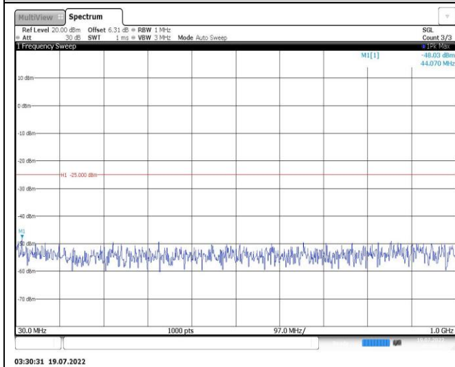
Band38-20MHz-16QAM-37850-1RB#0-Range1:30~1000MHz
