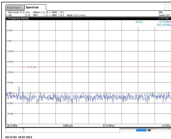
Band38-15MHz-QPSK-38175-1RB#0-Range1:30~1000MHz
