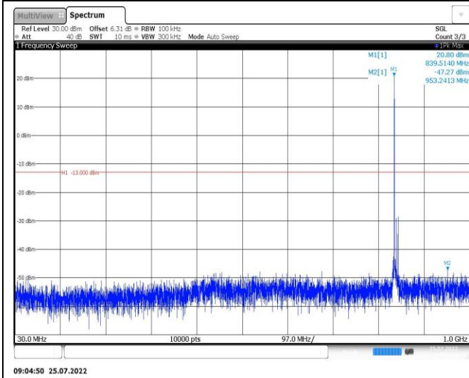
Band26-15MHz-QPSK-26865-1RB#0-Range1:30~1000MHz
