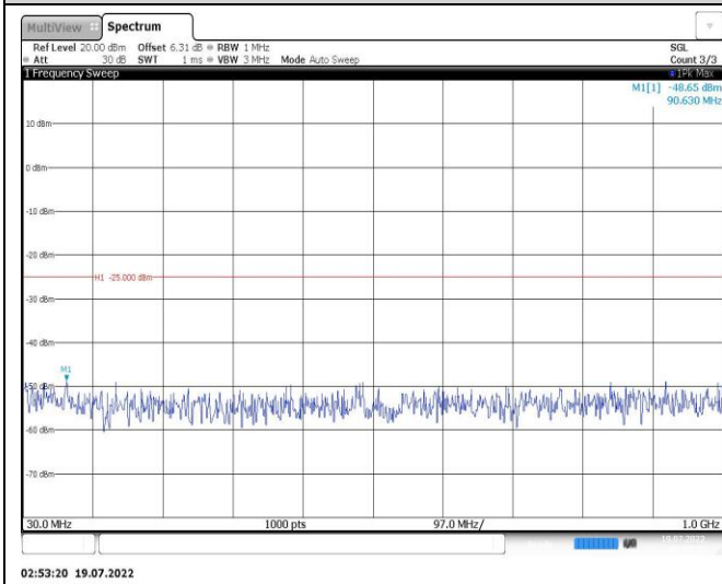
Band38-5MHz-QPSK-38000-1RB#0-Range1:30~1000MHz
