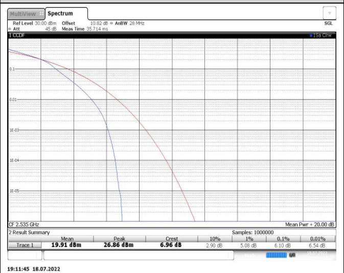
Band7-10MHz-16QAM-21100-50RB#0
