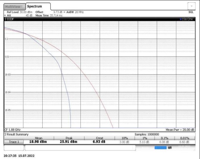
Band2-3MHz-16QAM-18900-15RB#0
