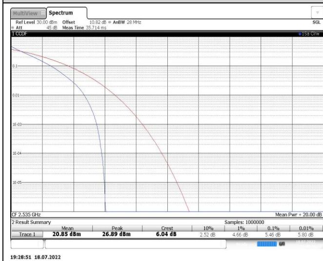
Band7-20MHz-QPSK-21100-100RB#0
