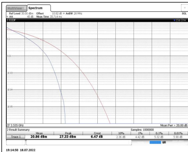
Band7-15MHz-QPSK-21100-75RB#0
