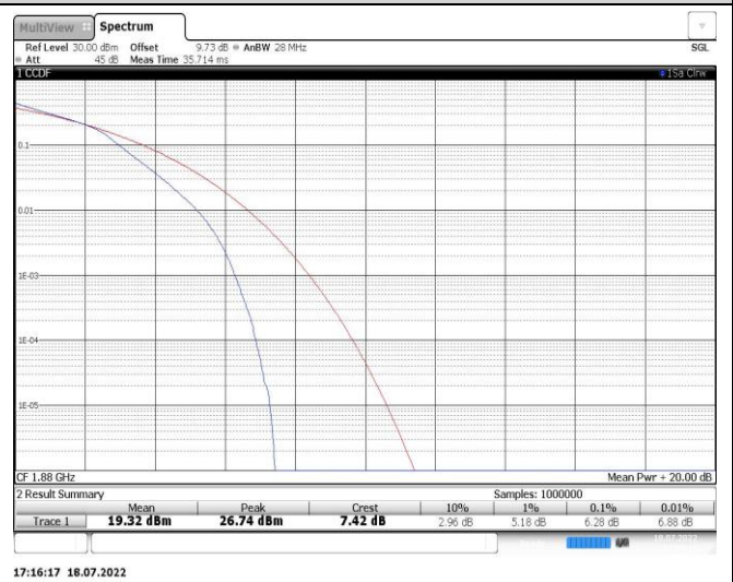
Band2-5MHz-16QAM-18900-25RB#0
