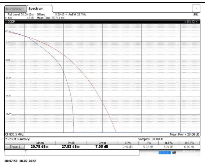
Band5-10MHz-16QAM-20525-50RB#0
