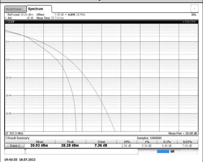
Band12-10MHz-16QAM-23095-50RB#0
