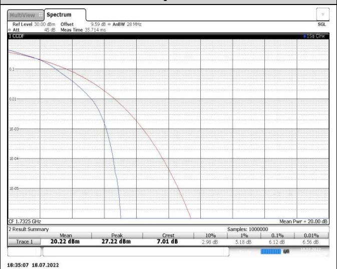
Band4-20MHz-16QAM-20175-100RB#0
