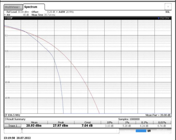
Band5-3MHz-16QAM-20525-15RB#0
