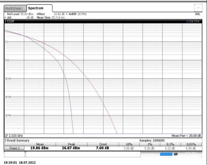
Band7-20MHz-16QAM-21100-100RB#0
