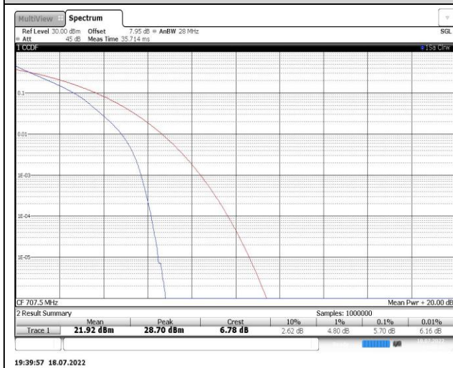
Band12-5MHz-QPSK-23095-25RB#0
