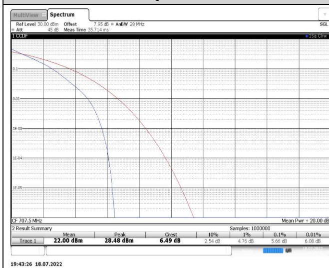
Band12-10MHz-QPSK-23095-50RB#0
