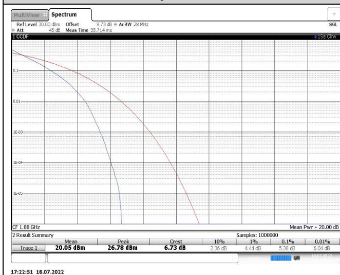
Band2-15MHz-QPSK-18900-75RB#0
