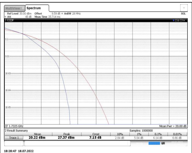
Band4-10MHz-16QAM-20175-50RB#0
