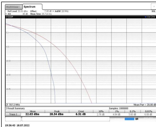
Band12-3MHz-QPSK-23095-15RB#0
