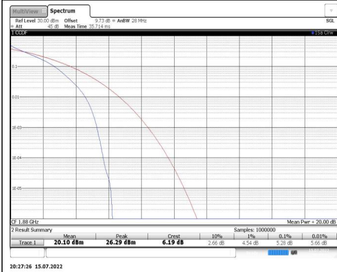
Band2-3MHz-QPSK-18900-15RB#0
