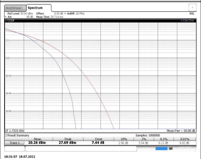
Band4-15MHz-16QAM-20175-75RB#0
