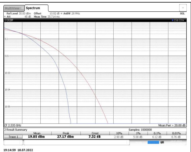
Band7-15MHz-16QAM-21100-75RB#0
