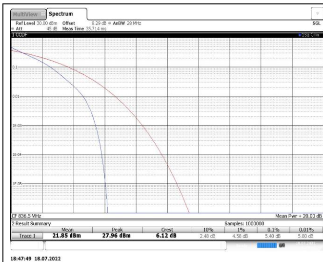
Band5-10MHz-QPSK-20525-50RB#0
