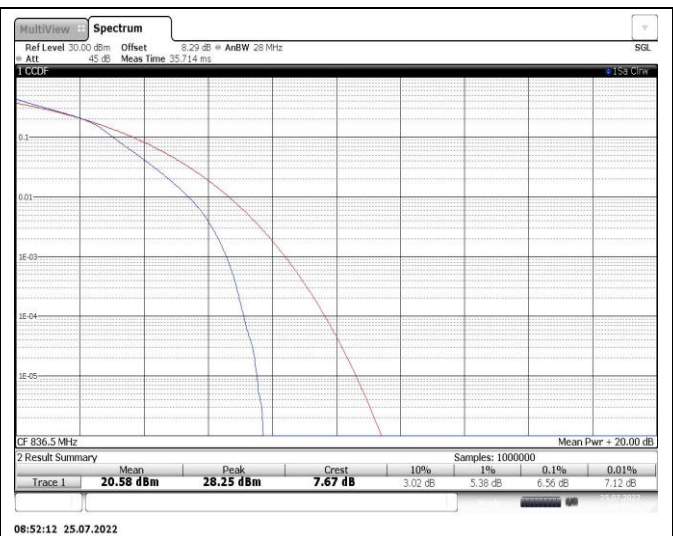
Band26-5MHz-QPSK-26915-25RB#0
