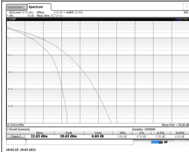
Band26-3MHz-16QAM-26740-15RB#0
