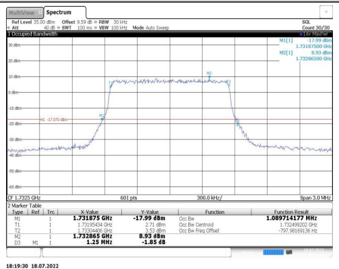
Band4-3MHz-16QAM-20175-15RB#0
