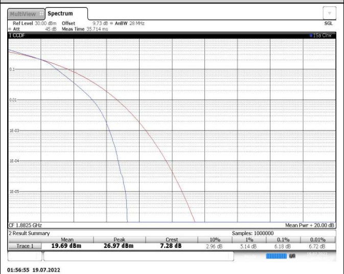
Band25-5MHz-16QAM-26365-25RB#0
