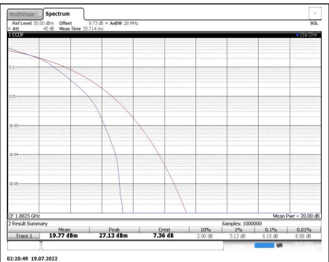
Band25-15MHz-16QAM-26365-75RB#0
