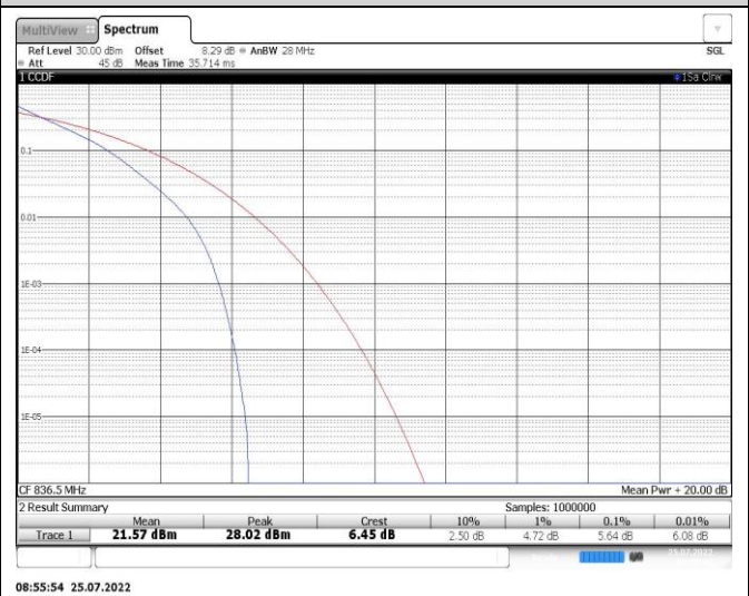
Band26-5MHz-16QAM-26915-25RB#0
