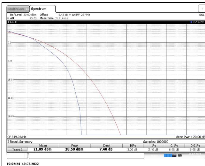
Band26-5MHz-QPSK-26740-25RB#0
