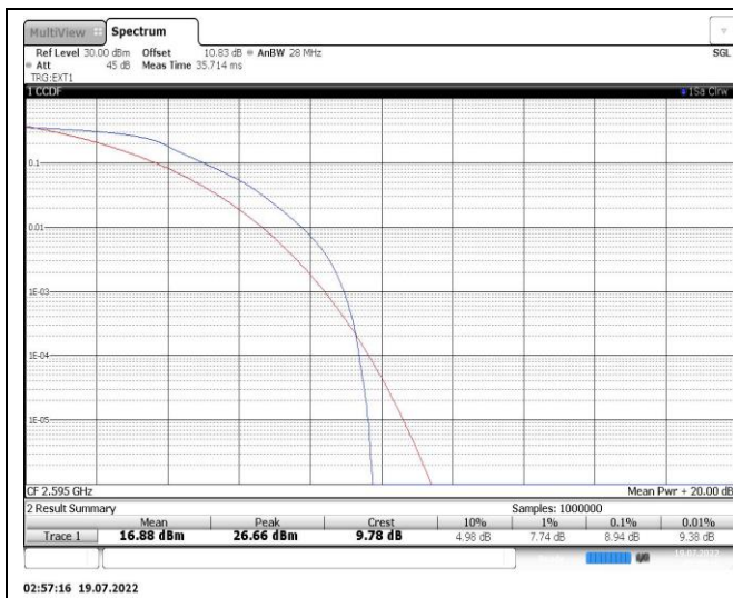
Band38-10MHz-QPSK-38000-50RB#0
