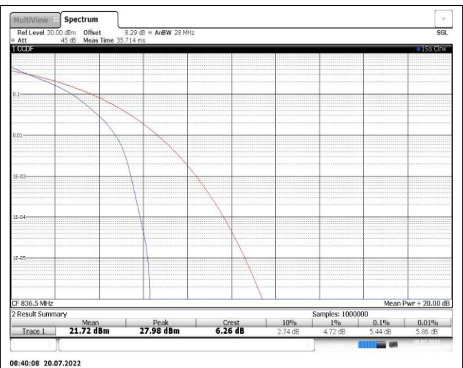
Band26-1.4MHz-16QAM-26915-6RB#0
