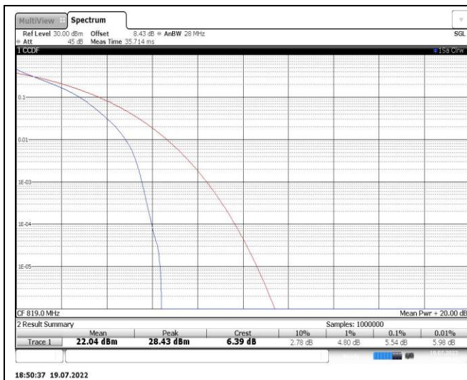
Band26-1.4MHz-16QAM-26740-6RB#0
