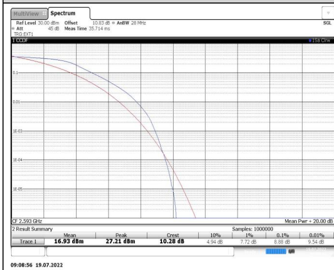
Band41-15MHz-QPSK-40620-75RB#0
