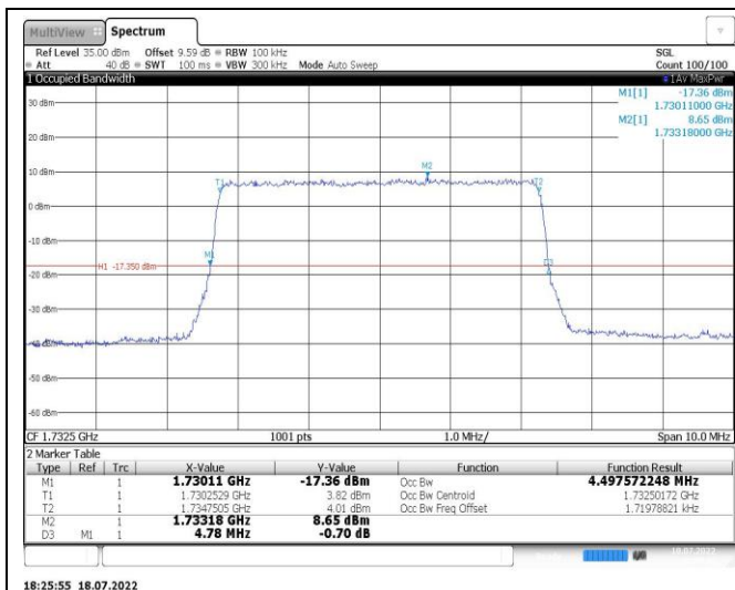
Band4-10MHz-QPSK-20175-50RB#0
