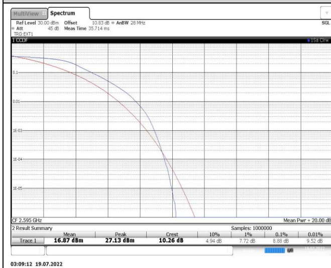
Band38-15MHz-QPSK-38000-75RB#0
