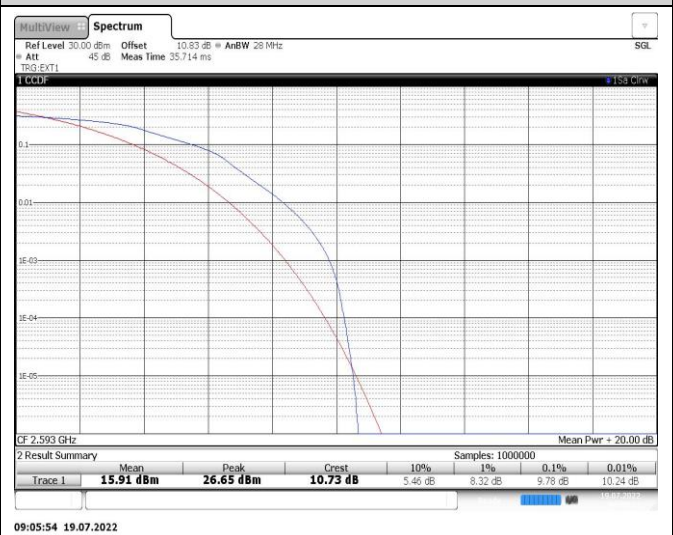
Band41-10MHz-16QAM-40620-50RB#0
