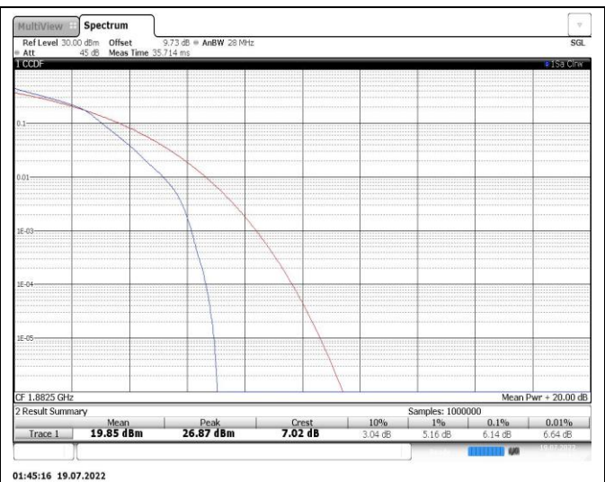
Band25-3MHz-16QAM-26365-15RB#0
