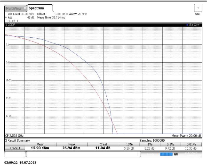
Band38-15MHz-16QAM-38000-75RB#0
