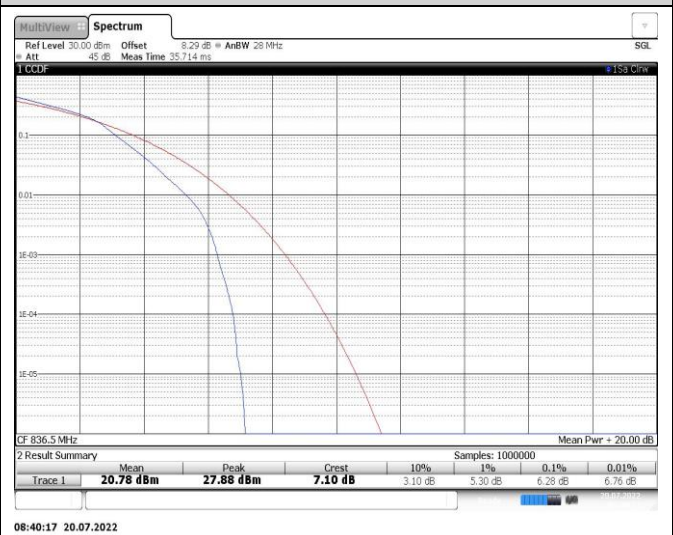
Band26-3MHz-QPSK-26915-15RB#0
