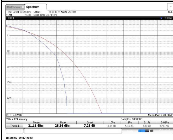
Band26-3MHz-QPSK-26740-15RB#0
