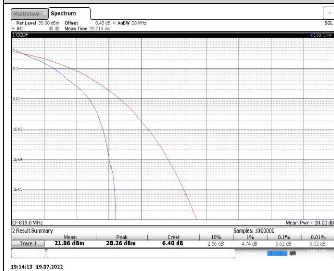
Band26-5MHz-16QAM-26740-25RB#0
