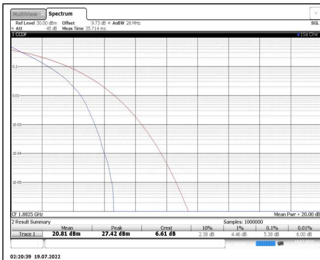
Band25-15MHz-QPSK-26365-75RB#0
