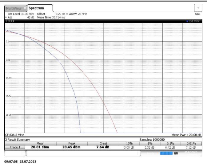
Band26-15MHz-16QAM-26915-75RB#0
