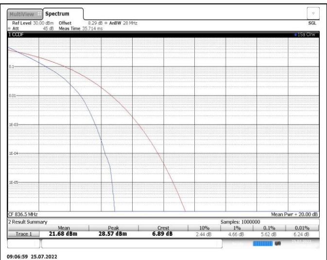
Band26-10MHz-16QAM-26915-50RB#0
