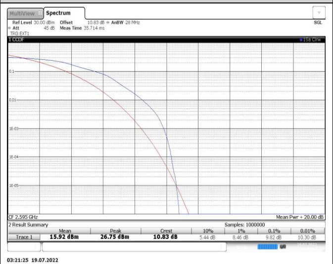
Band38-20MHz-16QAM-38000-100RB#0
