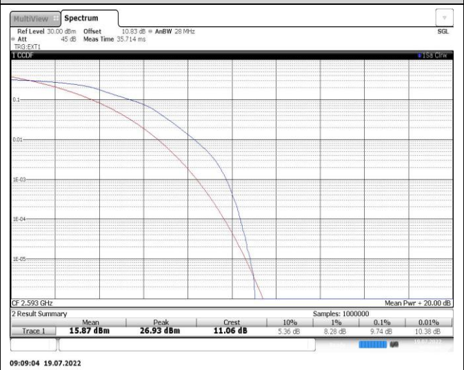
Band41-15MHz-16QAM-40620-75RB#0
