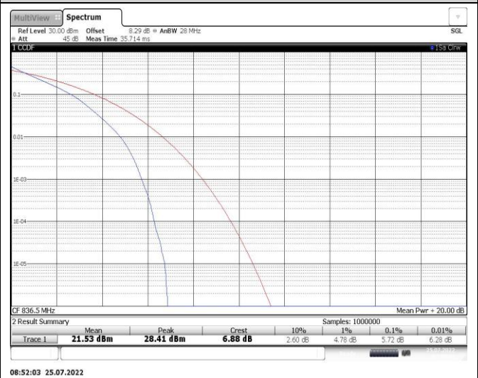
Band26-3MHz-16QAM-26915-15RB#0
