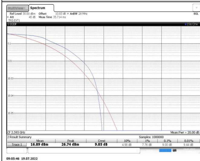
Band41-10MHz-QPSK-40620-50RB#0
