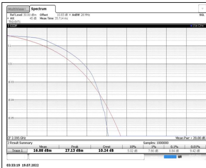
Band41-5MHz-QPSK-40620-25RB#0
