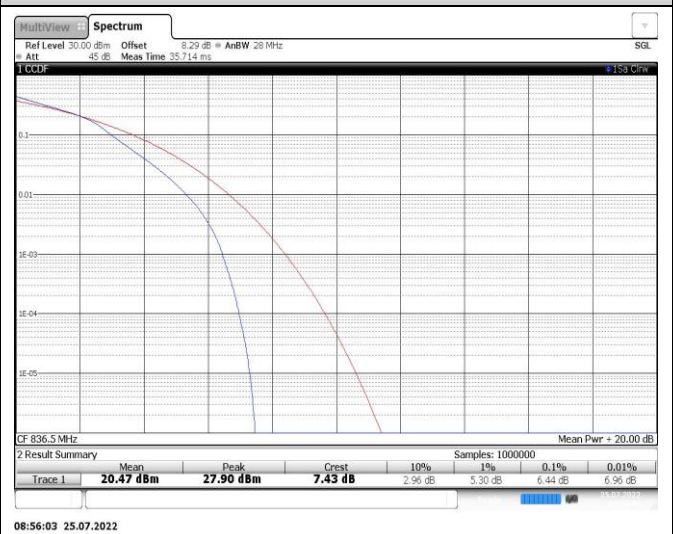
Band26-10MHz-QPSK-26915-50RB#0
