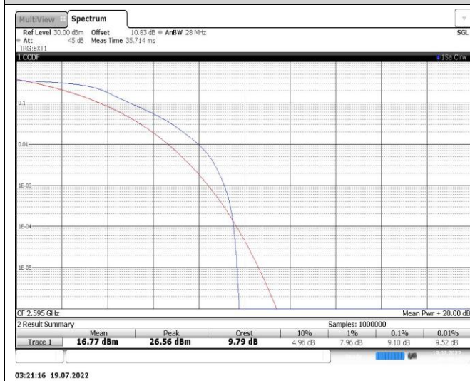
Band38-20MHz-QPSK-38000-100RB#0
