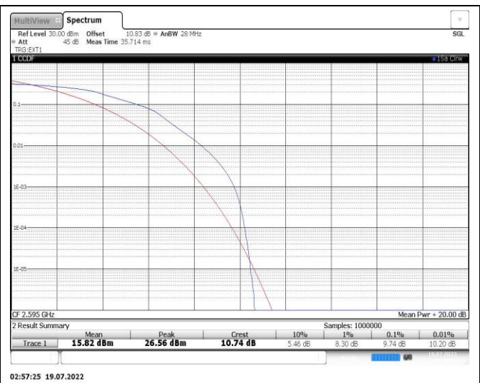
Band38-10MHz-16QAM-38000-50RB#0
