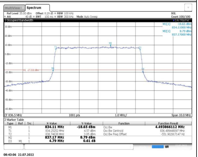
Band26-5MHz-16QAM-26915-25RB#0
