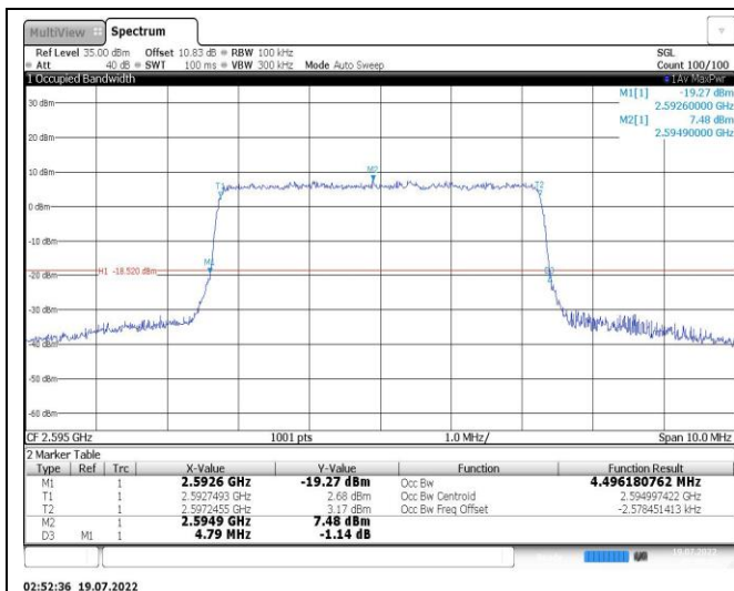
Band38-10MHz-QPSK-38000-50RB#0
