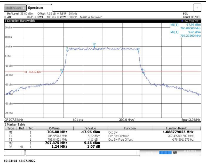
Band12-3MHz-16QAM-23095-15RB#0
