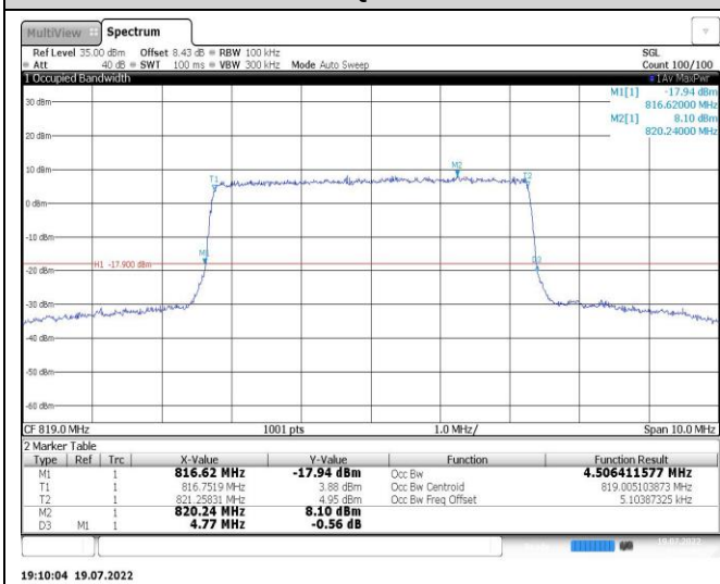
Band26-10MHz-QPSK-26740-50RB#0
