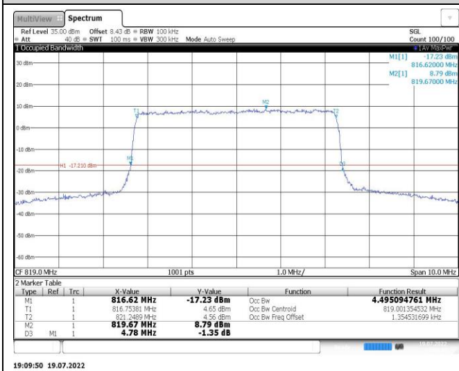
Band26-5MHz-16QAM-26740-25RB#0
