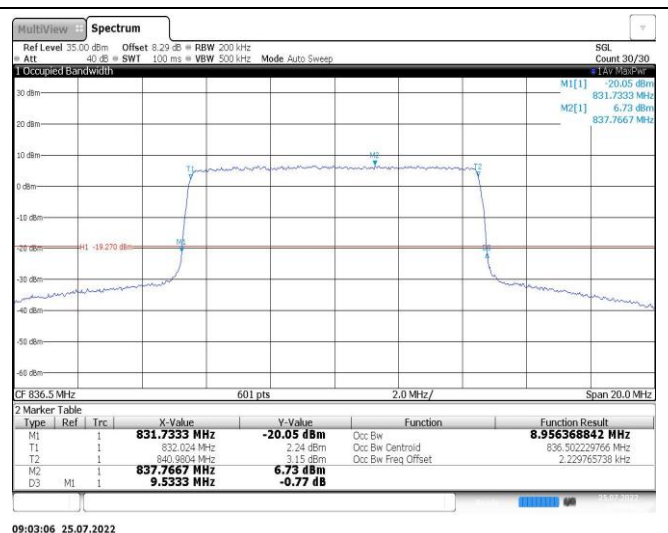
Band26-10MHz-16QAM-26915-50RB#0
