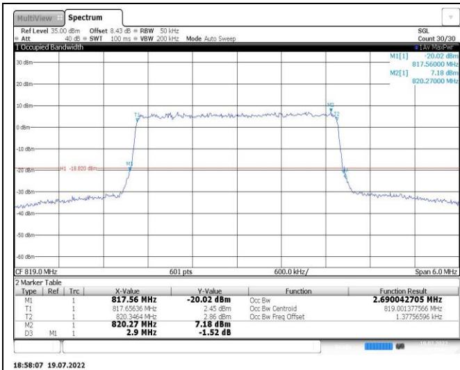
Band26-5MHz-QPSK-26740-25RB#0
