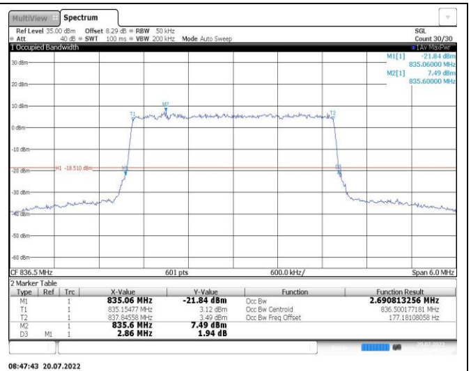
Band26-5MHz-QPSK-26915-25RB#0
