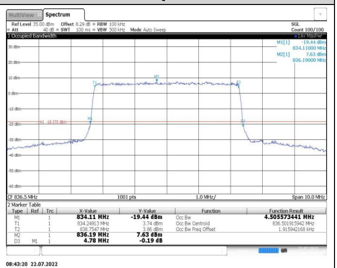
Band26-10MHz-QPSK-26915-50RB#0
