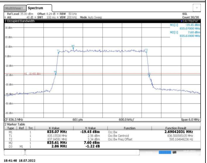
Band5-5MHz-16QAM-20525-25RB#0
