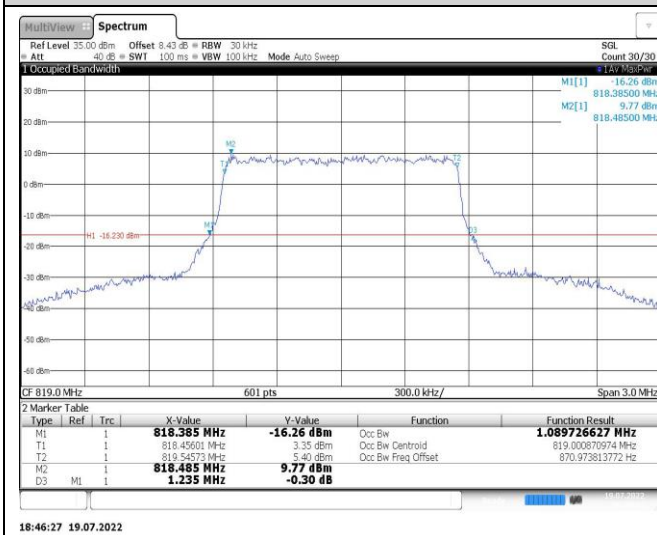
Band26-3MHz-QPSK-26740-15RB#0
