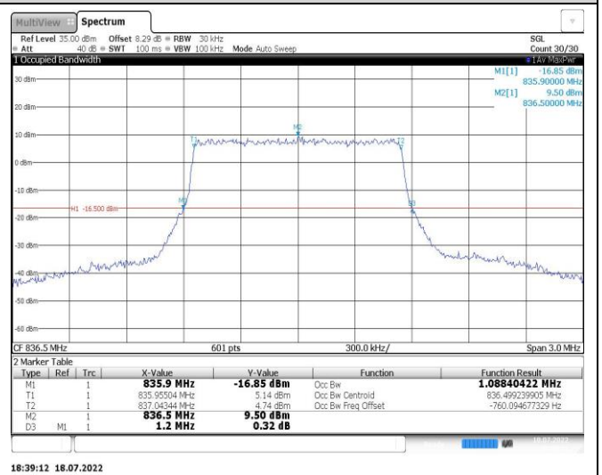
Band5-3MHz-16QAM-20525-15RB#0
