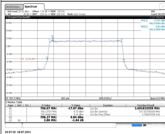
Band12-5MHz-QPSK-23095-25RB#0
