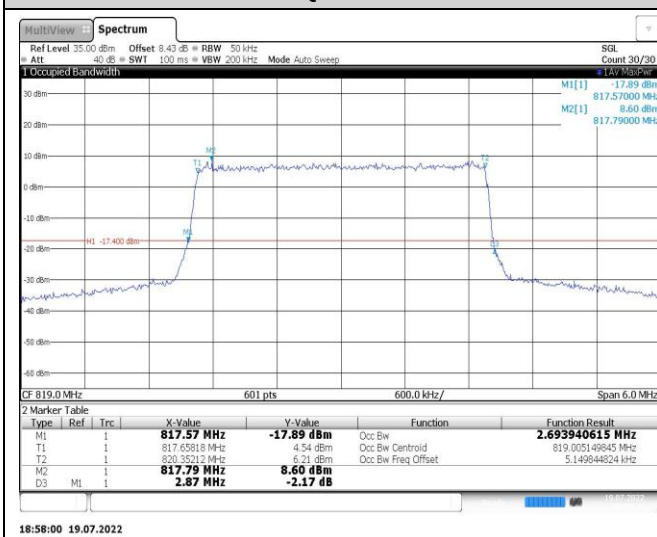
Band26-3MHz-16QAM-26740-15RB#0
