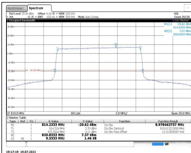
Band26-10MHz-16QAM-26740-50RB#0
