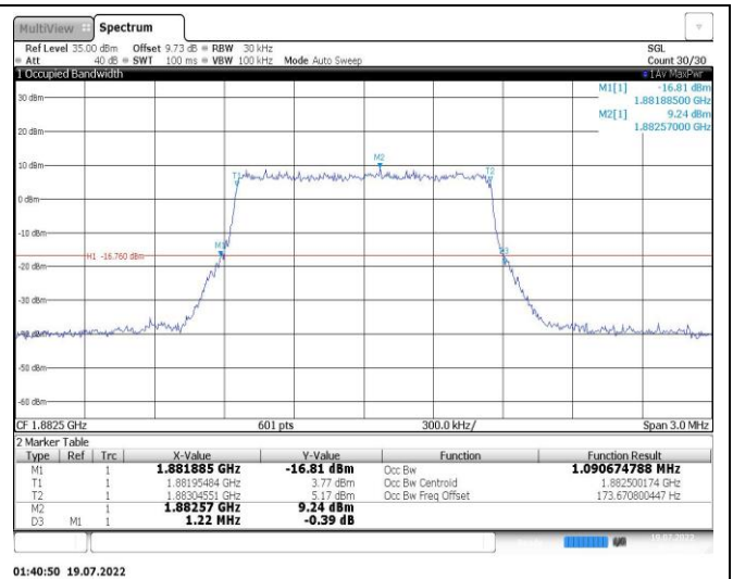
Band25-3MHz-16QAM-26365-15RB#0
