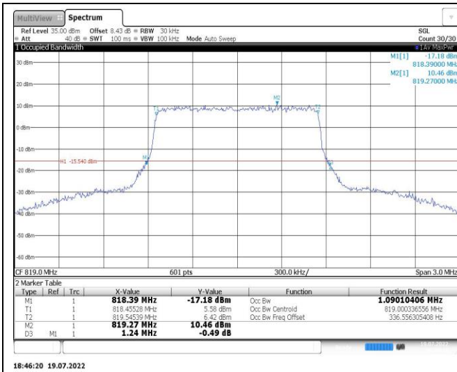
Band26-1.4MHz-16QAM-26740-6RB#0
