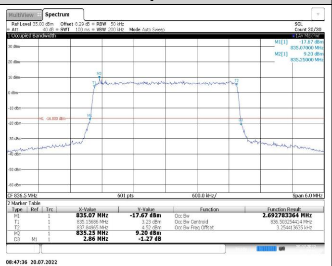
Band26-3MHz-16QAM-26915-15RB#0
