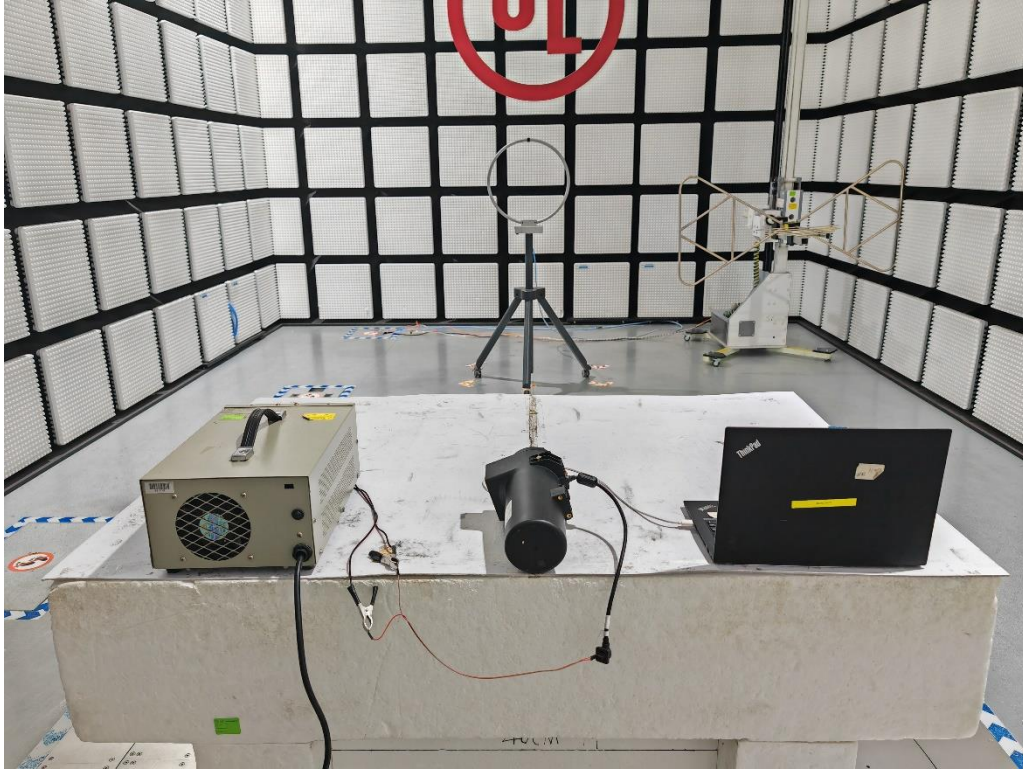
Setup photo of radar function
