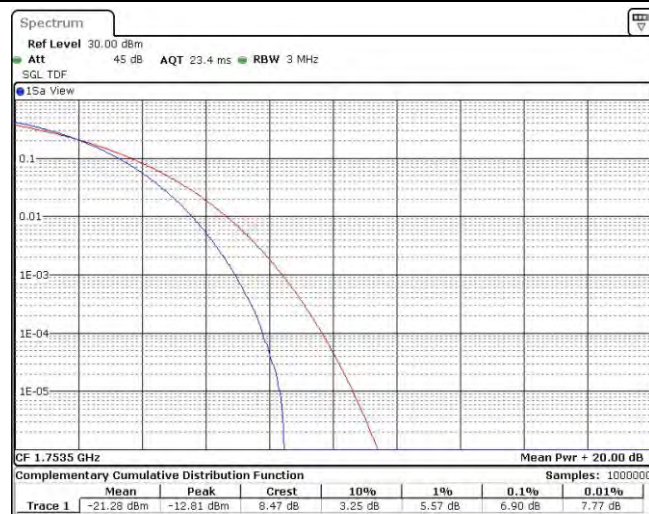
Band4-3MHz-QPSK-20385-15RB#0
