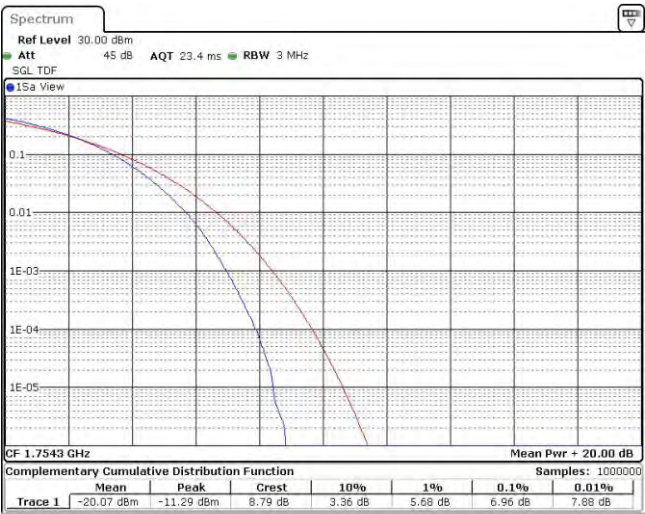
Band4-1.4MHz-16QAM-20393-6RB#0
