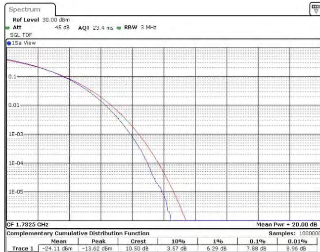
Band4-5MHz-16QAM-20175-25RB#0
