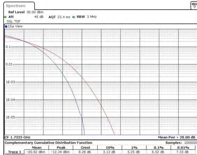
Band4-5MHz-QPSK-20375-1RB#0
