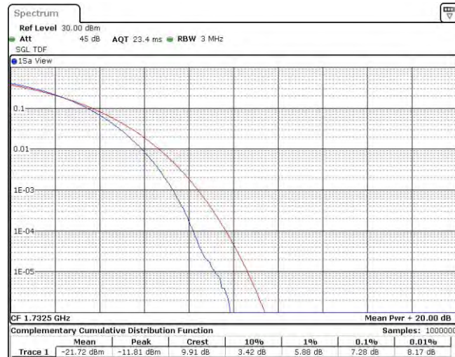
Band4-3MHz-16QAM-20175-15RB#0
