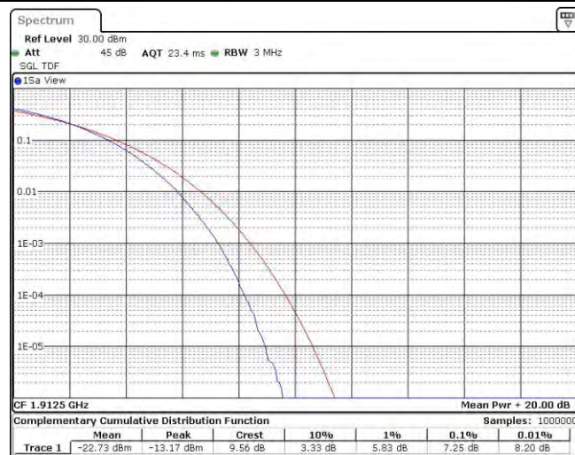
Band25-5MHz-QPSK-26665-25RB#0
