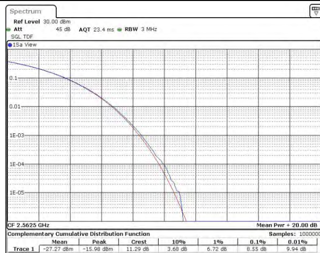
Band7-15MHz-16QAM-21375-75RB#0
