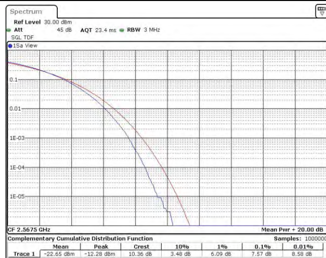
Band7-5MHz-16QAM-21425-25RB#0
