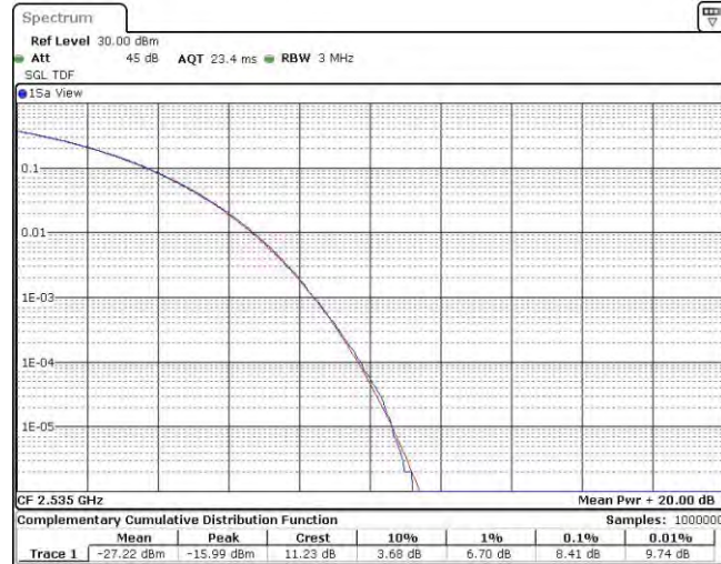
Band7-20MHz-QPSK-21100-100RB#0
