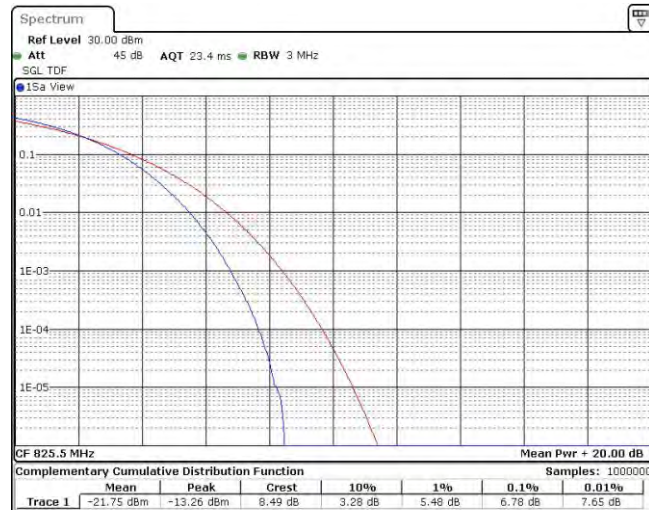
Band5-3MHz-16QAM-20415-15RB#0
