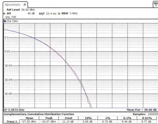
Band7-15MHz-QPSK-20825-75RB#0
