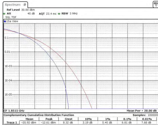
Band25-3MHz-QPSK-26055-15RB#0
