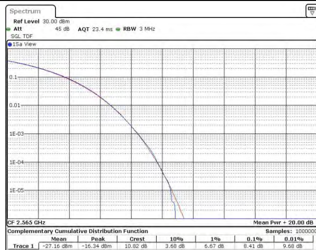
Band7-10MHz-QPSK-21400-50RB#0
