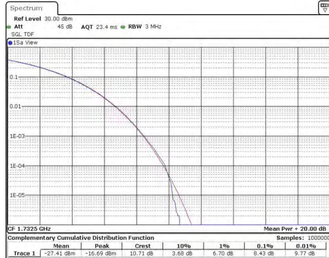
Band4-15MHz-QPSK-20175-75RB#0
