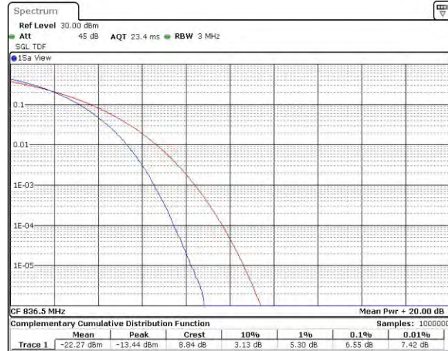
Band5-3MHz-QPSK-20525-15RB#0
