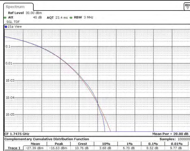
Band4-15MHz-QPSK-20325-75RB#0
