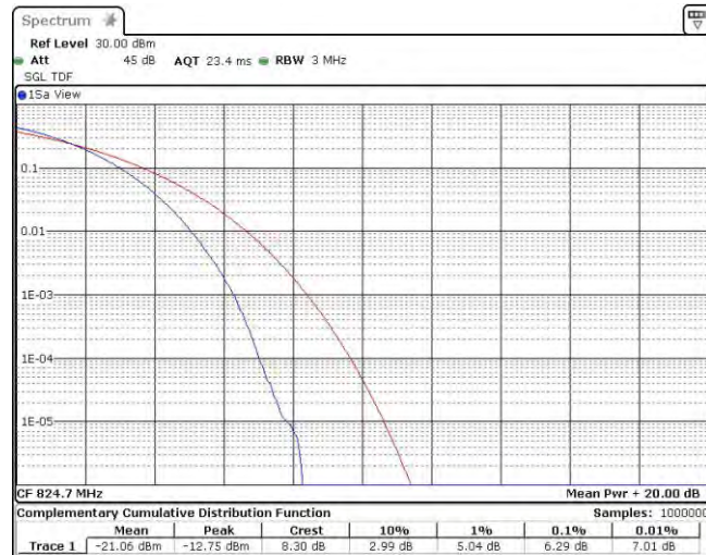
Band5-1.4MHz-QPSK-20407-6RB#0
