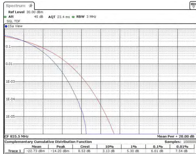
Band5-3MHz-QPSK-20415-15RB#0
