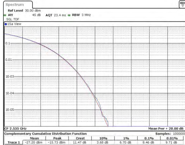
Band7-20MHz-16QAM-21100-100RB#0
