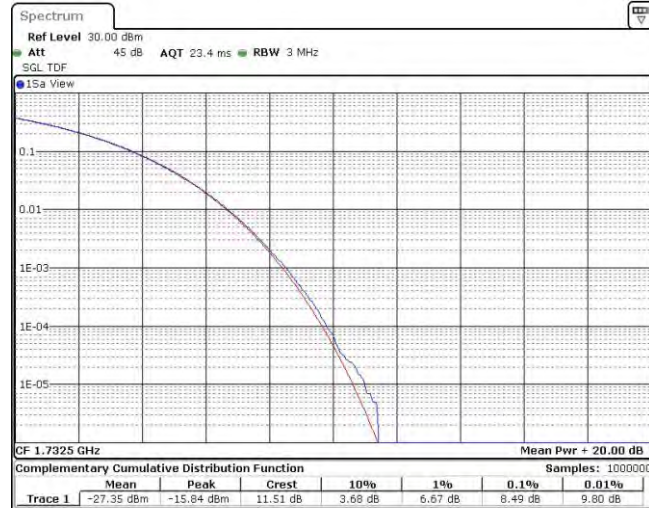
Band4-20MHz-QPSK-20175-100RB#0
