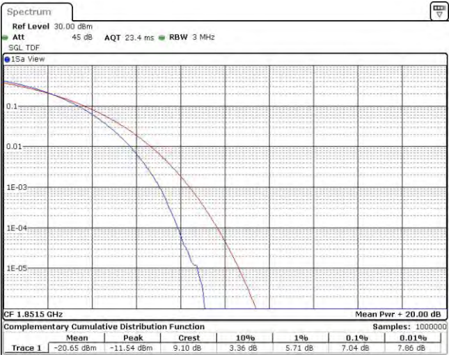
Band25-3MHz-16QAM-26055-15RB#0
