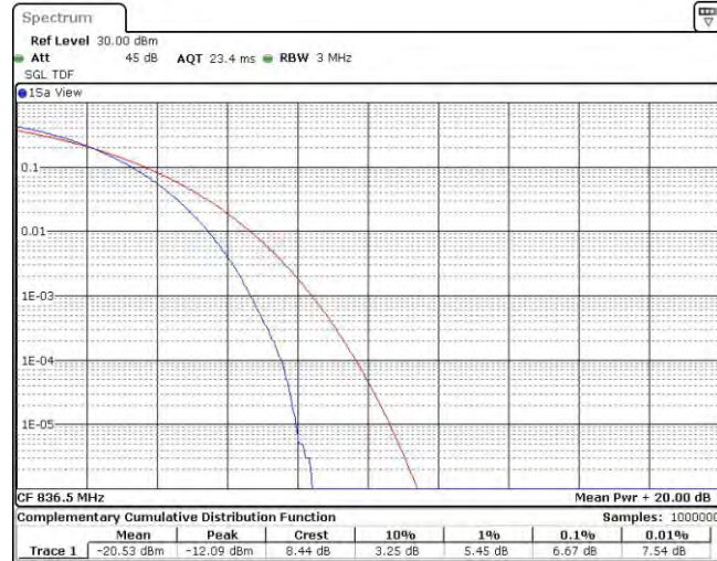
Band5-1.4MHz-16QAM-20525-6RB#0
