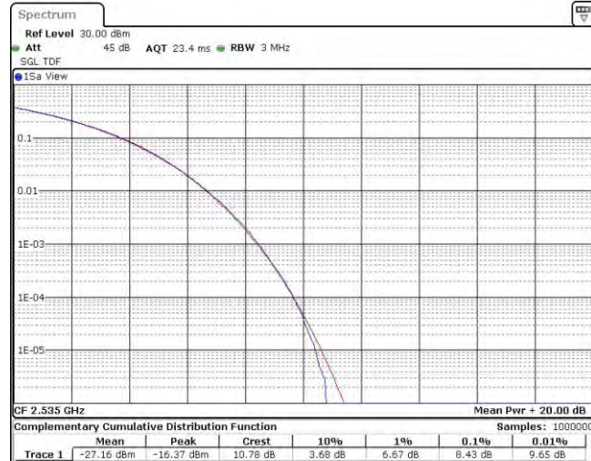
Band7-10MHz-QPSK-21100-50RB#0
