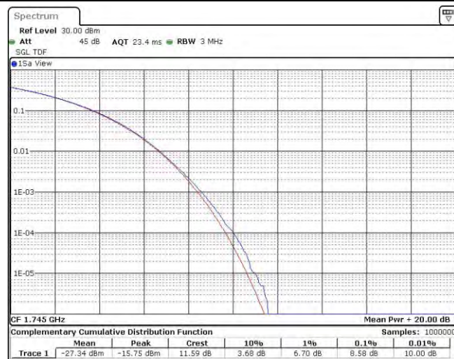
Band4-20MHz-16QAM-20300-100RB#0
