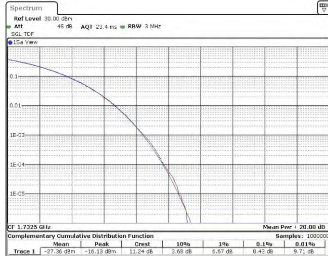
Band4-20MHz-16QAM-20175-100RB#0
