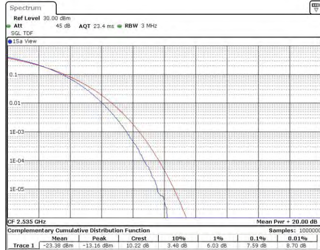
Band7-5MHz-QPSK-21100-25RB#0
