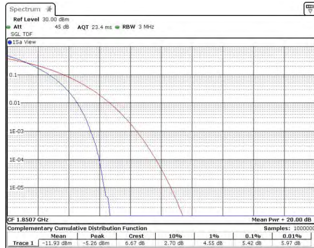
Band25-1.4MHz-QPSK-26047-6RB#0
