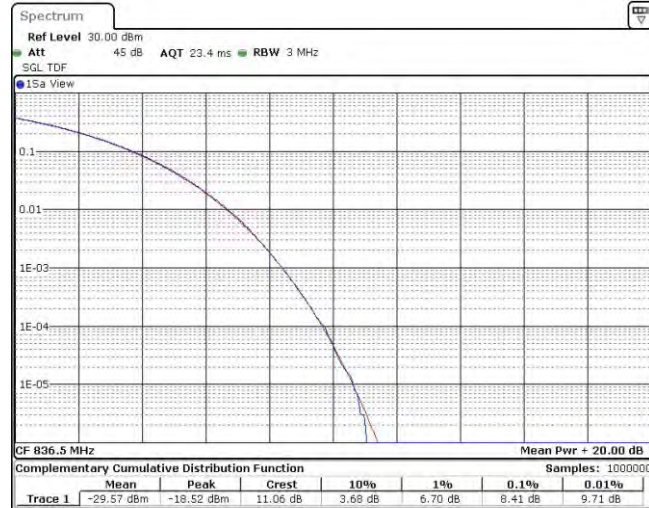
Band5-10MHz-QPSK-20525-50RB#0
