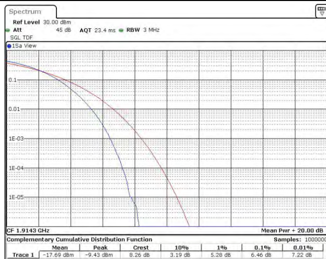
Band25-1.4MHz-16QAM-26683-6RB#0
