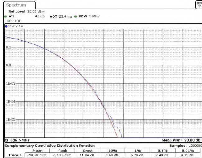
Band5-10MHz-16QAM-20525-50RB#0
