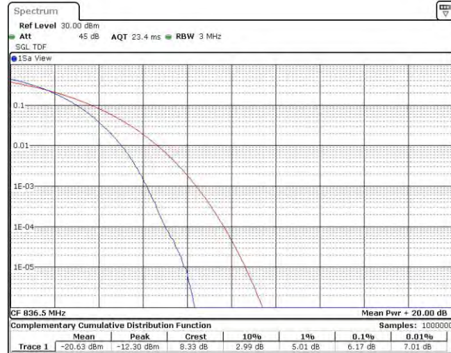
Band5-1.4MHz-QPSK-20525-6RB#0
