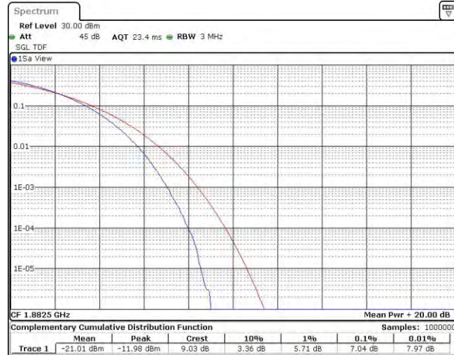
Band25-3MHz-16QAM-26365-15RB#0
