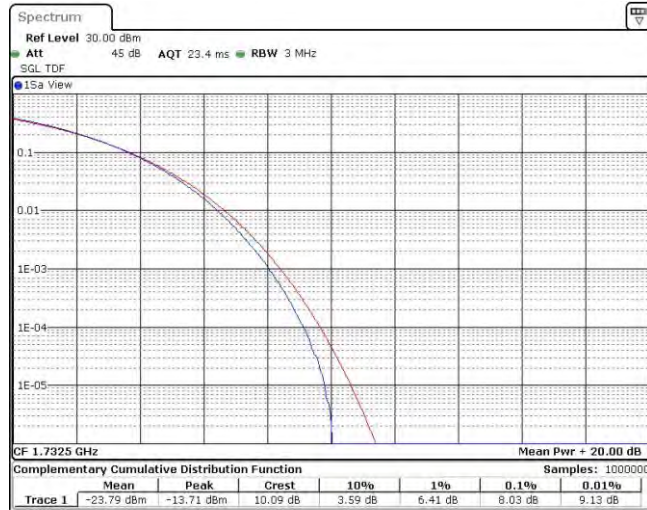
Band4-15MHz-16QAM-20325-1RB#0
