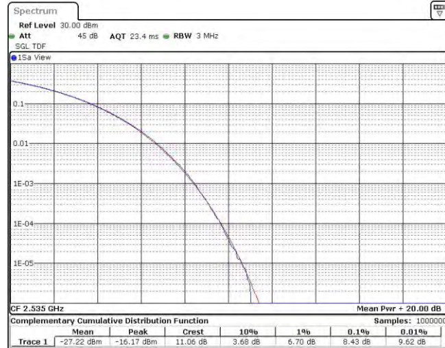
Band7-15MHz-QPSK-21100-75RB#0
