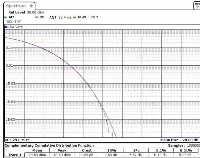
Band5-10MHz-QPSK-20450-50RB#0
