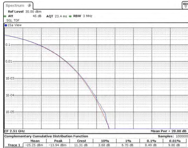
Band7-20MHz-QPSK-20850-100RB#0
