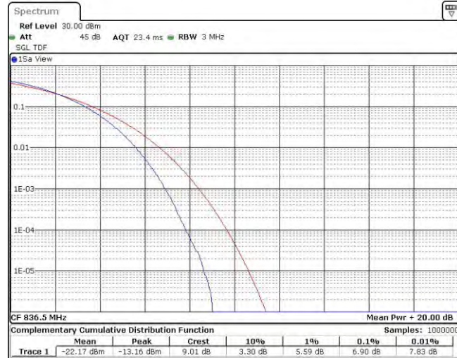
Band5-3MHz-16QAM-20525-15RB#0
