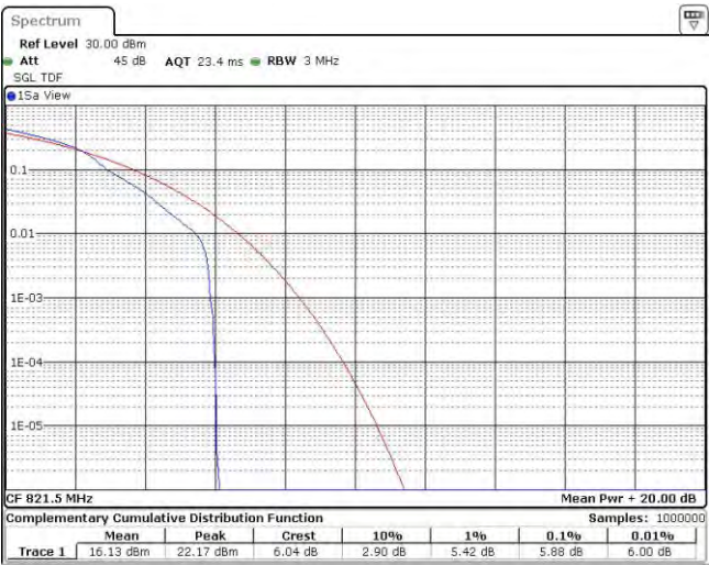
Band26-5MHz-16QAM-26765-25RB#0
