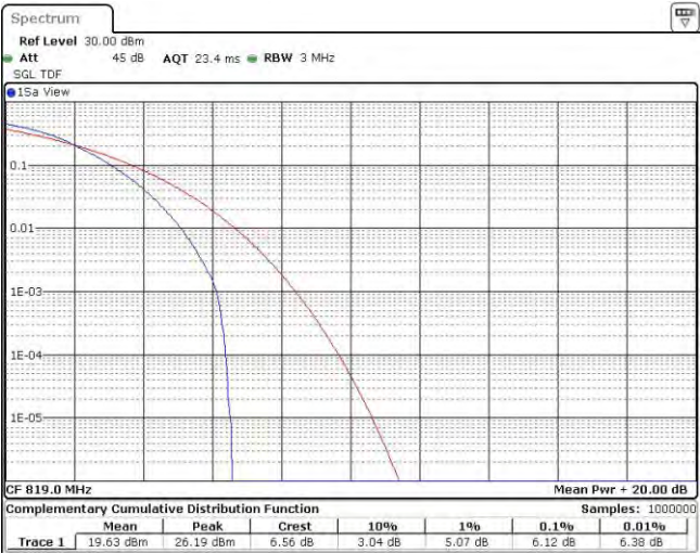
Band26-5MHz-16QAM-26765-1RB#0
