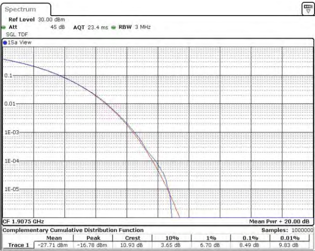
Band25-15MHz-QPSK-26615-75RB#0
