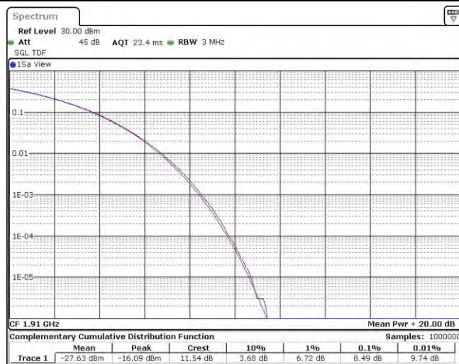
Band25-10MHz-16QAM-26640-50RB#0
