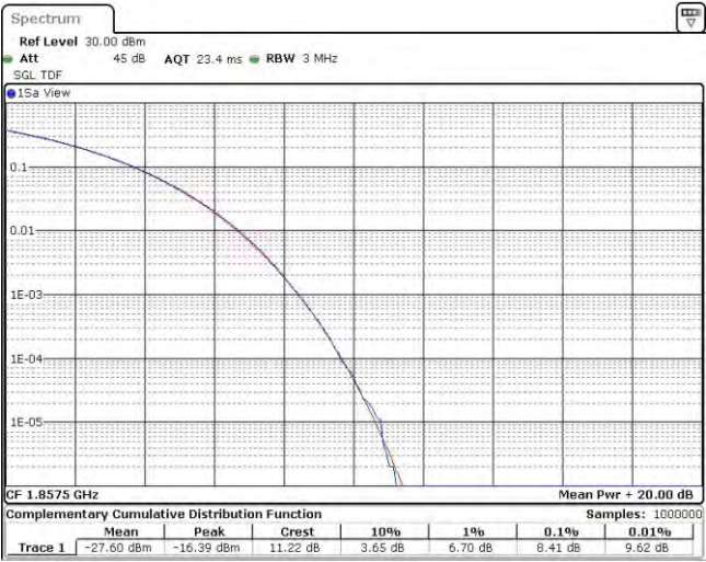
Band25-15MHz-16QAM-26115-75RB#0
