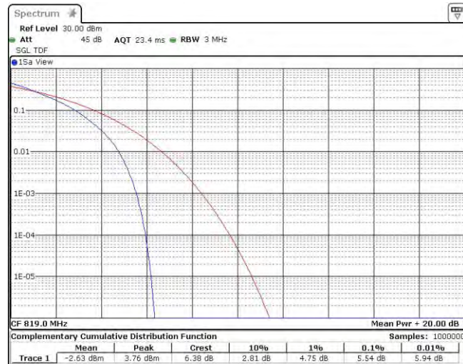
Band26-10MHz-QPSK-26740-50RB#0
