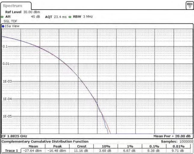
Band25-15MHz-QPSK-26365-75RB#0
