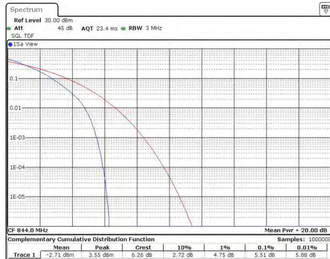
Band26-10MHz-QPSK-26990-50RB#0
