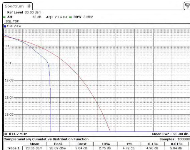
Band26-1.4MHz-QPSK-26697-6RB#0
