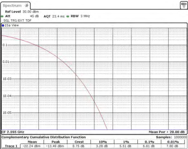
Band38-15MHz-16QAM-38000-75RB#0
