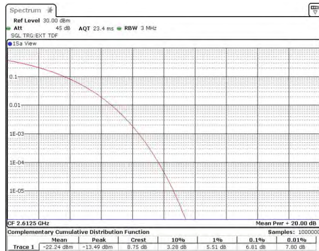
Band38-15MHz-QPSK-38175-75RB#0
