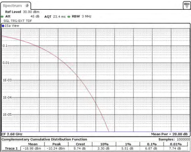
Band41-20MHz-16QAM-41490-100RB#0
