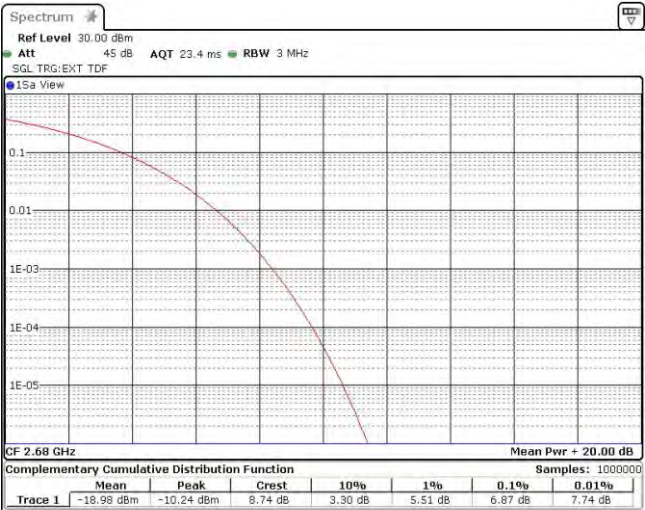
Band41-20MHz-16QAM-41490-100RB#0
