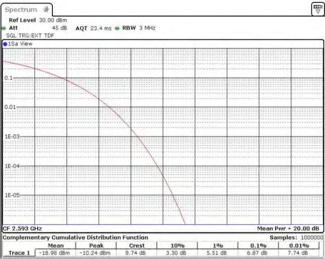
Band41-10MHz-16QAM-40620-50RB#0
