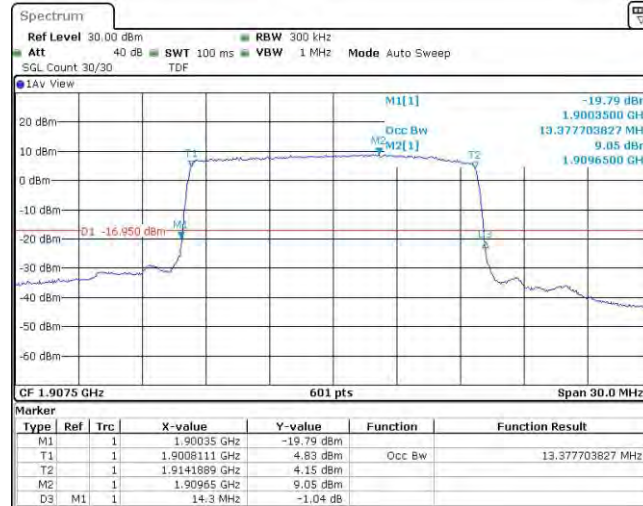
Band25-15MHz-16QAM-26115-75RB#0
