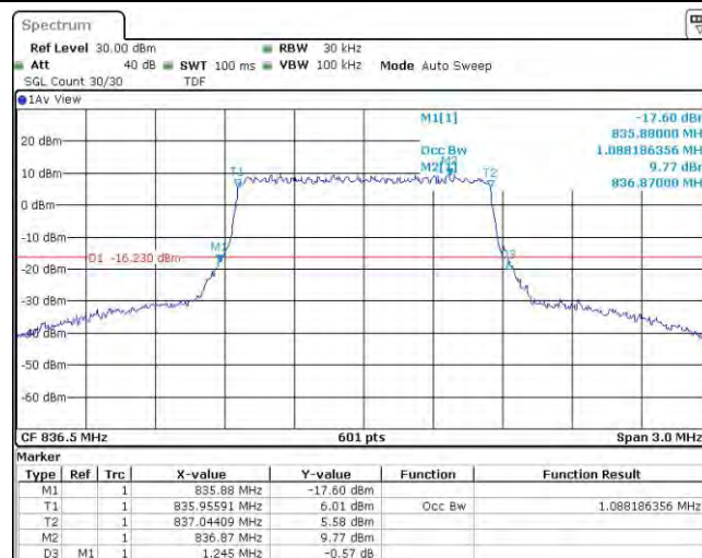
Band26-1.4MHz-16QAM-26915-6RB#0
