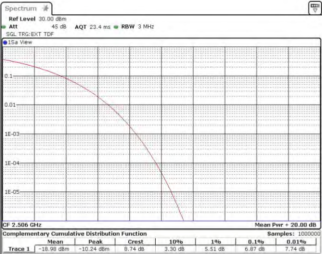
Band41-20MHz-16QAM-40620-1RB#0
