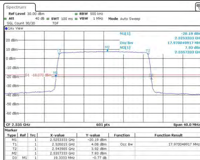
Band7-20MHz-QPSK-21350-100RB#0
