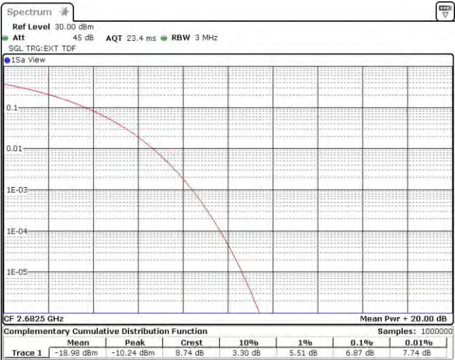
Band41-15MHz-16QAM-41515-75RB#0
