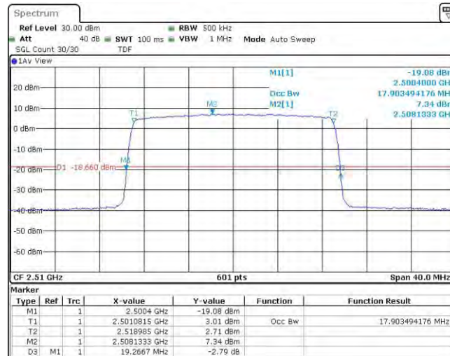
Band7-20MHz-16QAM-21100-100RB#0
