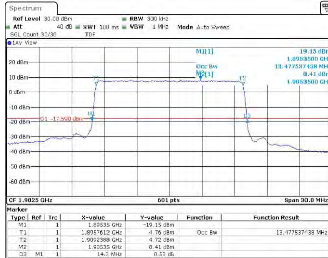
Band2-15MHz-16QAM-18675-75RB#0
