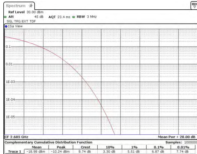
Band41-10MHz-16QAM-41540-50RB#0
