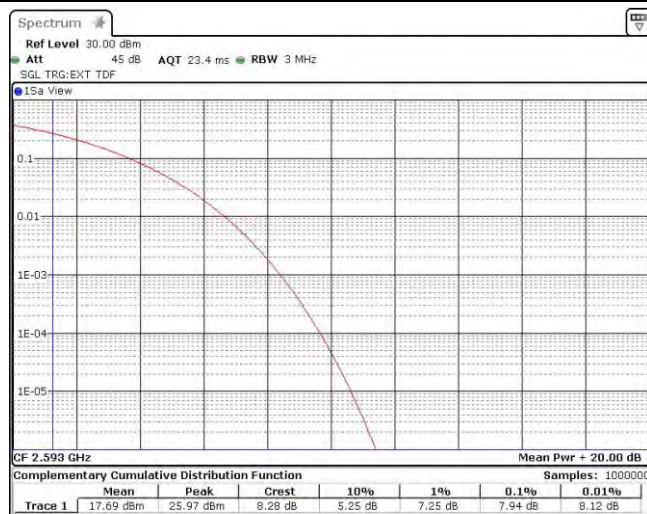
Band41-15MHz-QPSK-40620-75RB#0
