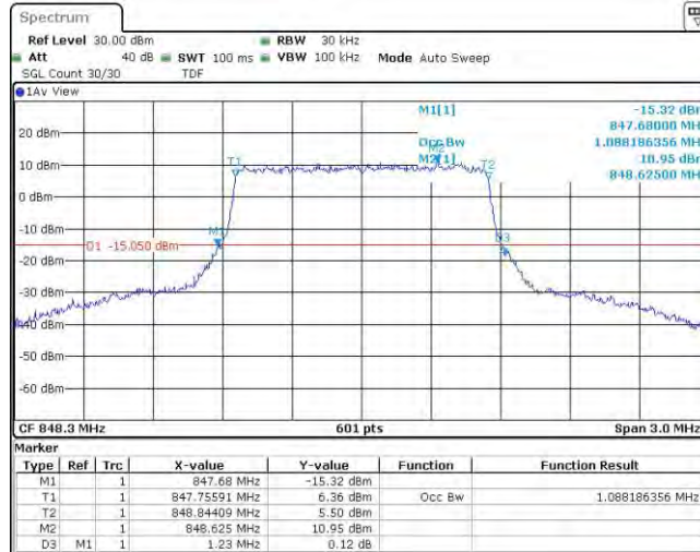
Band26-1.4MHz-16QAM-26697-6RB#0
