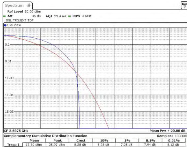
Band41-5MHz-QPSK-41565-25RB#0
