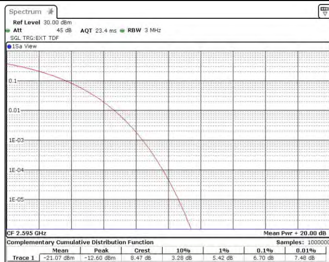
Band38-10MHz-16QAM-38000-50RB#0
