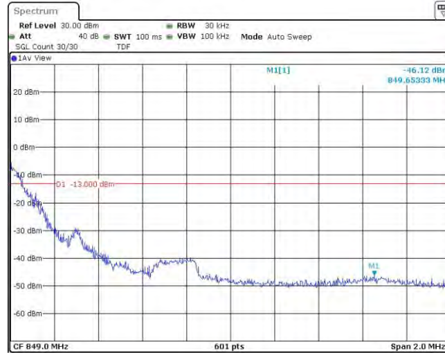
Band5-1.4MHz-16QAM-20643-1RB#5
