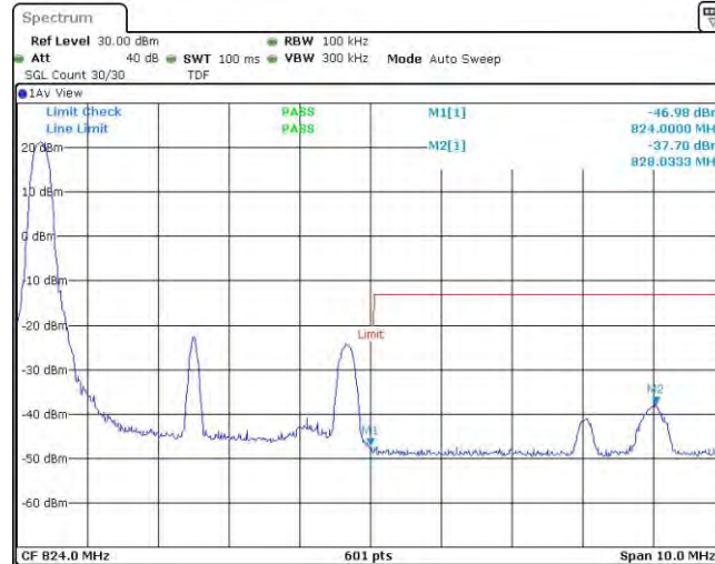
Band26-5MHz-QPSK-26765-1RB#24
