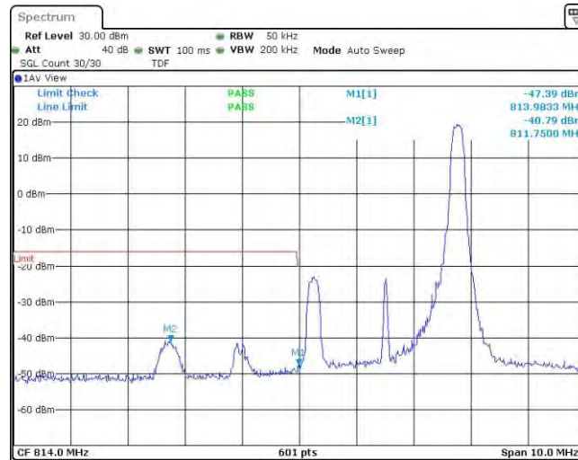
Band26-3MHz-QPSK-26705-15RB#0
