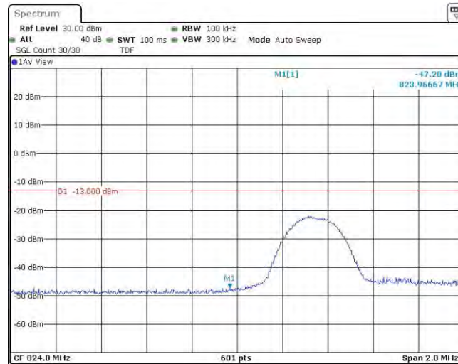
Band26-5MHz-16QAM-26815-25RB#0
