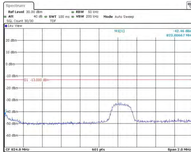
Band5-3MHz-16QAM-20415-15RB#0
