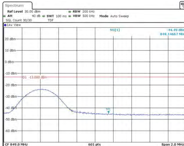
Band5-10MHz-16QAM-20600-1RB#49
