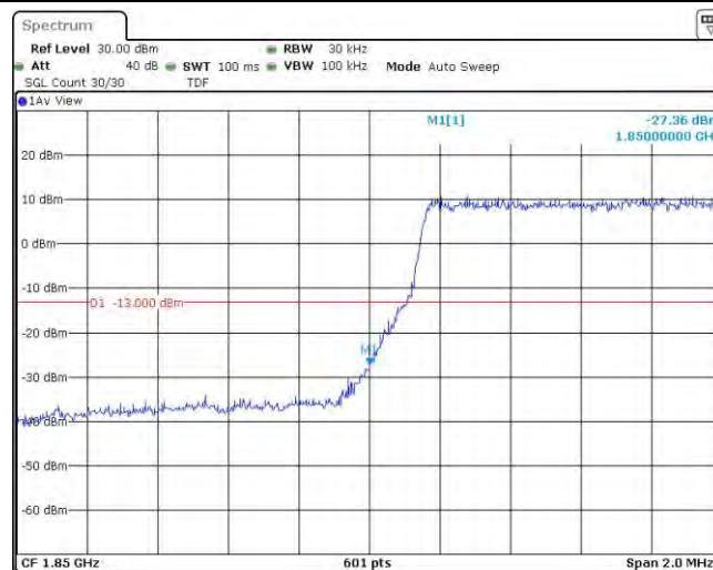
Band25-1.4MHz-16QAM-26683-1RB#0
