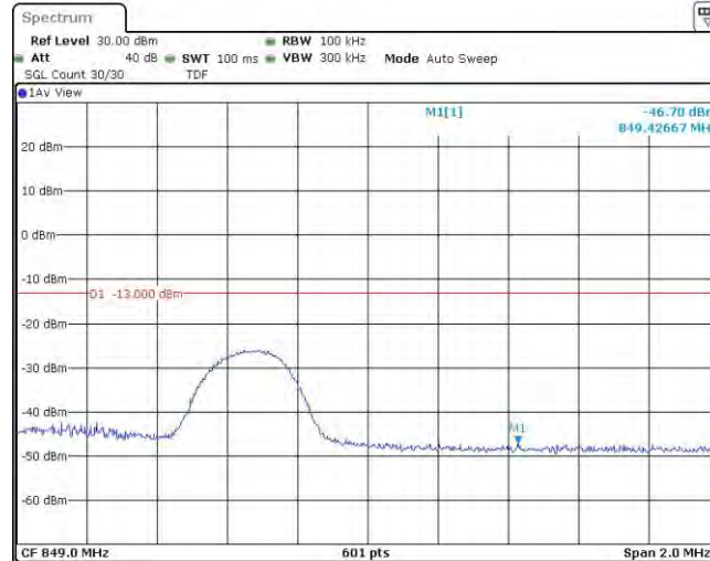
Band5-5MHz-QPSK-20625-1RB#24
