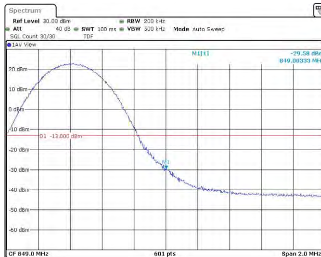
Band5-10MHz-16QAM-20600-50RB#0
