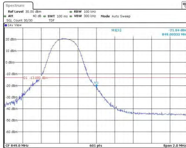
Band26-5MHz-16QAM-27015-25RB#0
