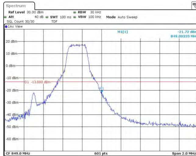
Band26-1.4MHz-16QAM-27033-6RB#0
