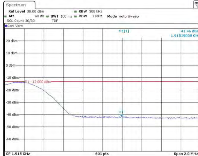
Band25-15MHz-16QAM-26615-1RB#74
