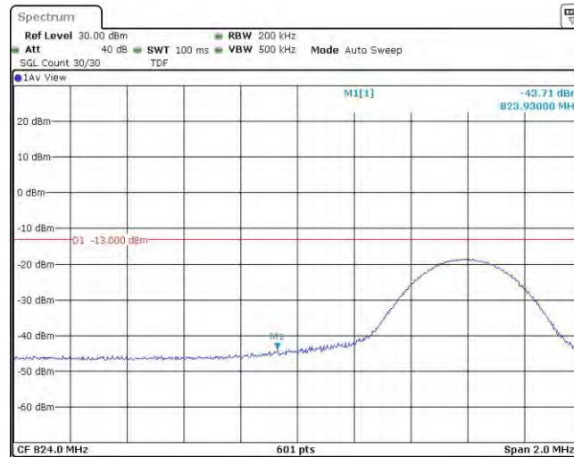
Band26-10MHz-QPSK-26840-50RB#0
