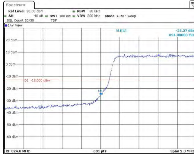
Band5-3MHz-QPSK-20415-1RB#14
