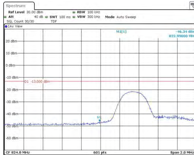
Band26-5MHz-QPSK-26815-25RB#0
