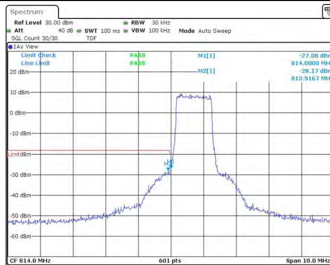
Band26-1.4MHz-16QAM-26783-1RB#0
