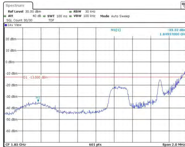
Band25-1.4MHz-QPSK-26047-6RB#0
