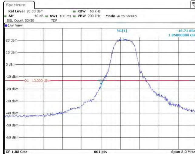
Band25-3MHz-QPSK-26055-1RB#14
