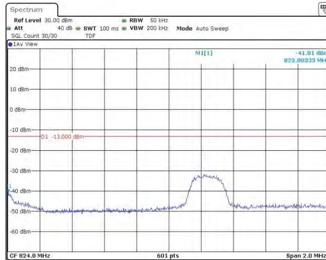
Band5-3MHz-QPSK-20415-15RB#0
