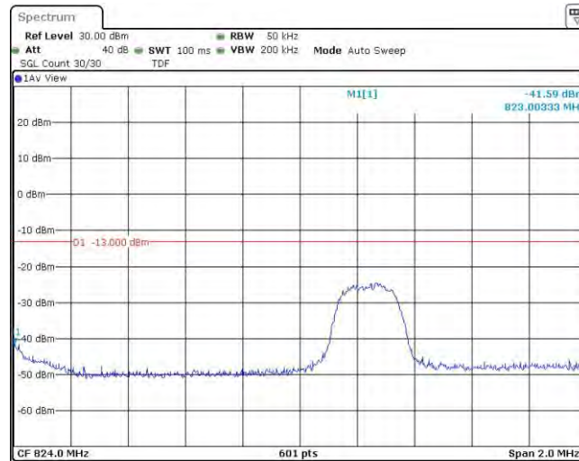
Band26-3MHz-16QAM-26805-15RB#0
