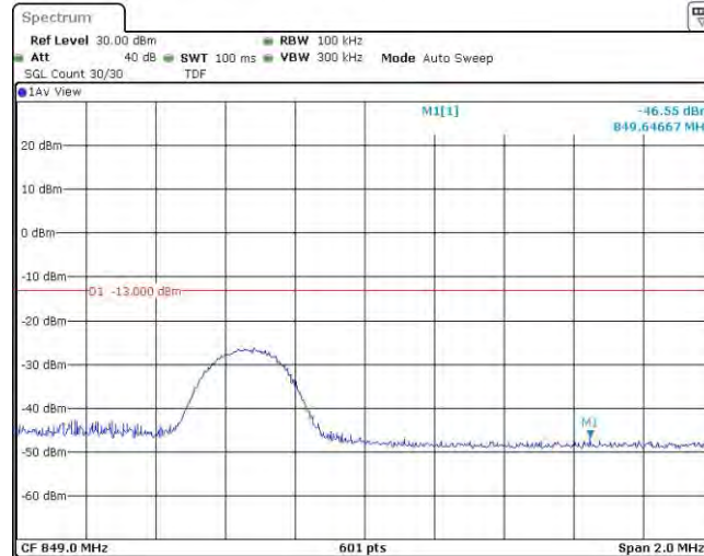
Band5-5MHz-16QAM-20625-1RB#24
