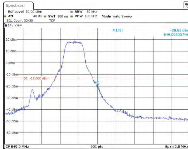
Band26-1.4MHz-QPSK-27033-6RB#0
