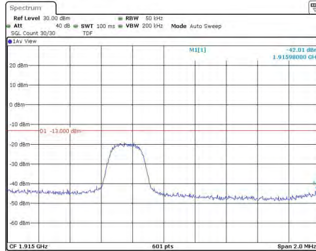
Band25-3MHz-16QAM-26675-1RB#14
