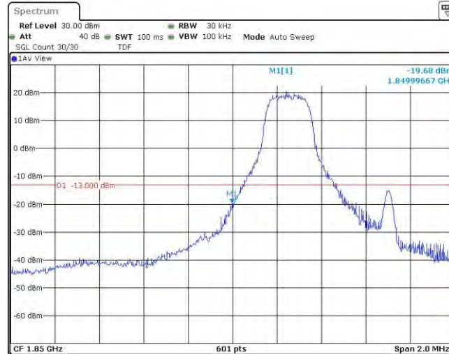
Band25-1.4MHz-QPSK-26047-1RB#5
