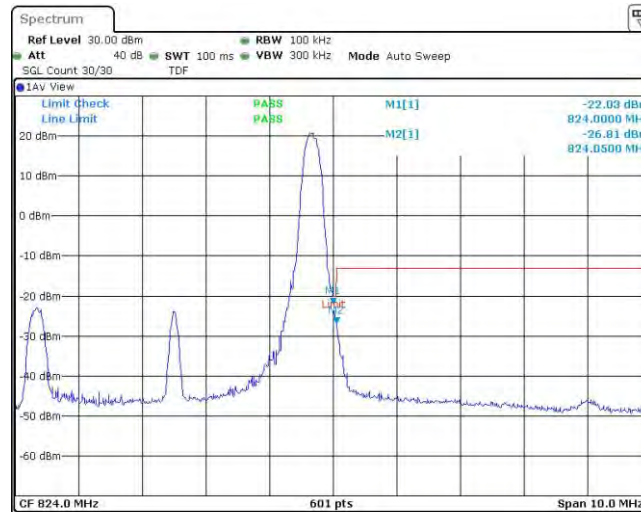
Band26-5MHz-16QAM-26765-25RB#0
