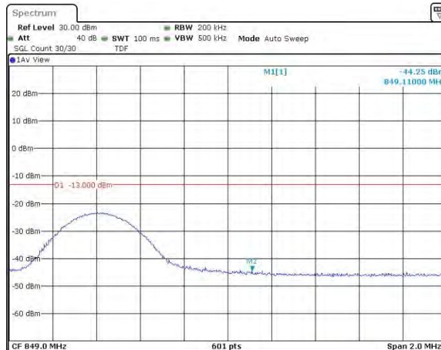
Band5-10MHz-QPSK-20600-1RB#49
