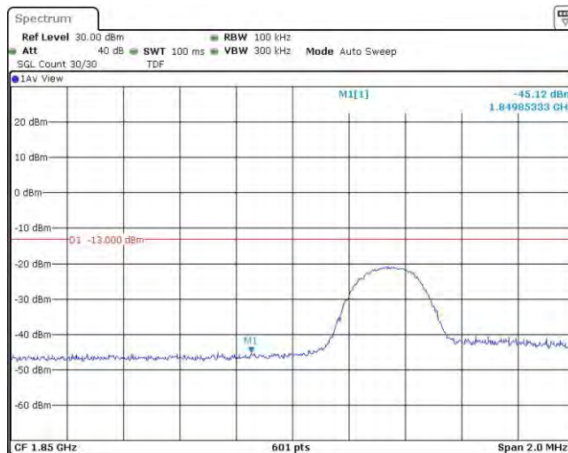
Band25-5MHz-QPSK-26065-25RB#0
