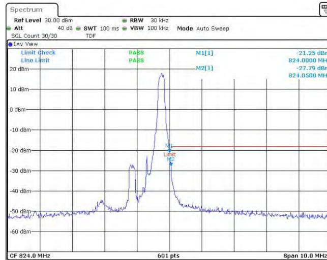
Band26-1.4MHz-16QAM-26783-6RB#0
