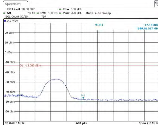
Band26-5MHz-QPSK-27015-1RB#24
