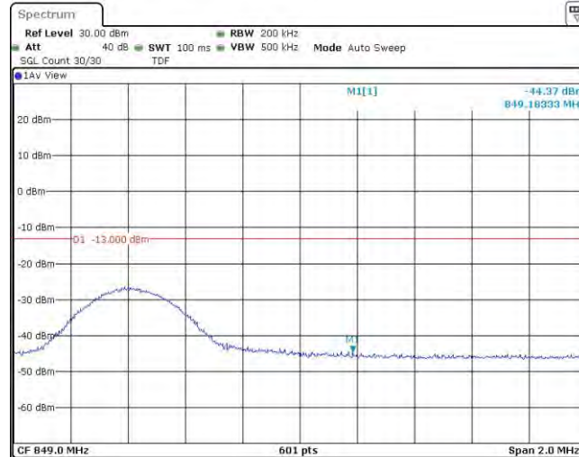
Band26-10MHz-16QAM-26990-1RB#49
