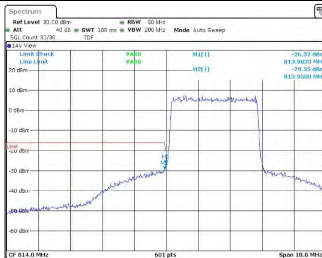
Band26-3MHz-16QAM-26705-15RB#0
