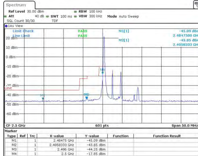
Band7-5MHz-QPSK-20775-1RB#24
