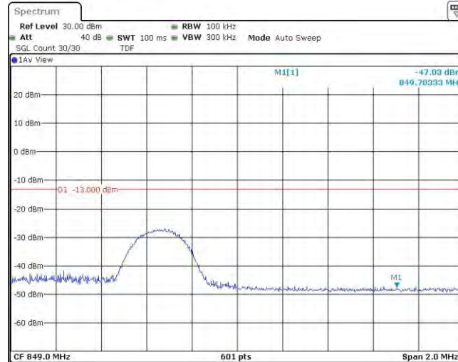
Band26-5MHz-16QAM-27015-1RB#24
