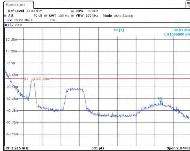
Band25-1.4MHz-16QAM-26683-1RB#5
