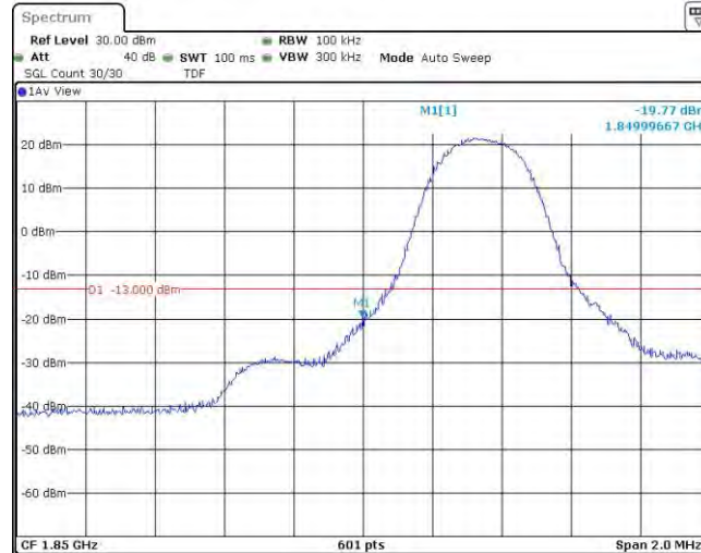
Band25-5MHz-16QAM-26065-1RB#24
