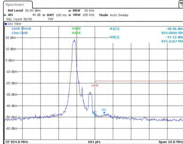
Band26-1.4MHz-16QAM-26783-1RB#5
