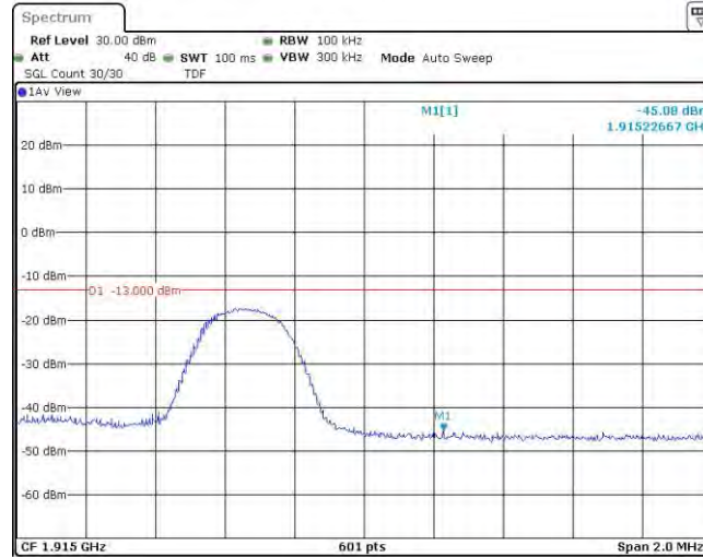
Band25-5MHz-QPSK-26665-1RB#24
