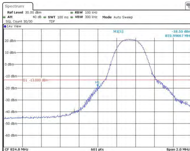
Band5-5MHz-QPSK-20425-1RB#24
