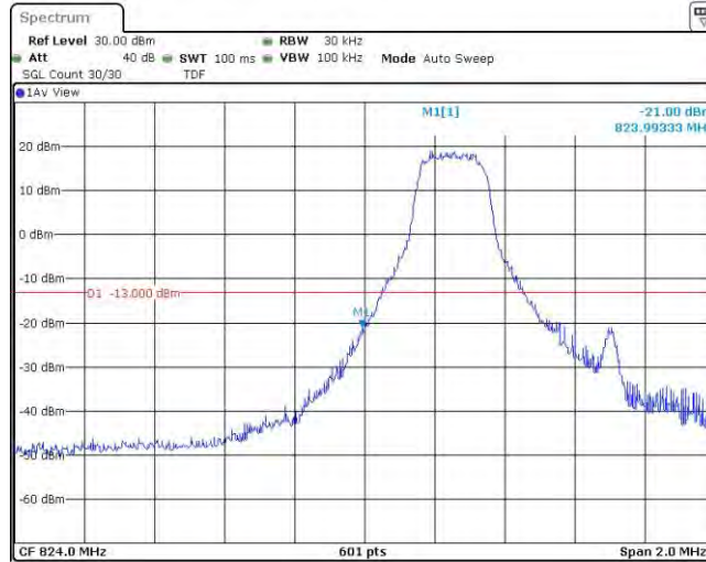
Band26-1.4MHz-QPSK-26797-1RB#5
