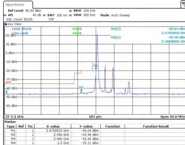
Band7-5MHz-16QAM-20775-1RB#24
