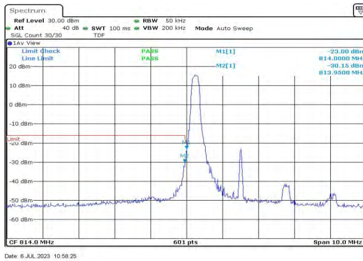
Band26-3MHz-16QAM-26705-1RB#14
