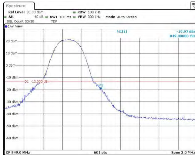
Band26-5MHz-QPSK-27015-25RB#0
