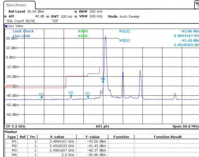
Band7-10MHz-QPSK-20800-1RB#49
