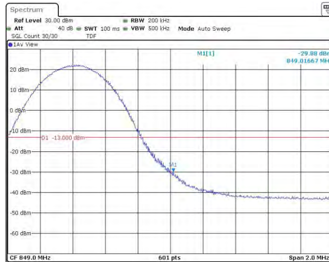
Band26-10MHz-16QAM-26990-50RB#0
