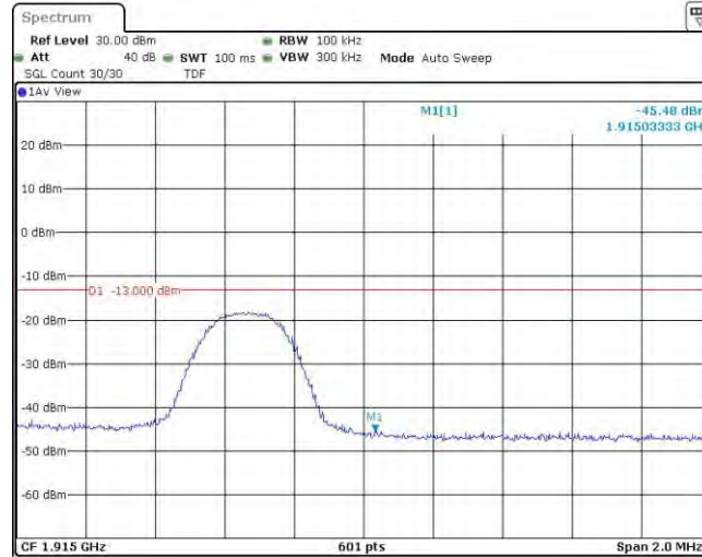
Band25-5MHz-16QAM-26665-1RB#24
