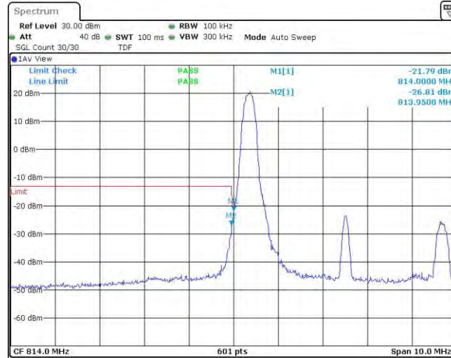
Band26-5MHz-16QAM-26715-1RB#24
