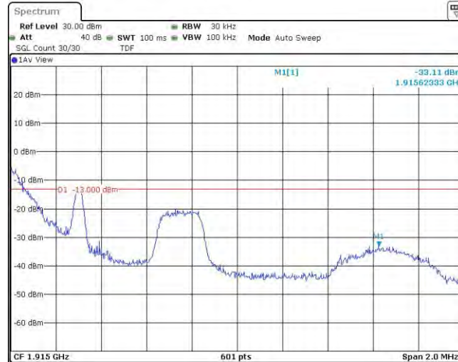
Band25-1.4MHz-QPSK-26683-1RB#5
