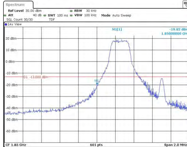
Band25-1.4MHz-16QAM-26047-1RB#5
