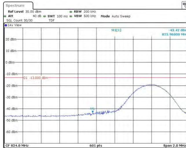
Band26-10MHz-16QAM-26840-50RB#0
