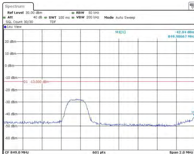
Band26-3MHz-QPSK-27025-1RB#14
