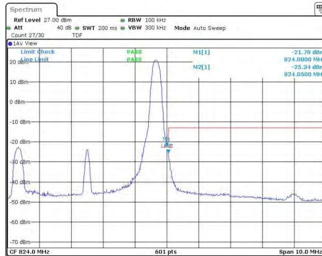
Band26-5MHz-QPSK-26765-25RB#0
