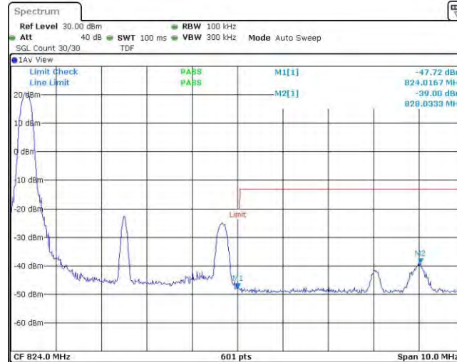
Band26-5MHz-16QAM-26765-1RB#24
