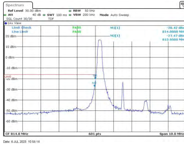
Band26-3MHz-QPSK-26705-1RB#14
