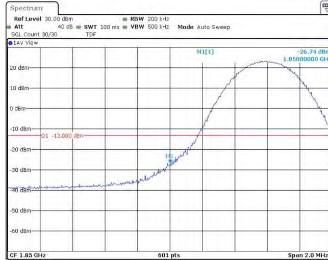
Band25-10MHz-16QAM-26090-1RB#49
