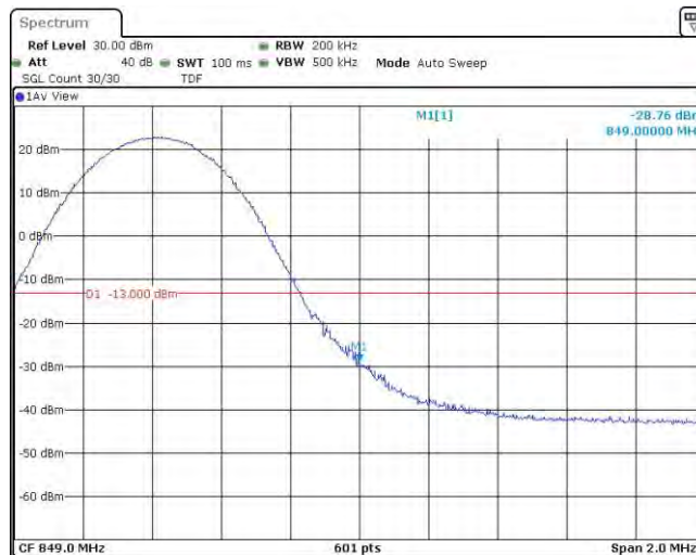
Band5-10MHz-QPSK-20600-50RB#0
