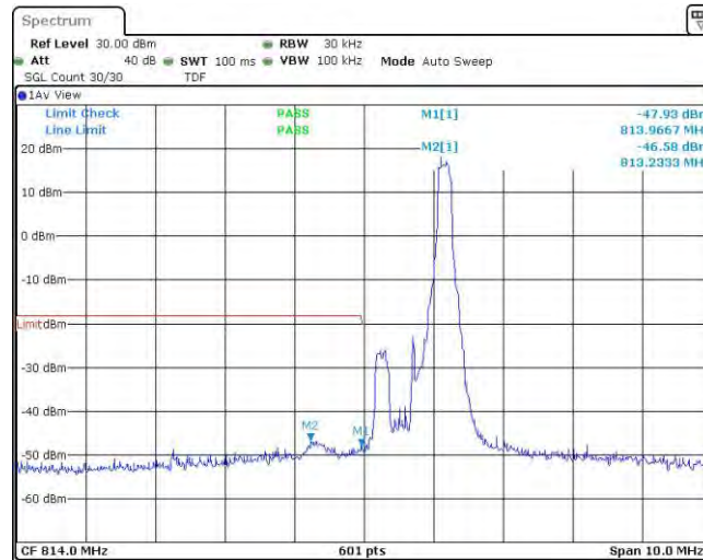
Band26-1.4MHz-16QAM-26697-6RB#0
