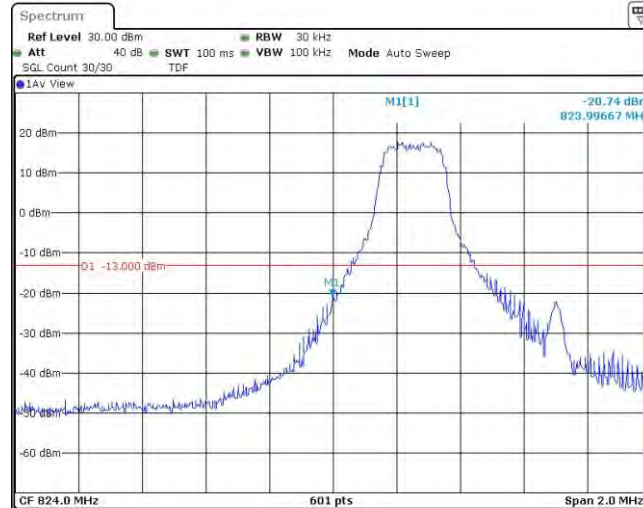
Band26-1.4MHz-16QAM-26797-1RB#5
