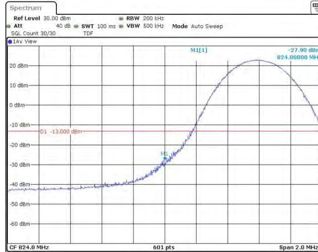
Band26-10MHz-QPSK-26840-1RB#49
