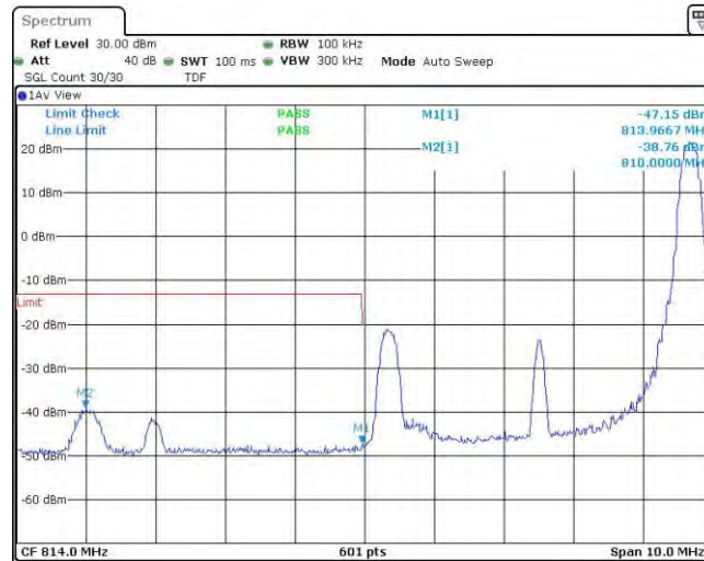
Band26-5MHz-QPSK-26715-25RB#0
