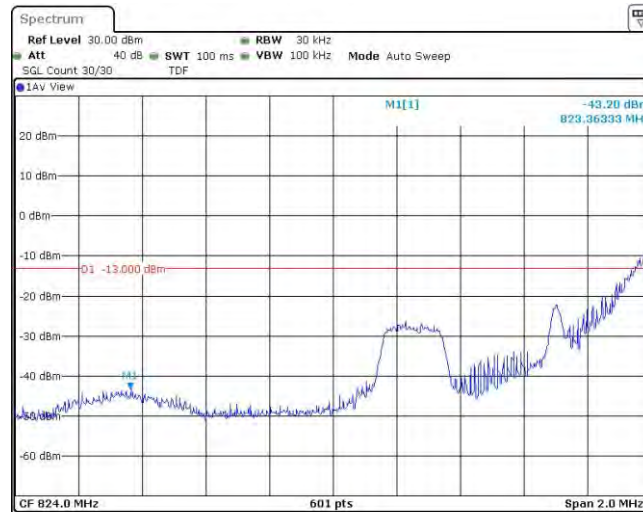
Band26-1.4MHz-16QAM-26797-6RB#0
