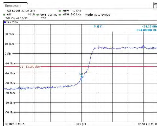
Band5-3MHz-16QAM-20635-1RB#0
