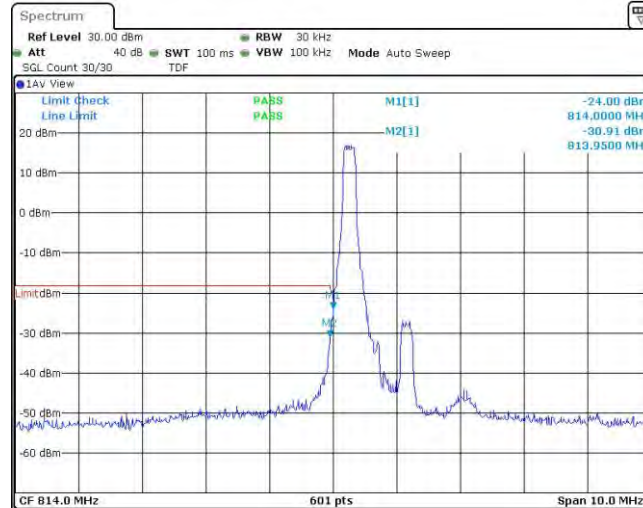
Band26-1.4MHz-16QAM-26697-1RB#5
