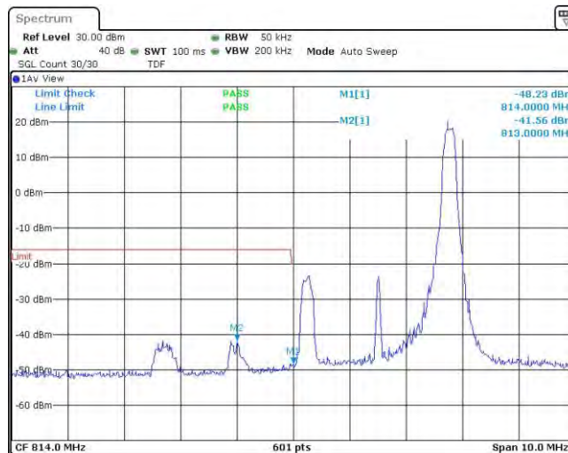
Band26-3MHz-16QAM-26705-1RB#14
