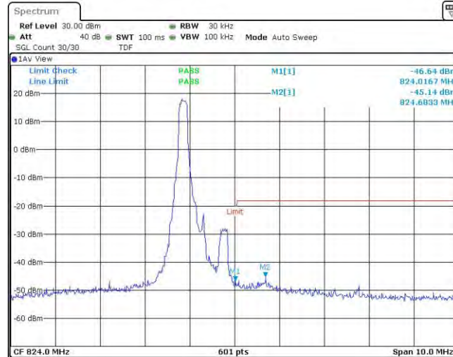
Band26-1.4MHz-QPSK-26783-1RB#5
