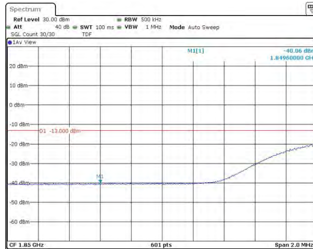
Band25-20MHz-16QAM-26140-100RB#0
