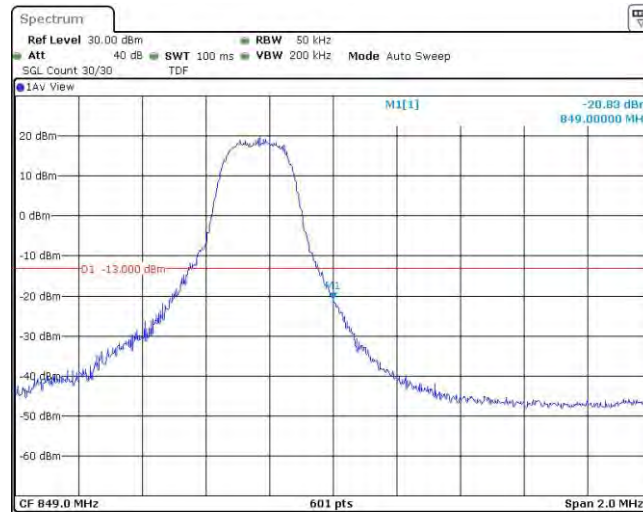
Band26-3MHz-16QAM-27025-15RB#0
