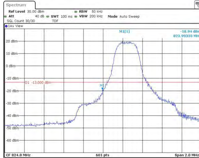
Band5-3MHz-16QAM-20415-1RB#14
