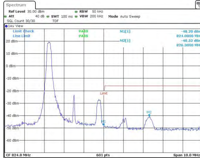
Band26-3MHz-QPSK-26775-1RB#14
