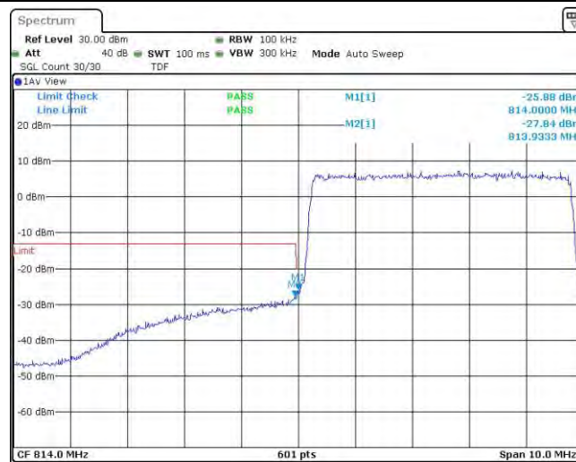
Band26-5MHz-16QAM-26765-1RB#0
