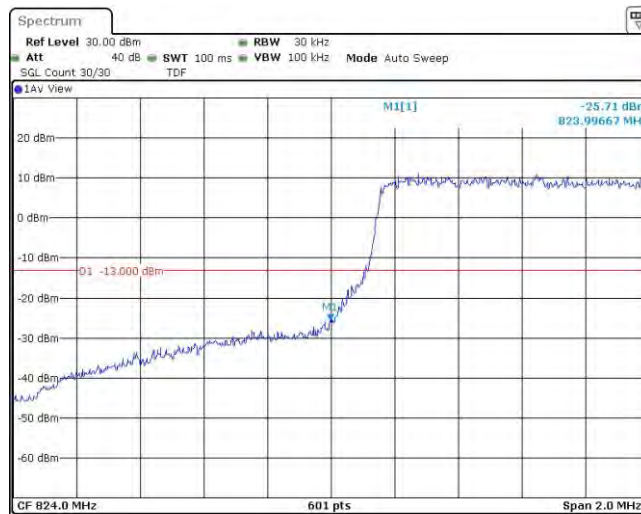
Band26-1.4MHz-QPSK-27033-1RB#0
