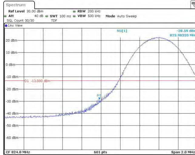
Band26-10MHz-16QAM-26840-1RB#49
