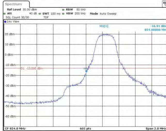
Band26-3MHz-QPSK-26805-1RB#14
