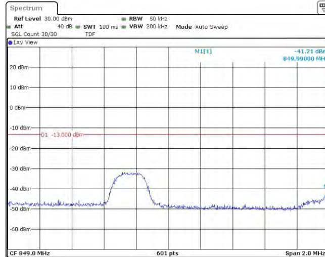
Band5-3MHz-16QAM-20635-1RB#14
