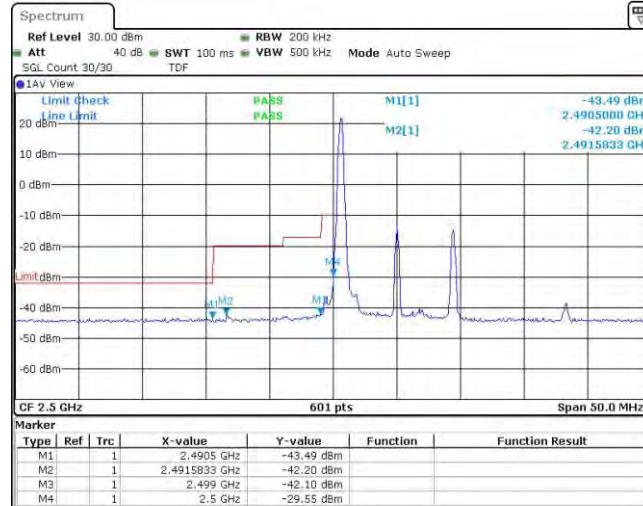
Band7-10MHz-16QAM-20800-1RB#49
