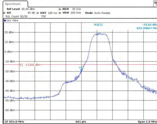
Band26-3MHz-16QAM-26805-1RB#14
