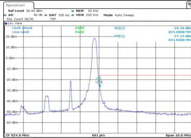
Band26-3MHz-QPSK-26775-1RB#14
