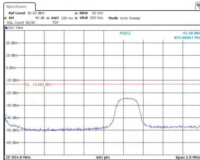
Band26-3MHz-QPSK-26805-15RB#0
