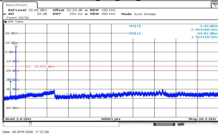
CSS 812kHz_Ant1_2404_1000~26500
