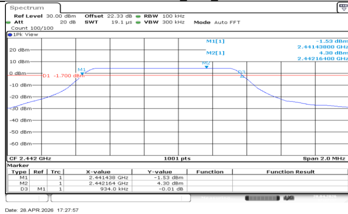
CSS 812kHz_Ant1_2442
