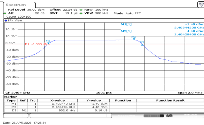
CSS 812kHz_Ant1_2404
