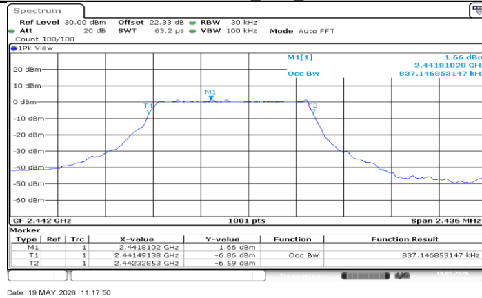
CSS 812kHz_Ant1_2442
