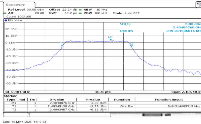
CSS 812kHz_Ant1_2404
