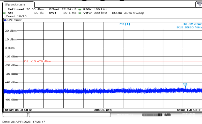
CSS 812kHz_Ant1_2404_30~1000
