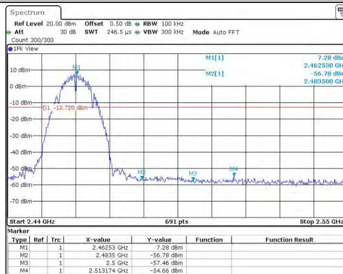
11B_Ant2_High_2462
