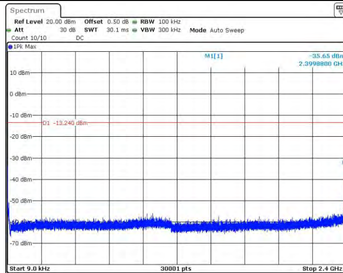
11N20_Ant1_2412_0.009~2400
