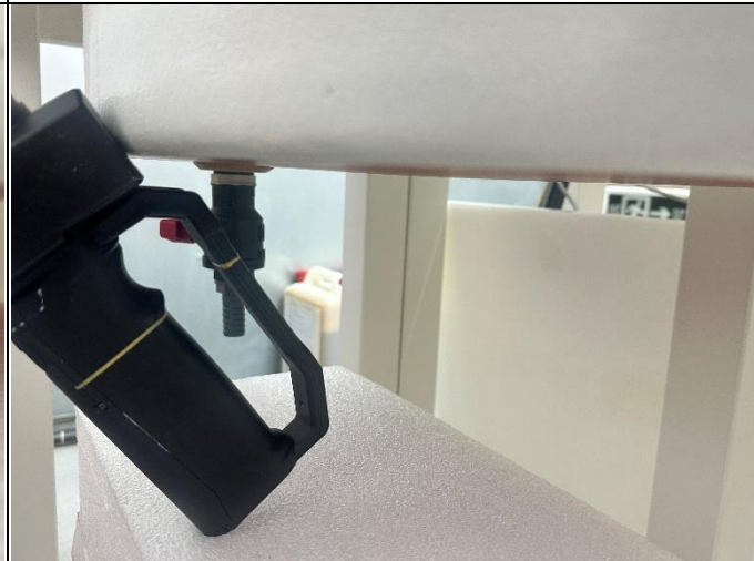
Test Position 4 of EUT with 1.0 cm Gap
