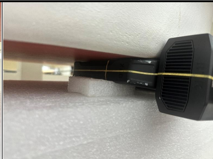
Test Position 2 of EUT with 0 cm Gap
