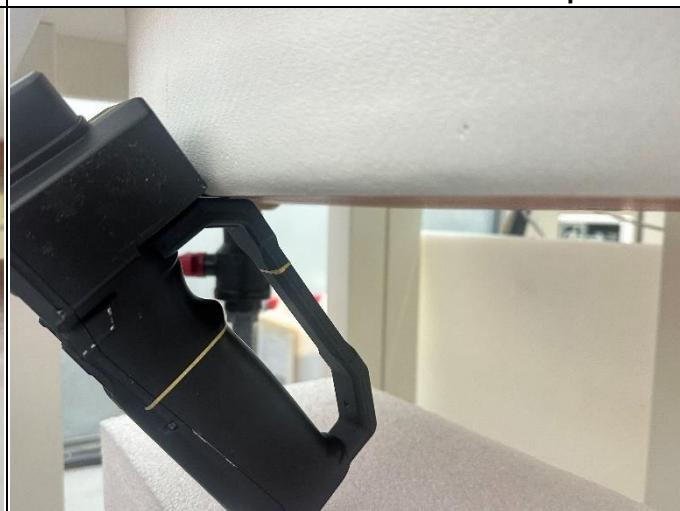
Test Position 4 of EUT with 0 cm Gap
