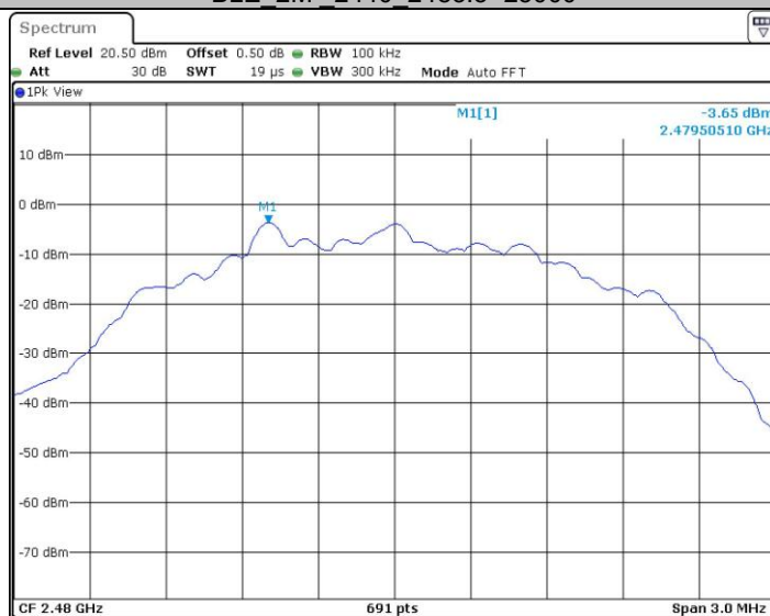
BLE_2M_2480_0~Reference
