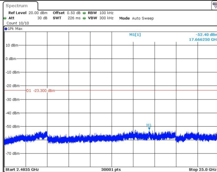
BLE_1M_2480_2483.5~25000
