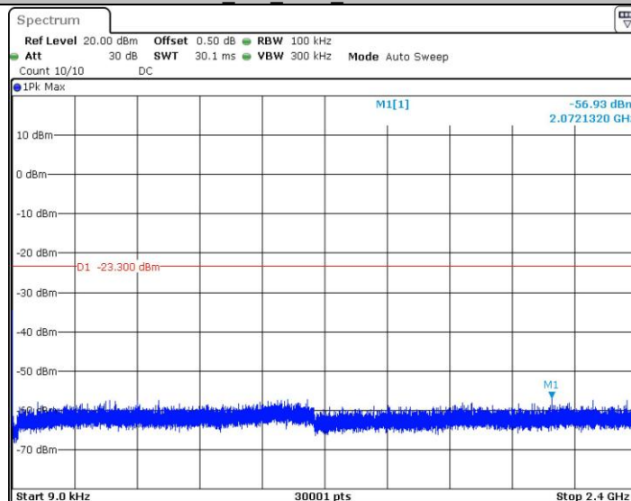
BLE_1M_2480_0.009~2400
