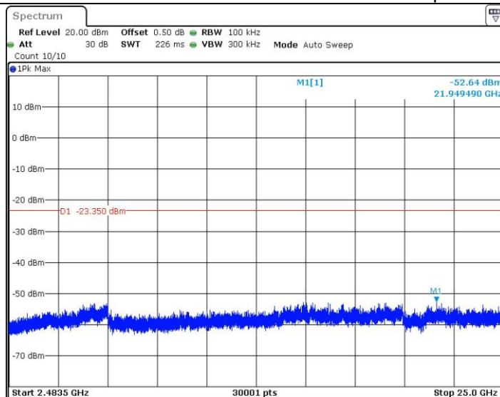
BLE_2M_2440_2483.5~25000
