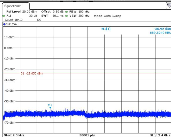
BLE_2M_2480_0.009~2400
