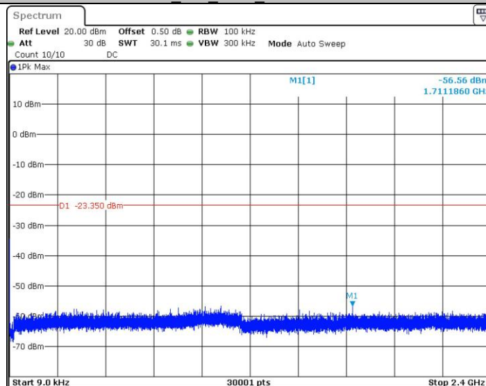
BLE_2M_2440_0.009~2400
