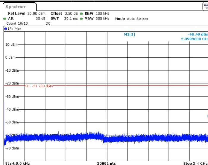
BLE_2M_2402_0.009~2400
