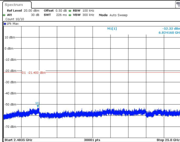
BLE_1M_2402_2483.5~25000
