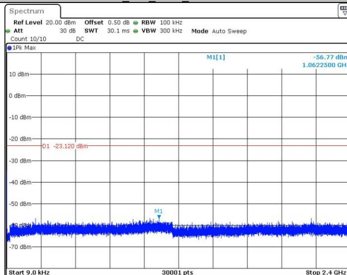
BLE_1M_2440_0.009~2400
