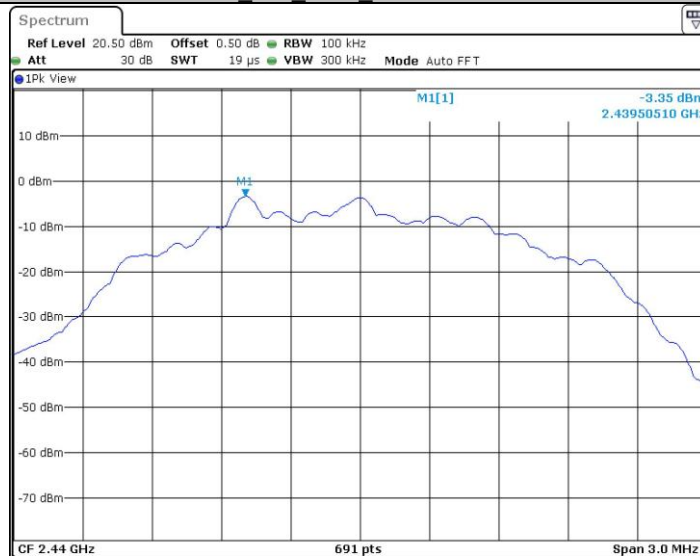
BLE_2M_2440_0~Reference
