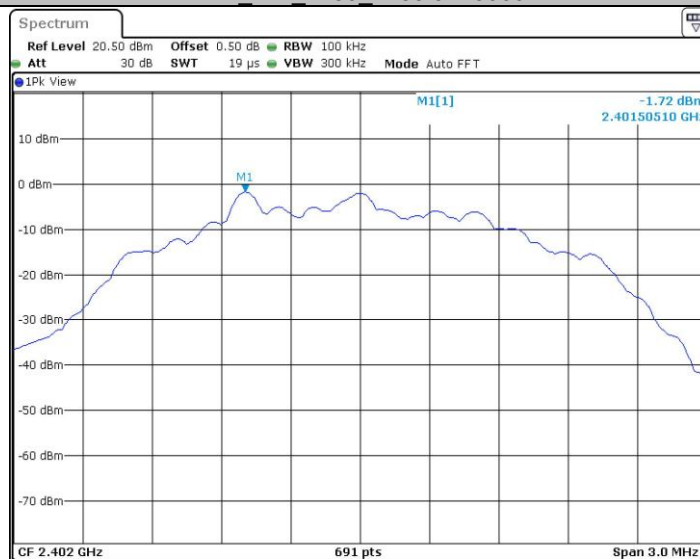
BLE_2M_2402_0~Reference
