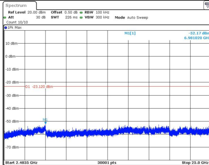
BLE_1M_2440_2483.5~25000
