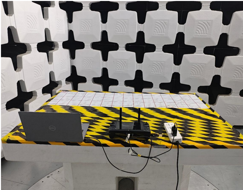
Back View (Below 1GHz)
