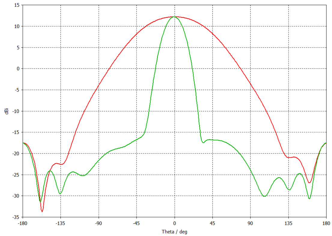
Fig2.Antenna1,Gain=12.2dBi Antenna type: Integrated Antenna
