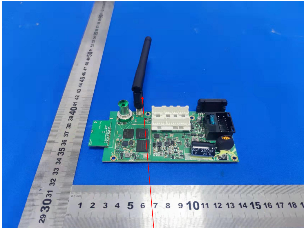
External antenna
