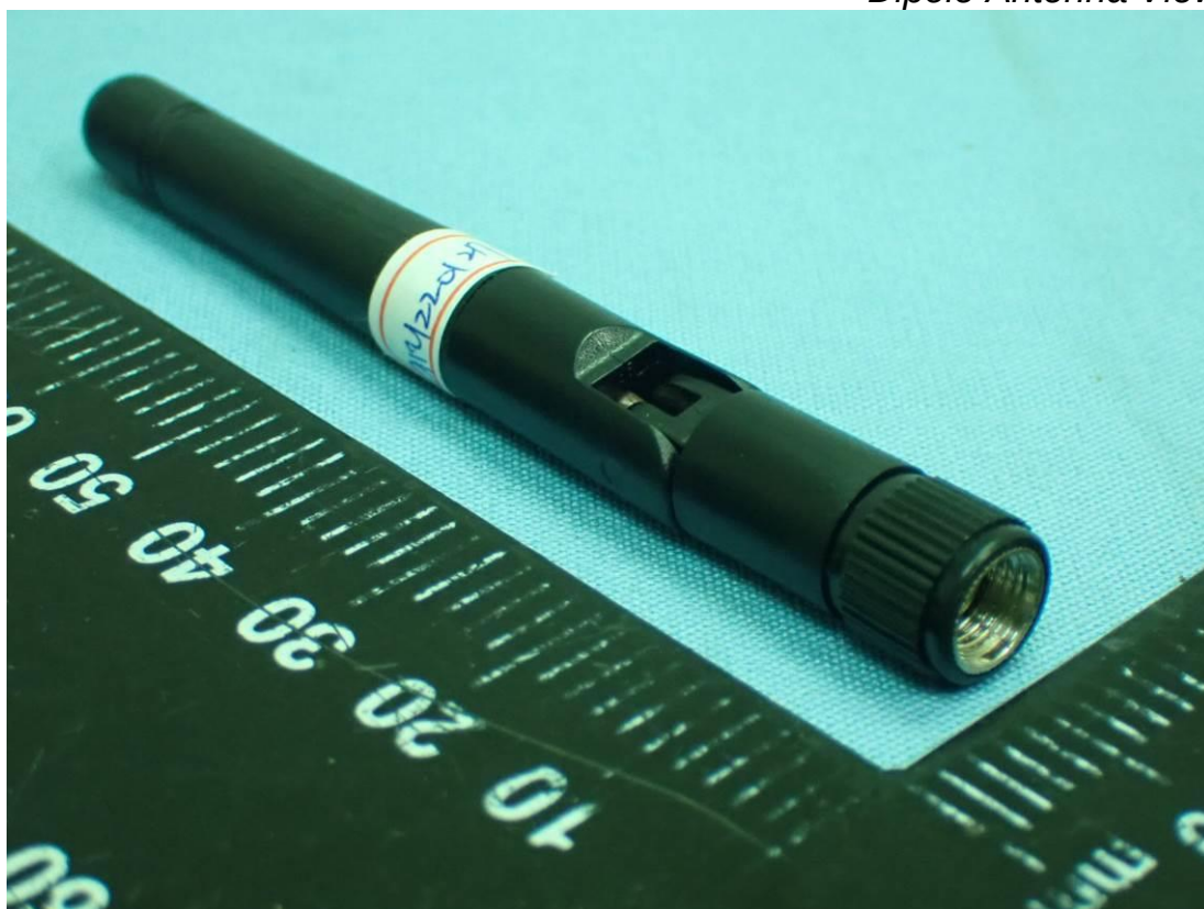
Figure 9 Dipole Antenna View
