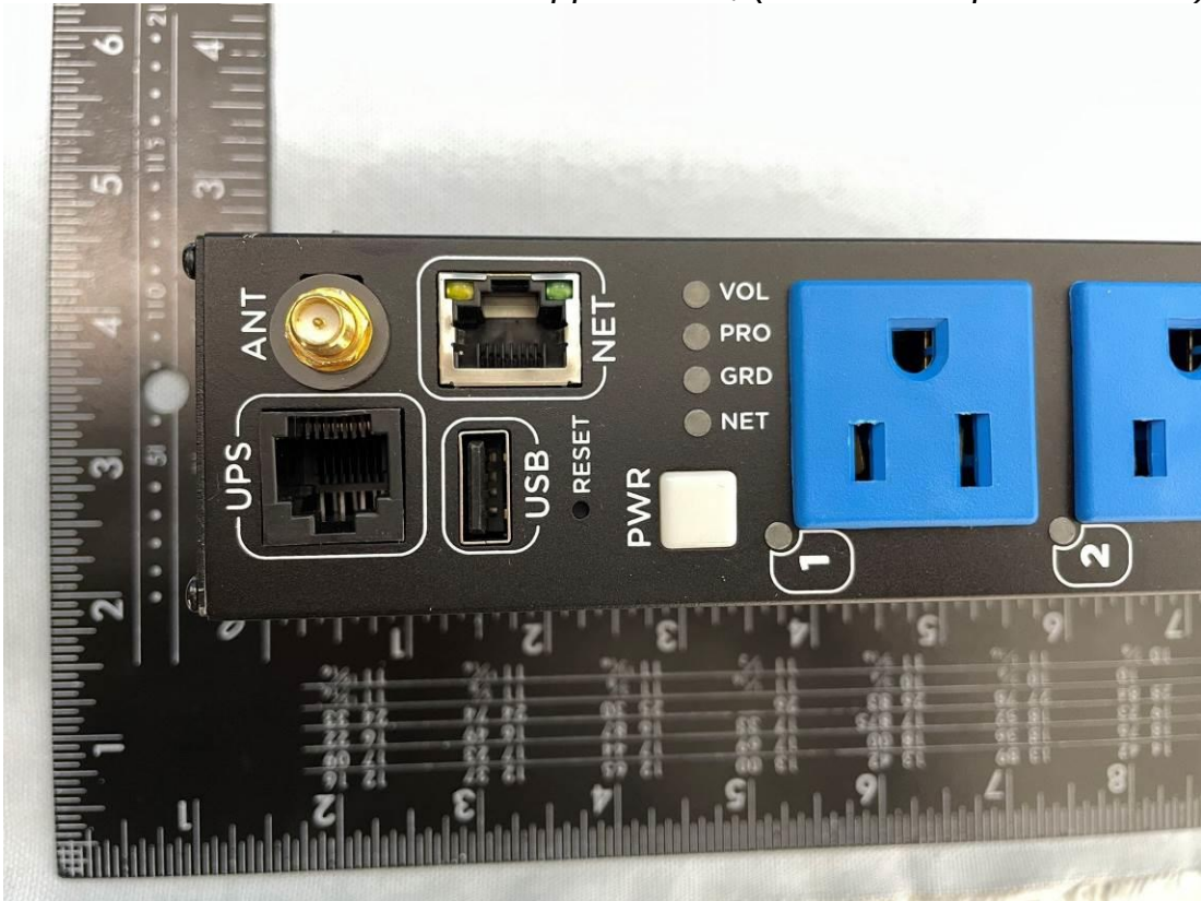
Figure 8 General Appearance, (Removed Dipole Antenna)
