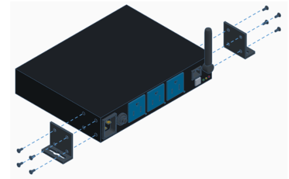
Surface Mount Step 1
